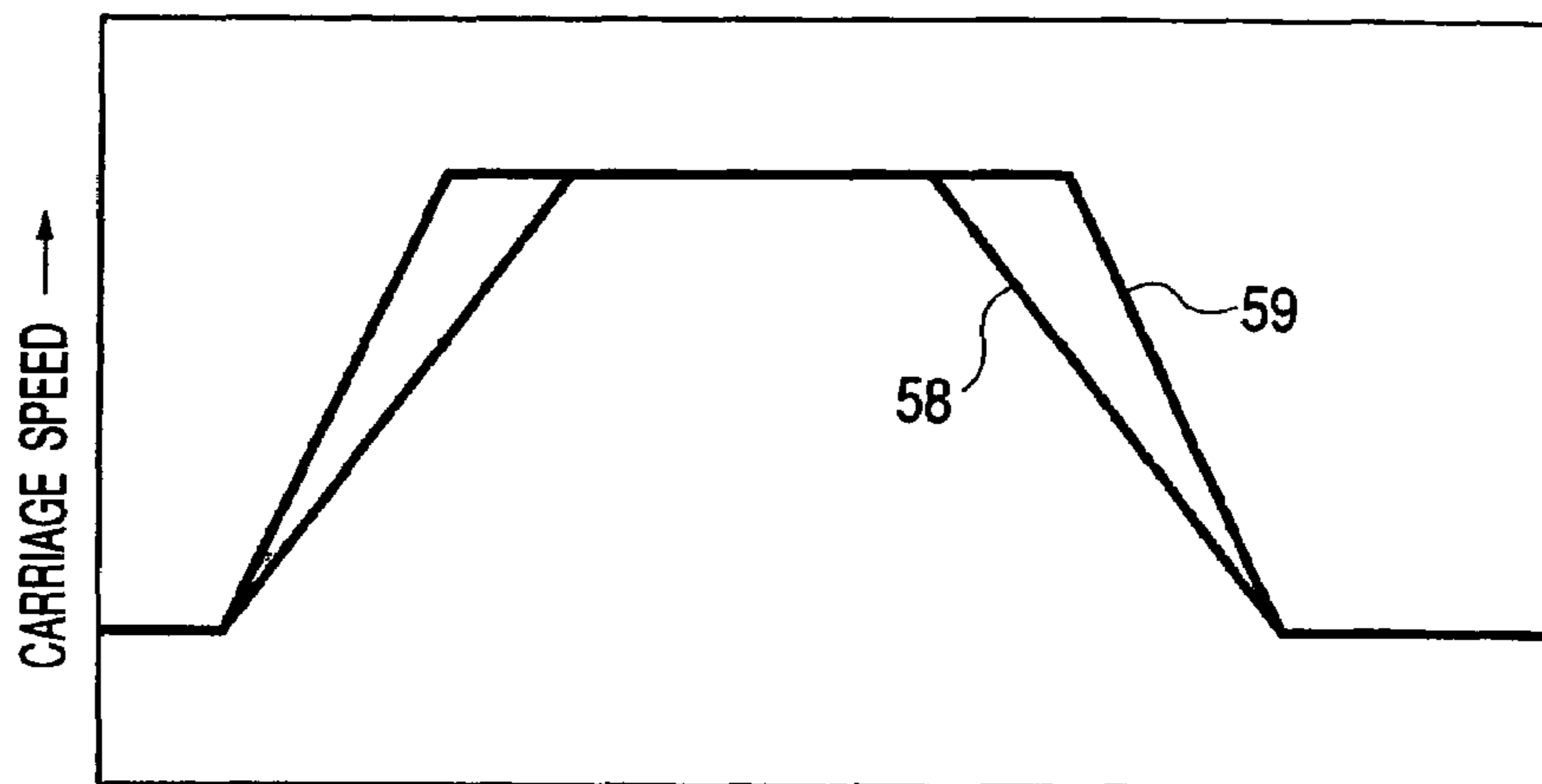
OPERATION RANGE OF CARRIAGE DURING STEP-PRINTING OPERATION
