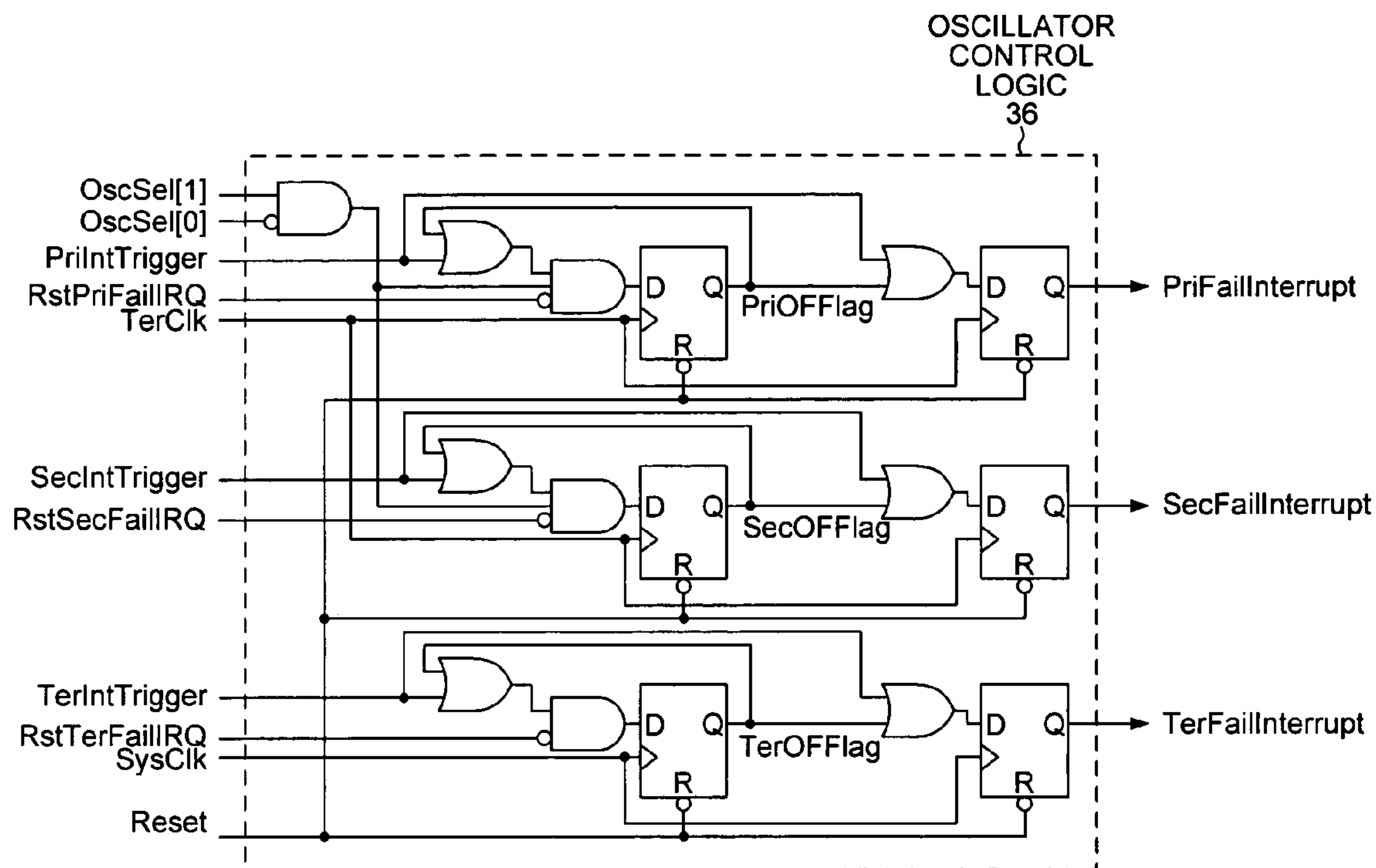
OSCILLATOR CONTROL LOGIC FIG. 5
