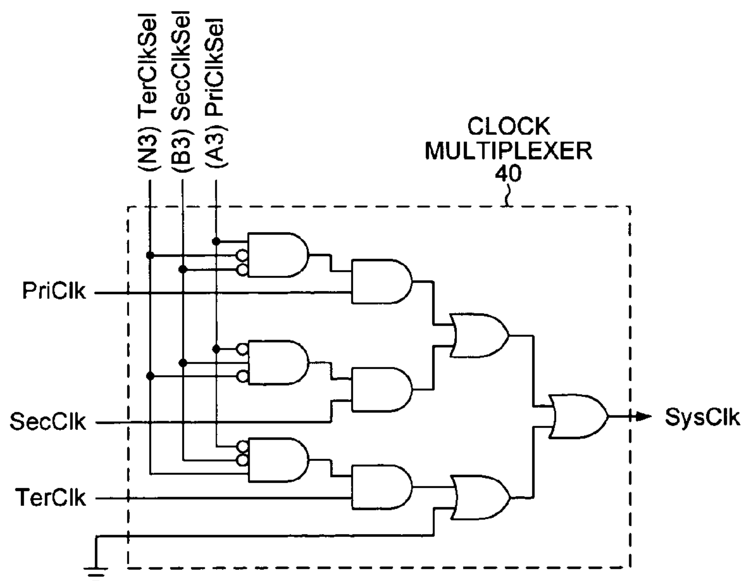
CLOCK MULTIPLEXER FIG. 6
