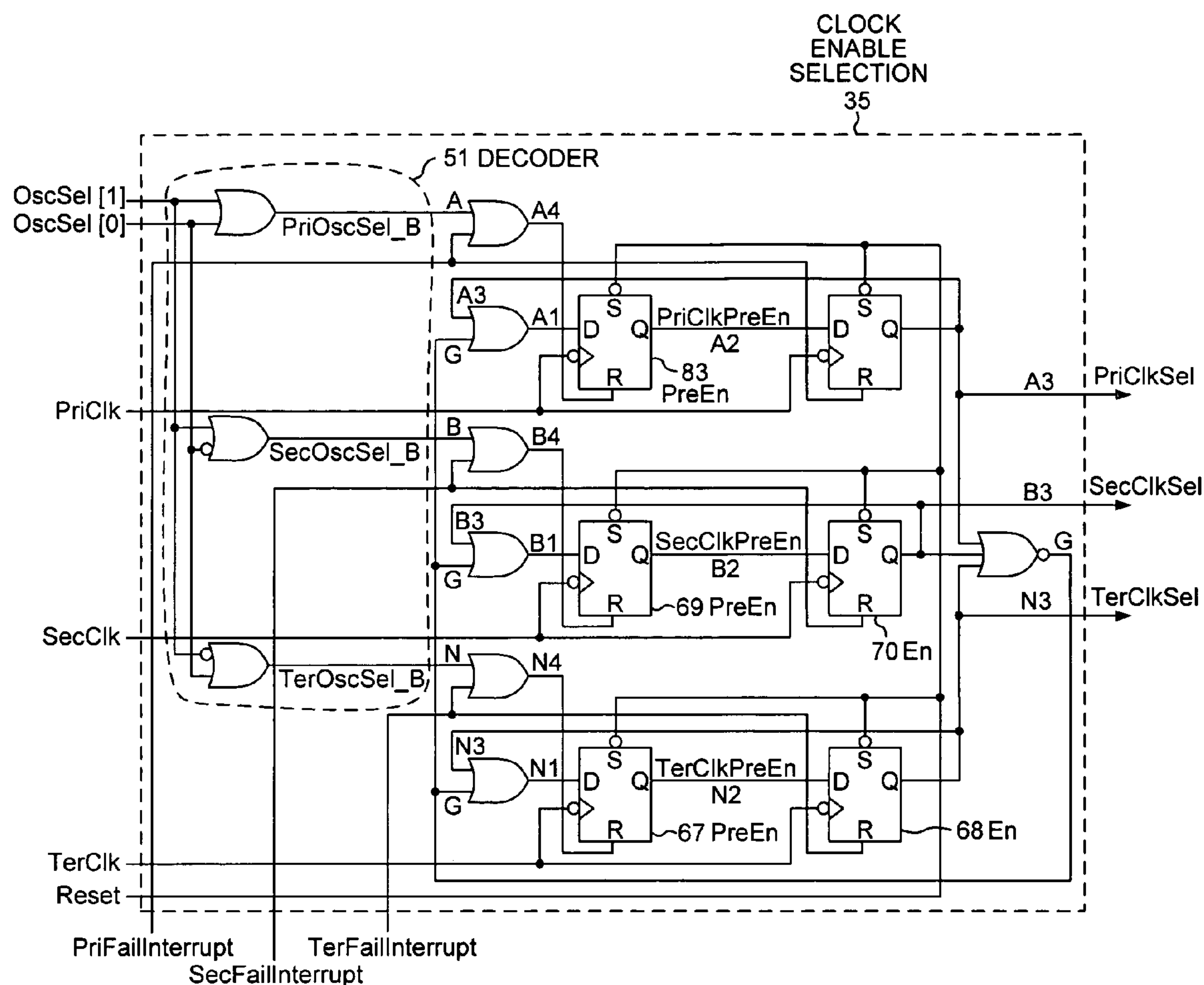
CLOCK ENABLE SELECTION FIG. 3
