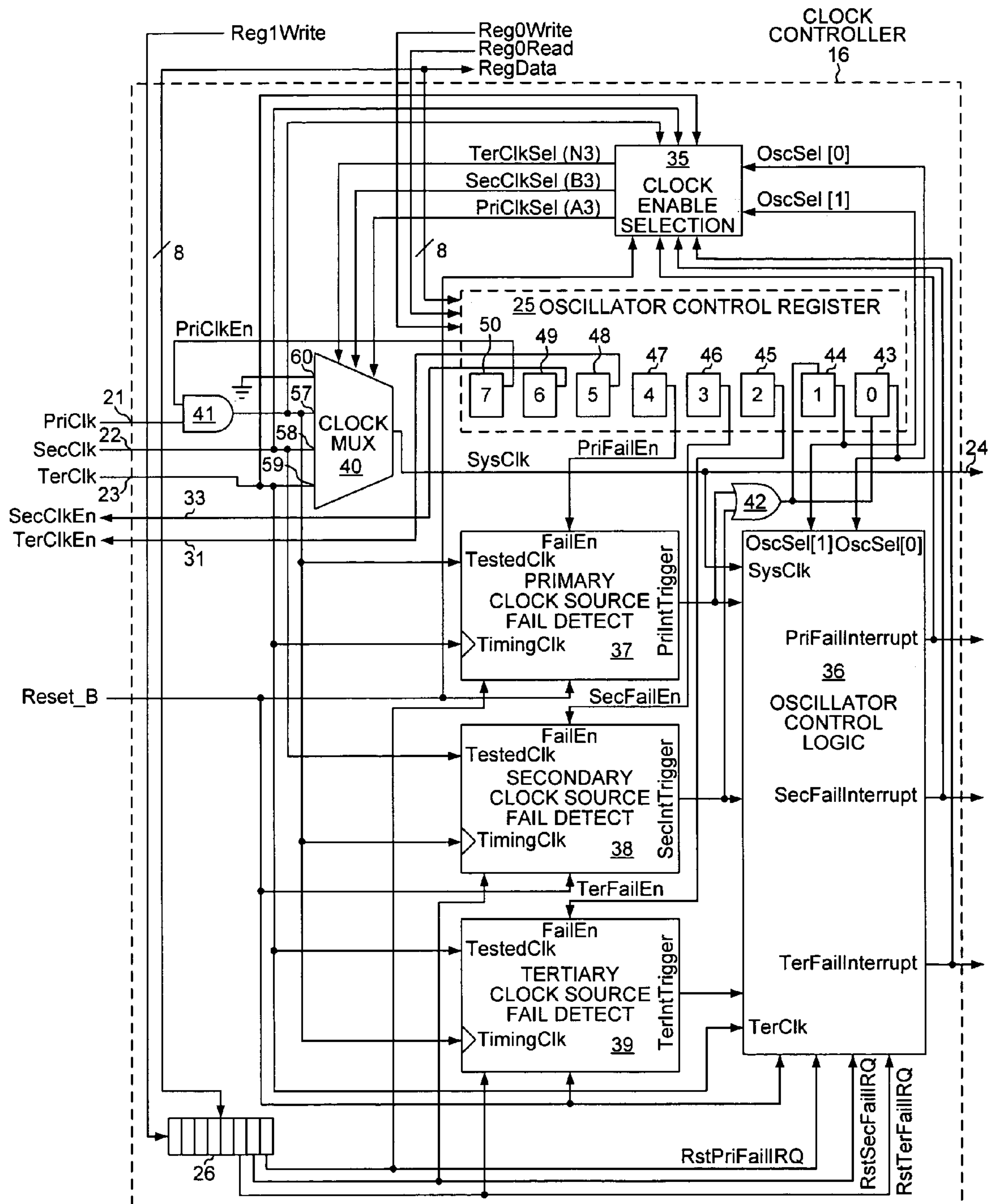
CLOCK CONTROLLER FIG. 2
