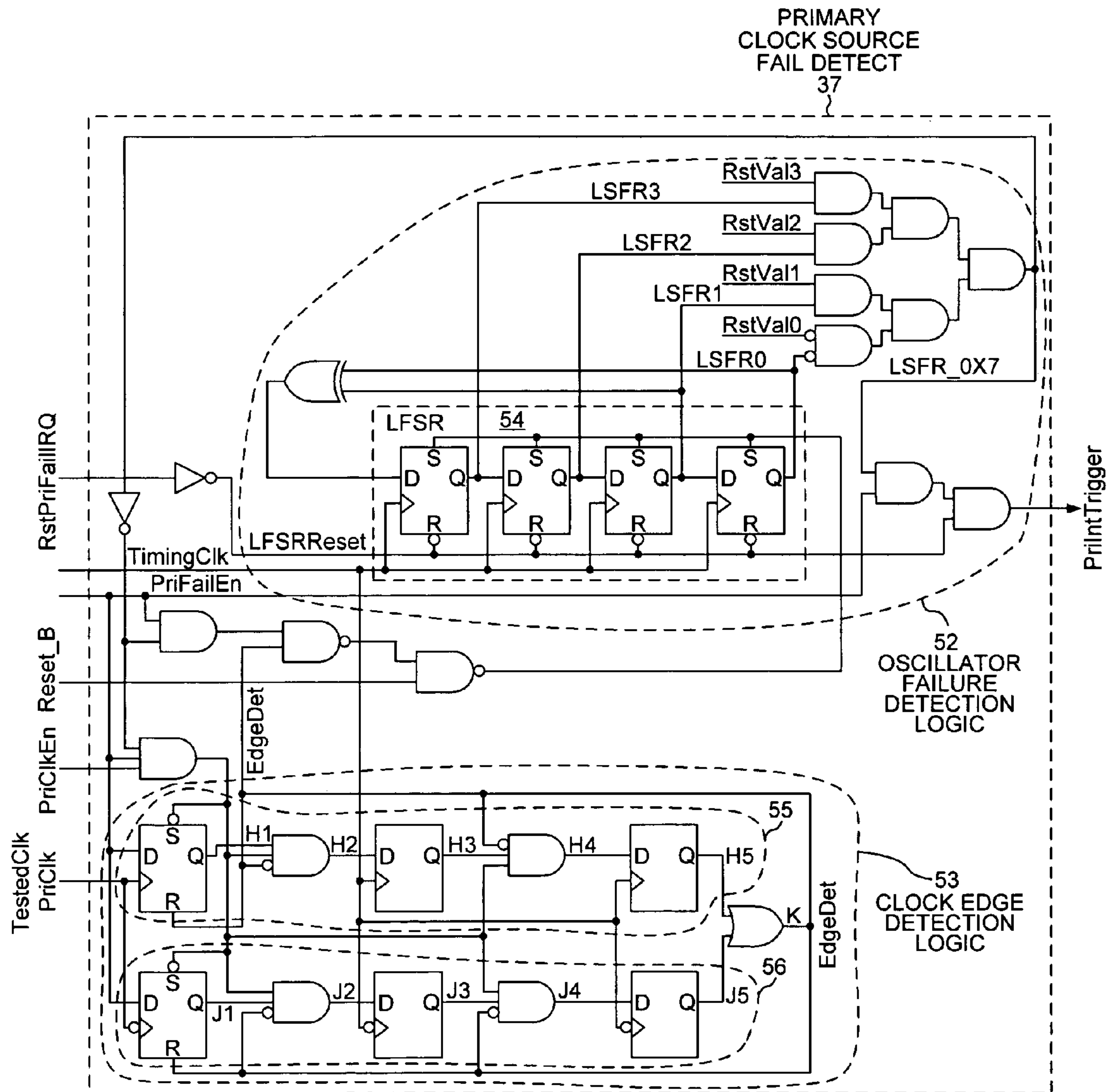
PRIMARY CLOCK SOURCE FAIL DETECT FIG. 4
