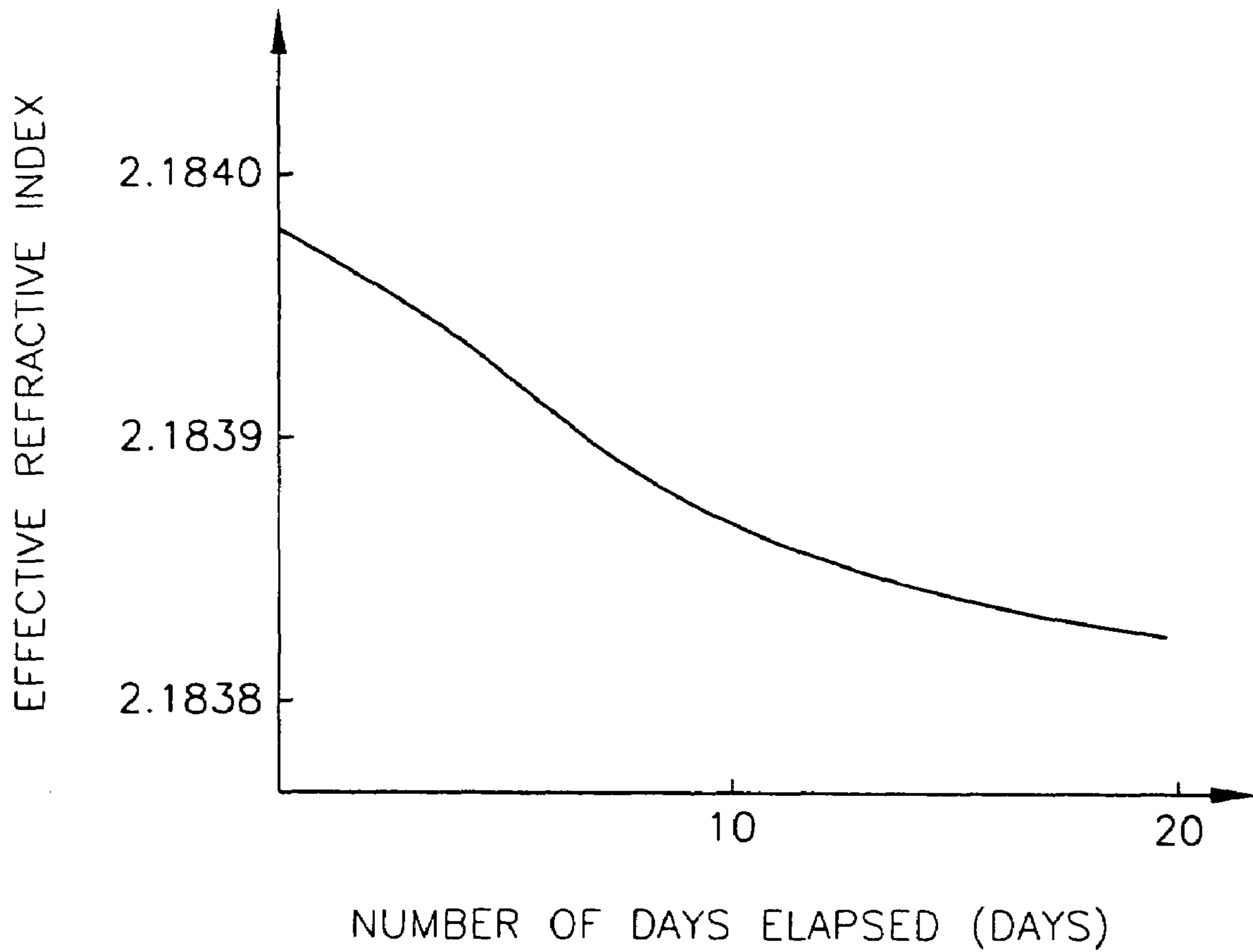
FIG. 6 (Prior Art)
