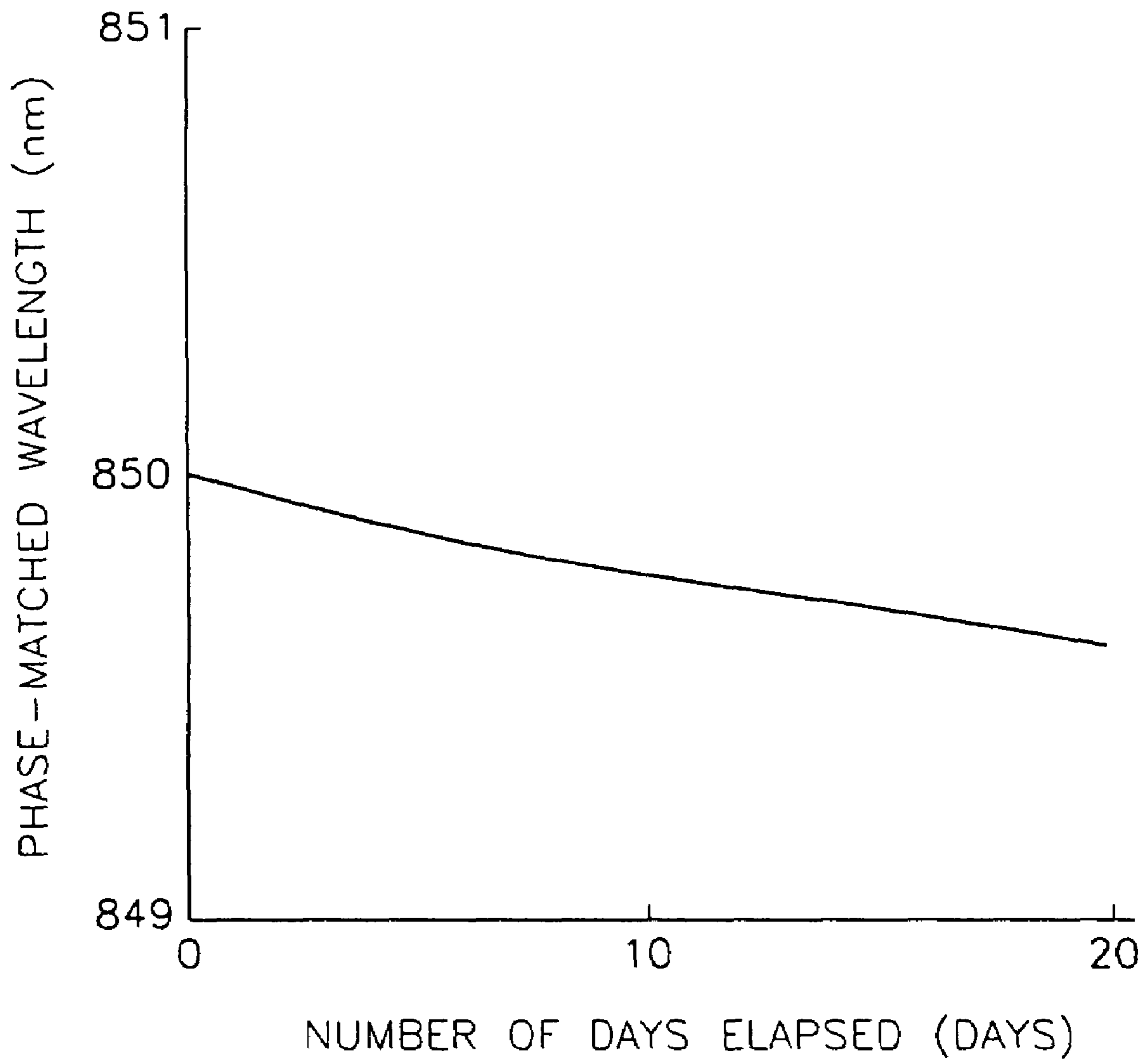
FIG. 5 (Prior Art)
