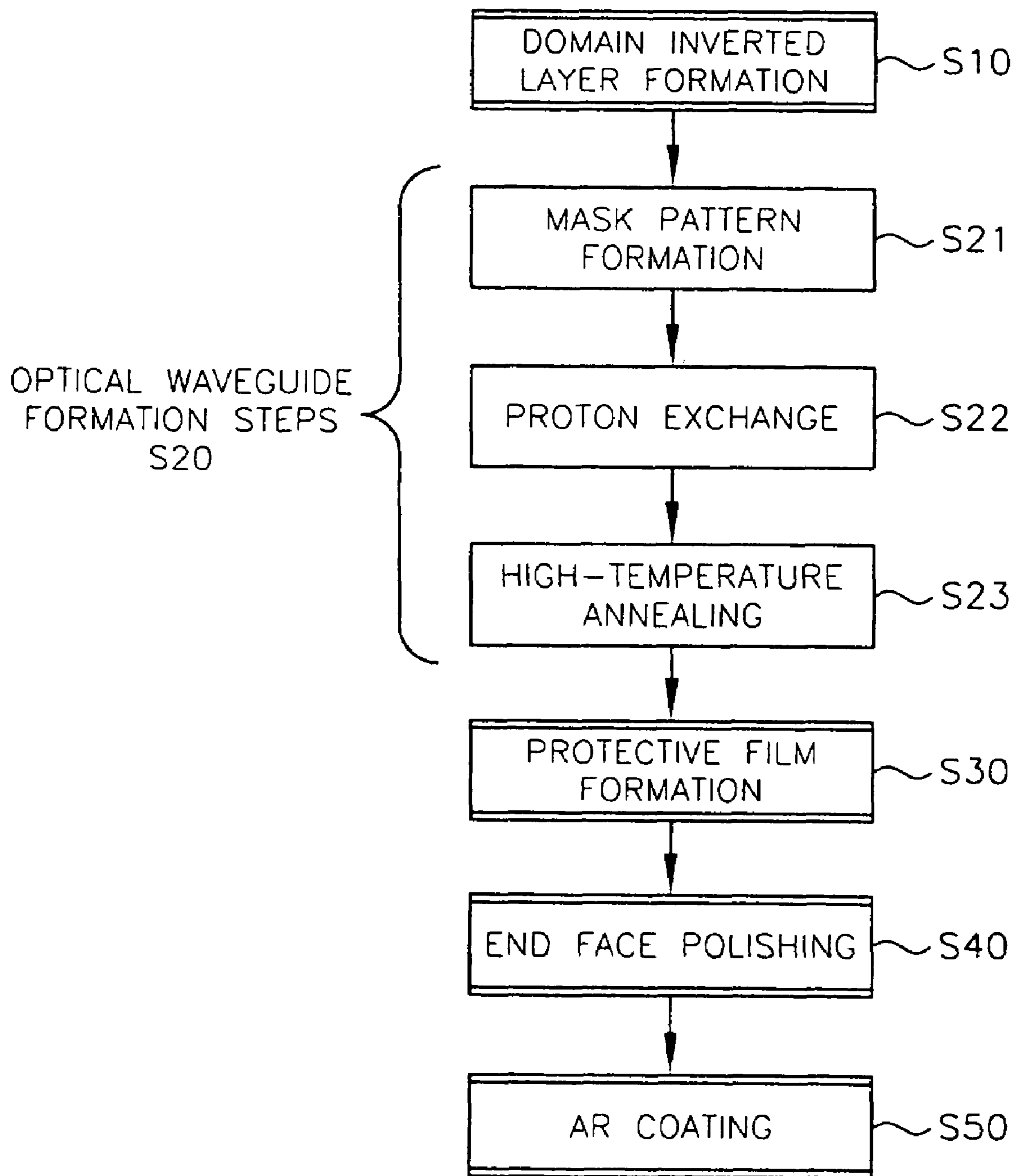
FIG. 3 (Prior Art)
