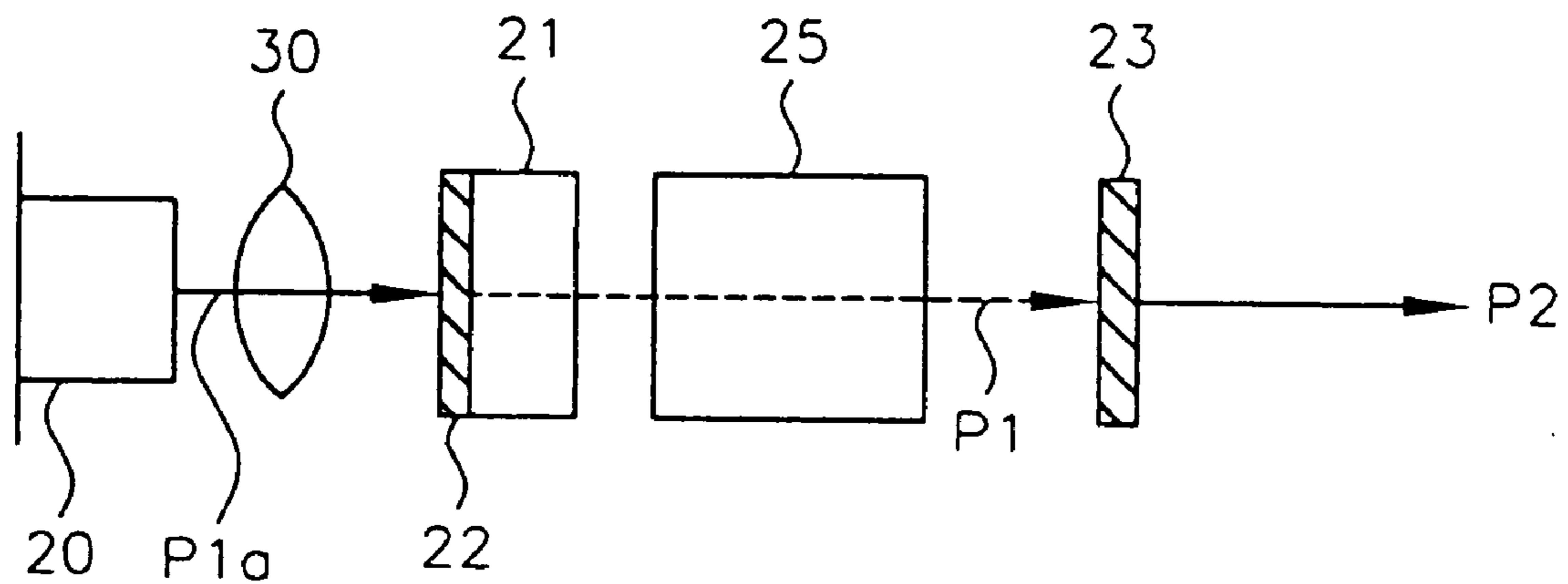
FIG. 1 (Prior Art)
