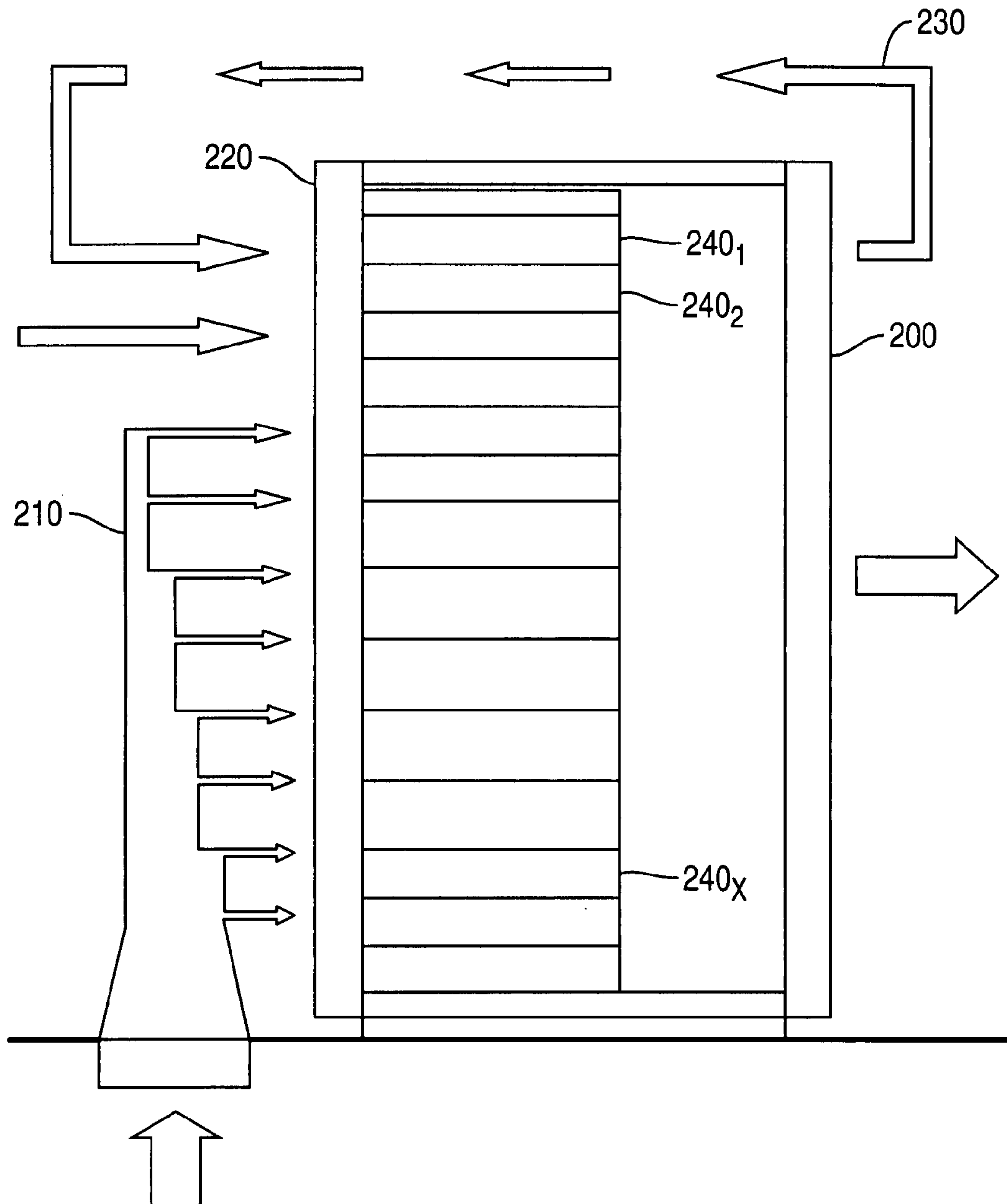
FIG. 2 PRIOR ART
