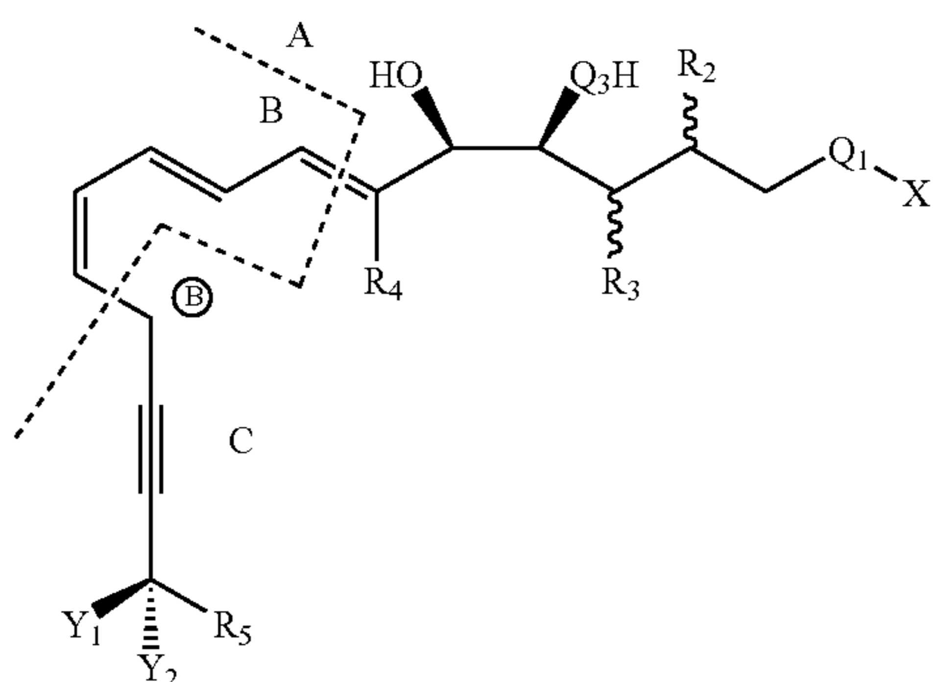
Scheme II.
