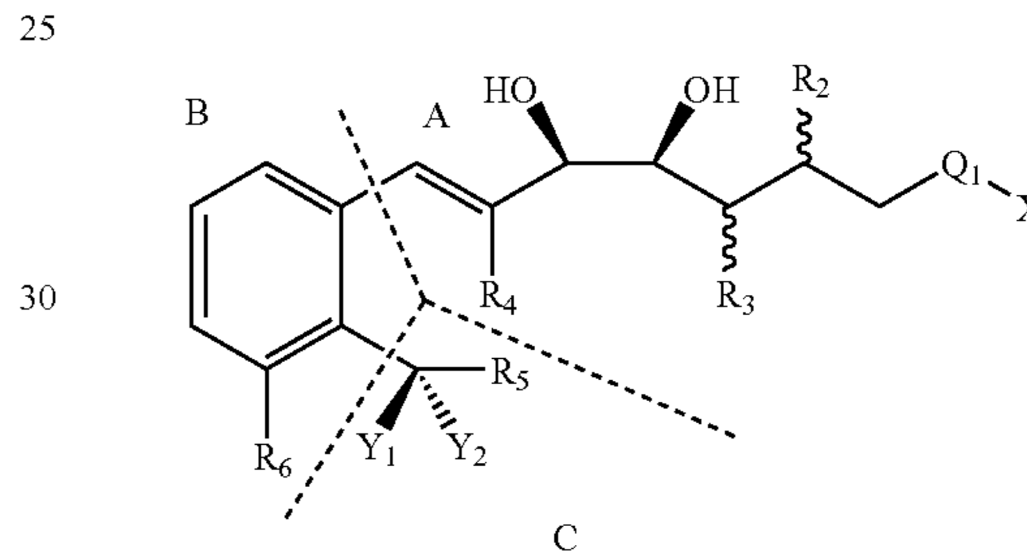
Scheme III.
