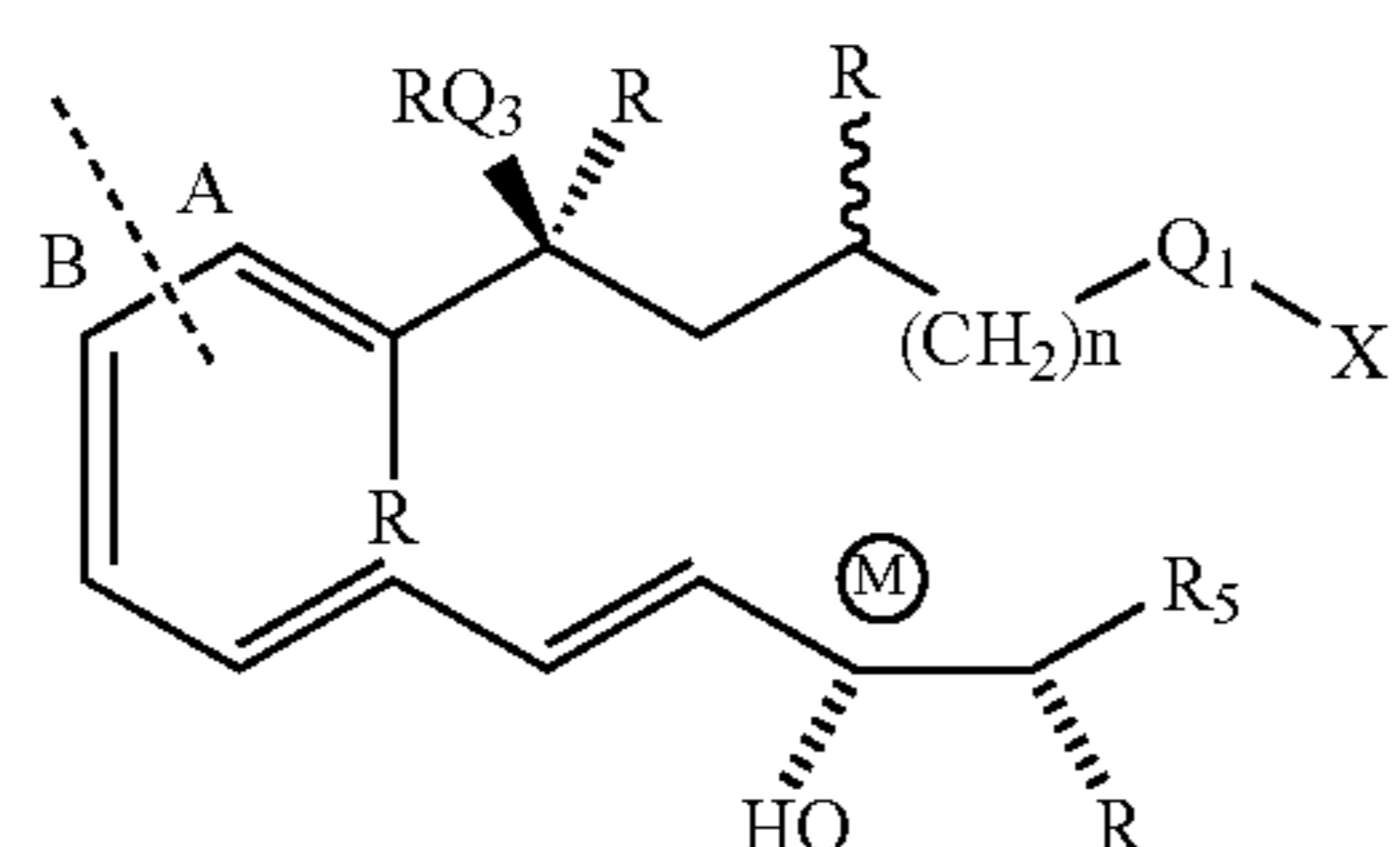
Scheme IV
