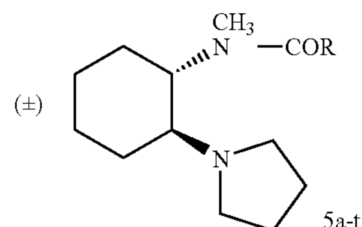
Compounds of Formula IV
