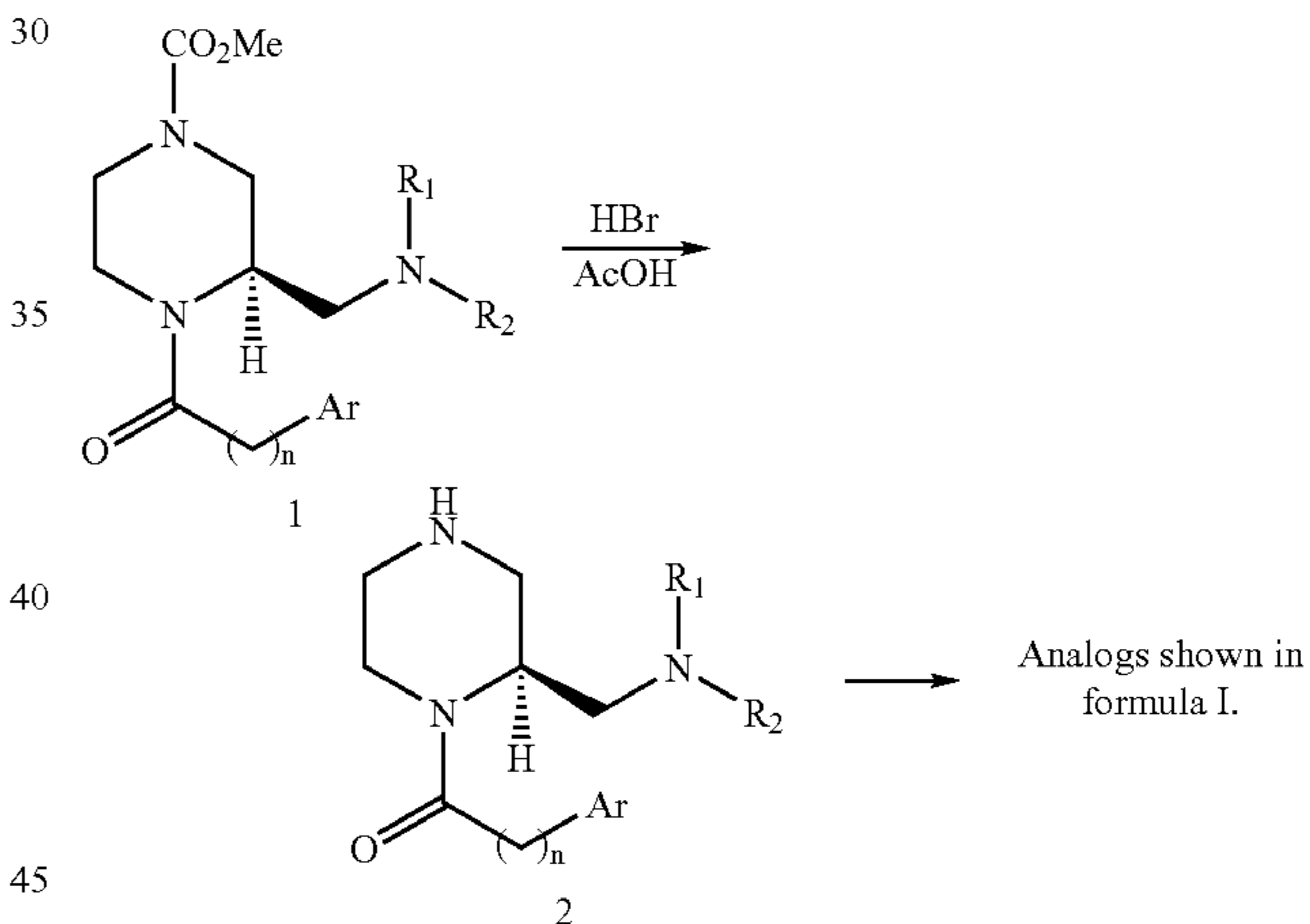
Scheme 1
