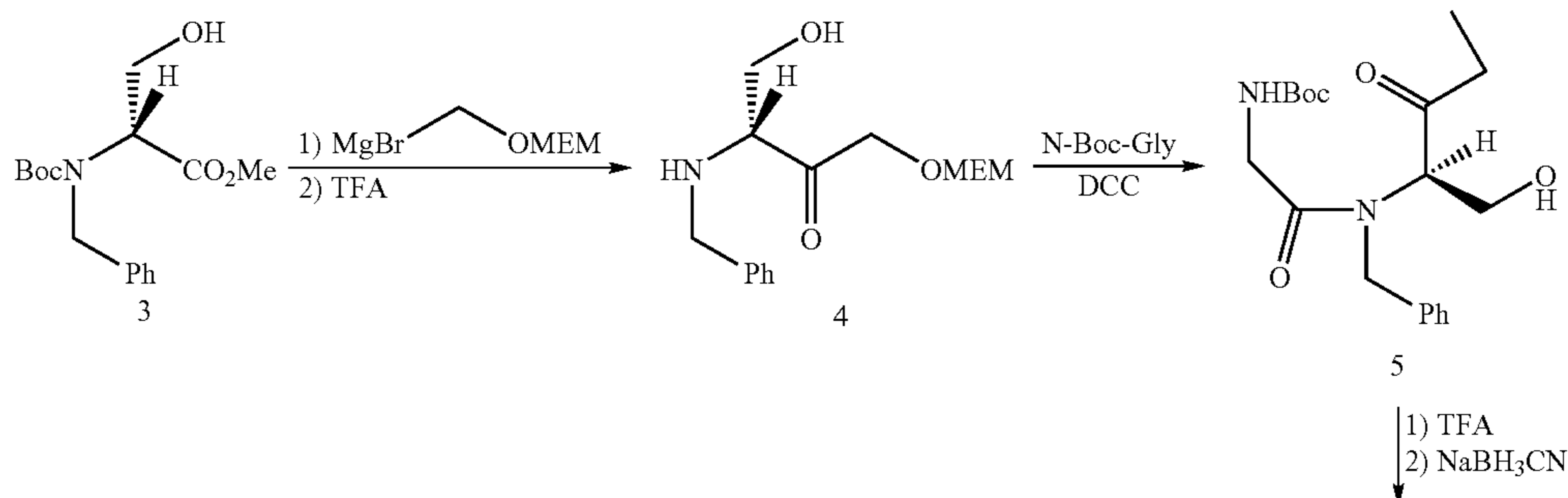
Scheme 2.
