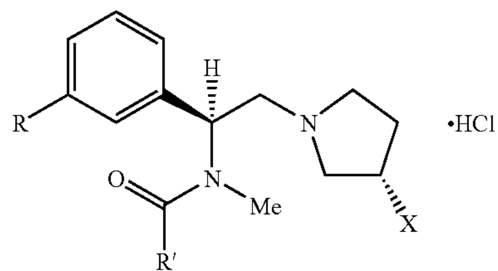
Compounds of Formula III
