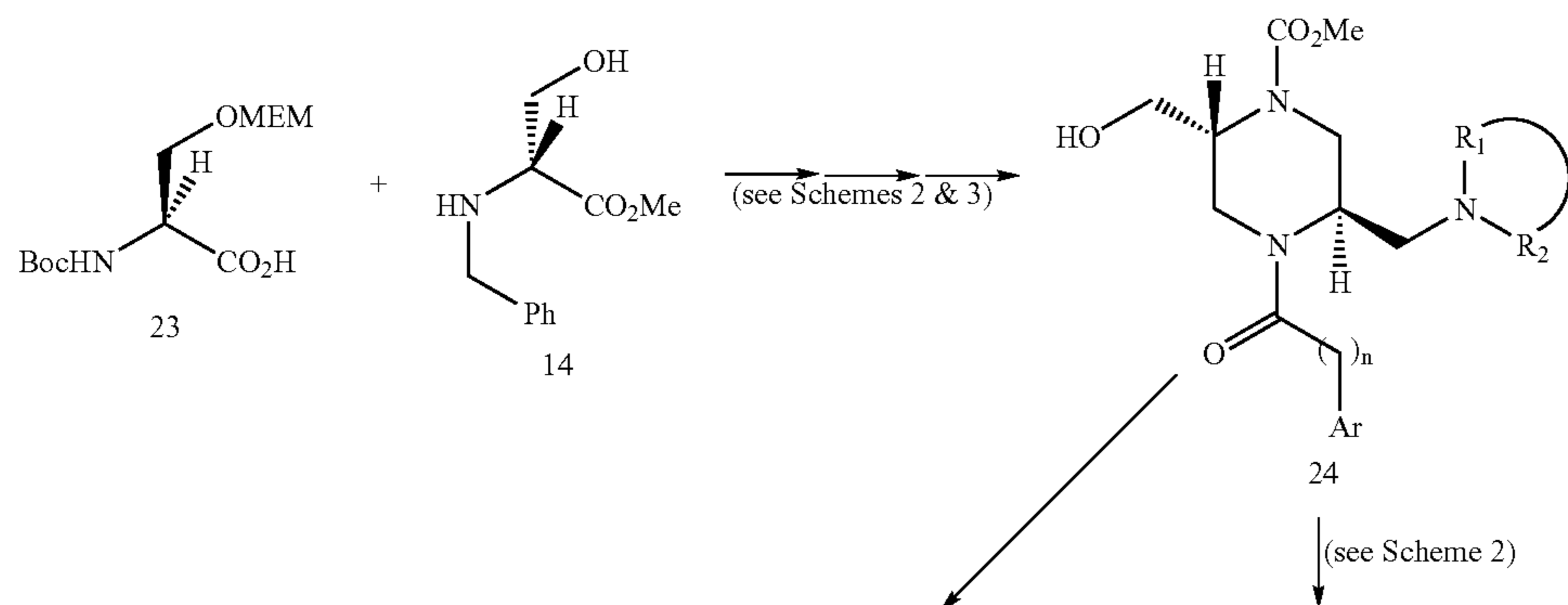
Scheme 4
