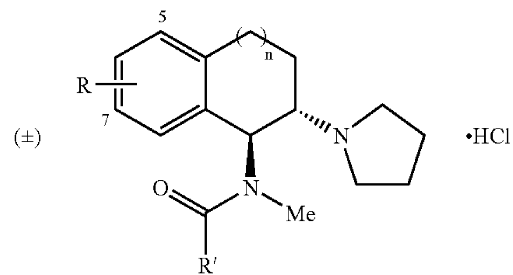
Compounds of Formula II
