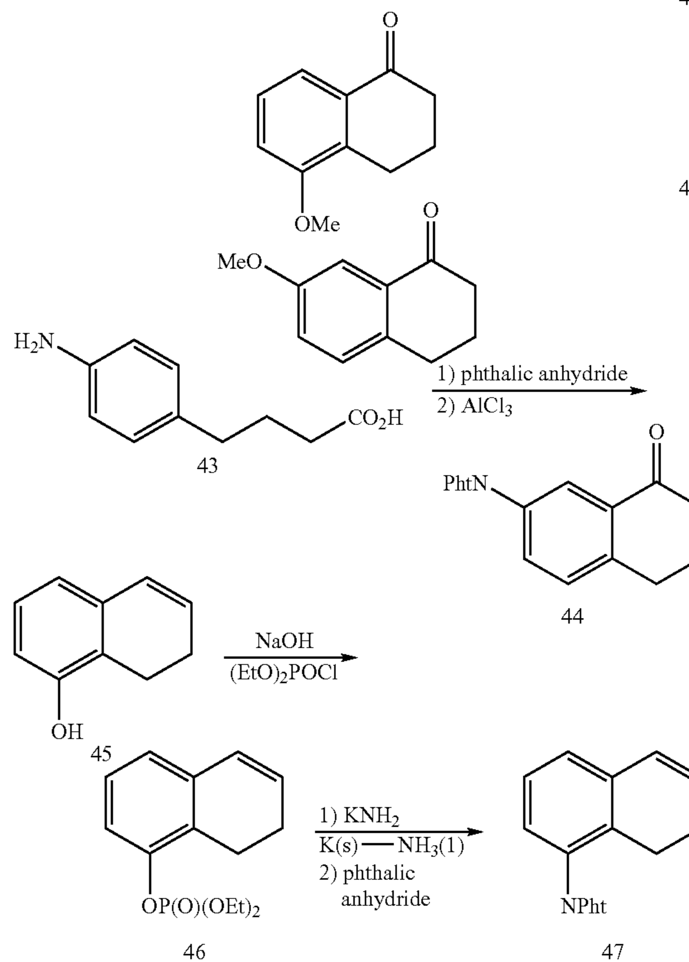
Scheme 5.
