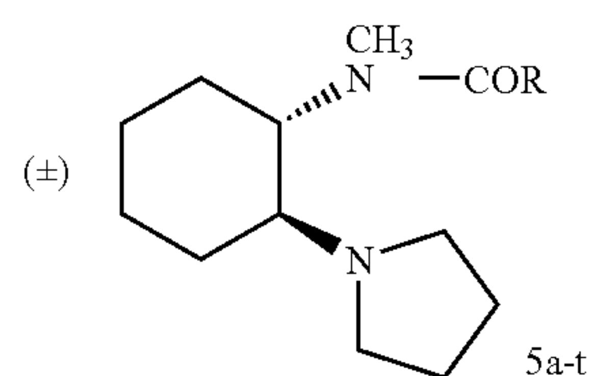
Compounds of Formula IV
