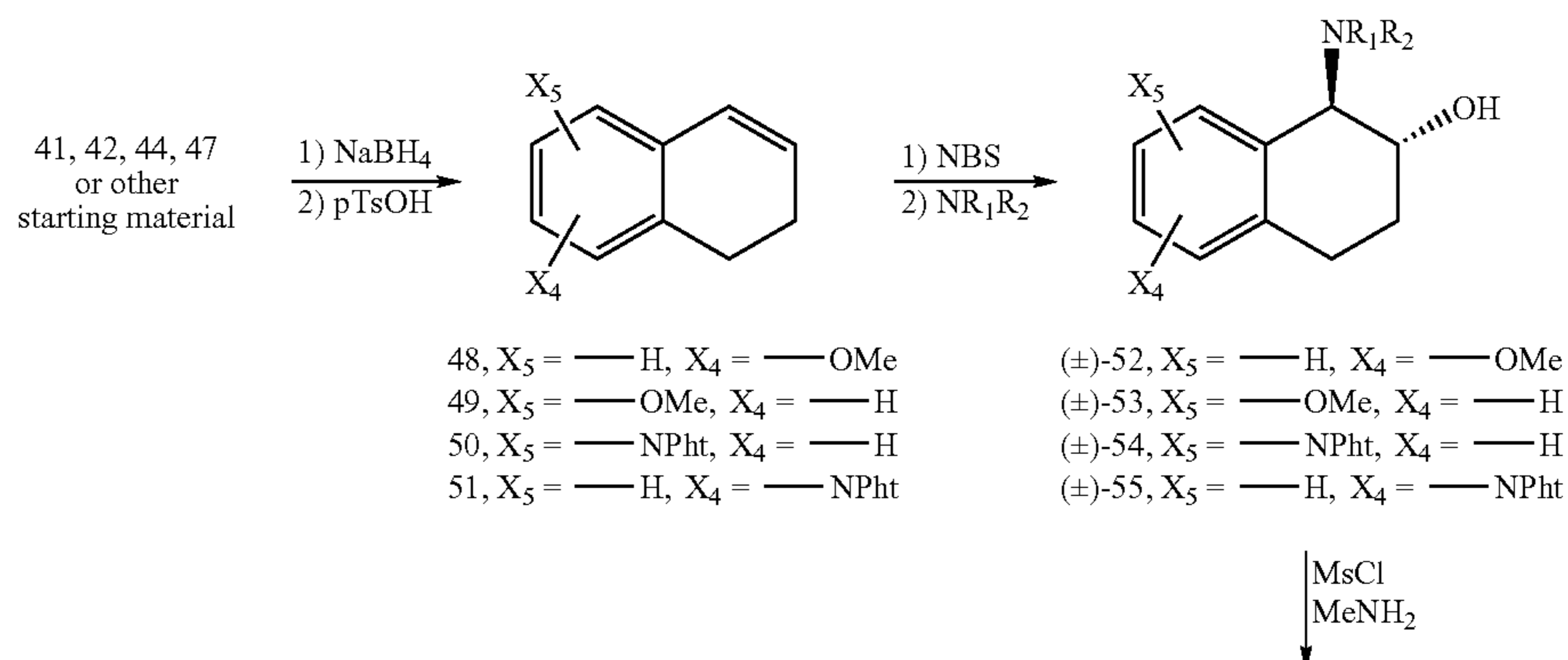
Scheme 6.
