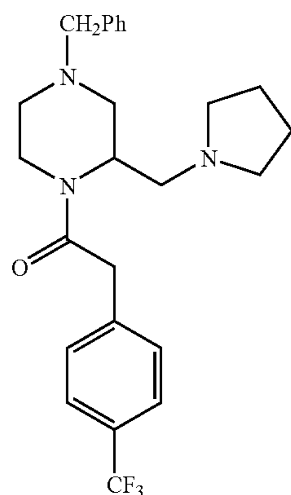
(R,S)-11
