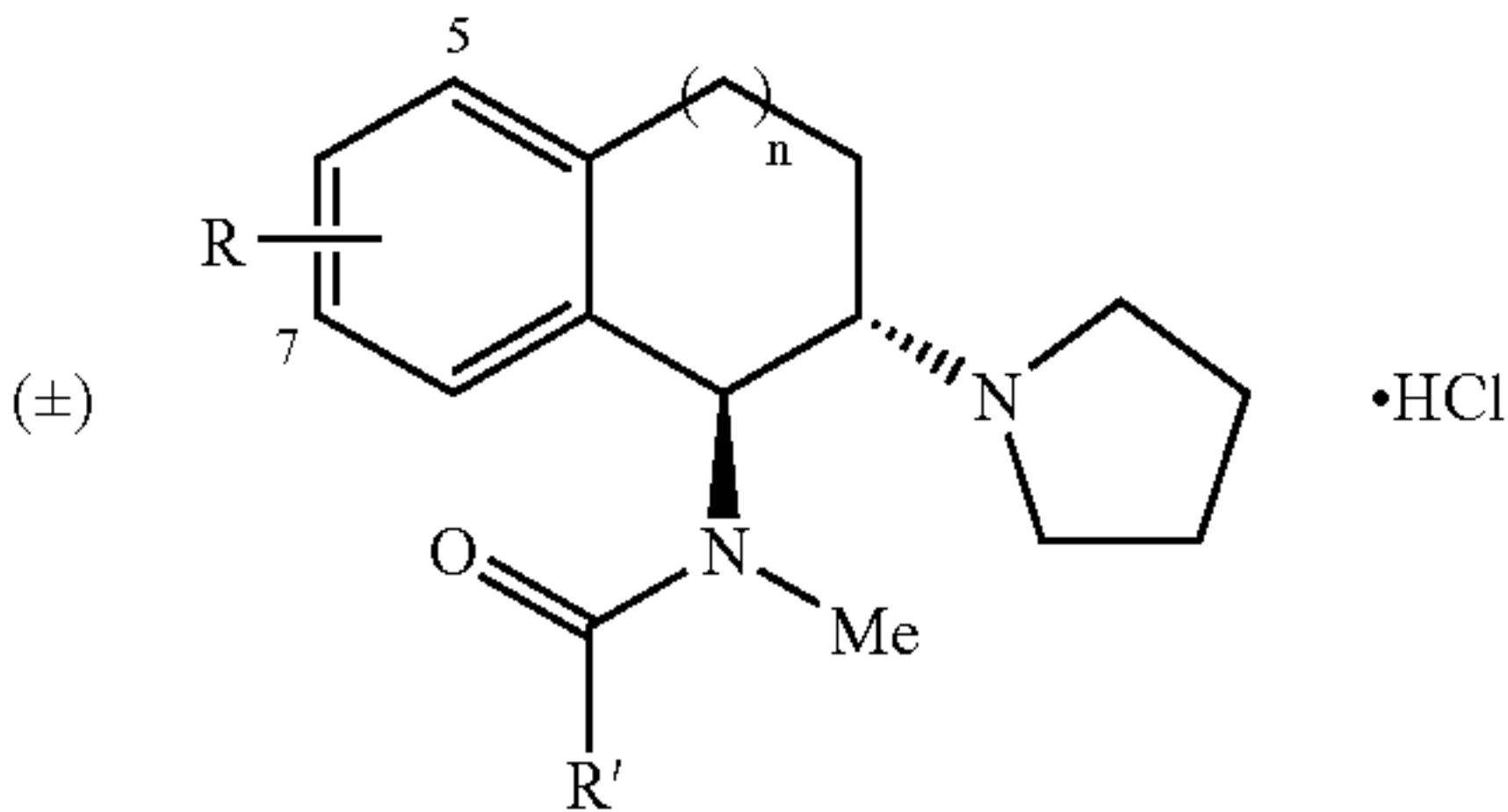
Compounds of Formula II
