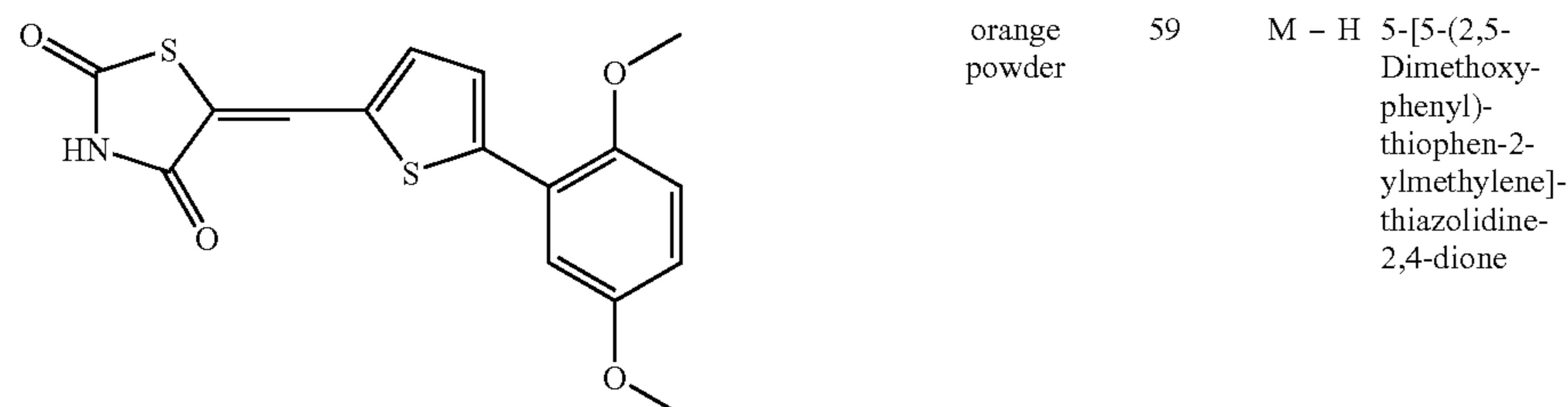
Compound F10
