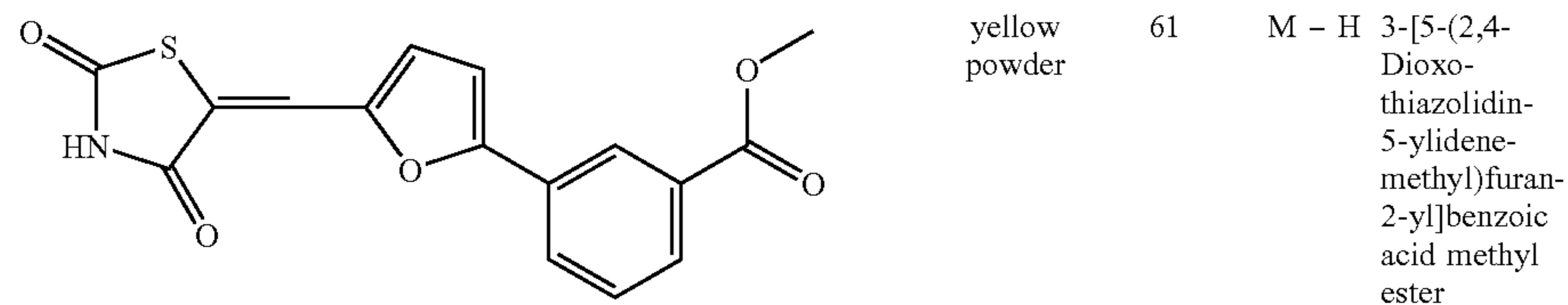
Compound F8
