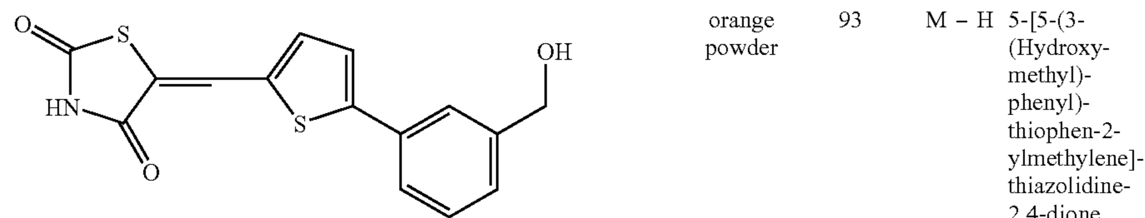
Compound F9
