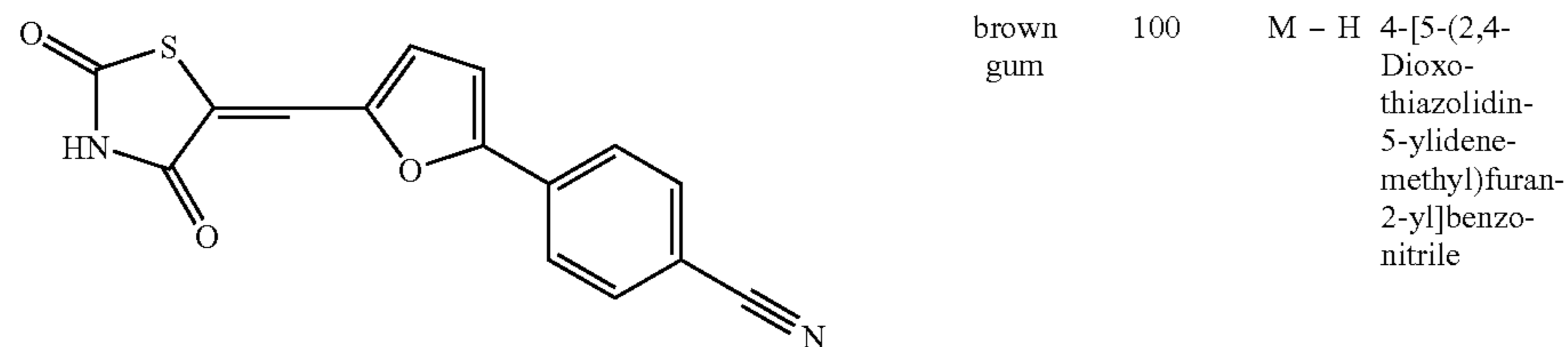
Compound F7
