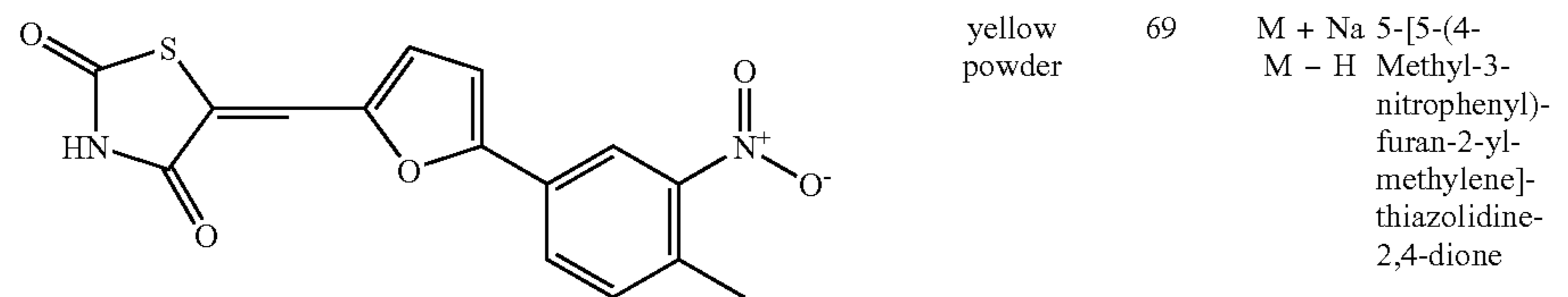
Compound F6
