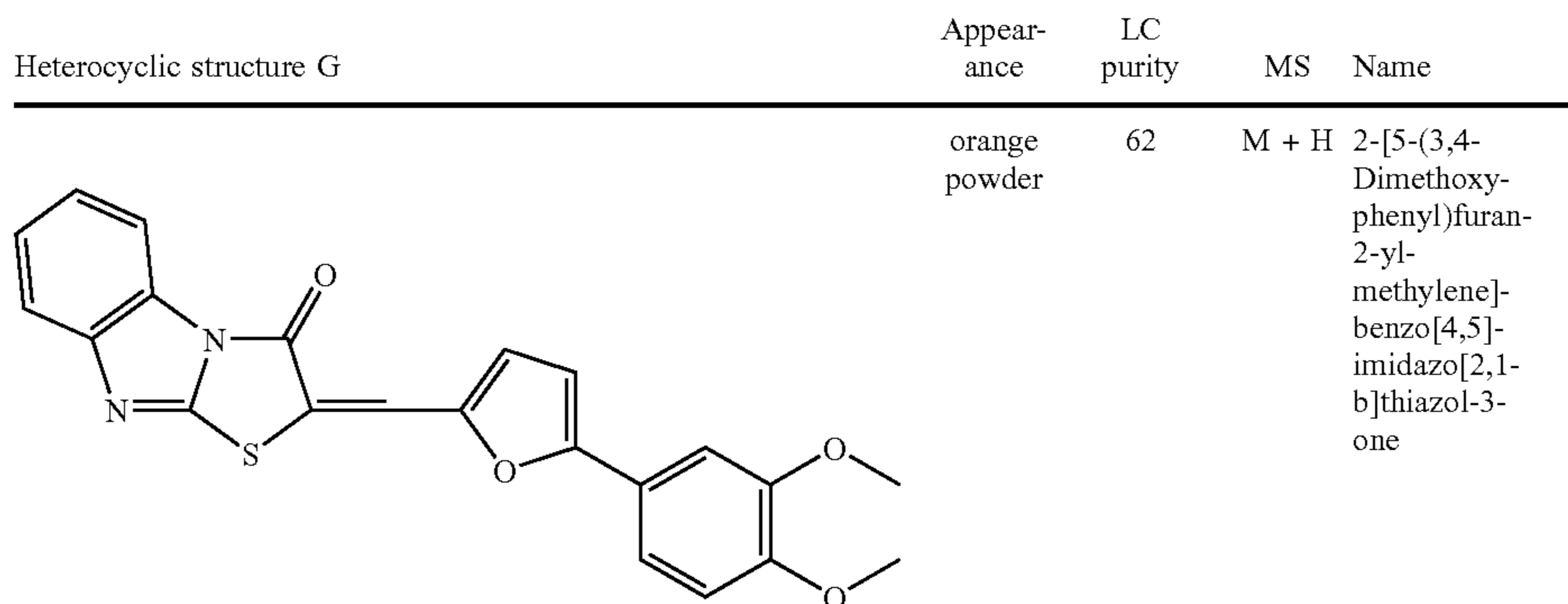
Compound G1
