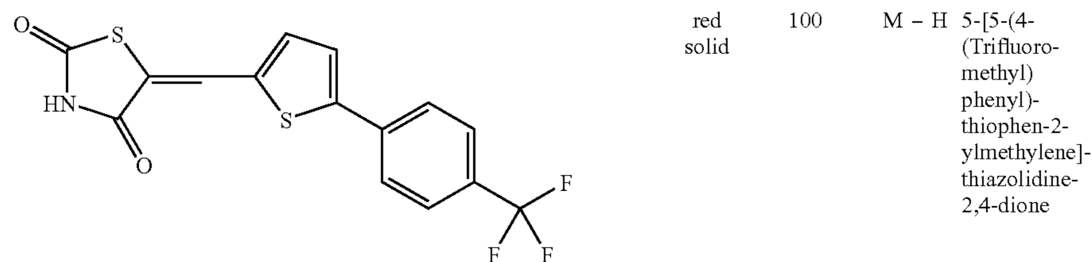
Compound F11
