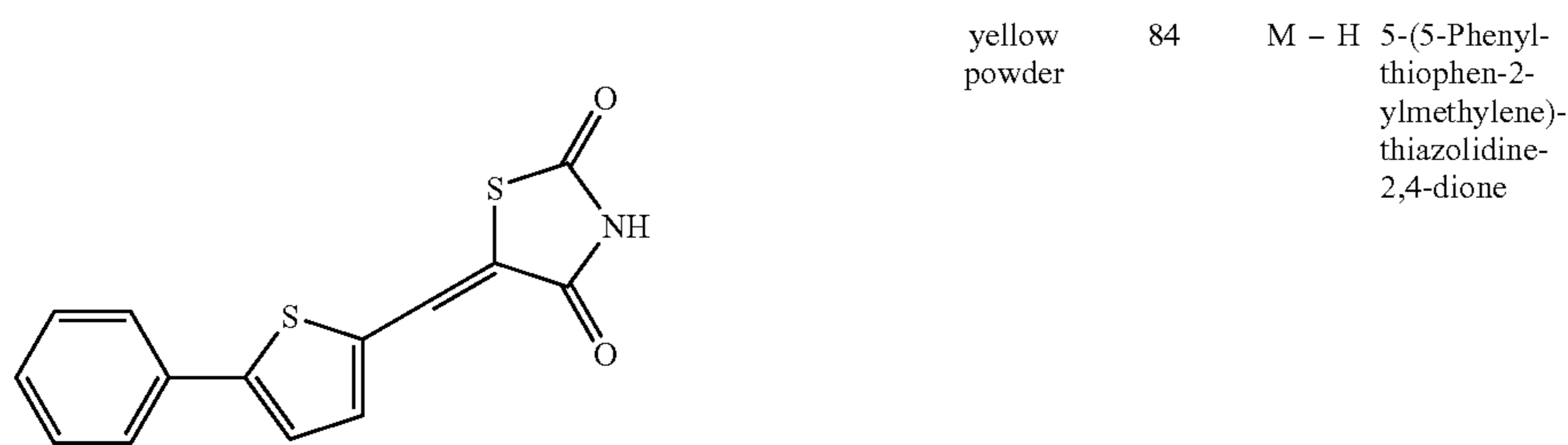
Compound F18
