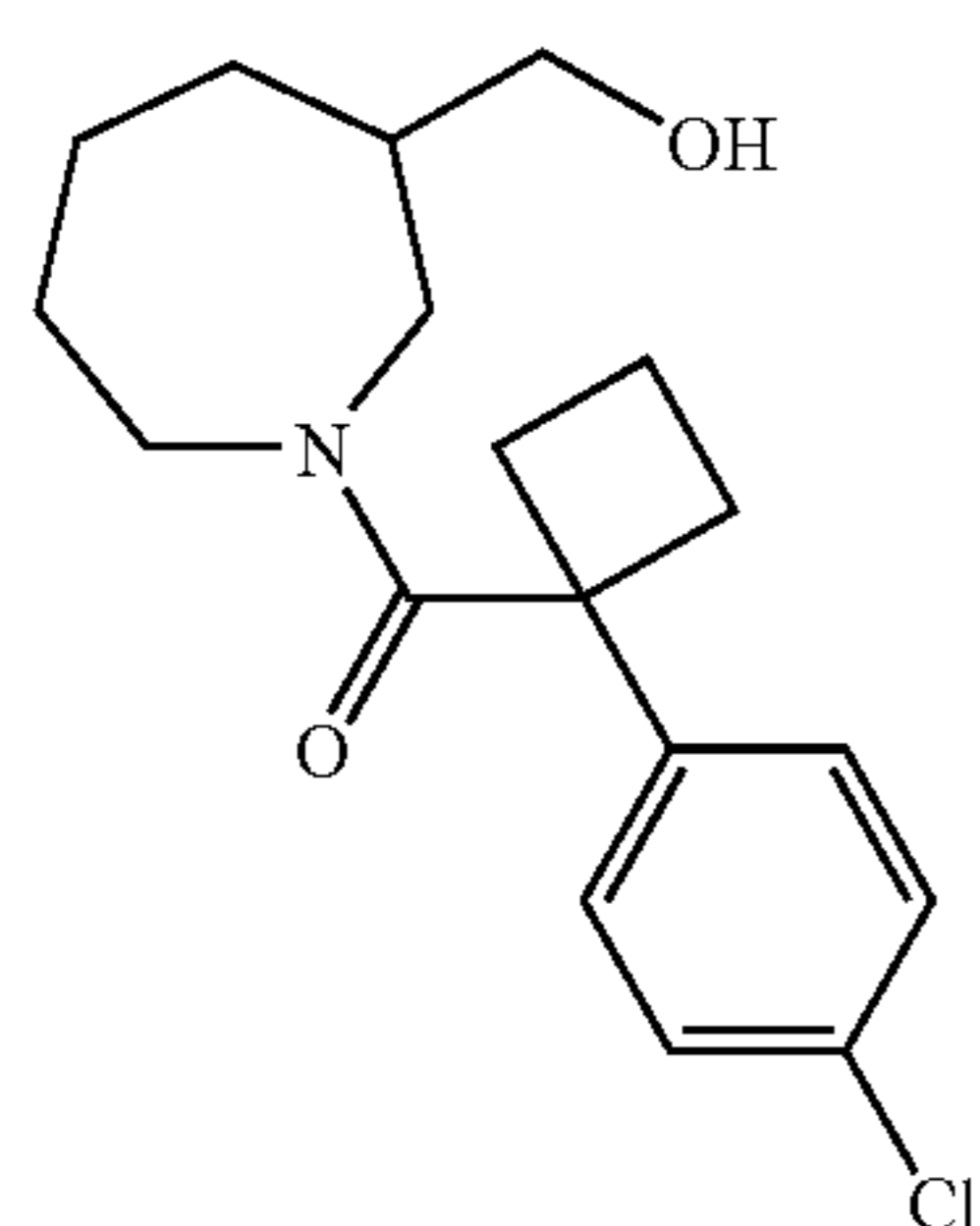
[1-(4-Chloro-phenyl)-cyclobutyl]- [3-(3-hydroxymethyl-azepan-1-yl)- methanone
