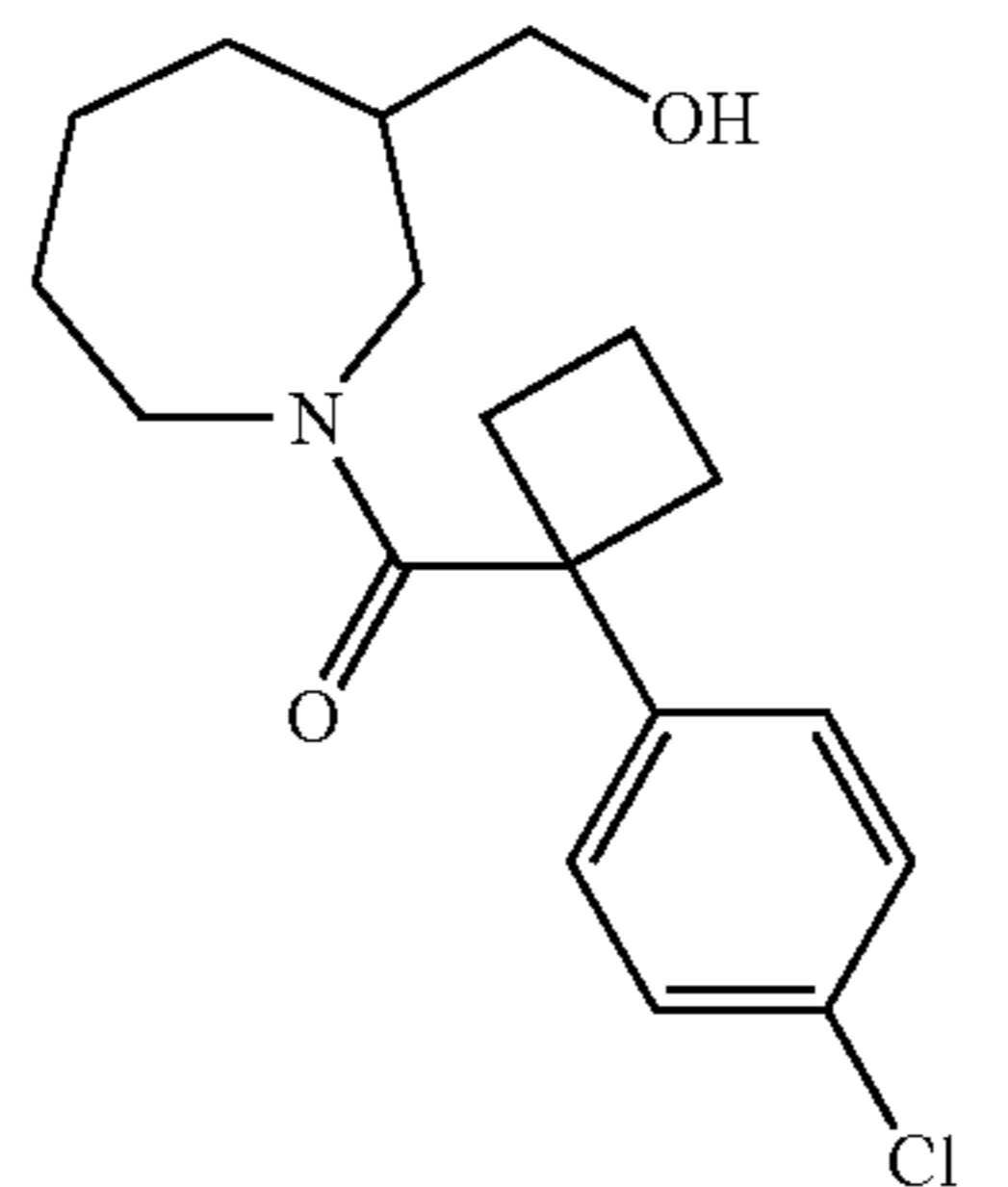
[1-(4-Chloro-phenyl)-cyclobutyl]- [3-(3-hydroxymethyl-azepan-1-yl)- methanone
