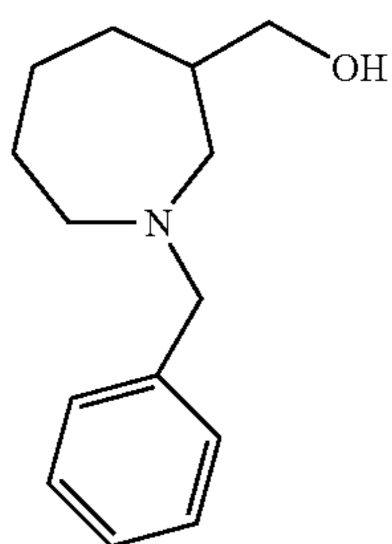
(1-Benzyl-azepan-3-yl)-methanol
