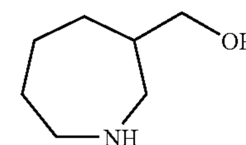
Azepan-3-yl-methanol
