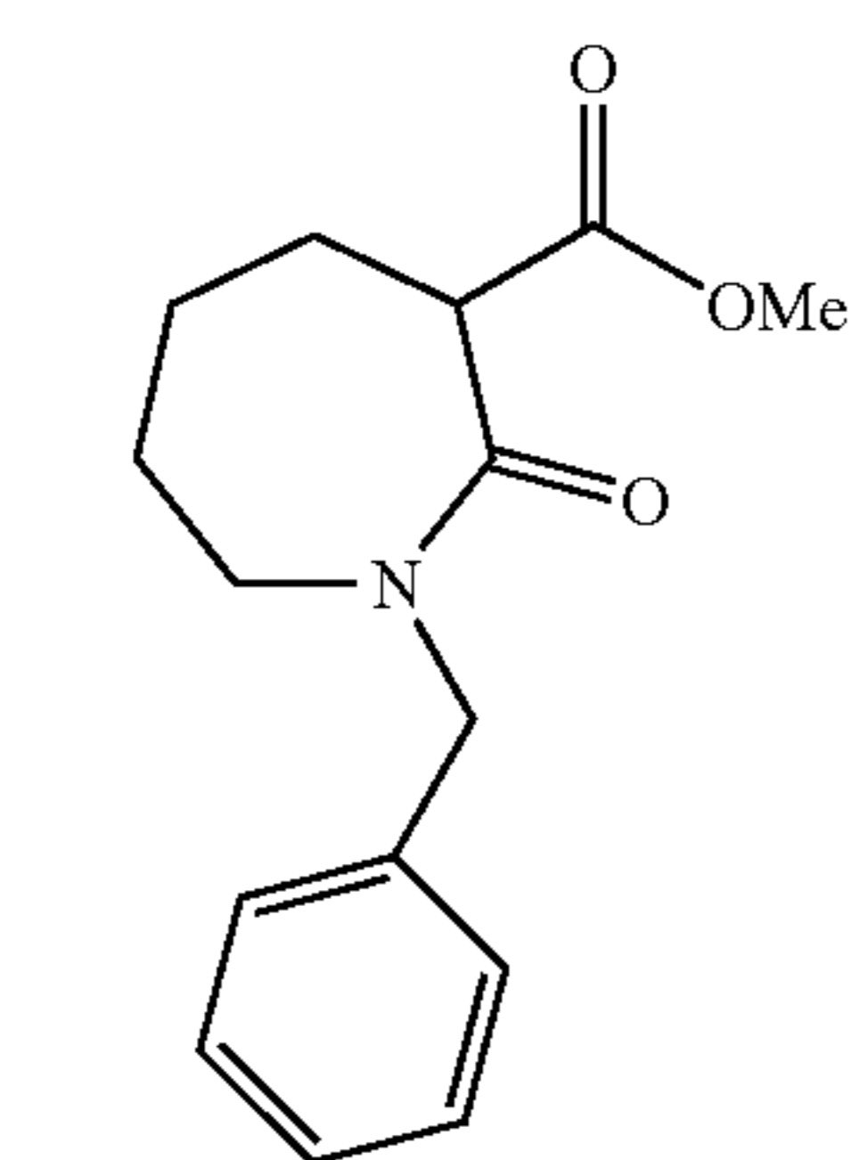
1-Benzyl-2-oxo-azepane-3-carboxylic acid methyl ester
