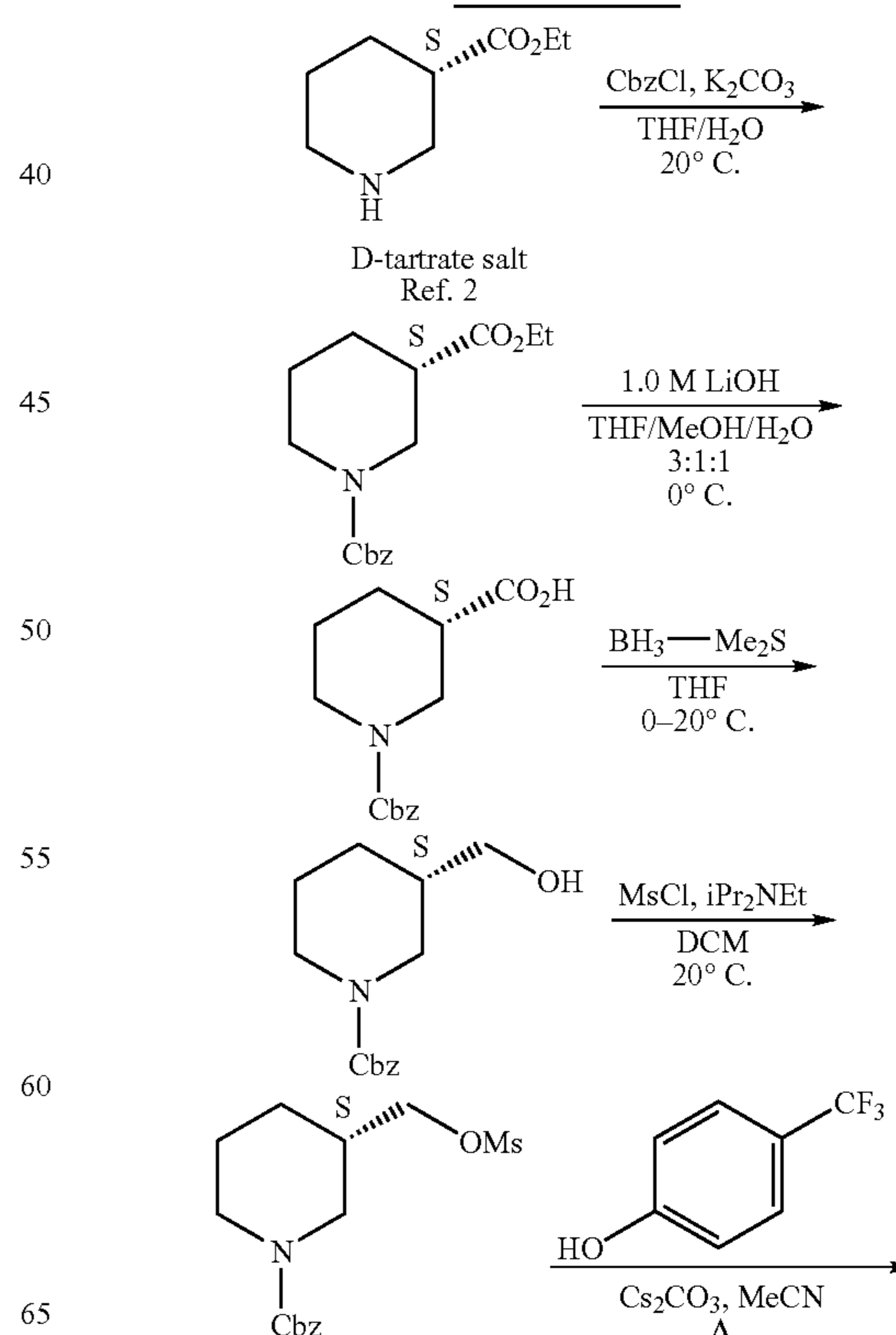
Scheme 2 Synthesis of 124
