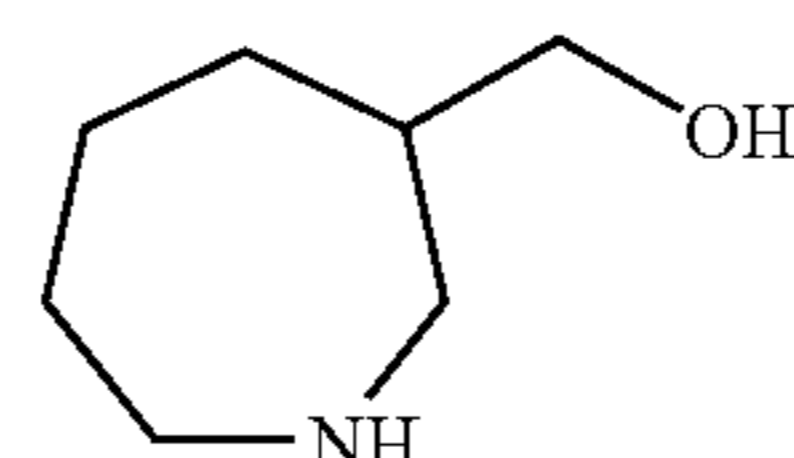
Azepan-3-yl-methanol
