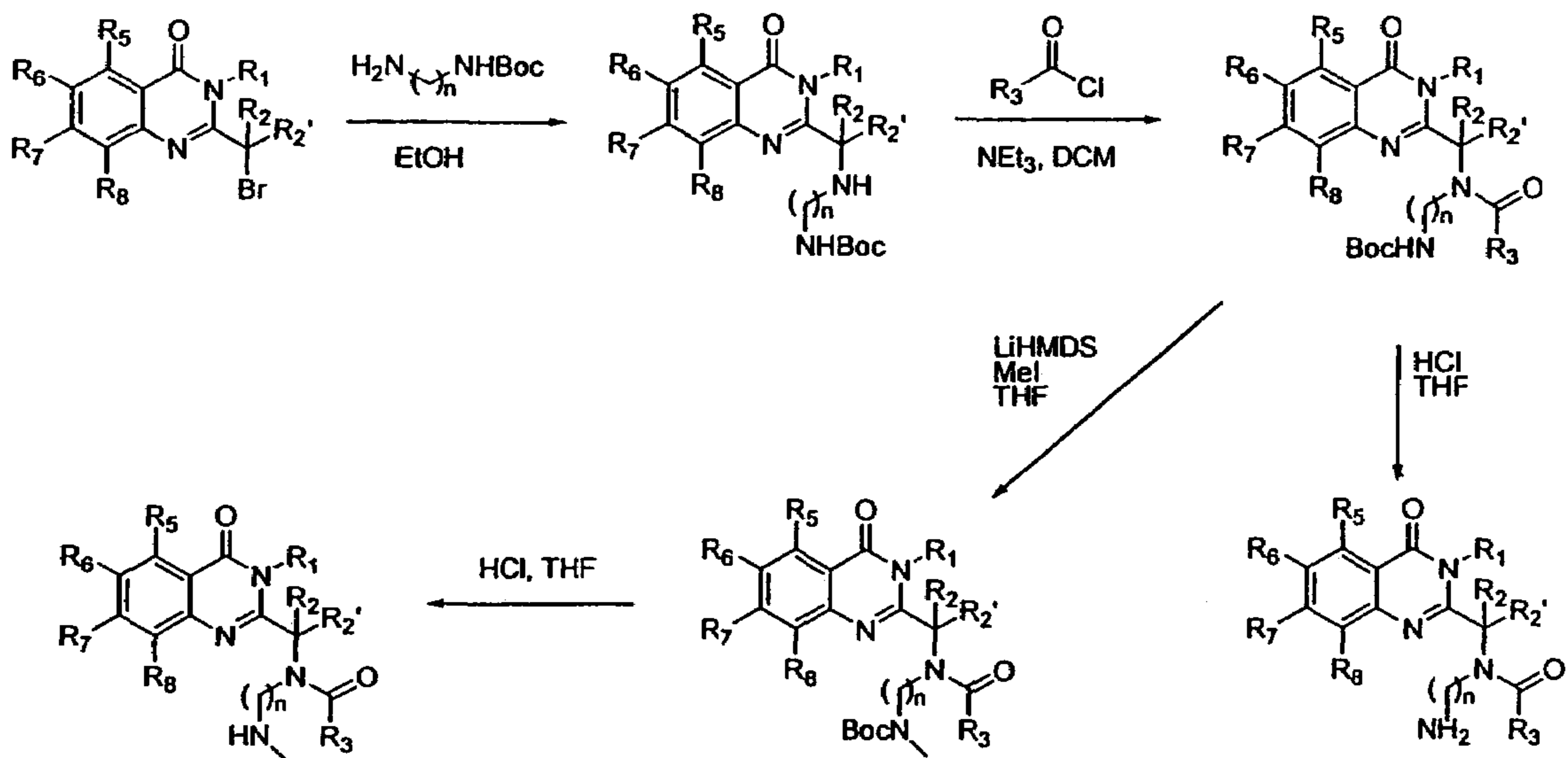
Figure 5d: Primary and Secondary Amine R4 Synthesis
