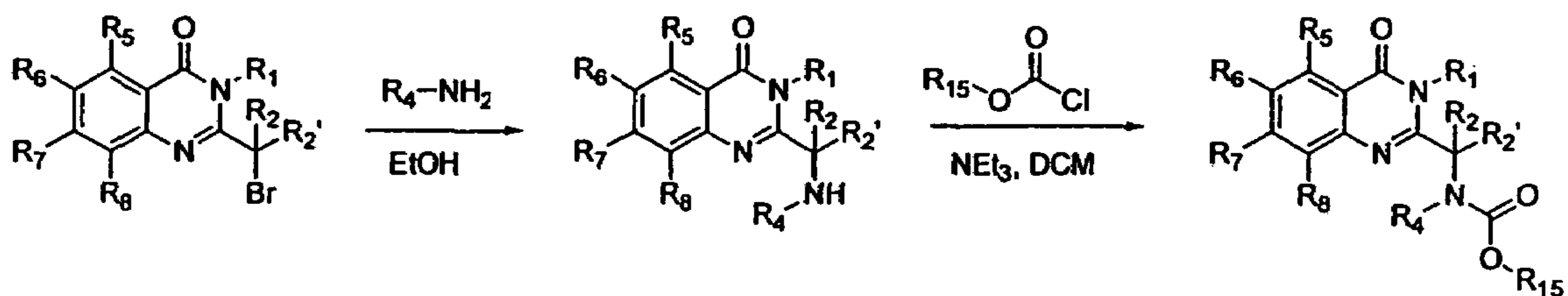
Figure 5c: Urea Synthesis
