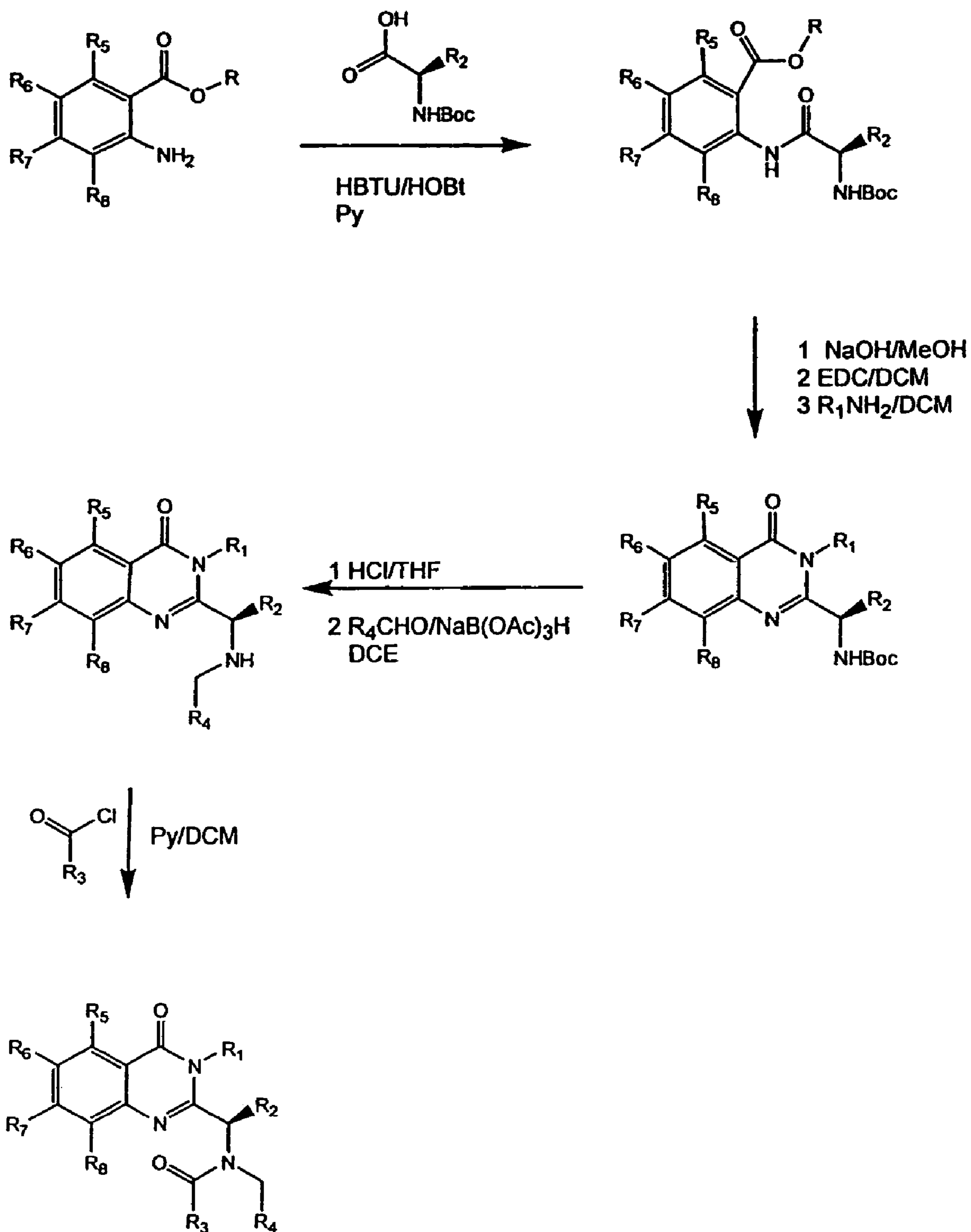
Figure 4: Asymmetric Synthesis
