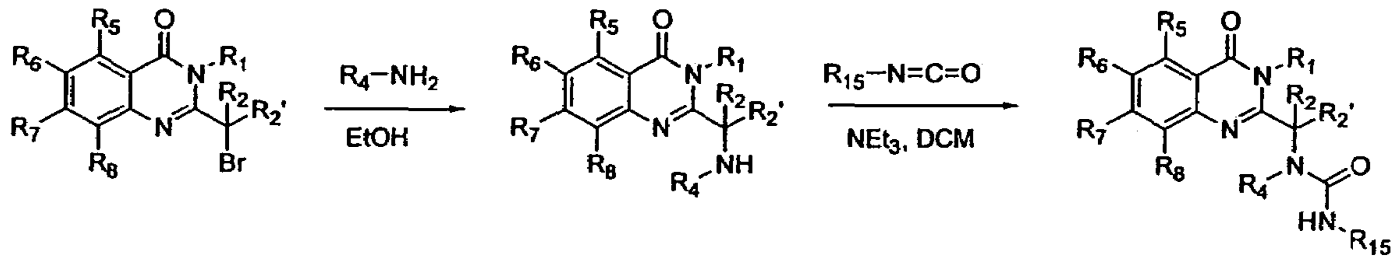
Figure 5d: Primary and Secondary Amine R4 Synthesis
