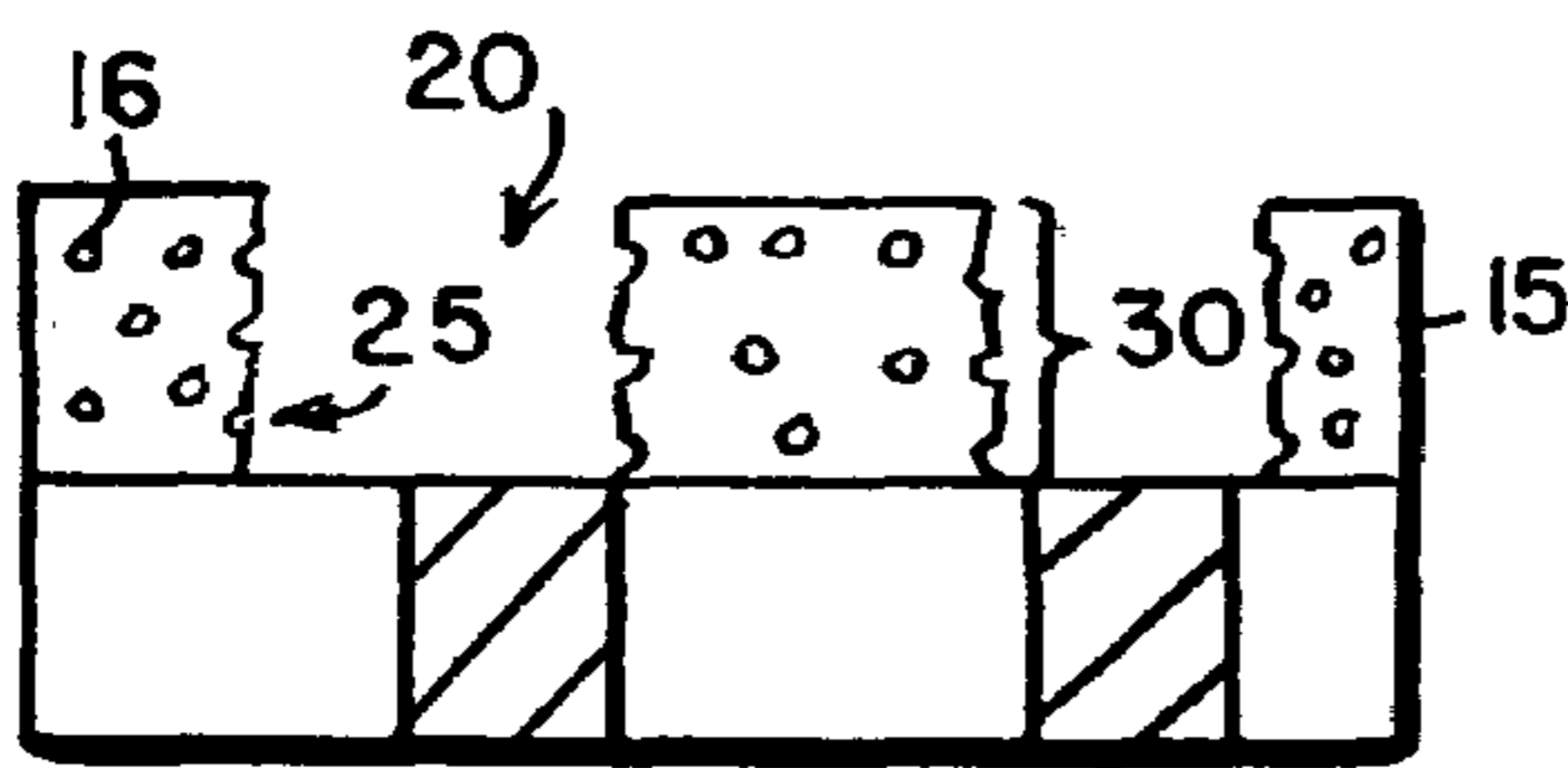
FIG. 2 PRIOR ART
