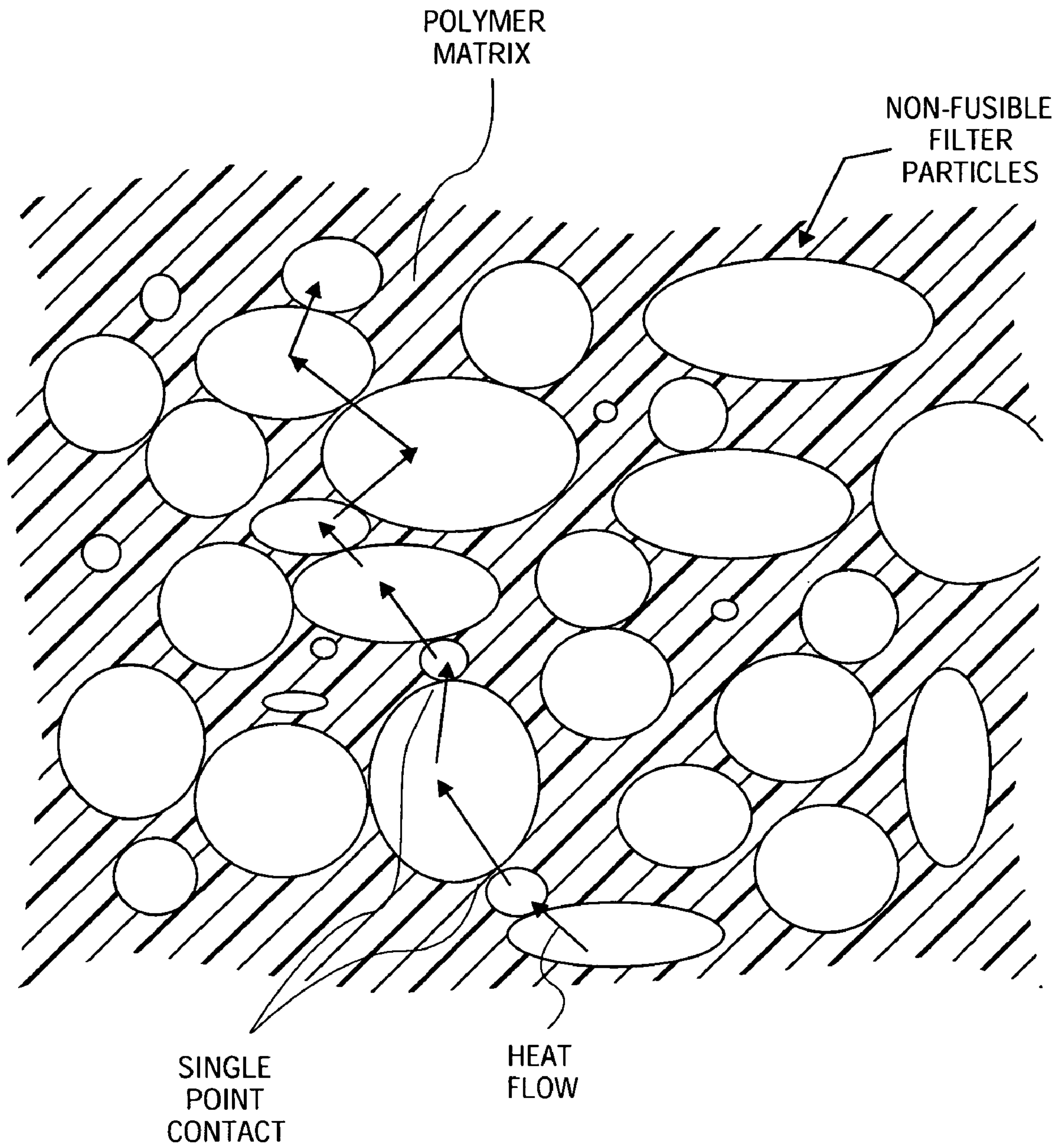
FIG. 2 (PRIOR ART)
