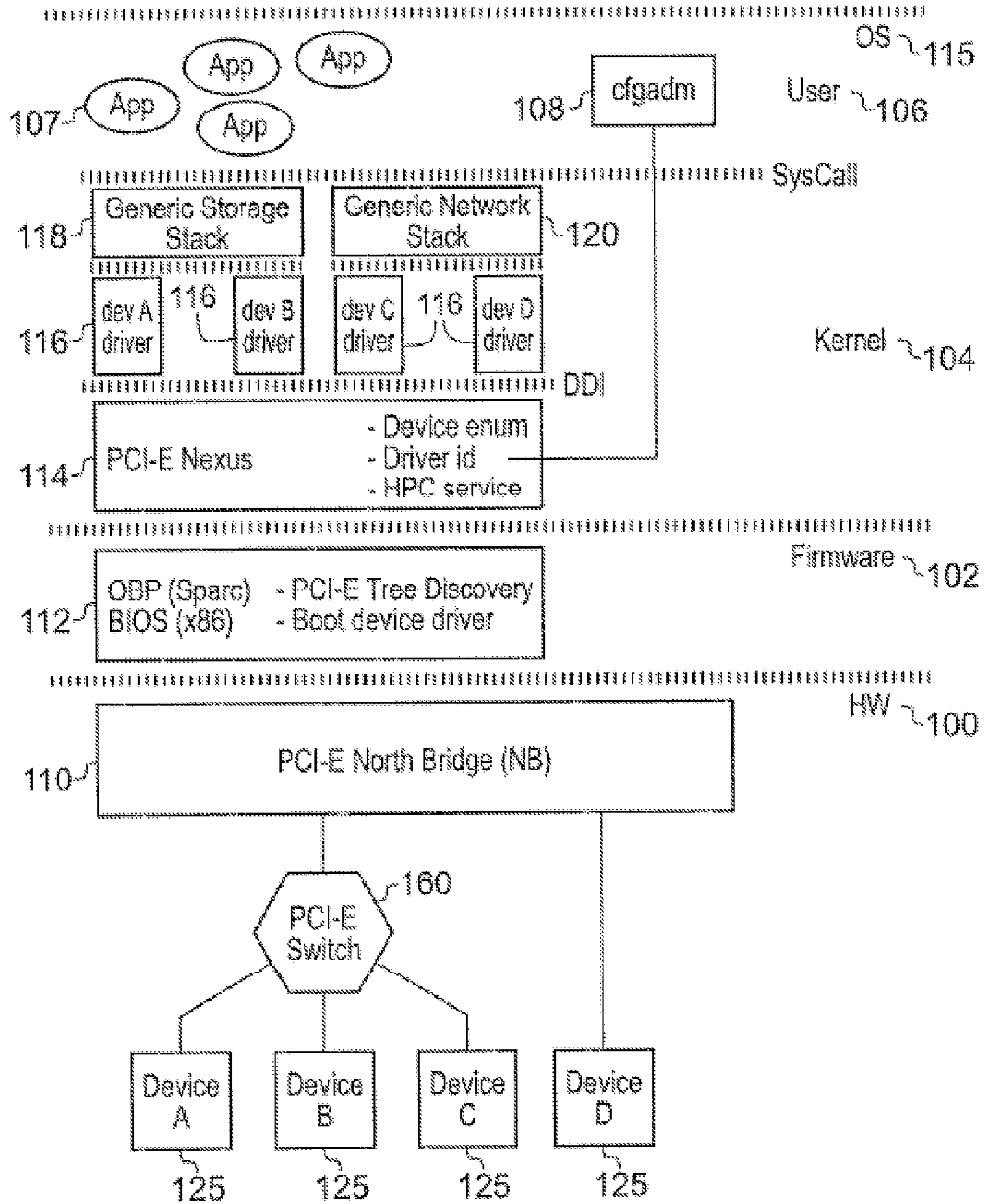
Fig. 8 (PRIOR ART)
