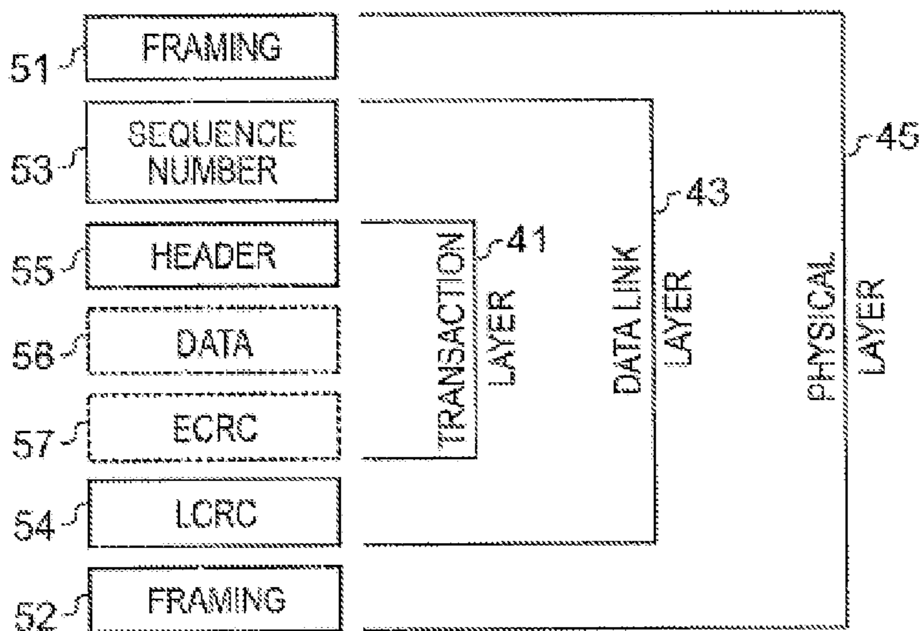
Fig. 5 (PRIOR ART)
