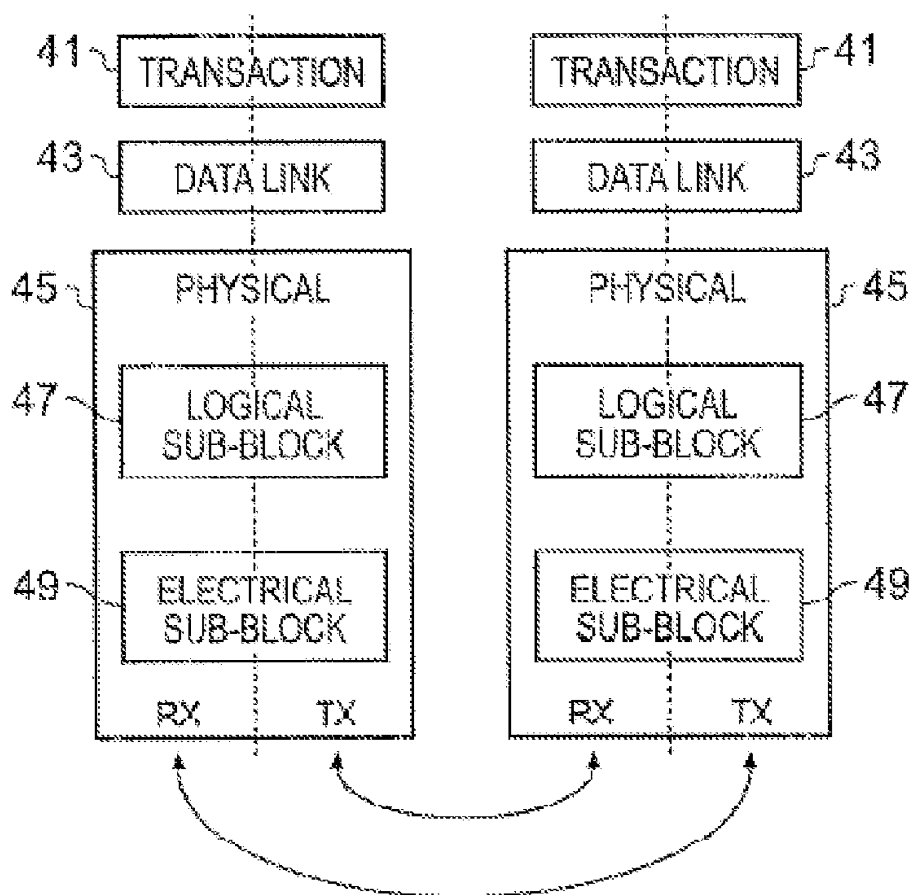
Fig. 4 (PRIOR ART)
