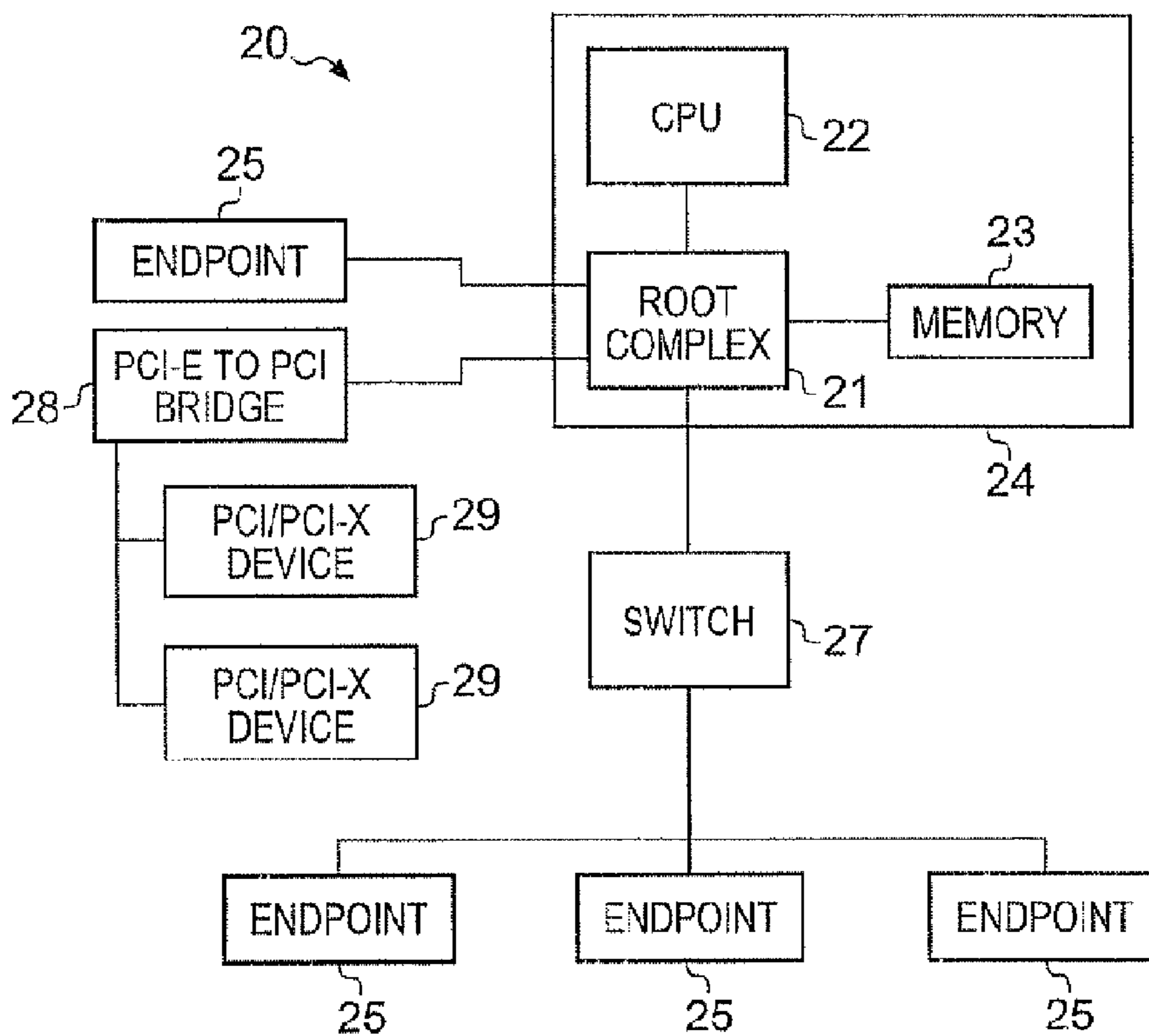
Fig. 1 (PRIOR ART)
