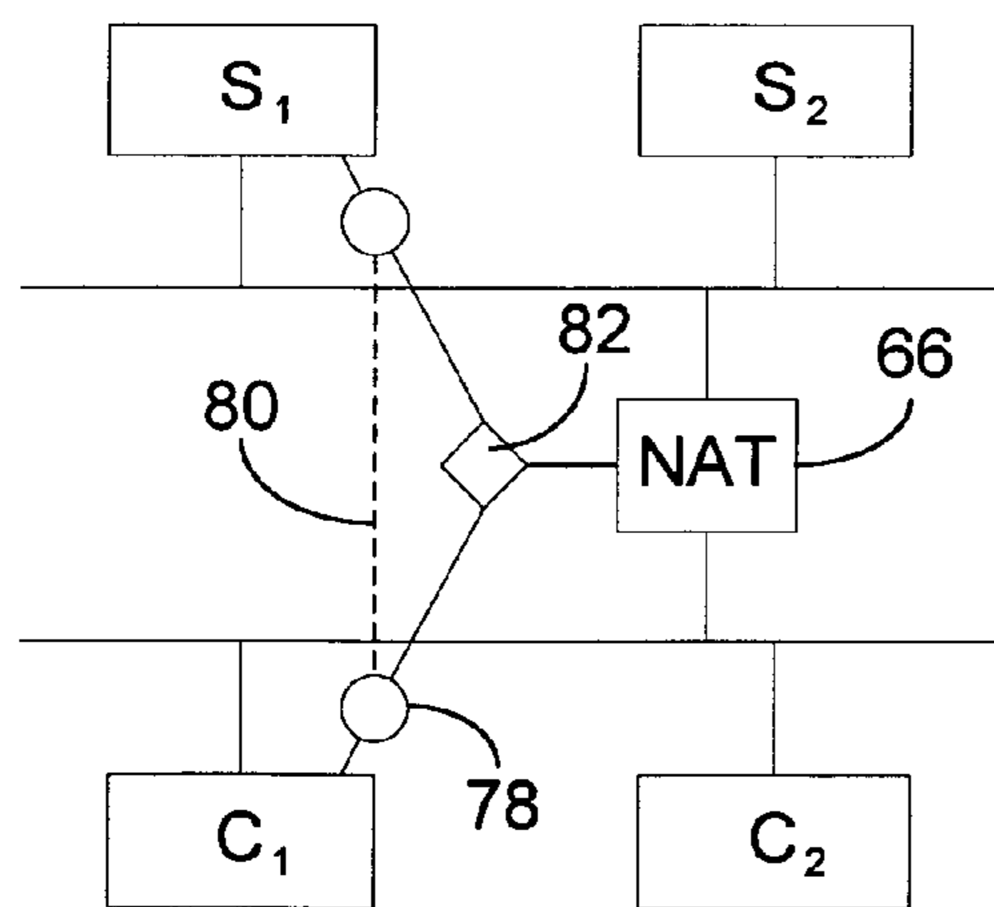
FIG. 3 (PRIOR ART)
