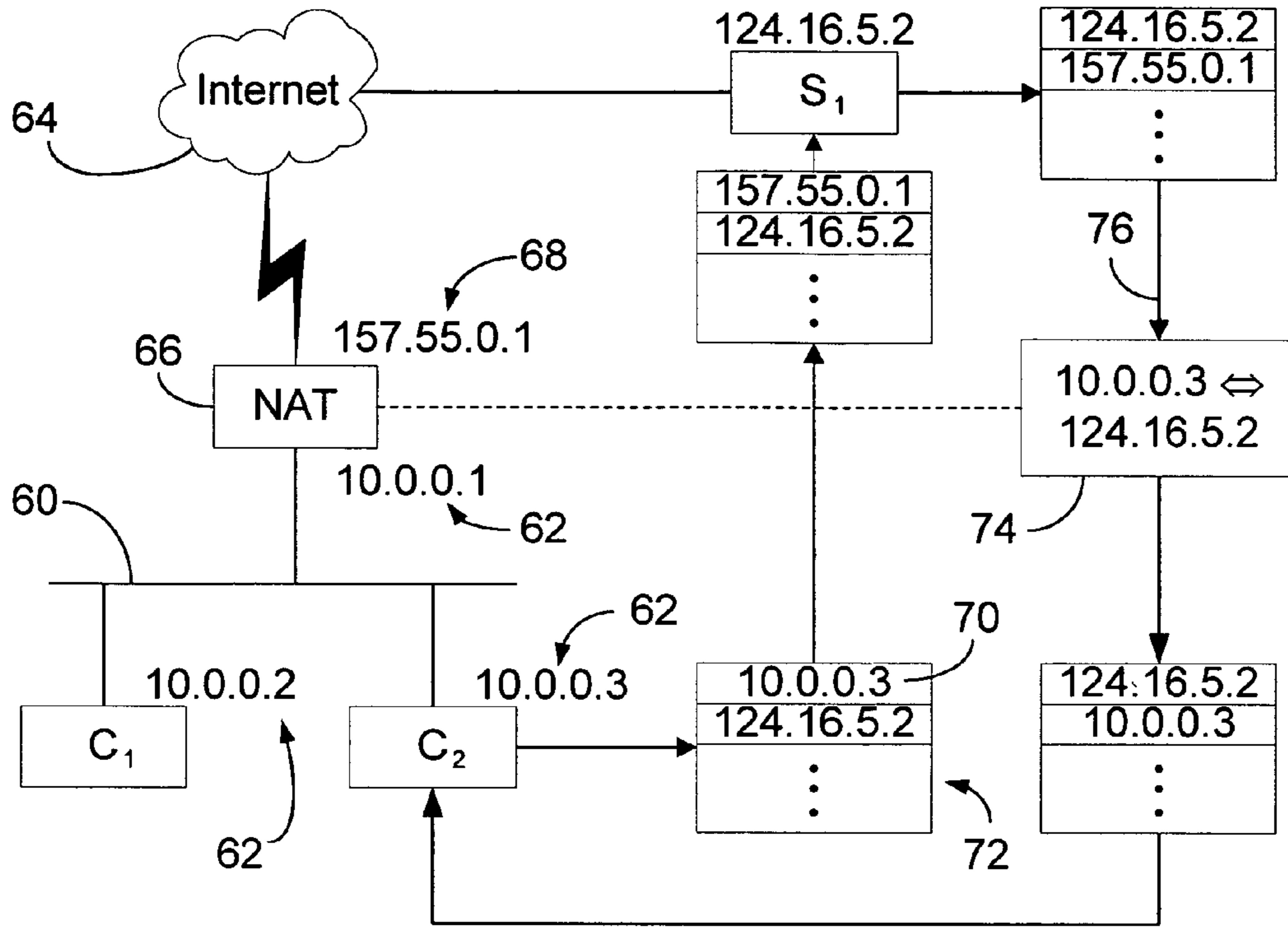
FIG. 2 (PRIOR ART)
