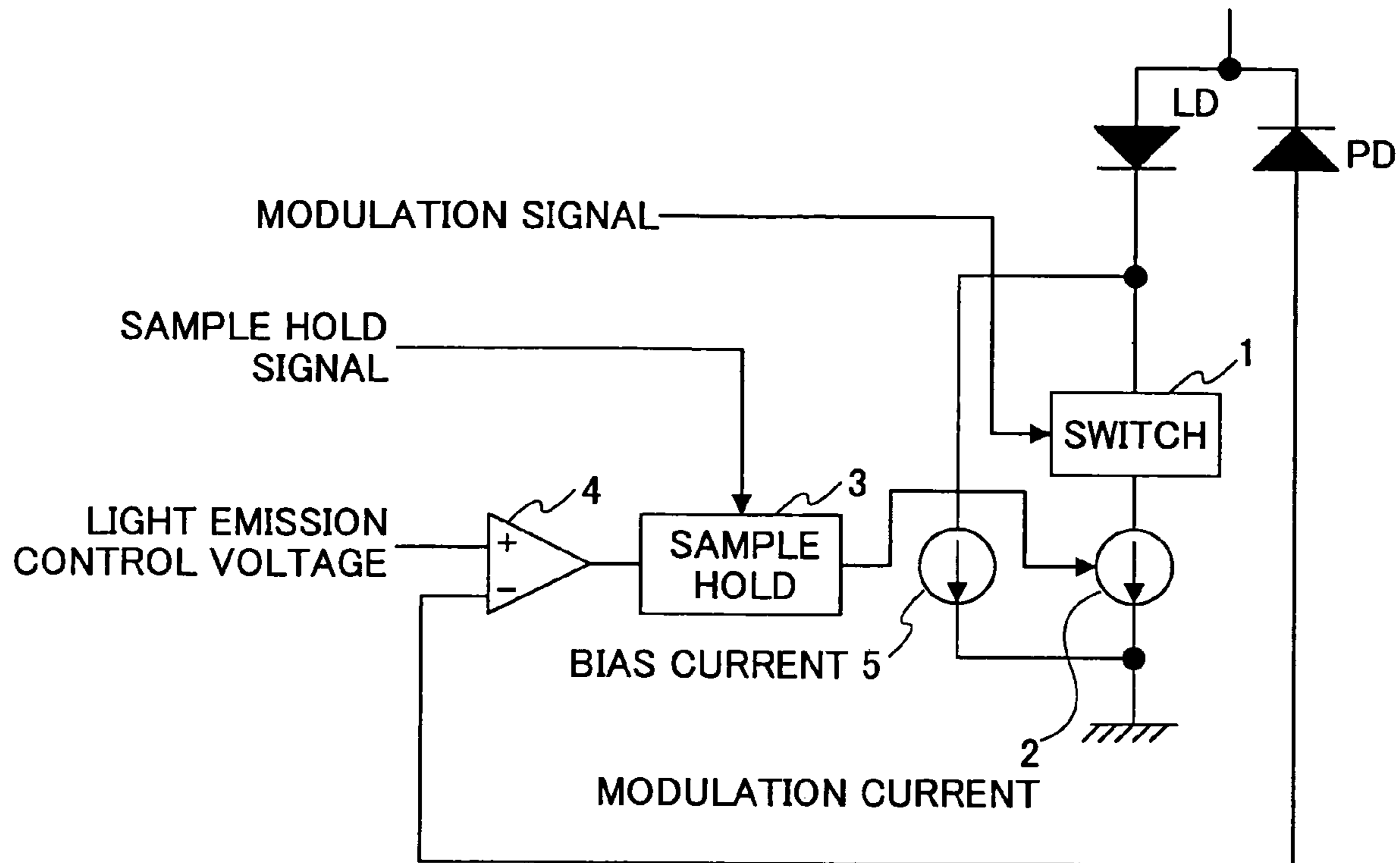
FIG.5 PRIOR ART
