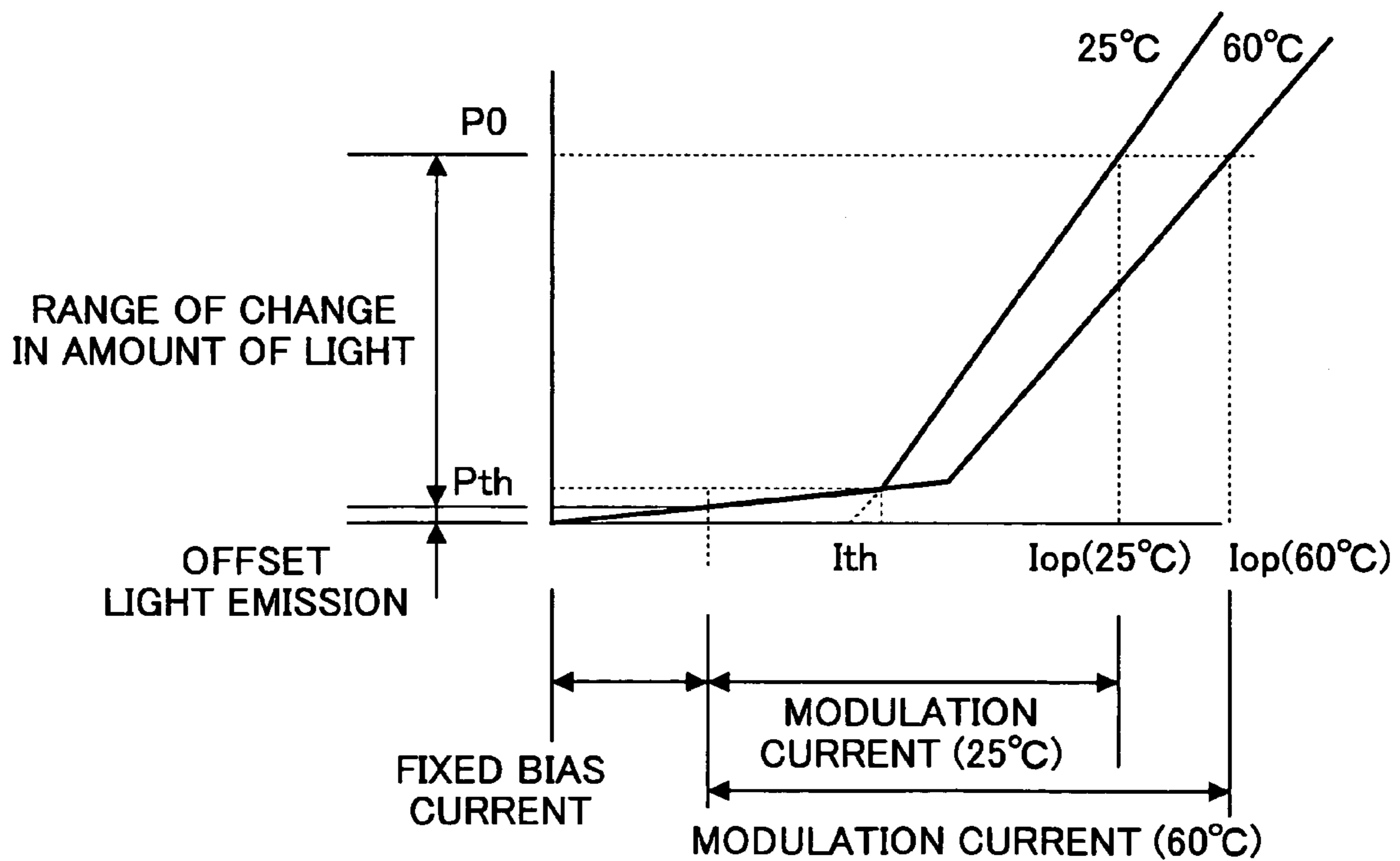
FIG.4 PRIOR ART
