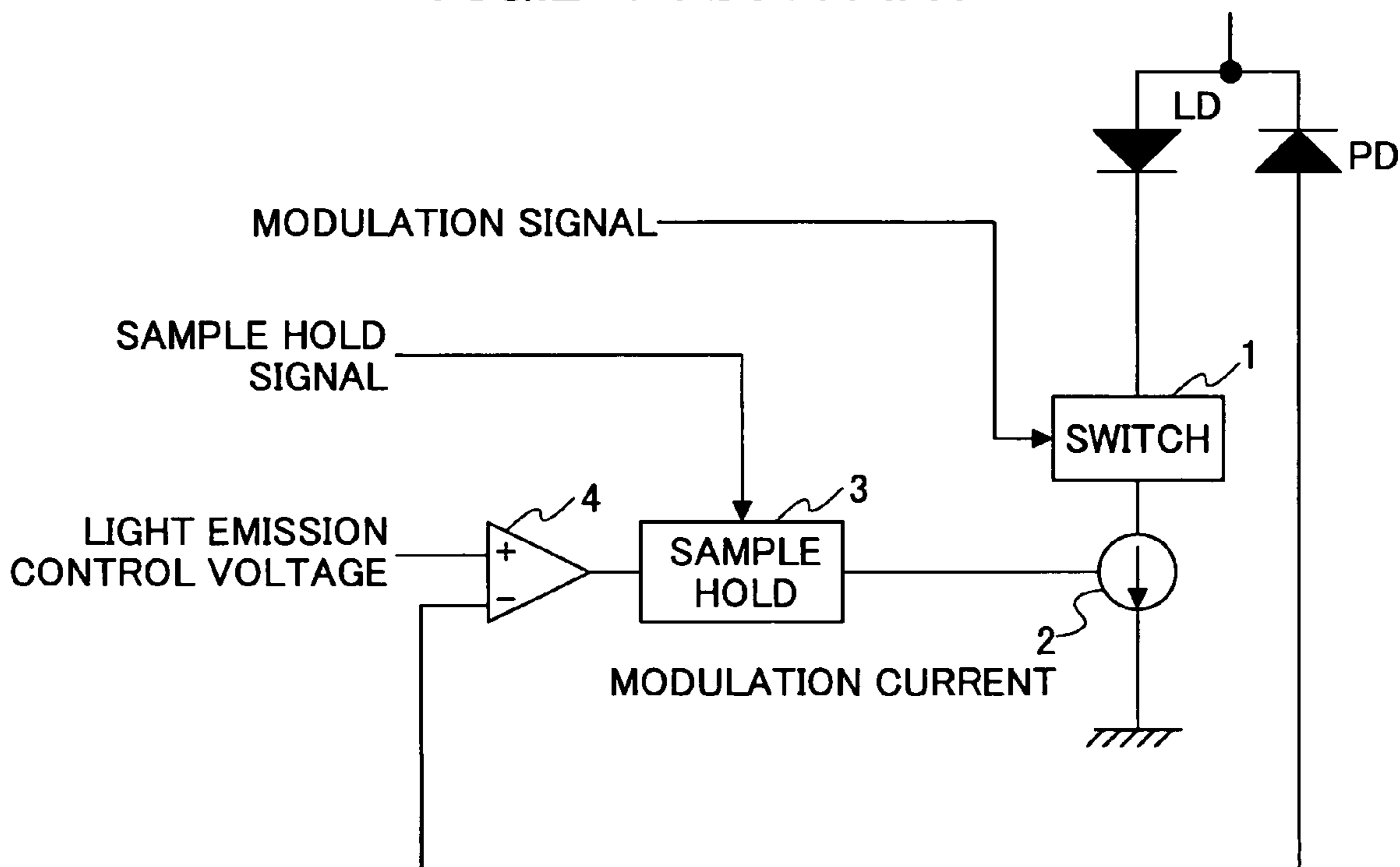
FIG.2 PRIOR ART
