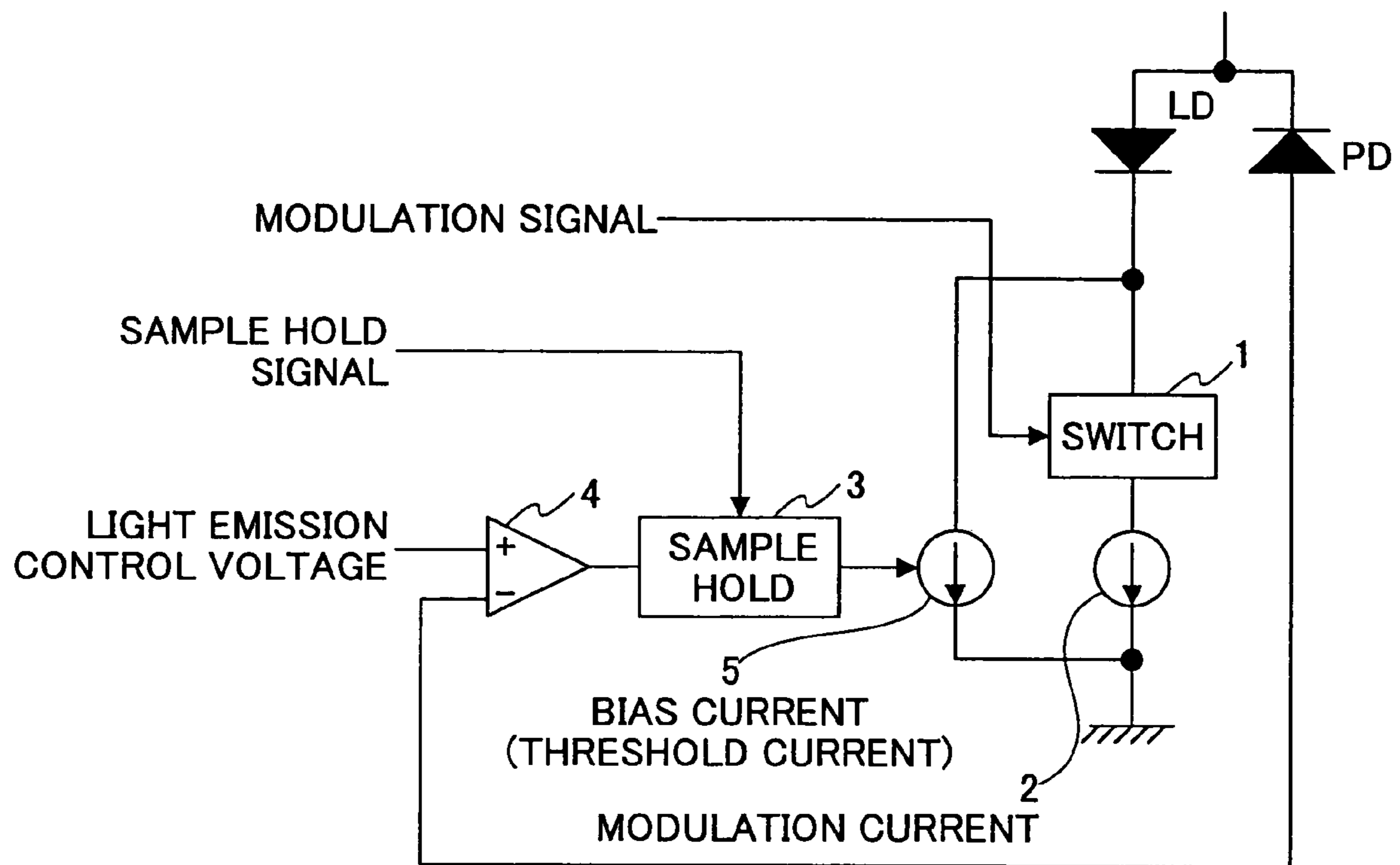
FIG.7 PRIOR ART
