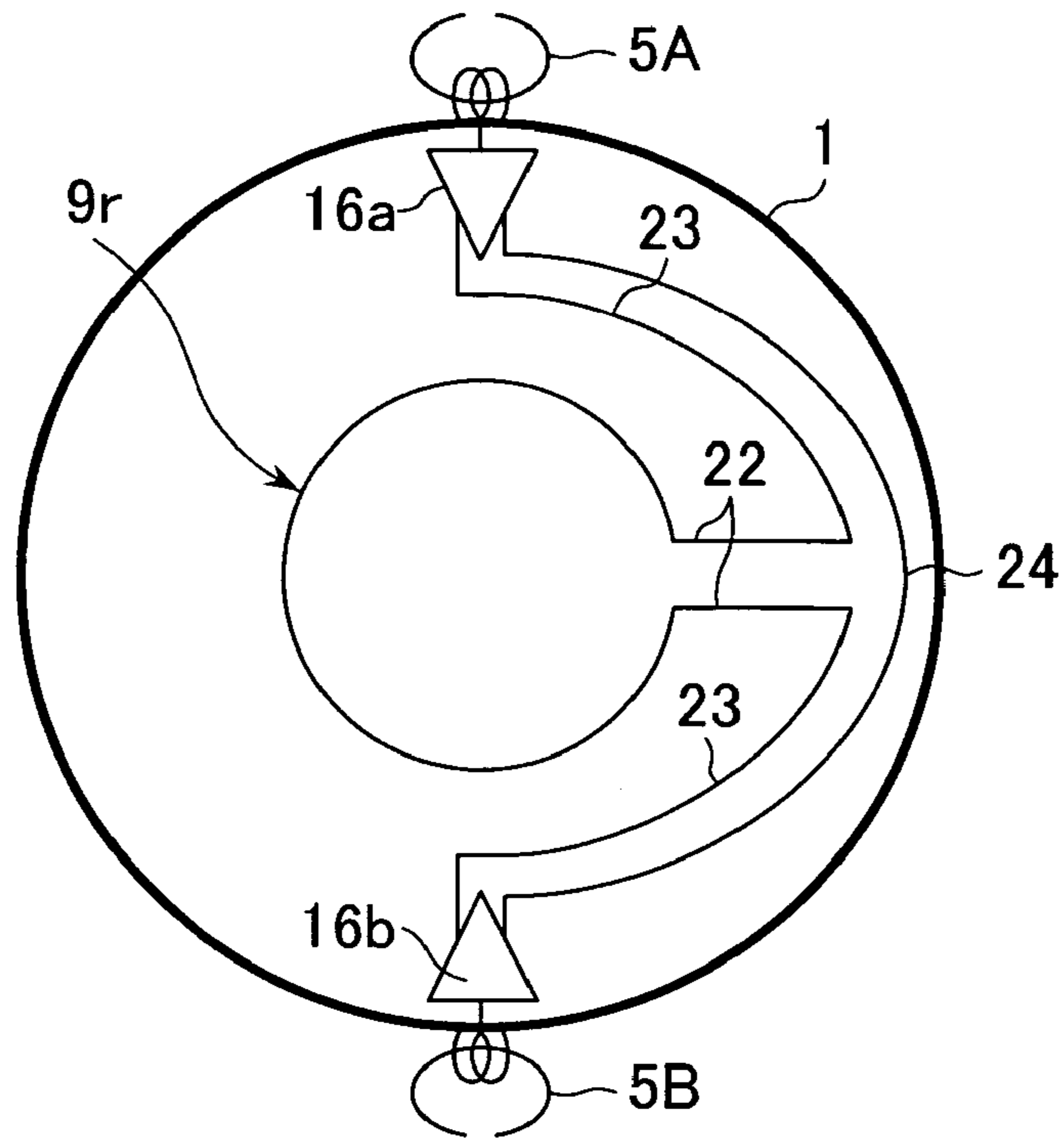
FIG.13 RELATED ART (B)
