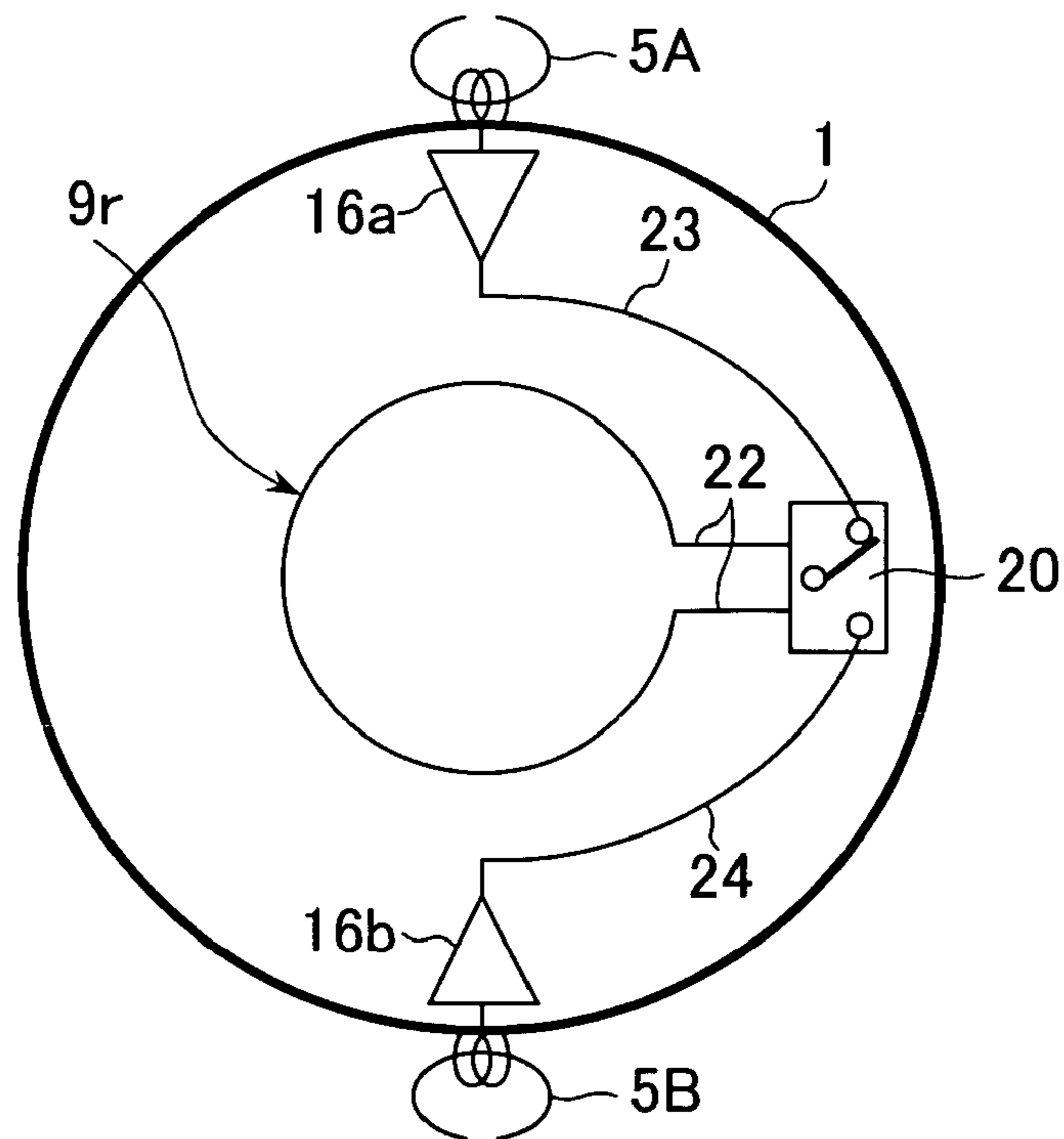
FIG.14 RELATED ART (C)
