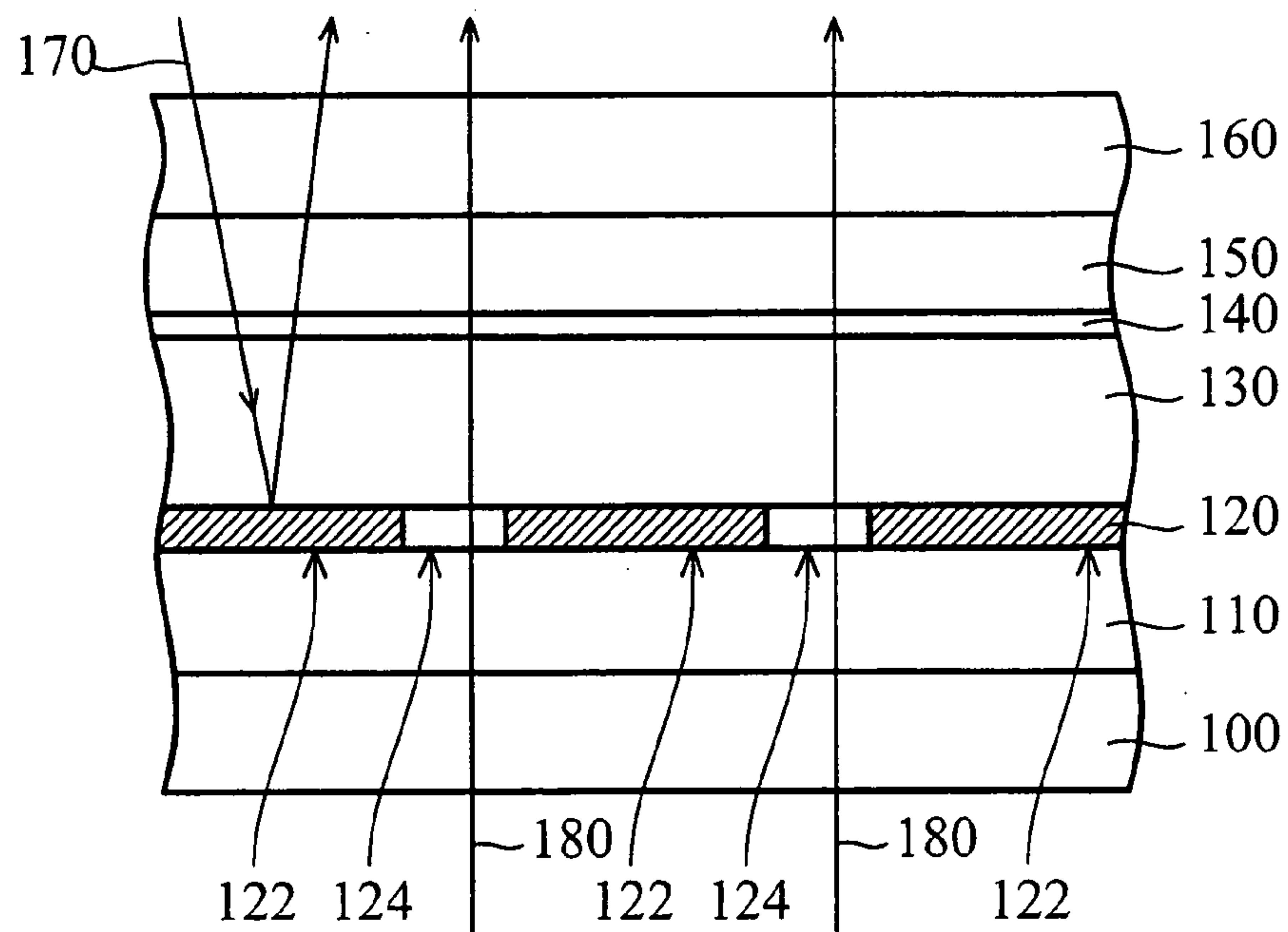
FIG. 1 ( PRIOR ART )
