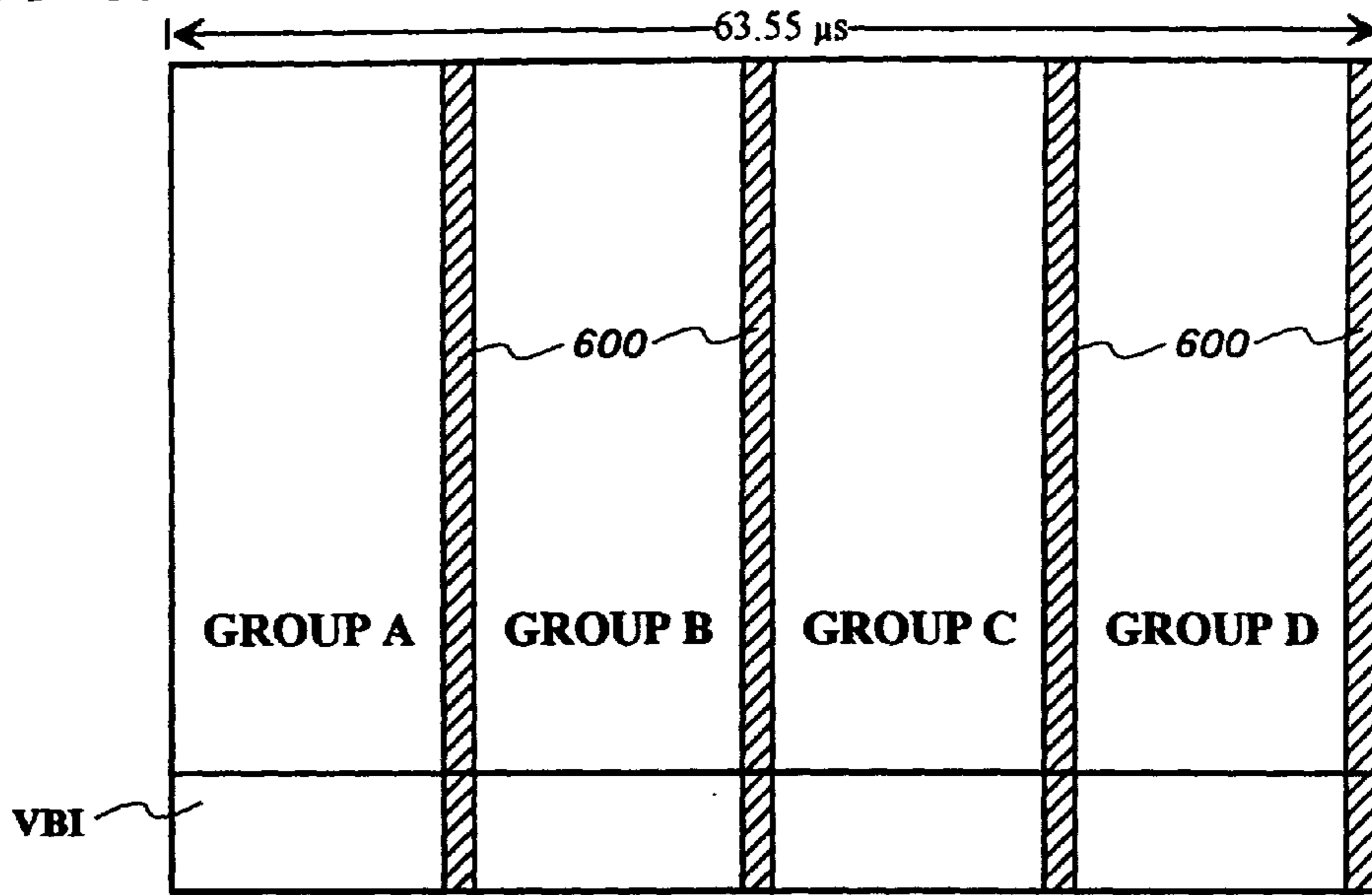
STAGGERED GROUPING IN TIME DOMAIN
