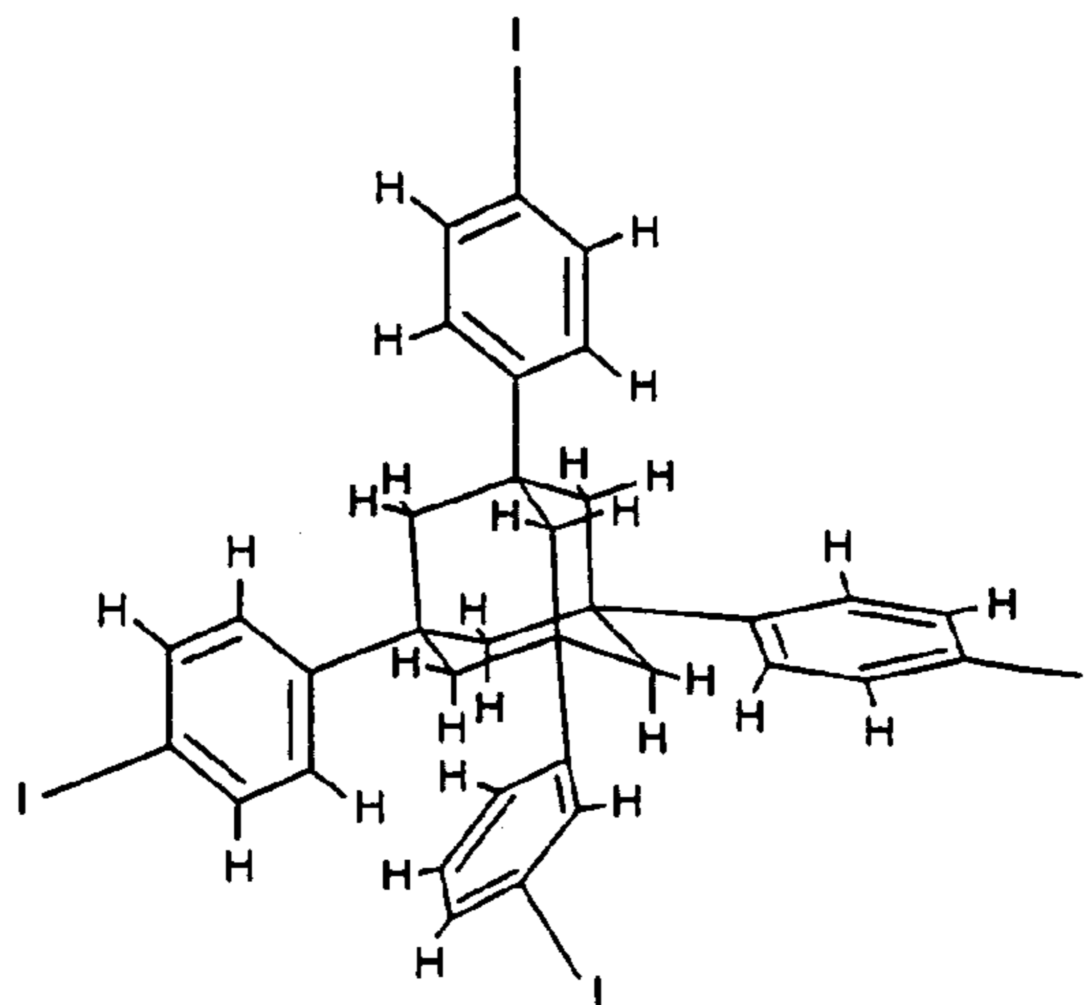
1,3,5,7-tetrakis(4-iodophenyl)adamantane
