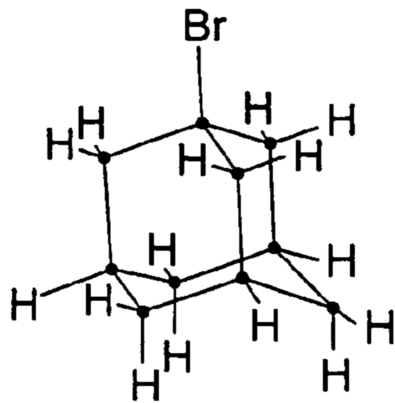
1-Bromoadamantane
