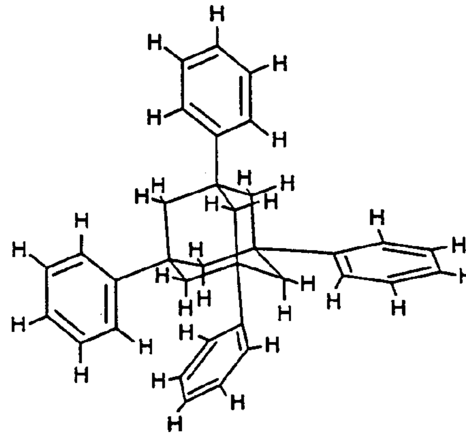
1,3,5,7-tetraphenyladamantane
