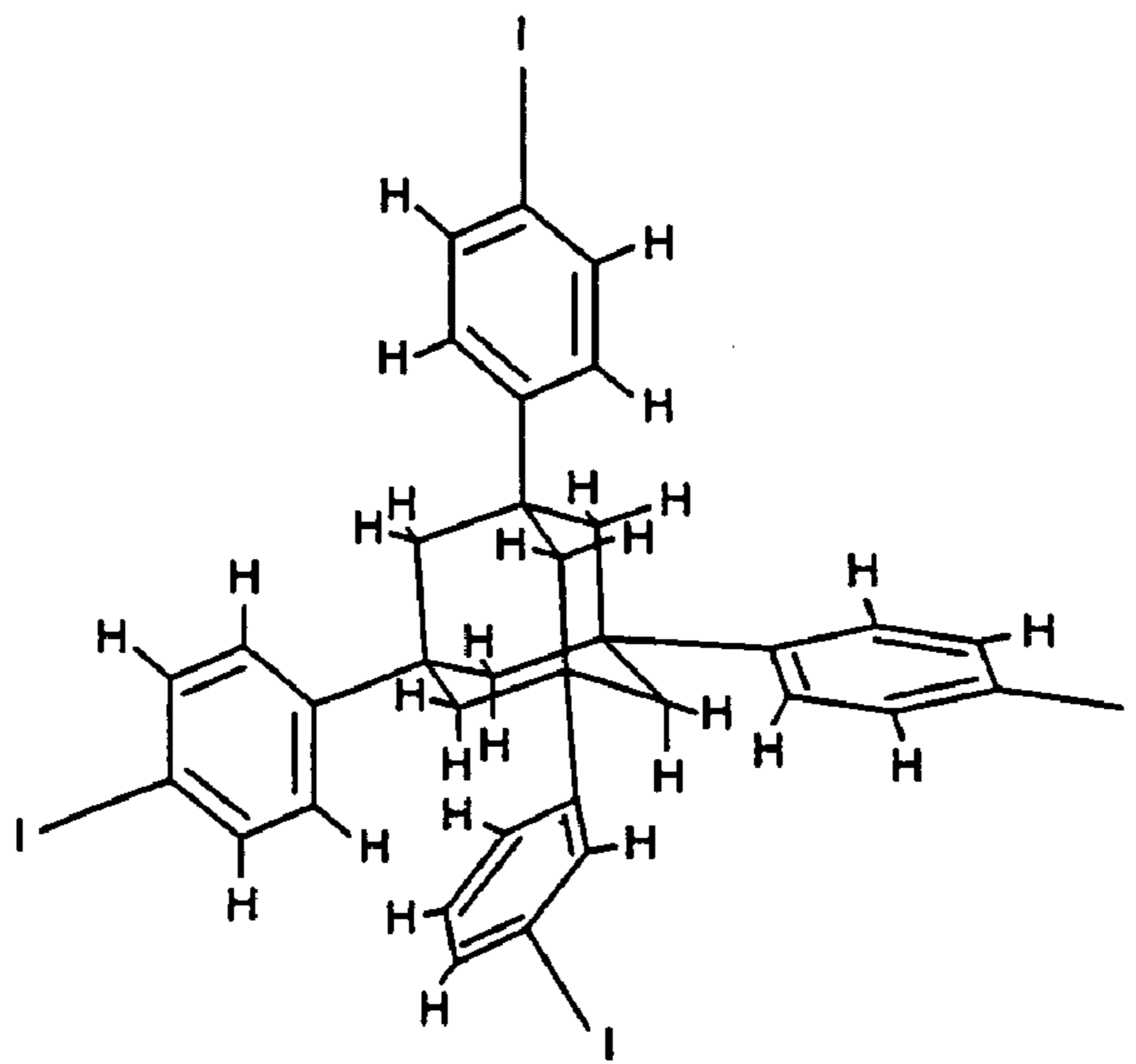
1,3,5,7-tetrakis(4-iodophenyl)adamantane
