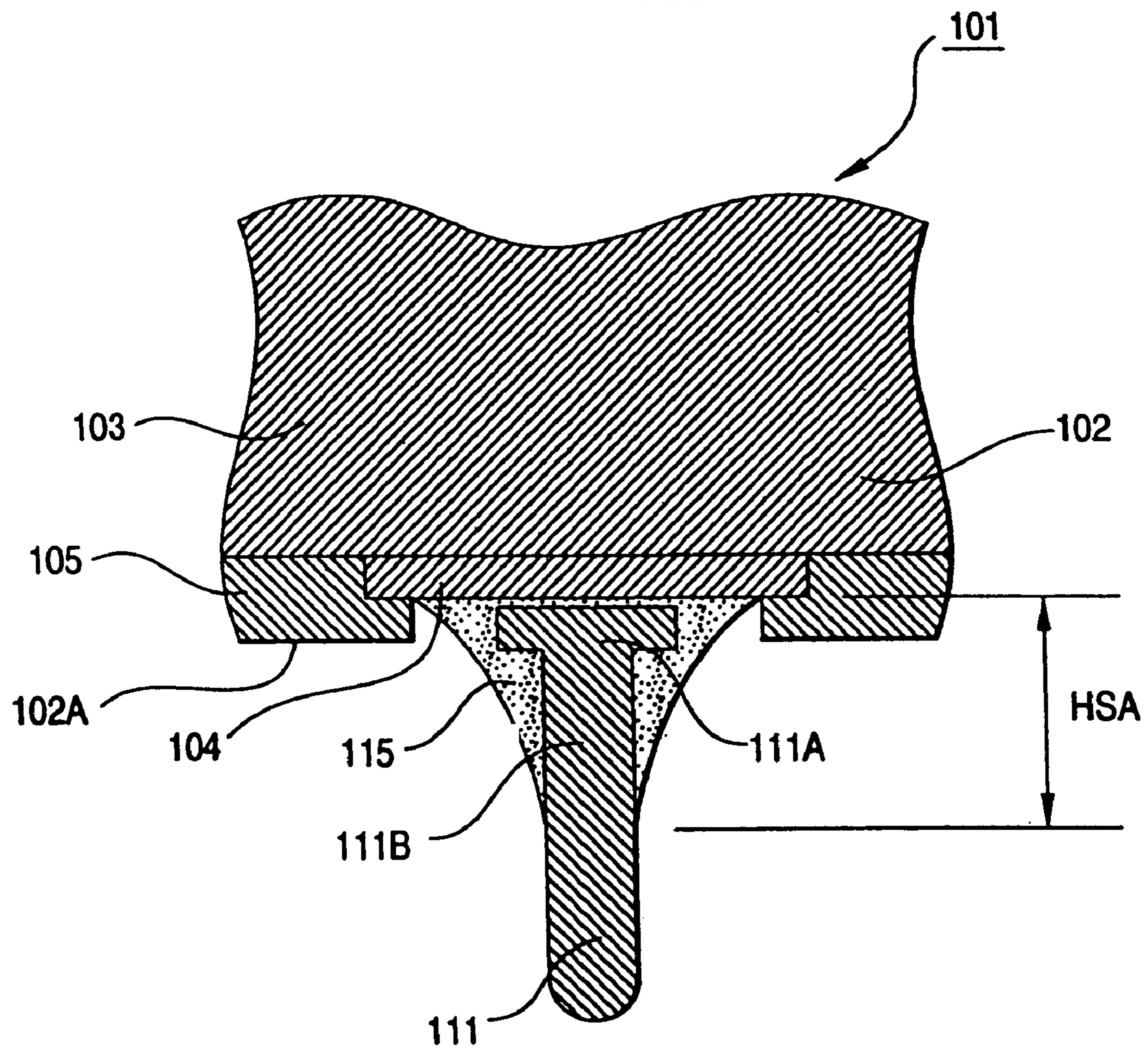
FIG. 6 PRIOR ART
