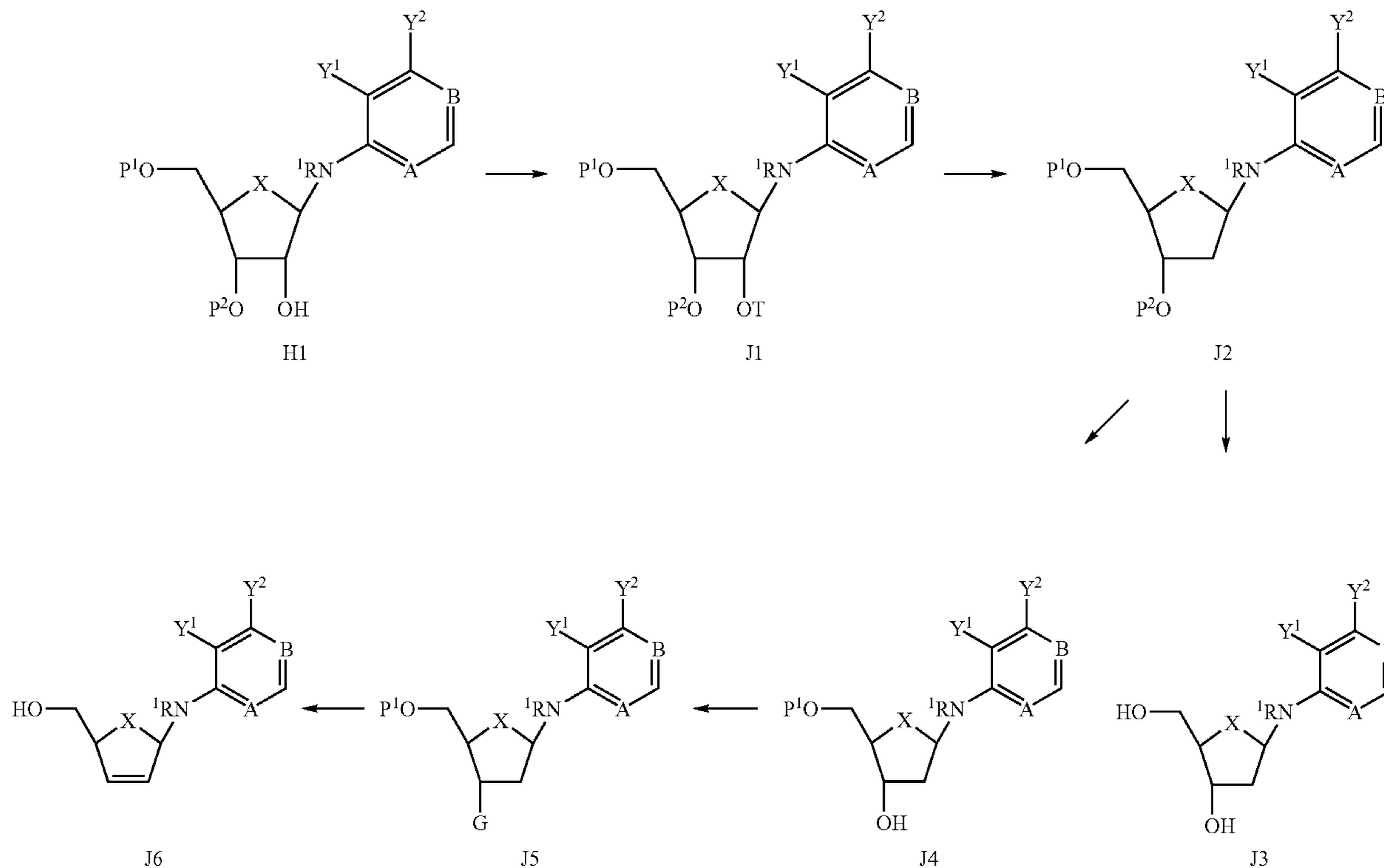
Scheme I
