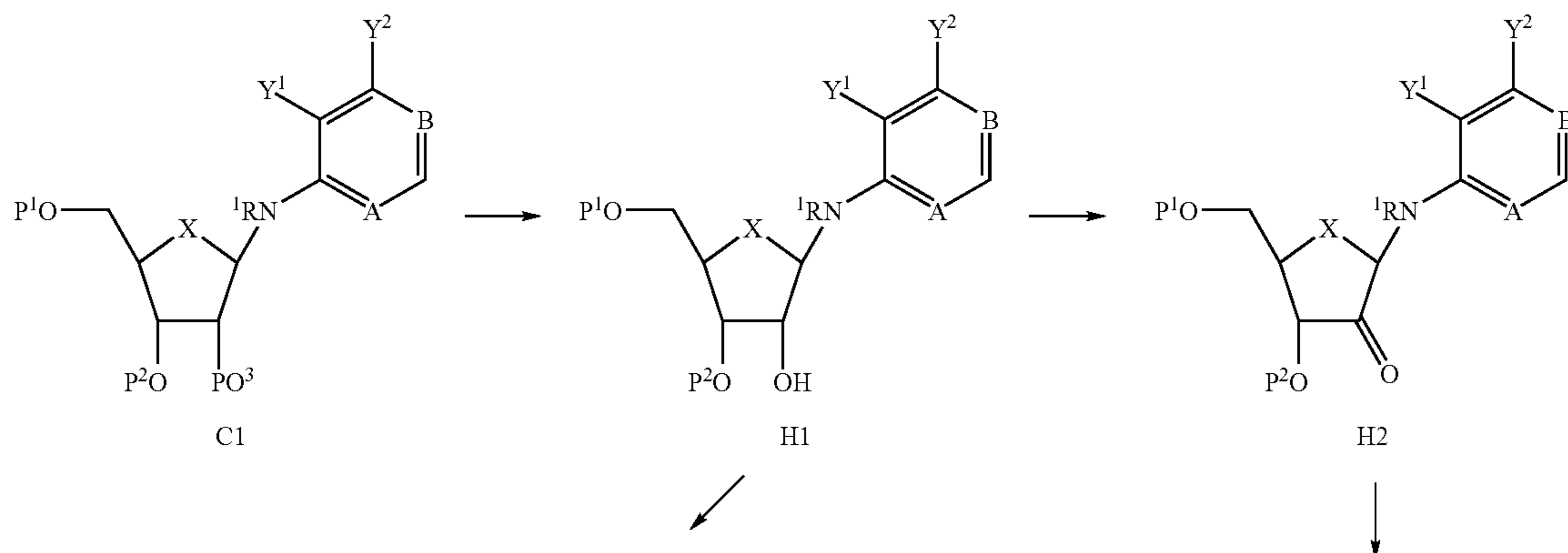
Scheme H
