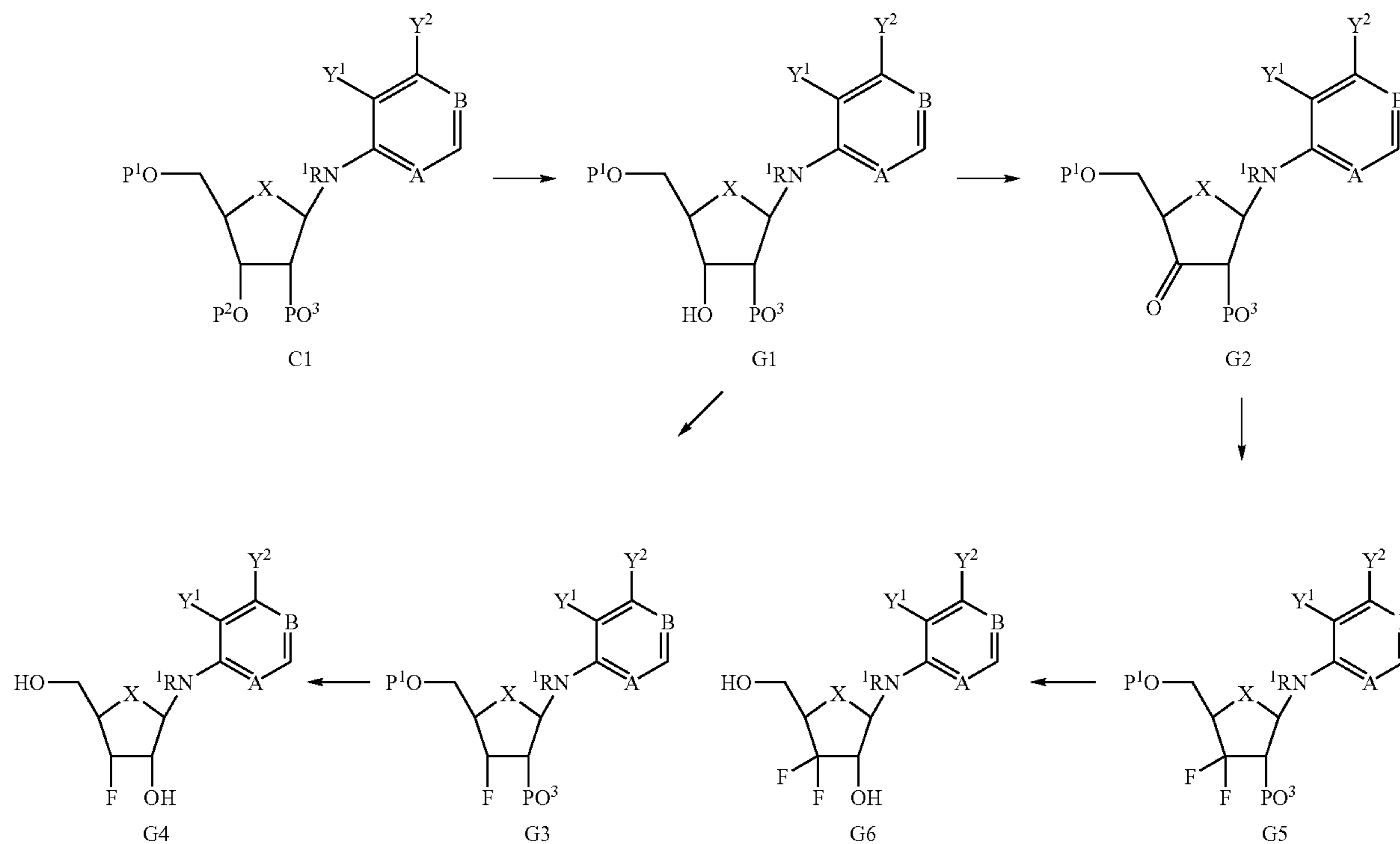
Scheme G
