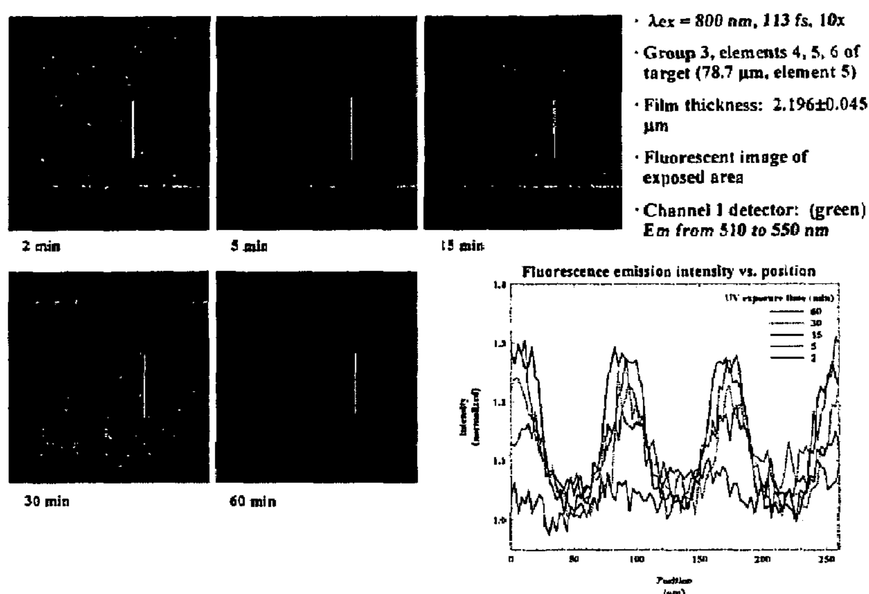
Figure 9. Two-photon fluorescent images of photosensitive films developed (via 350 nm broadband exposure, 4.4 \text{ mW}/\text{cm}^2 ) using an Air Force resolution target mask. Image recorded by channel 1 at various exposure times. Data readout as a function of exposure time determined from fluorescence intensity by scanning an xy line across one set of three-member elements (yellow line across set 5).
