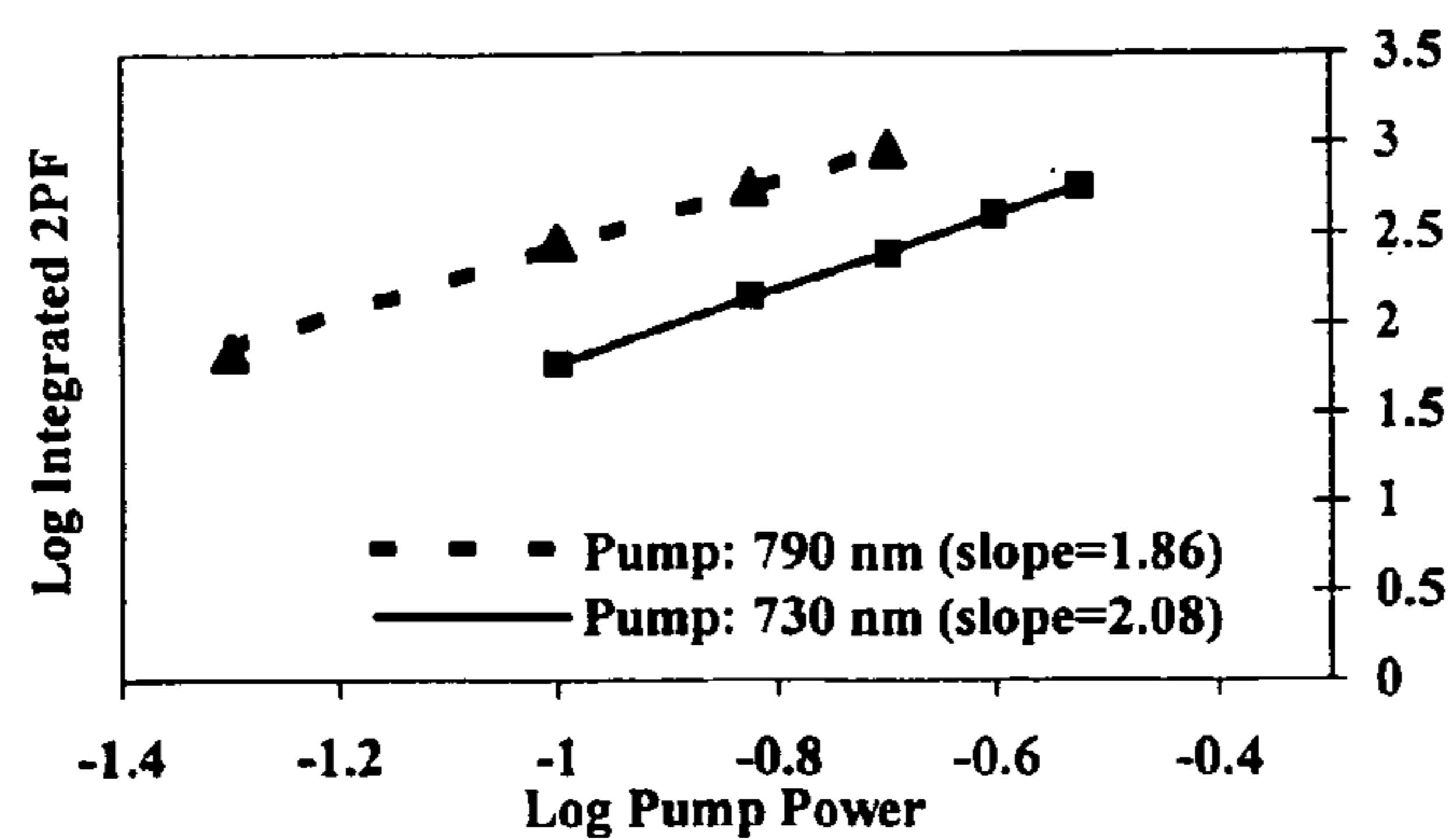
Figure 5. Plot of the total integrated fluorescence intensity of I as a function of pump power at two fs pump wavelengths.
