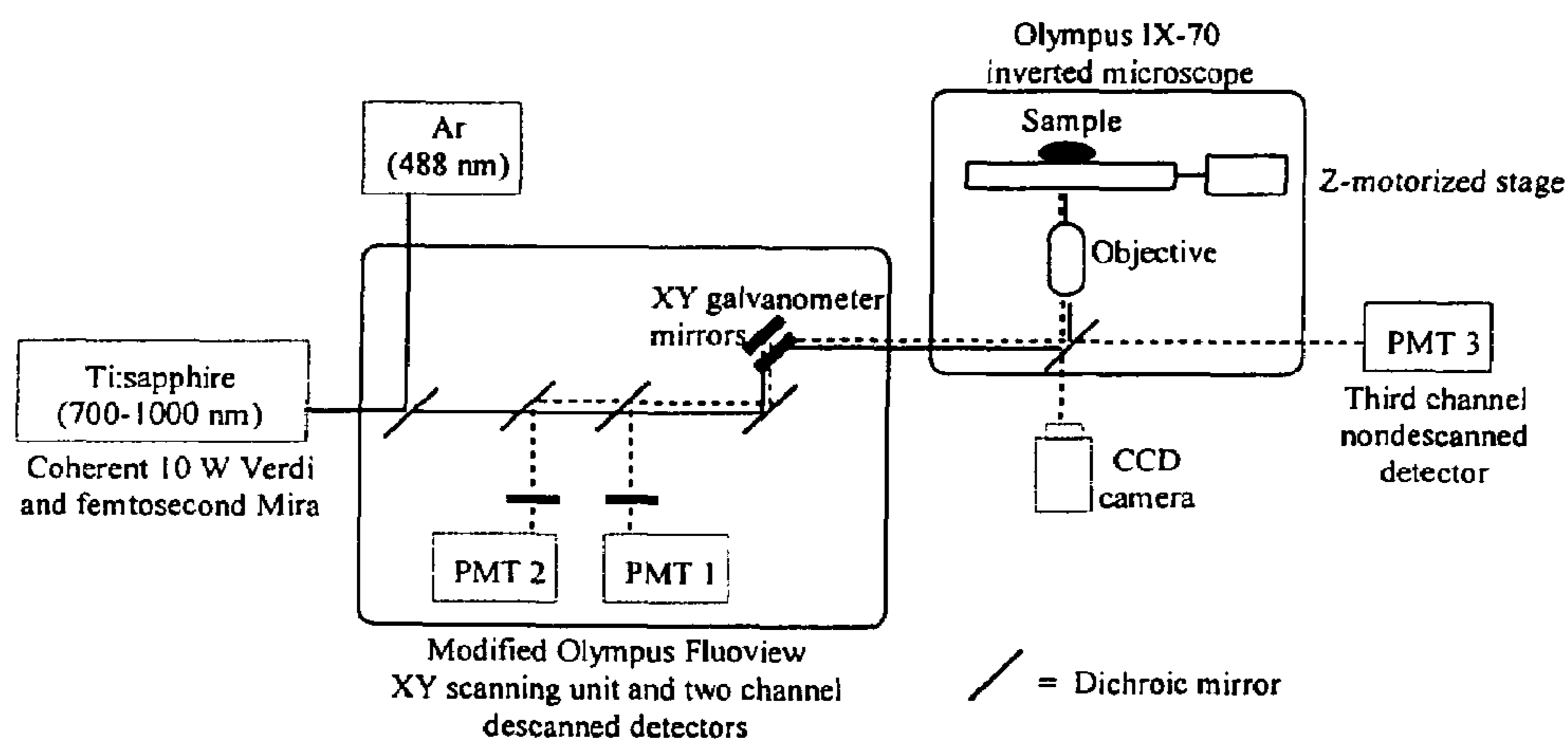
Figure 23. Schematic diagram of two-photon writing and recording system.
