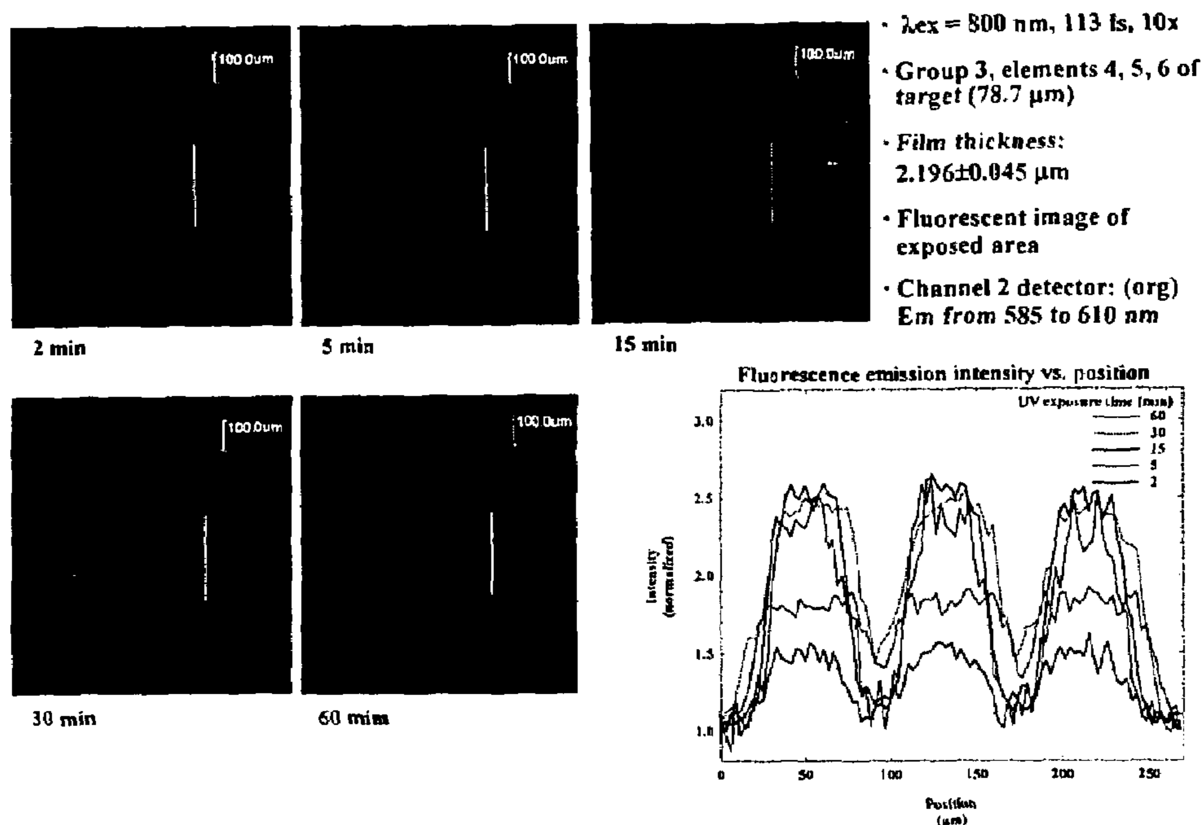
Figure 10. Two-photon fluorescent images of photosensitive films developed (via 350 nm broadband exposure, 4.4 \text{ mW/cm}^2 ) using an Air Force resolution target mask. Image recorded by channel 2 at various exposure times. Data readout as a function of exposure time determined from fluorescence intensity by scanning an xy line across one set of three-member elements (yellow line across set 5).
