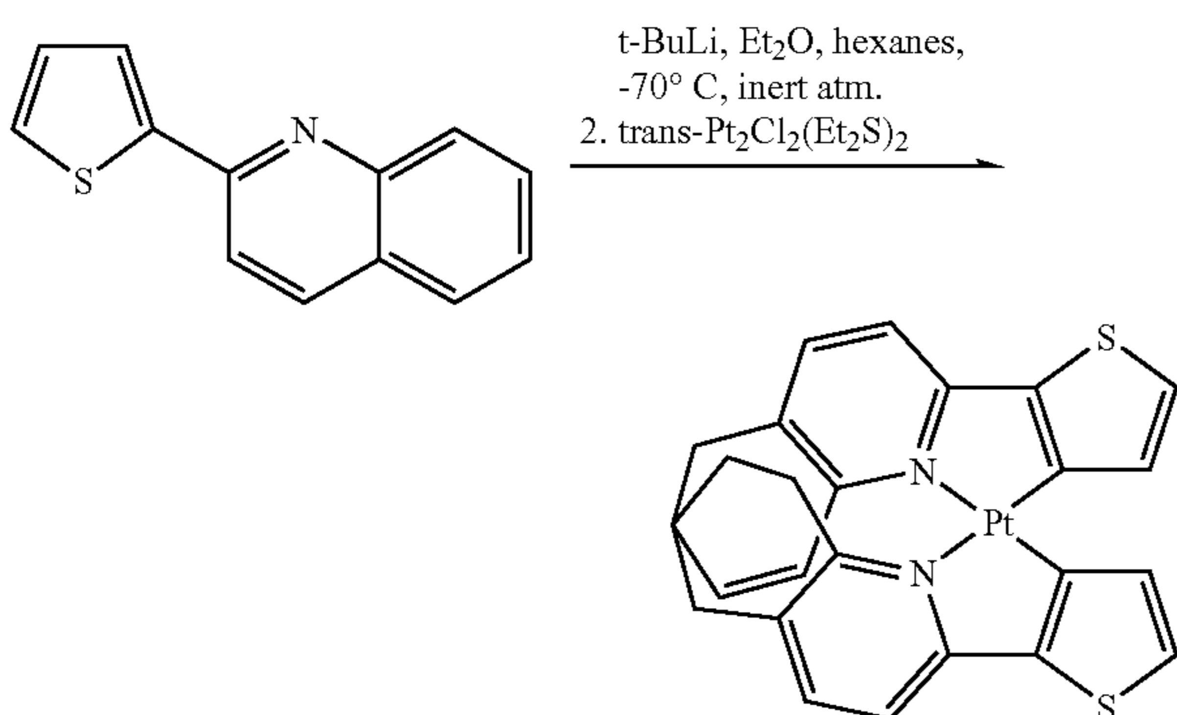
Scheme 10: Synthesis of cis-Bis[2-(2'-thienyl)quinolinato-N,C 5 ]platinum (II)
