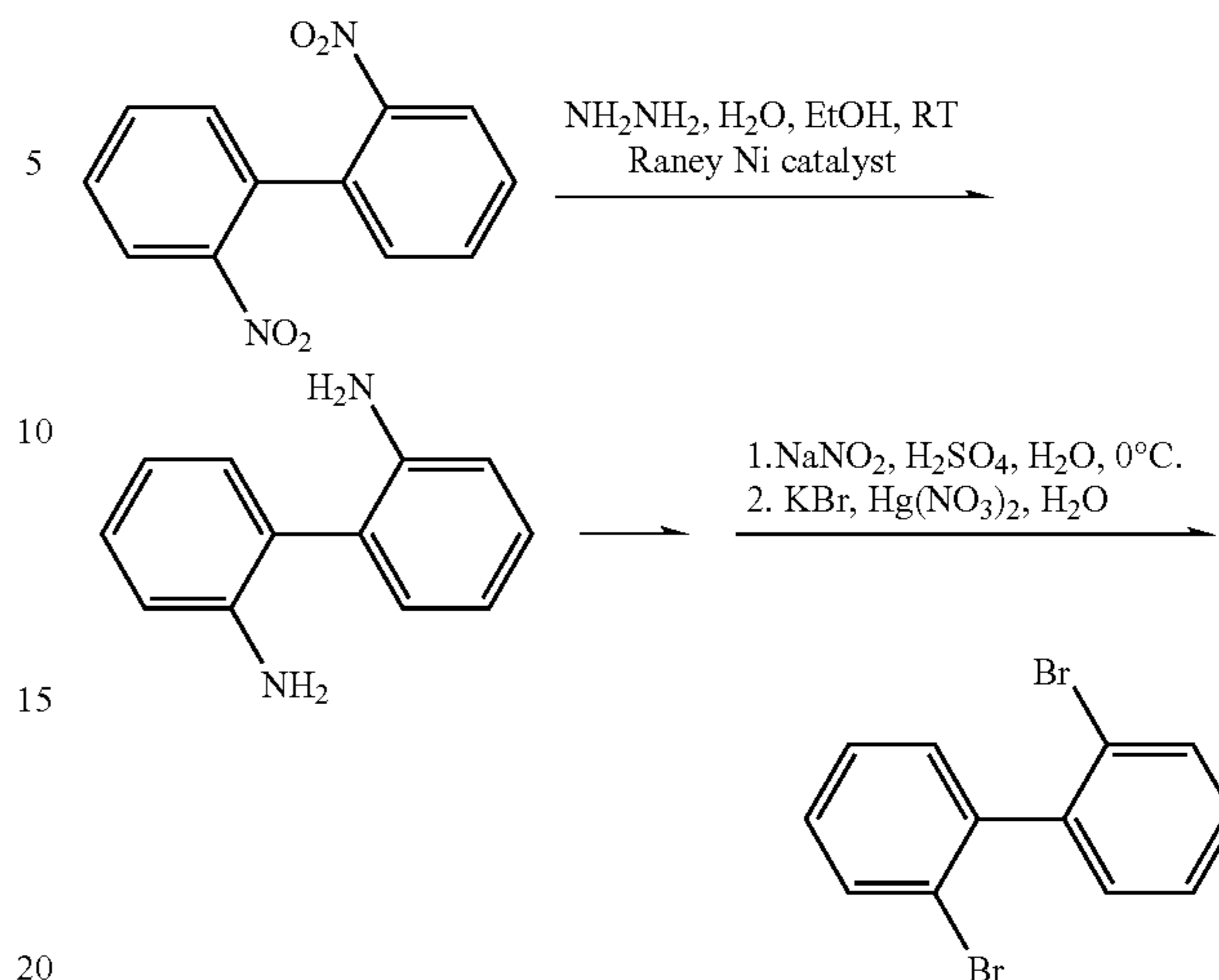
Scheme 6: Synthesis of 2,2'-dibromobiphenyl from 2,2'-dinitrophenyl.
