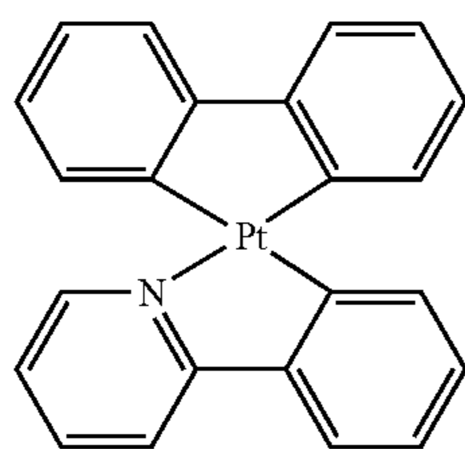
(Biphénylino-C,C)-(bipyridino-N,N) Pt (II) Pt(bph)(bpy)
