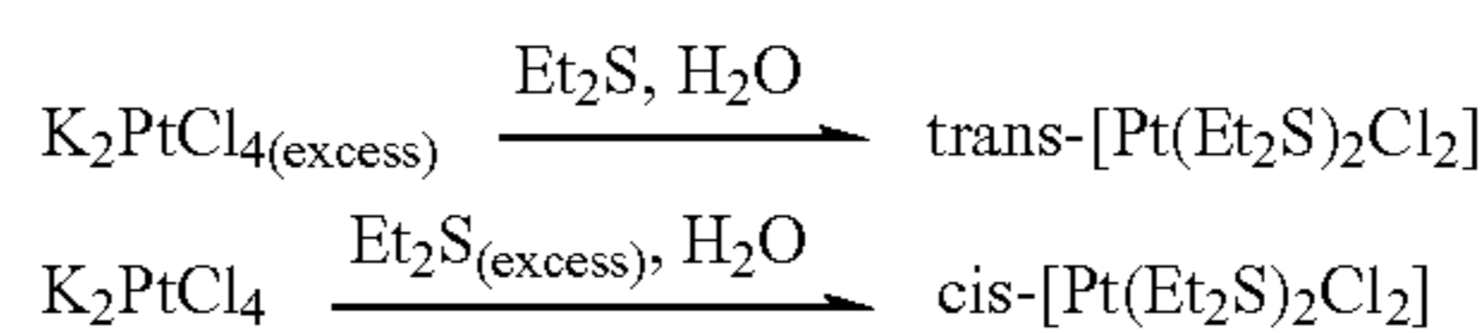
Scheme 8: Synthesis of cis- and trans-Dichloro-bis-(diethyl sulfide) platinum (II).
