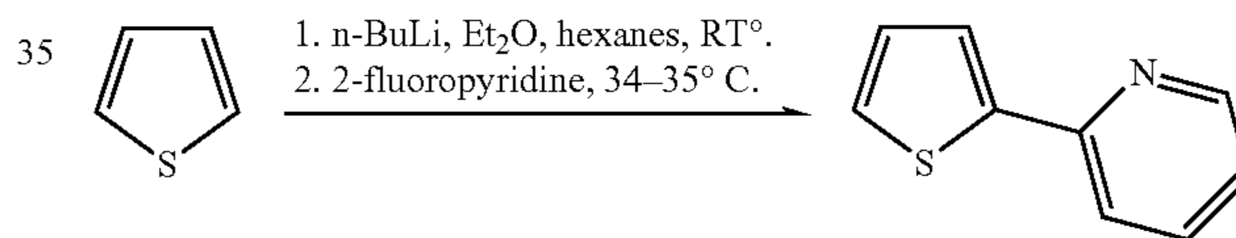
Scheme 2: Synthesis of 2-(2-thienyl)pyridine.
