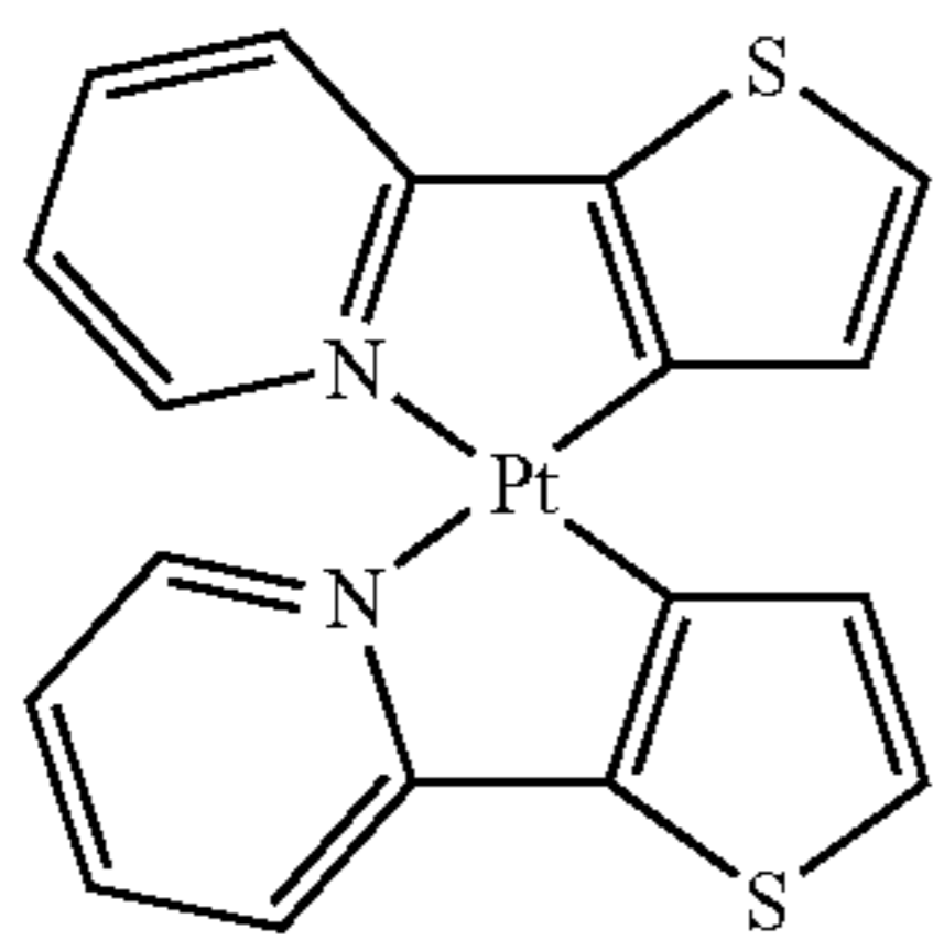
cis-Bis[2-(2-phenyl)pyridinato-N,C 2 ] Pt (II) Pt(Phpy) 2 (1)
