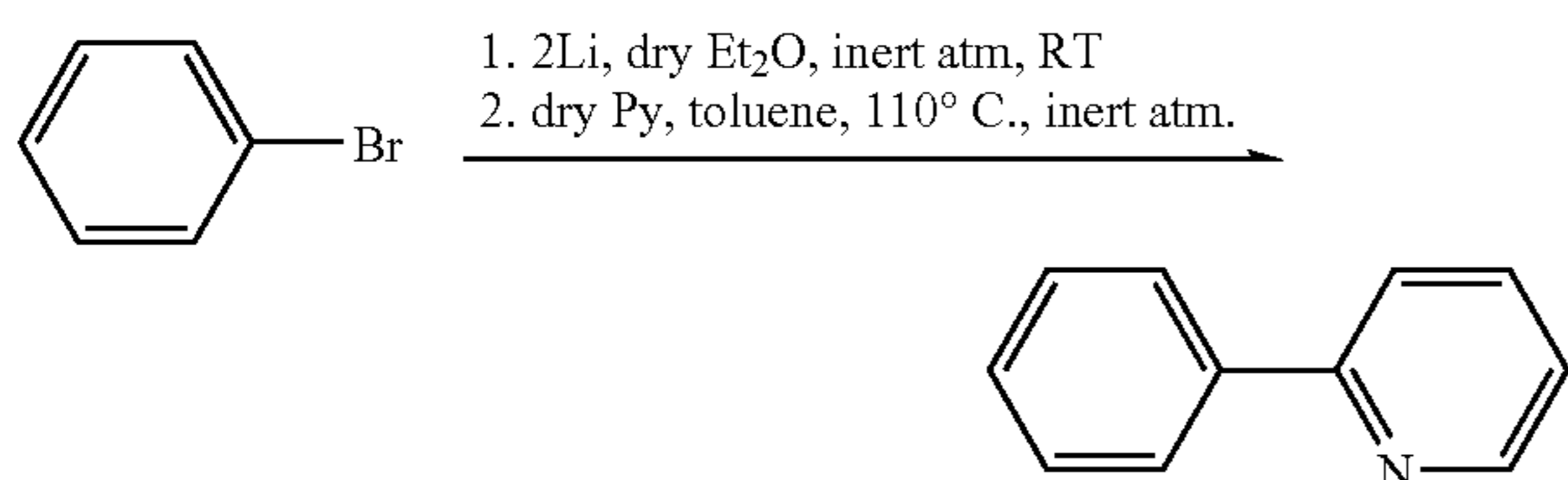
Scheme 5: Synthesis of 2-phenylpyridine.
