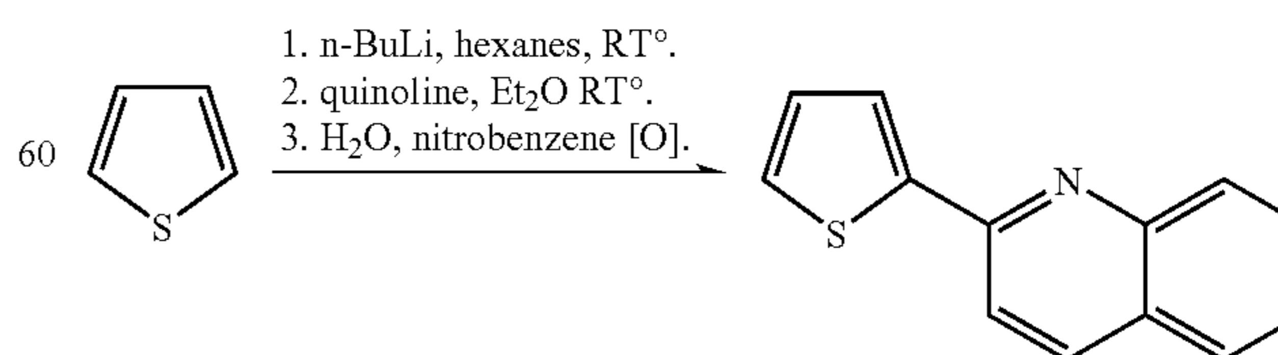
Scheme 3: Synthesis of 2-(2-thienyl)quinoline.
