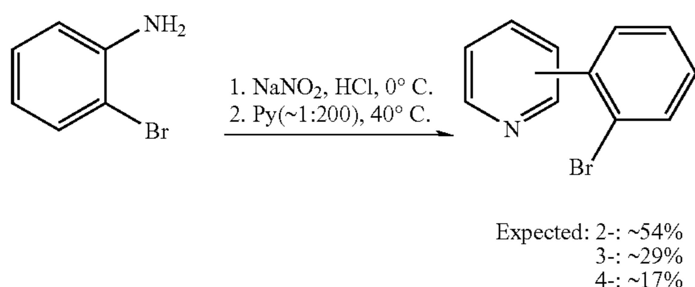
Scheme 4: Synthesis of n-(2'-bromophenyl)pyridines.
