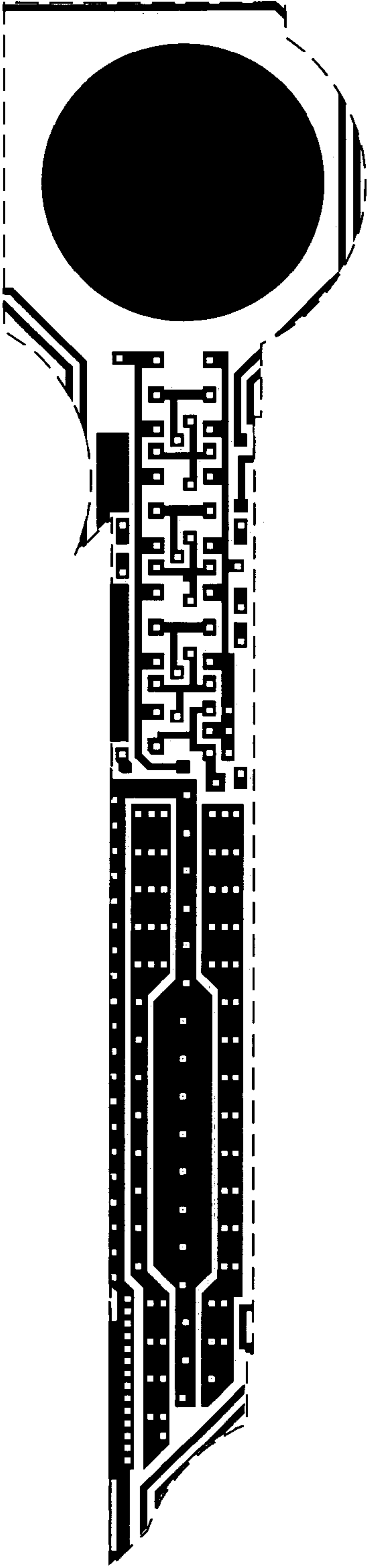
Metal 1 mask
