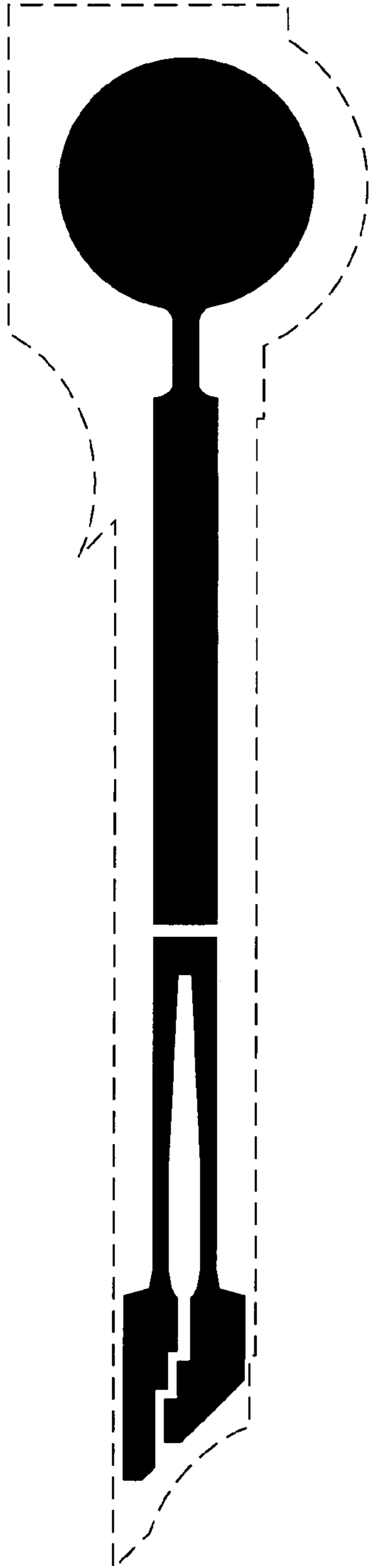
Heater mask
