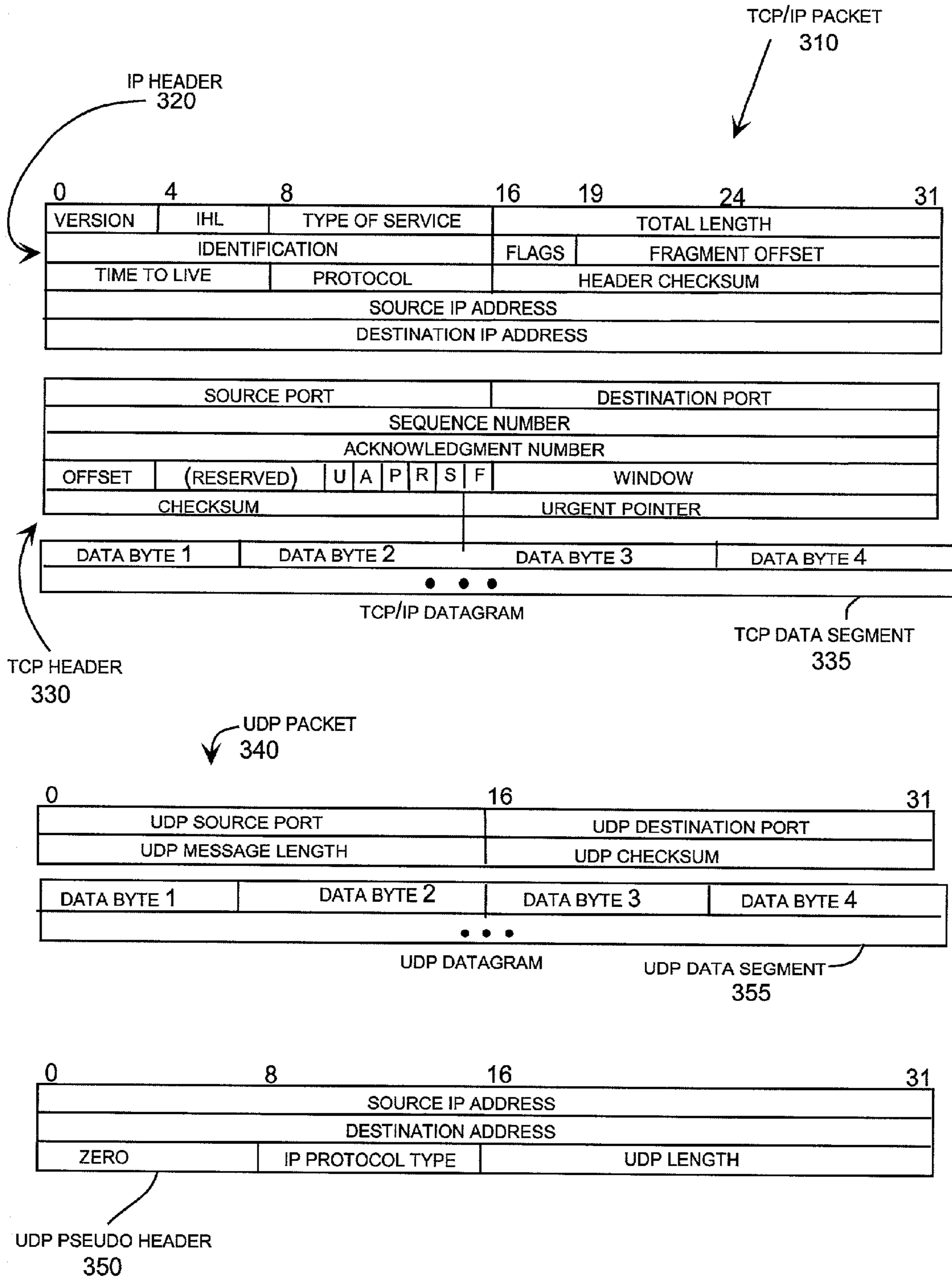
PACKET HEADERS FIG. 3
