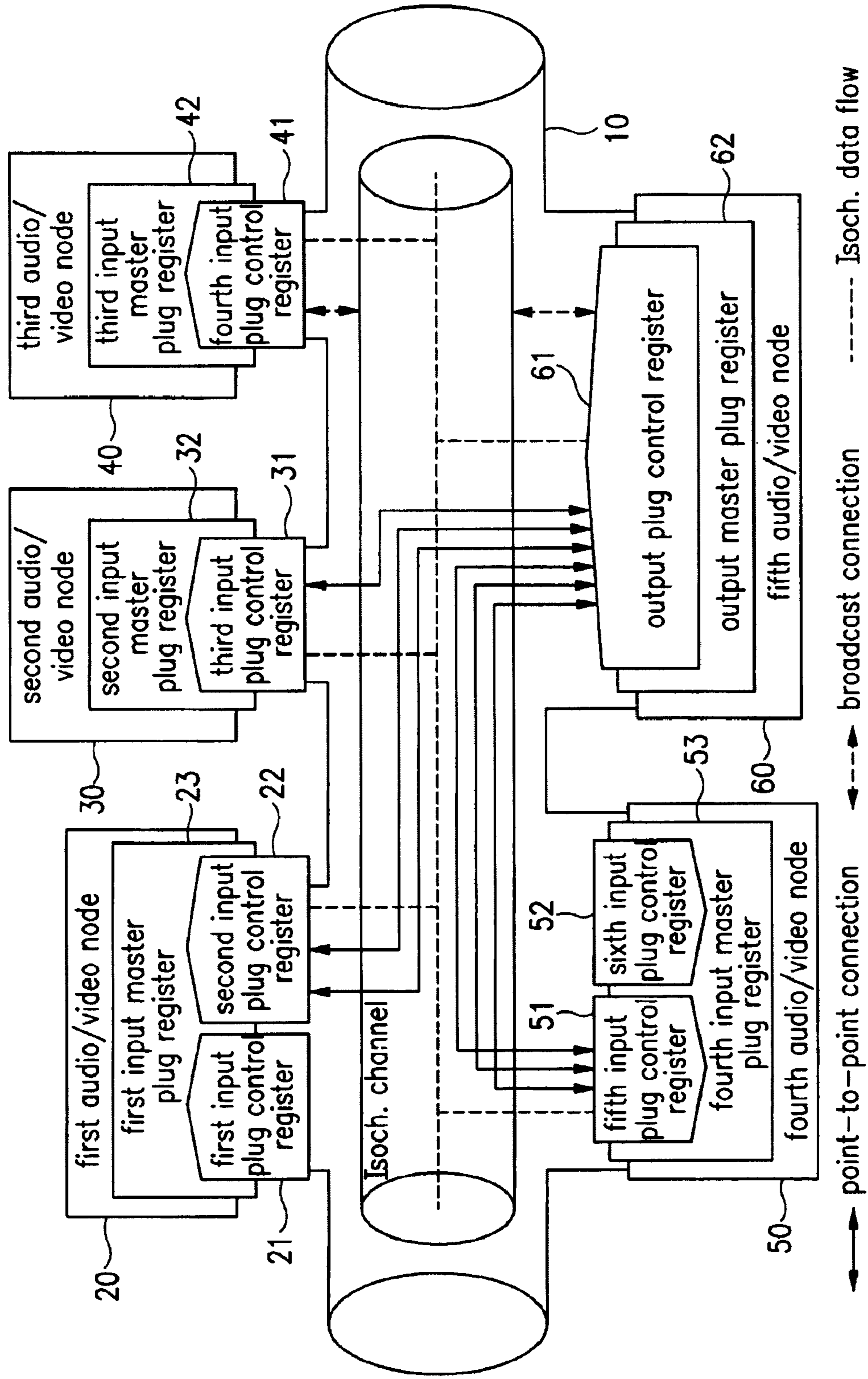
FIG. 1 Related Art
