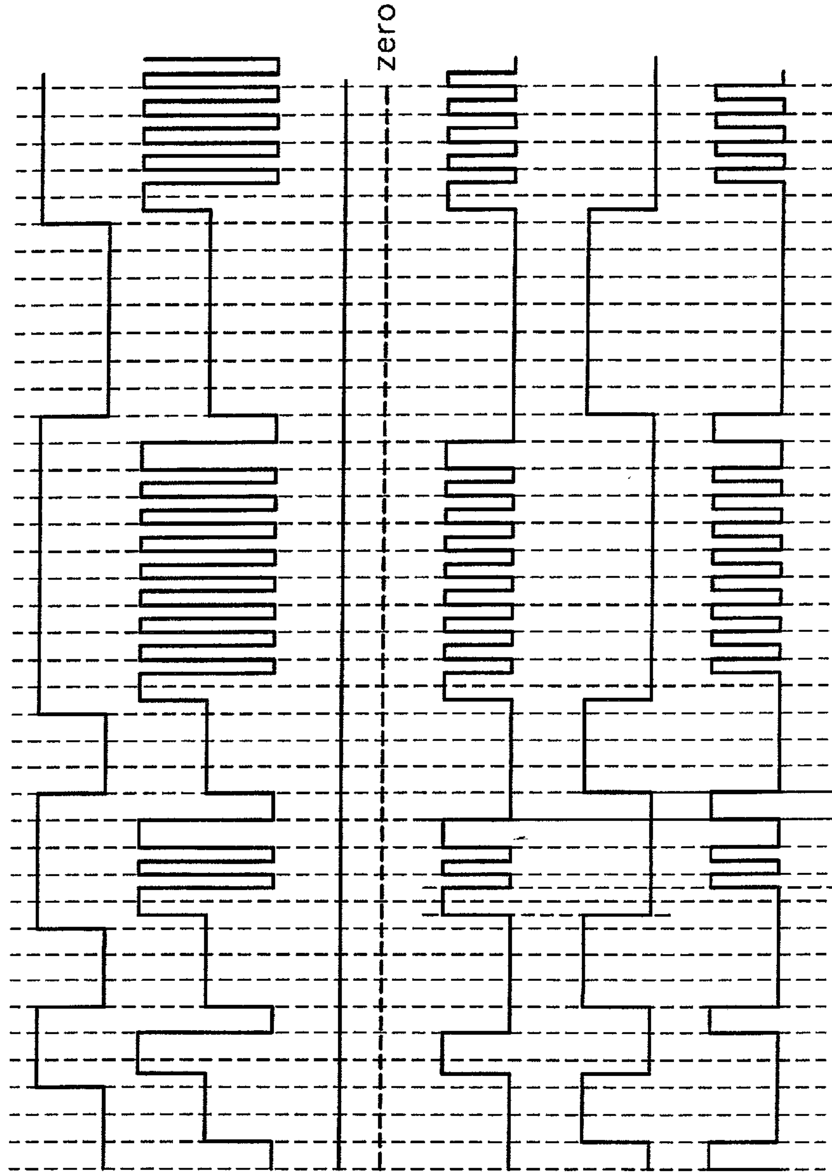
FIG. 8F Bottom Control (WHEN FOUR CHANNELS ARE USED)
