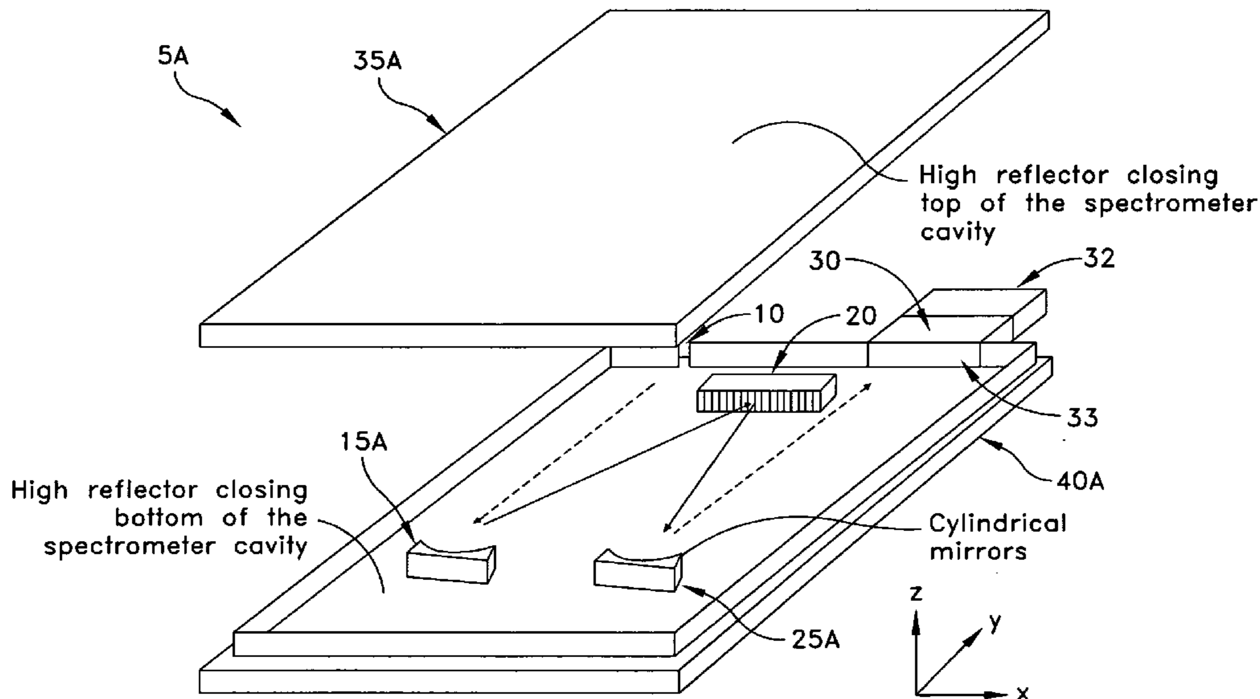
Slab spectrometer using cylindrical mirrors and two high reflectivity top and bottom plats to bound propogation of optical beam in z direction and allow construction of a thin spectrometer.
