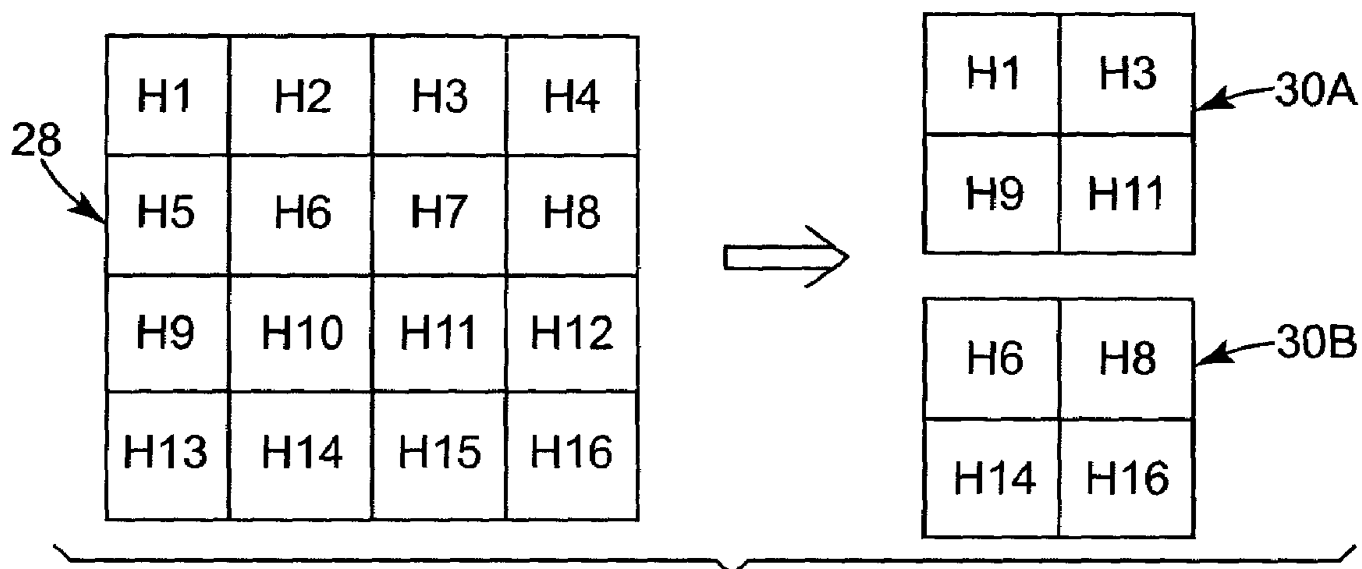
Fig. 5 (NEAREST NEIGHBOR)
