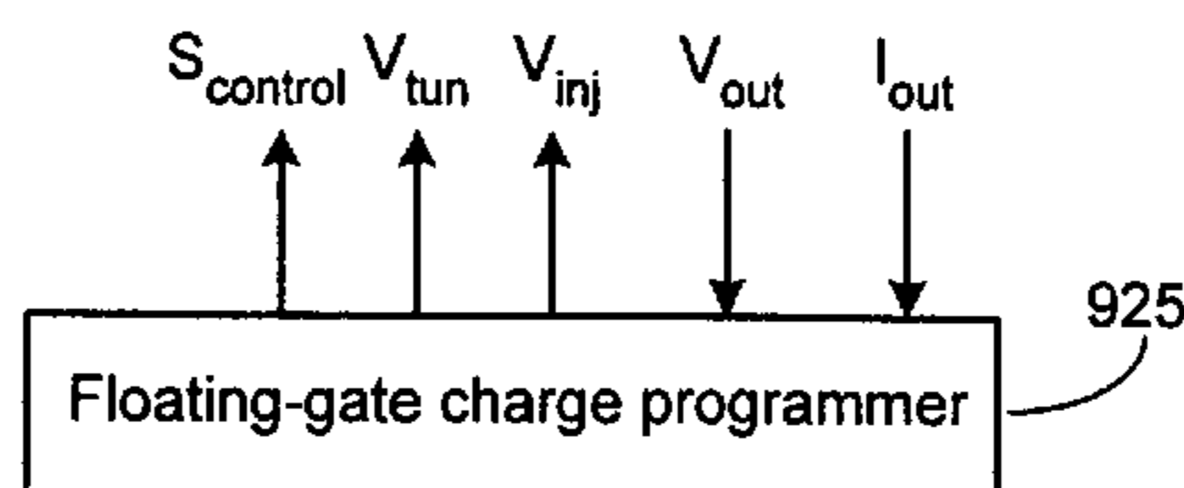
Programmer connections to/from individual MOSFETs (connections not shown on MOSFETs)
