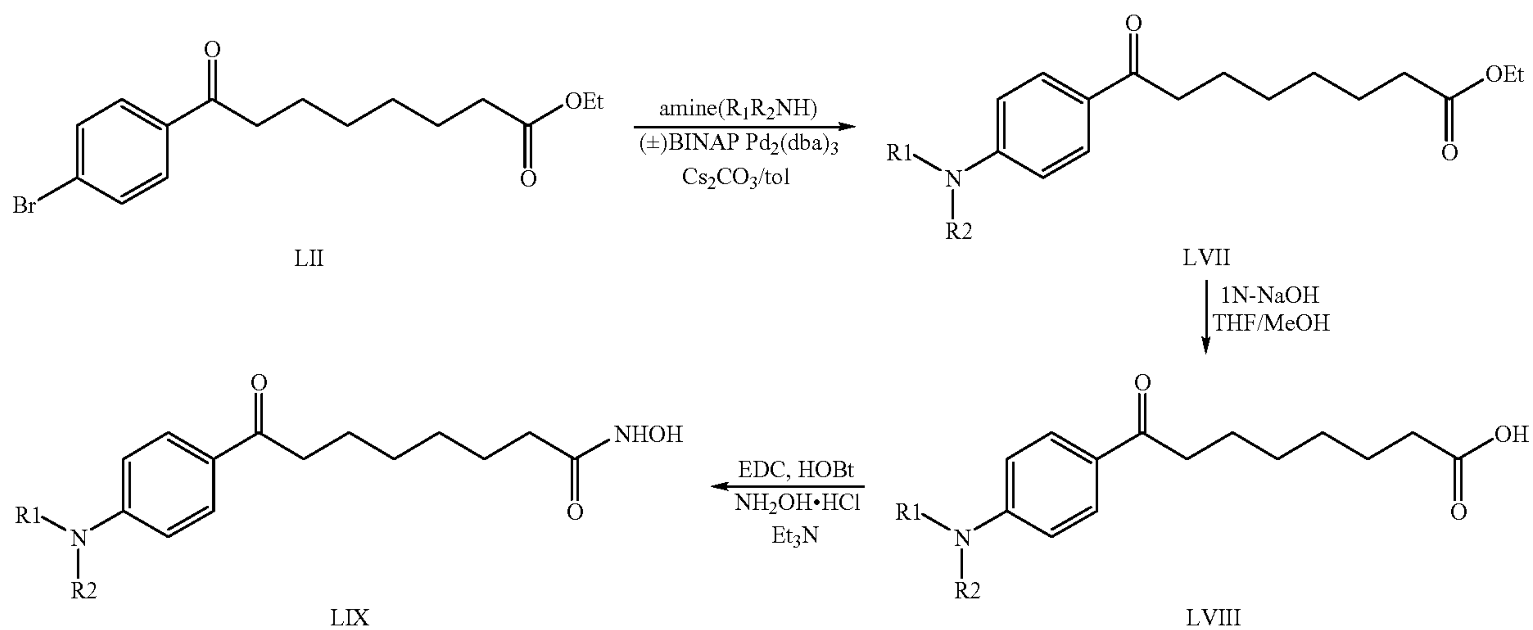
Scheme 11
