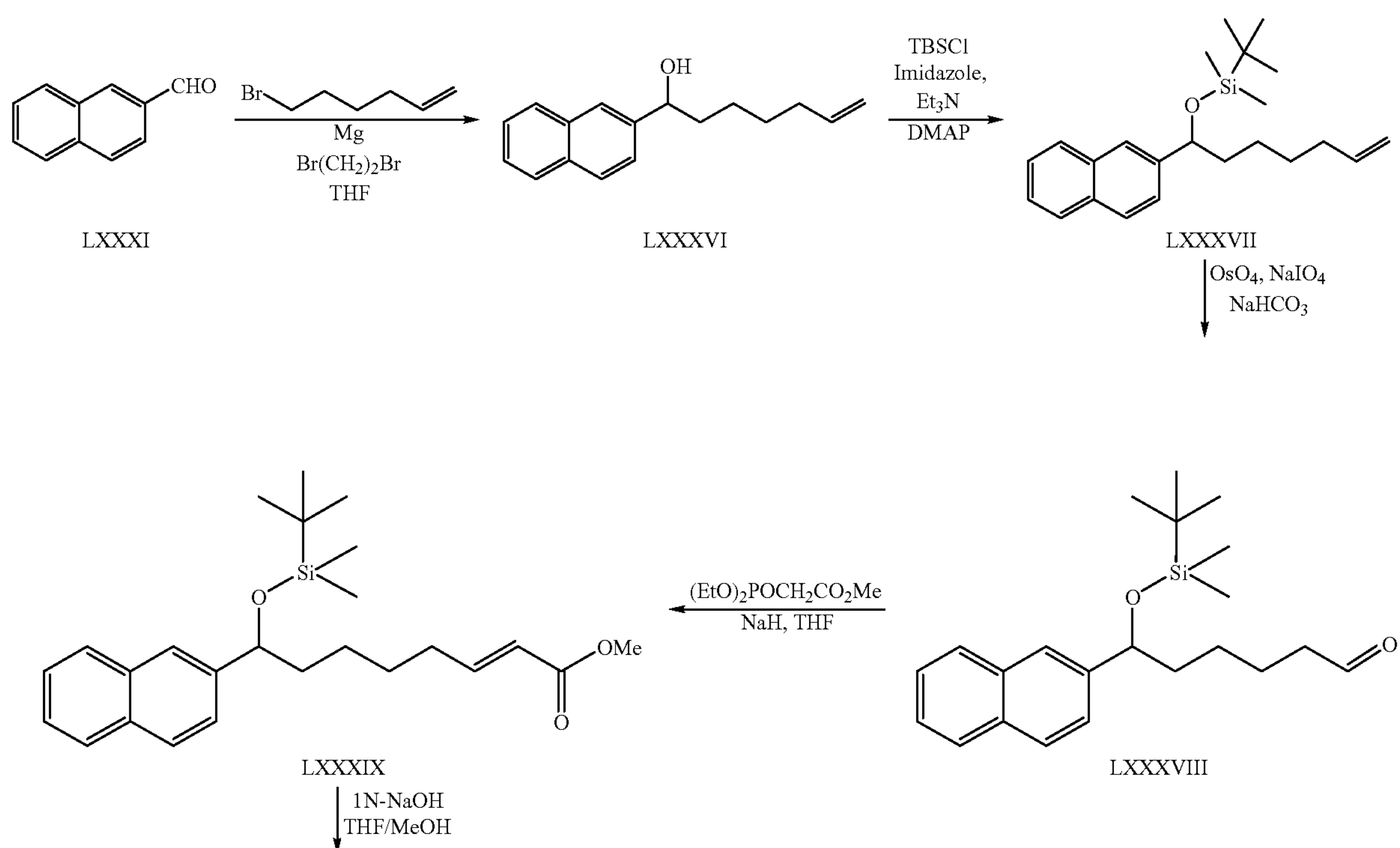
Scheme 16
