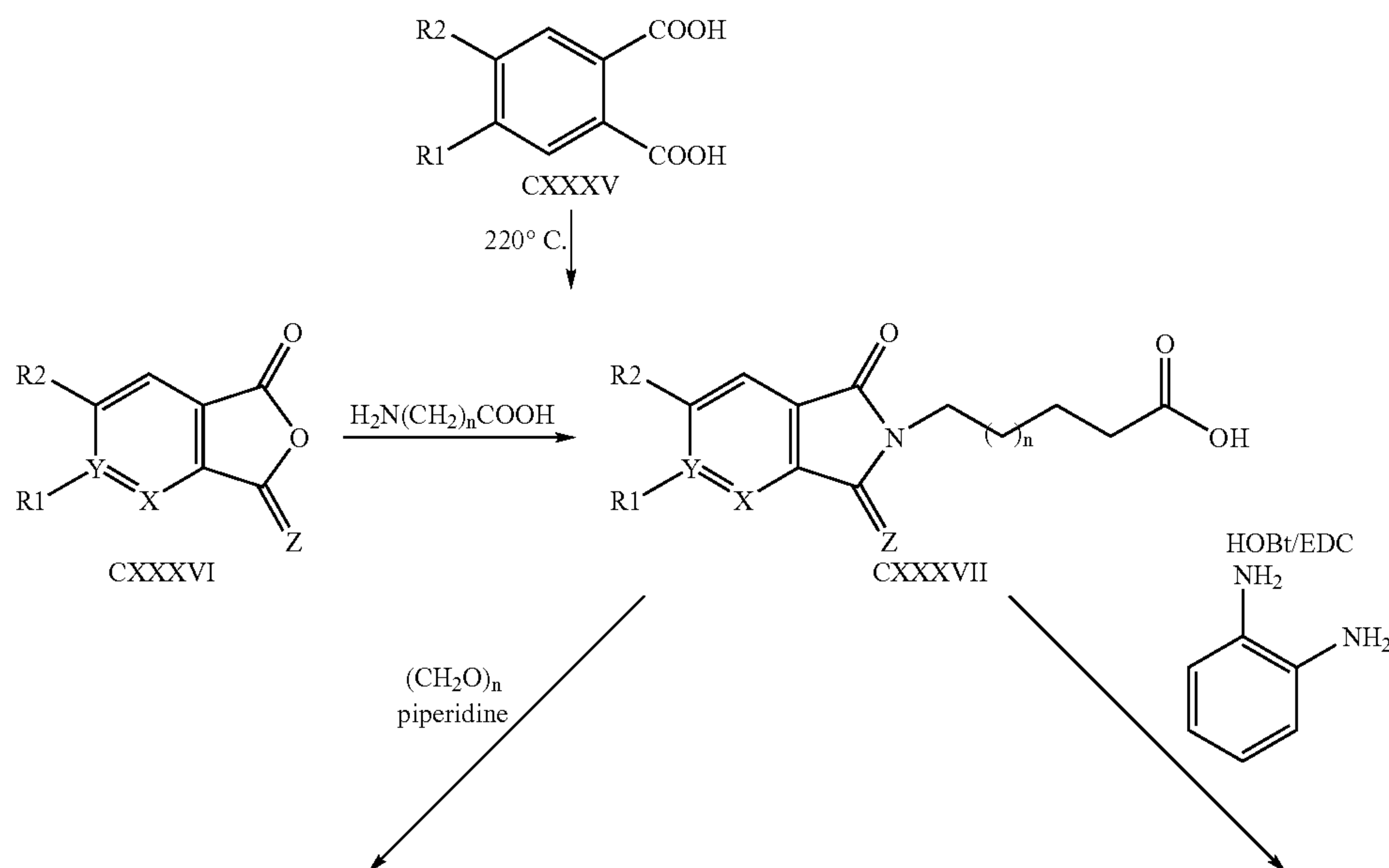
Scheme 23
