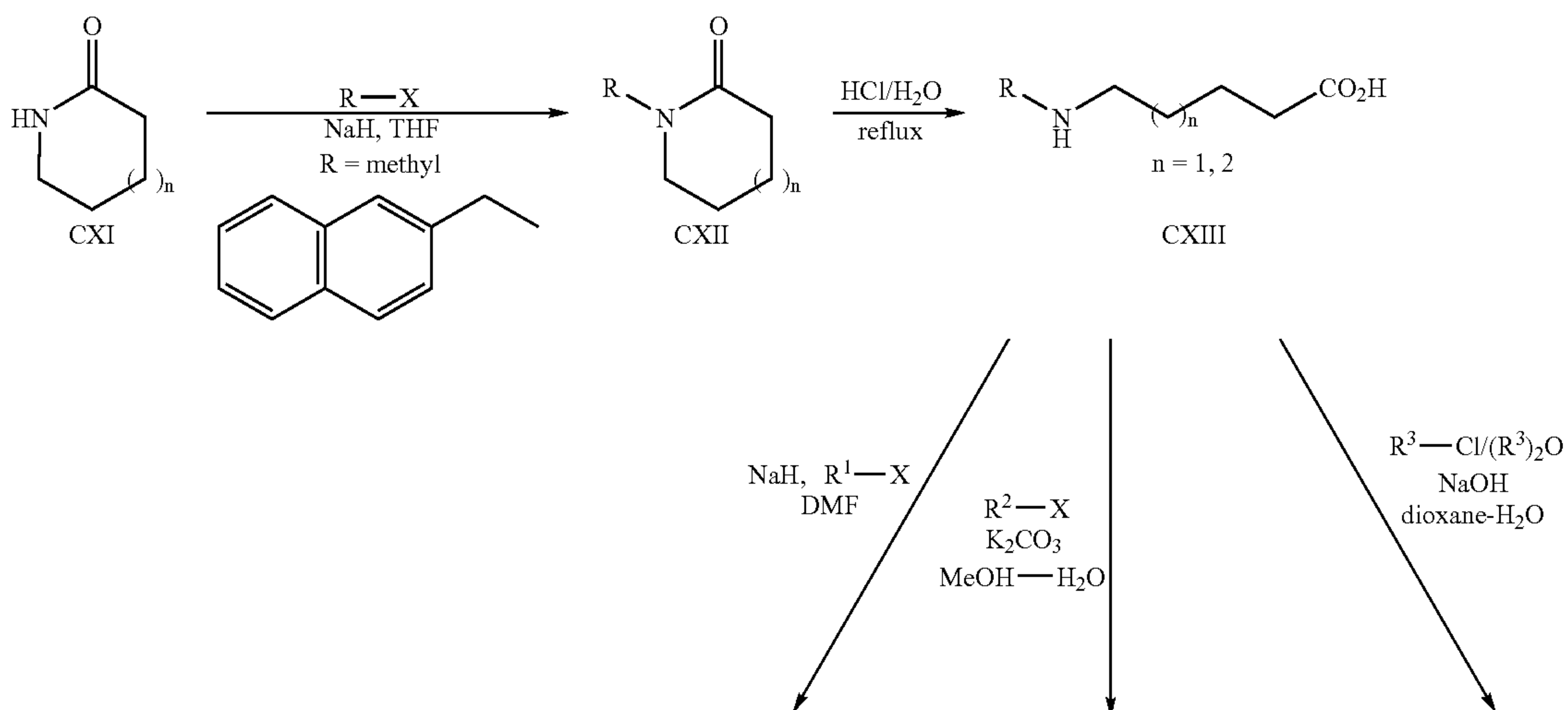
Scheme 19
