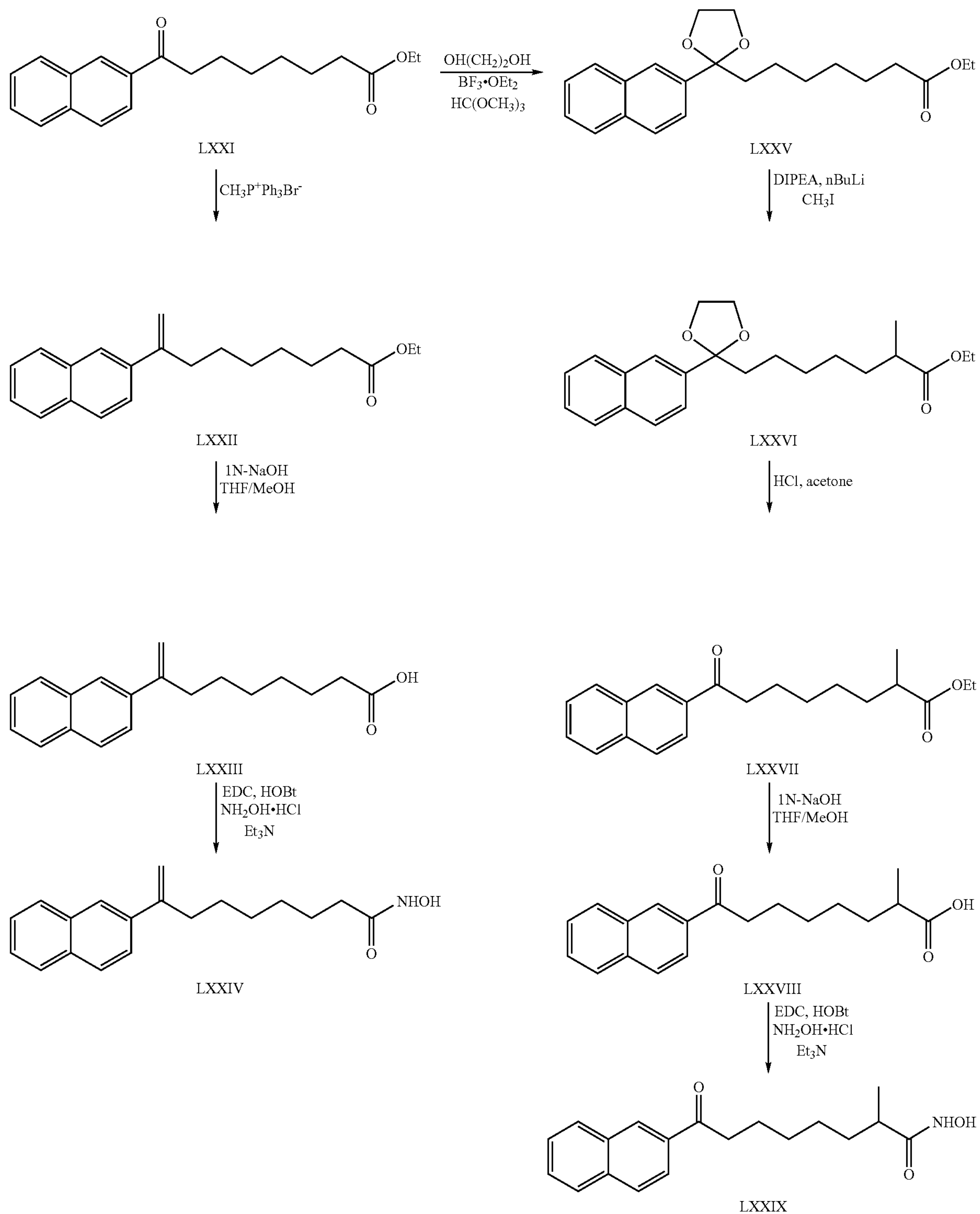
Scheme 14
