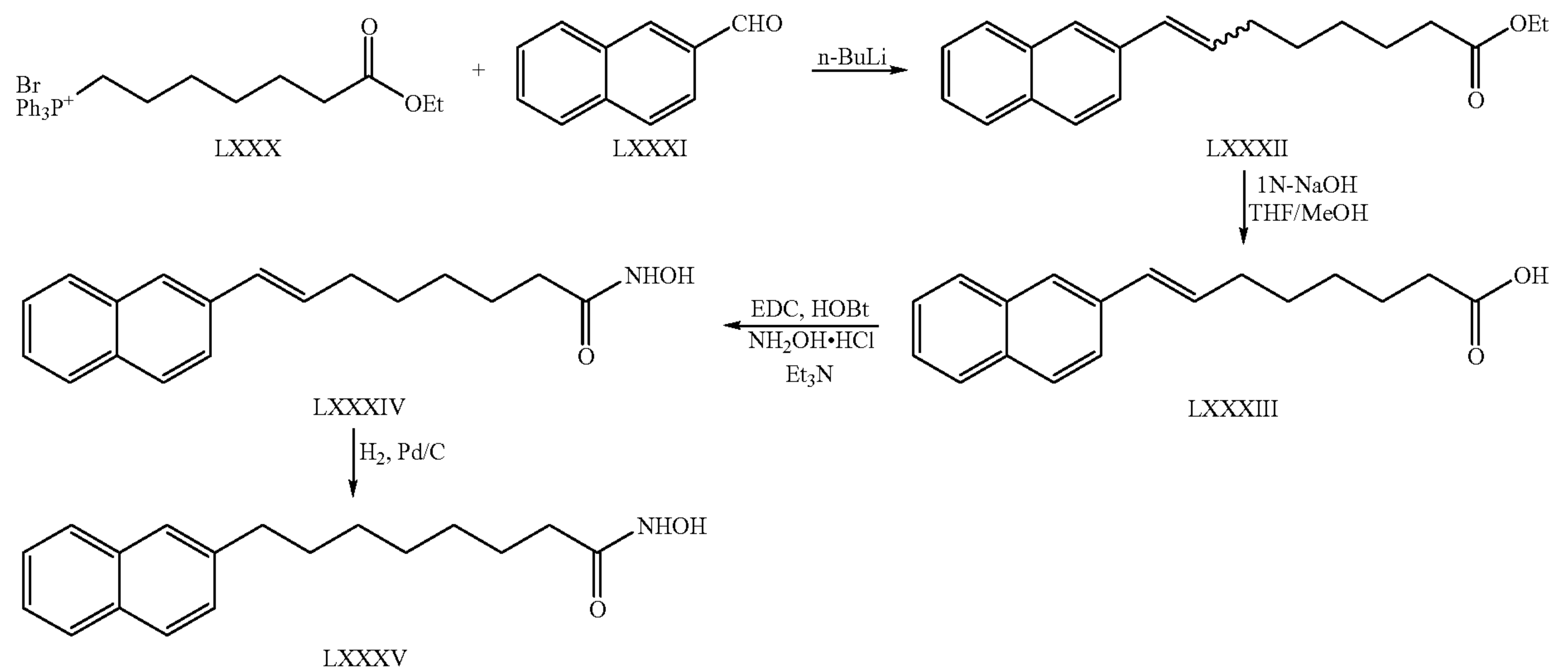
Scheme 15
