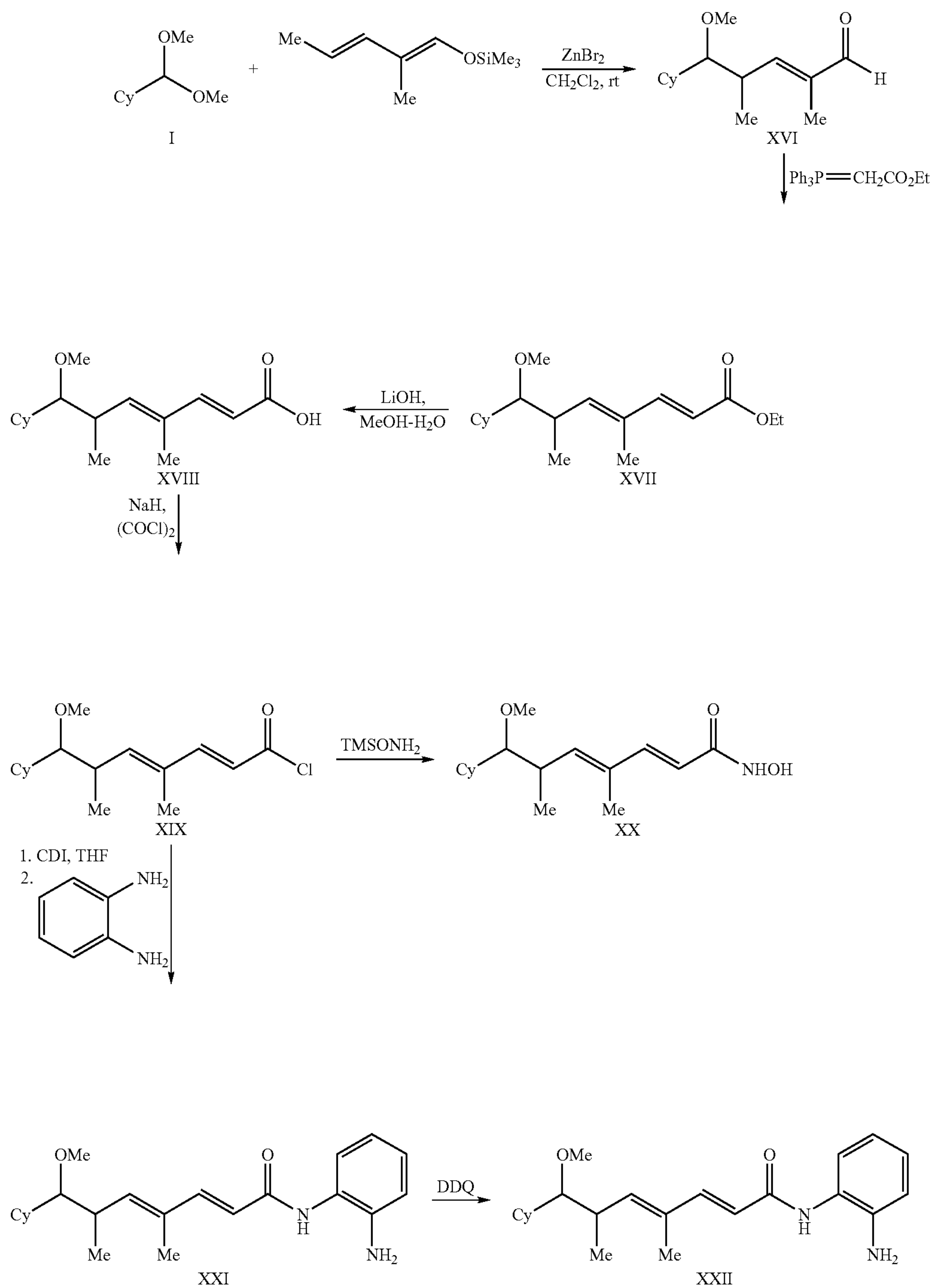
Scheme 3
