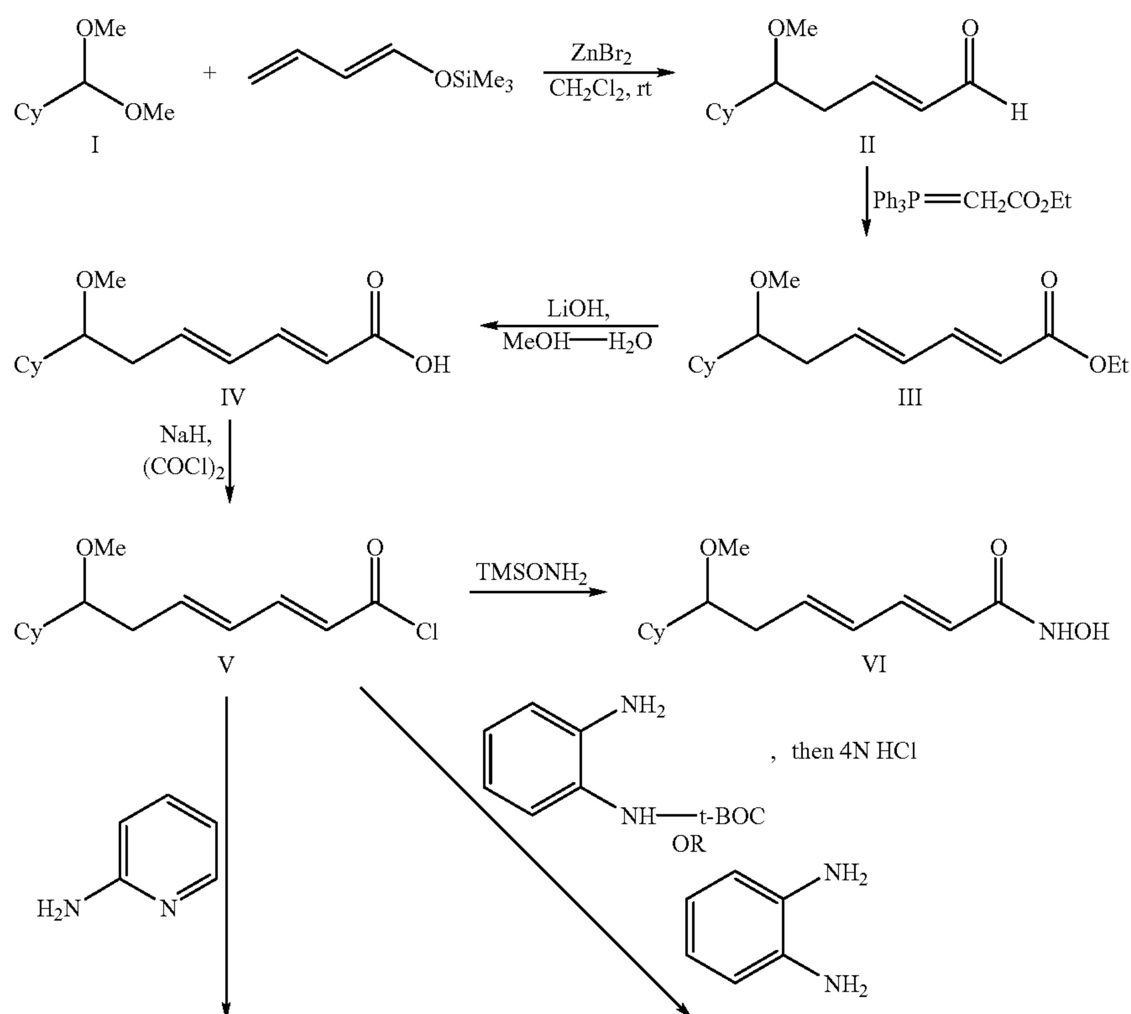
Scheme 1
