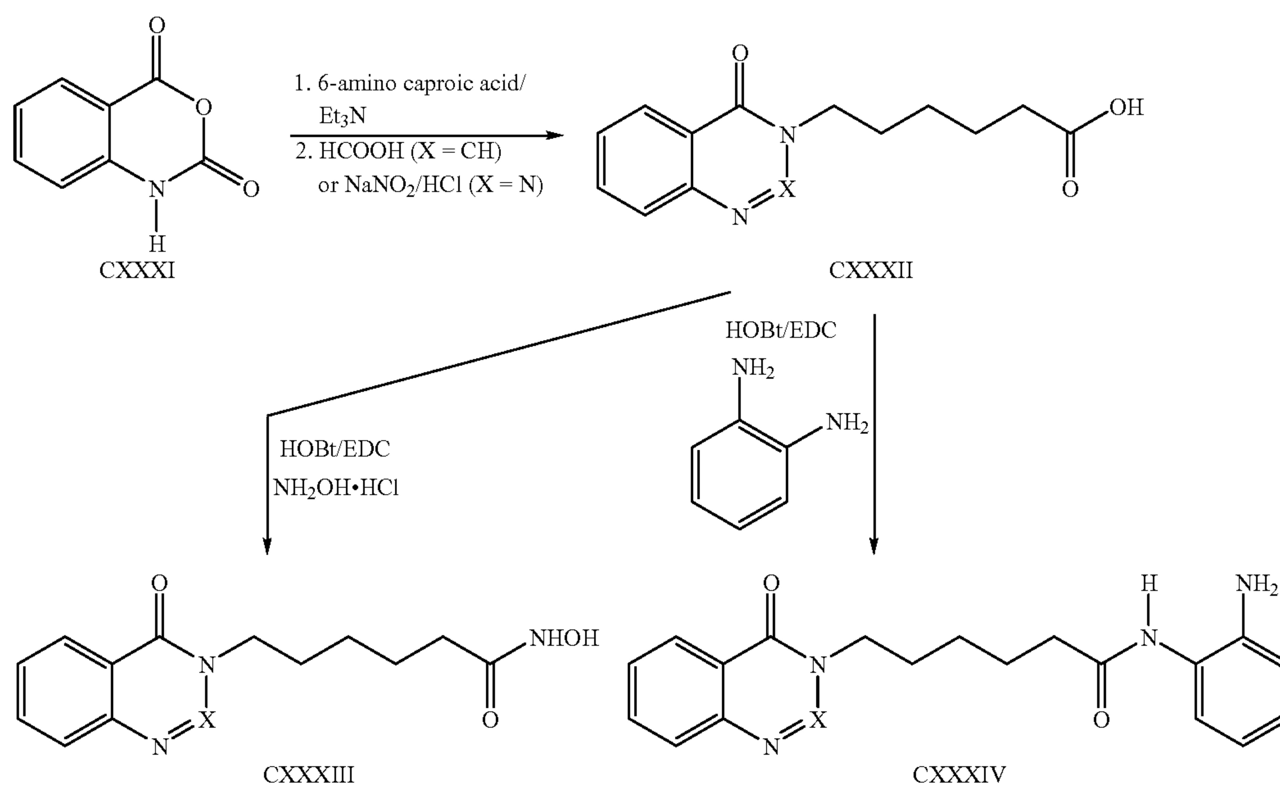
Scheme 22
