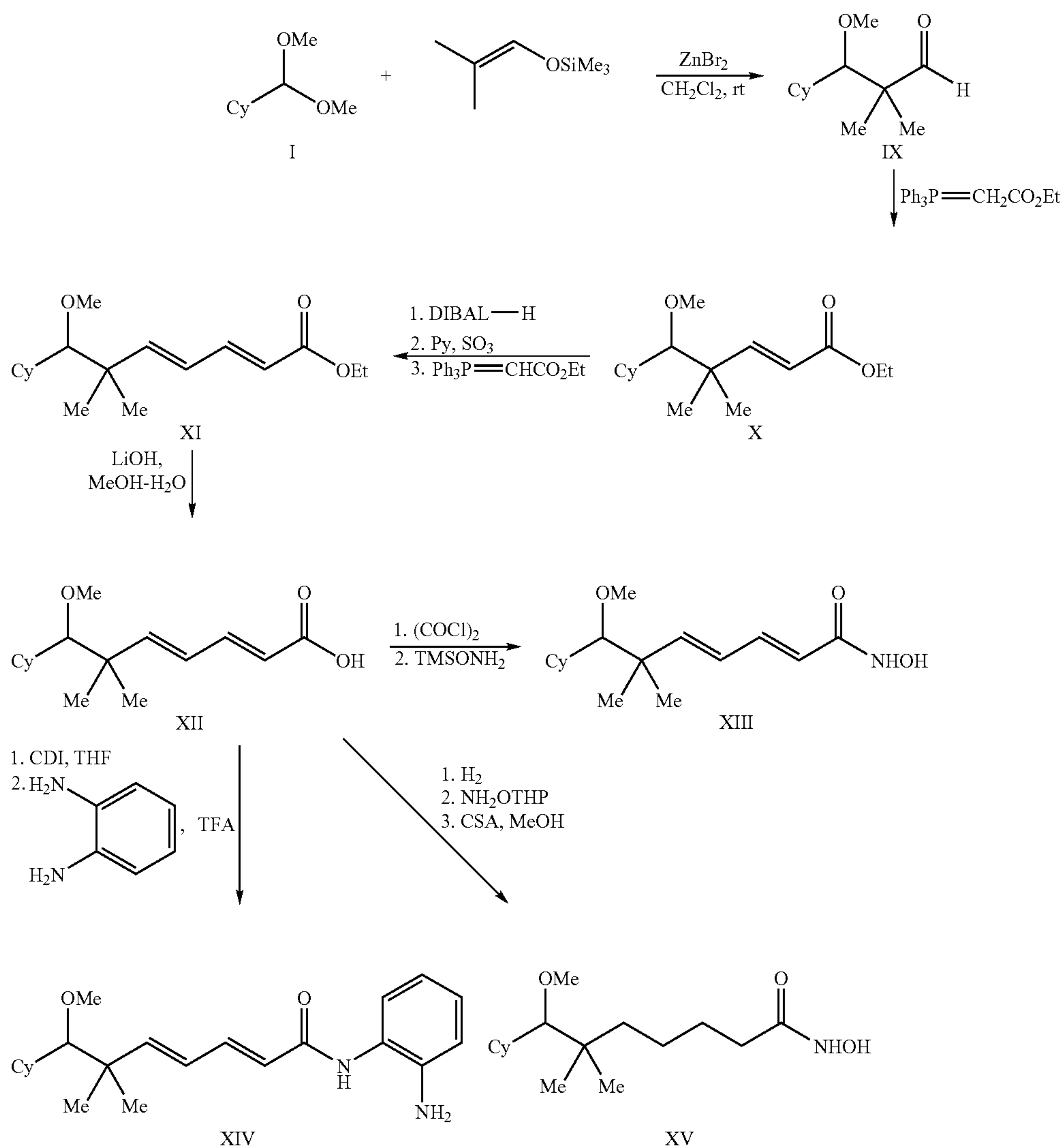
Scheme 2
