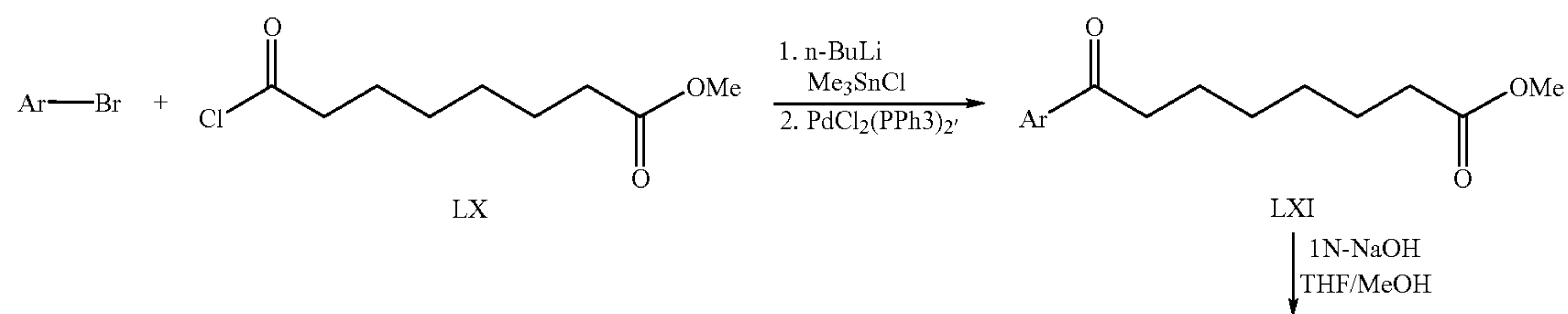
Scheme 12
