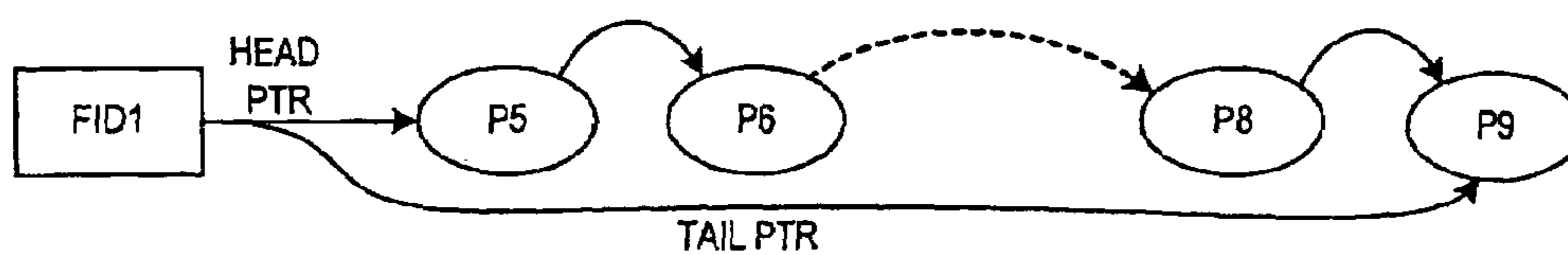
PACKET QUEUE
