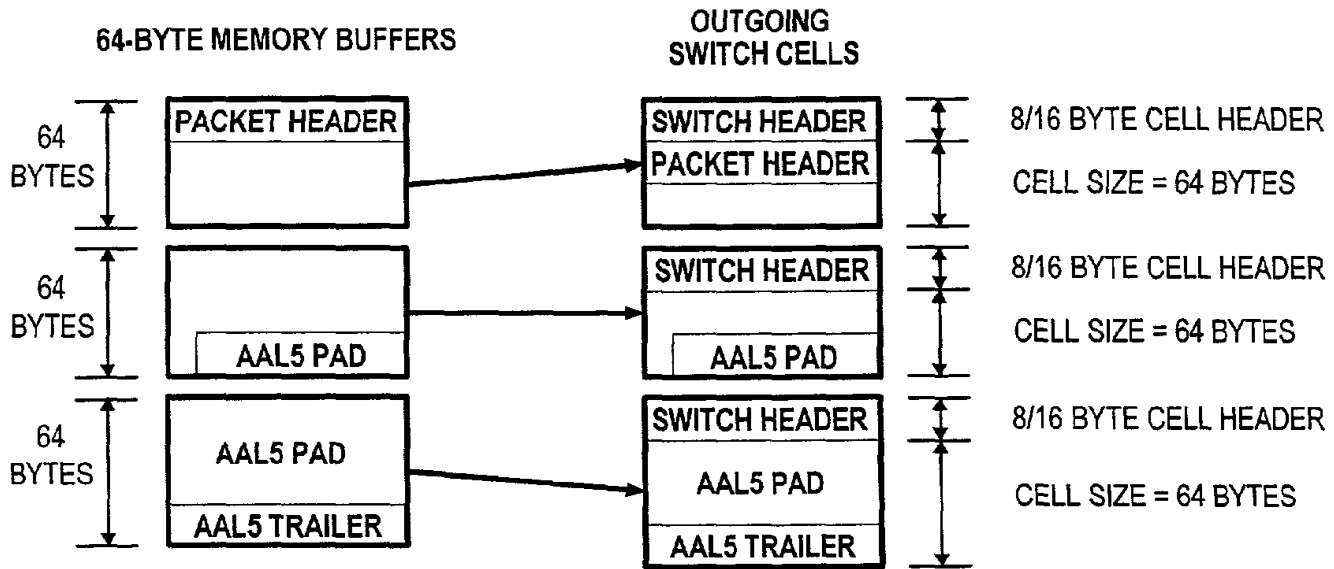
REASSEMBLY TYPE 1 (INGRESS APPLICATION TYPE 3) FIG. 60C
