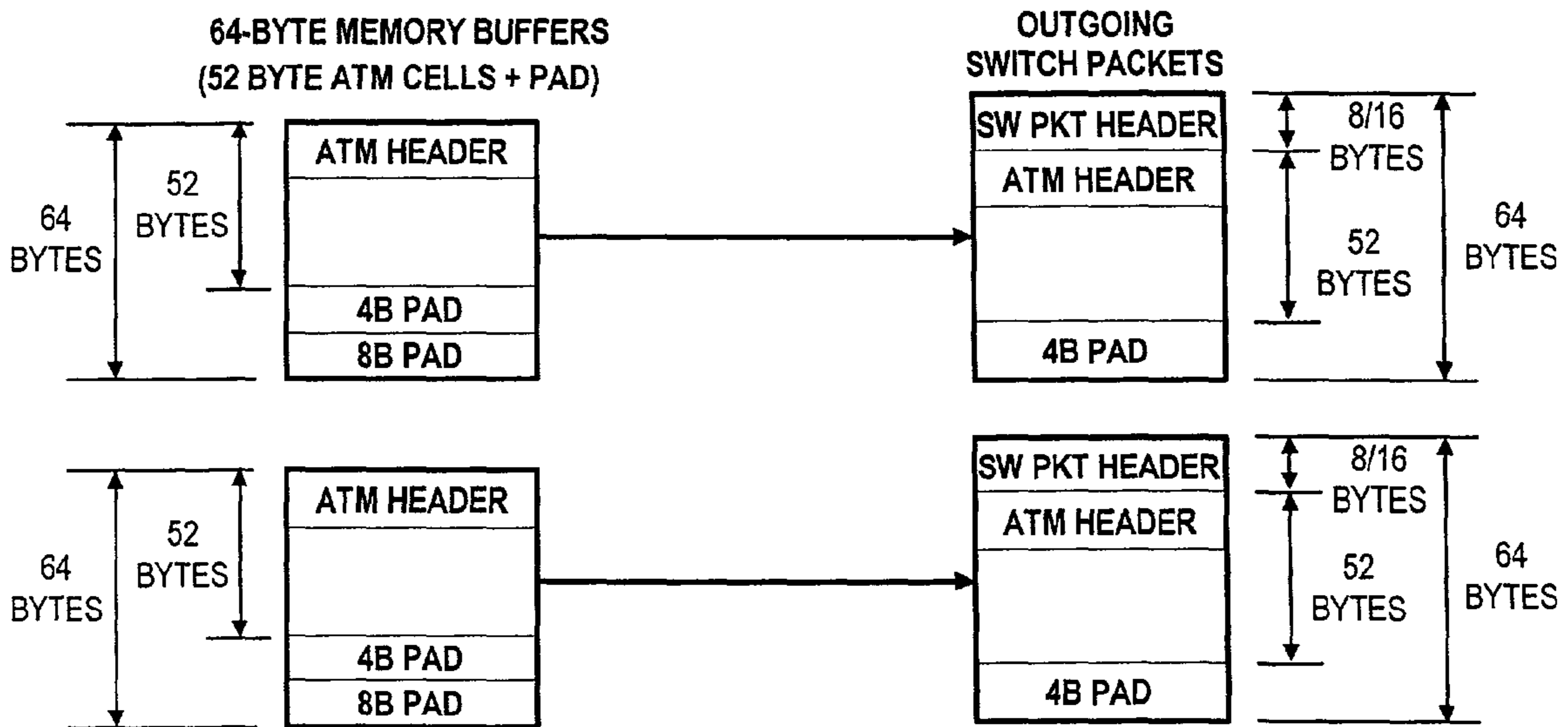
REASSEMBLY TYPE 2 (INGRESS APPLICATION TYPE 4) FIG. 60D
