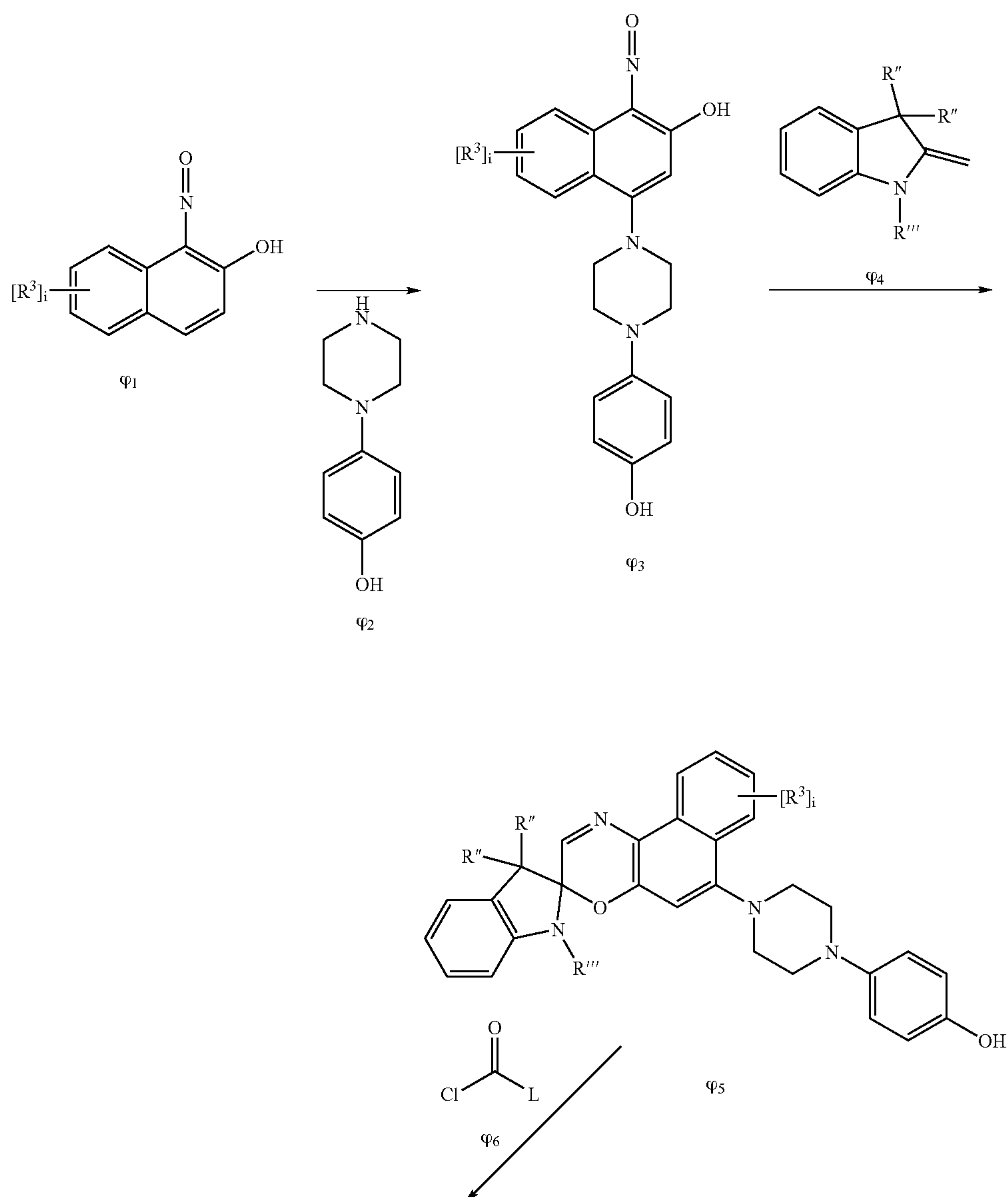
Reaction Sequence J
