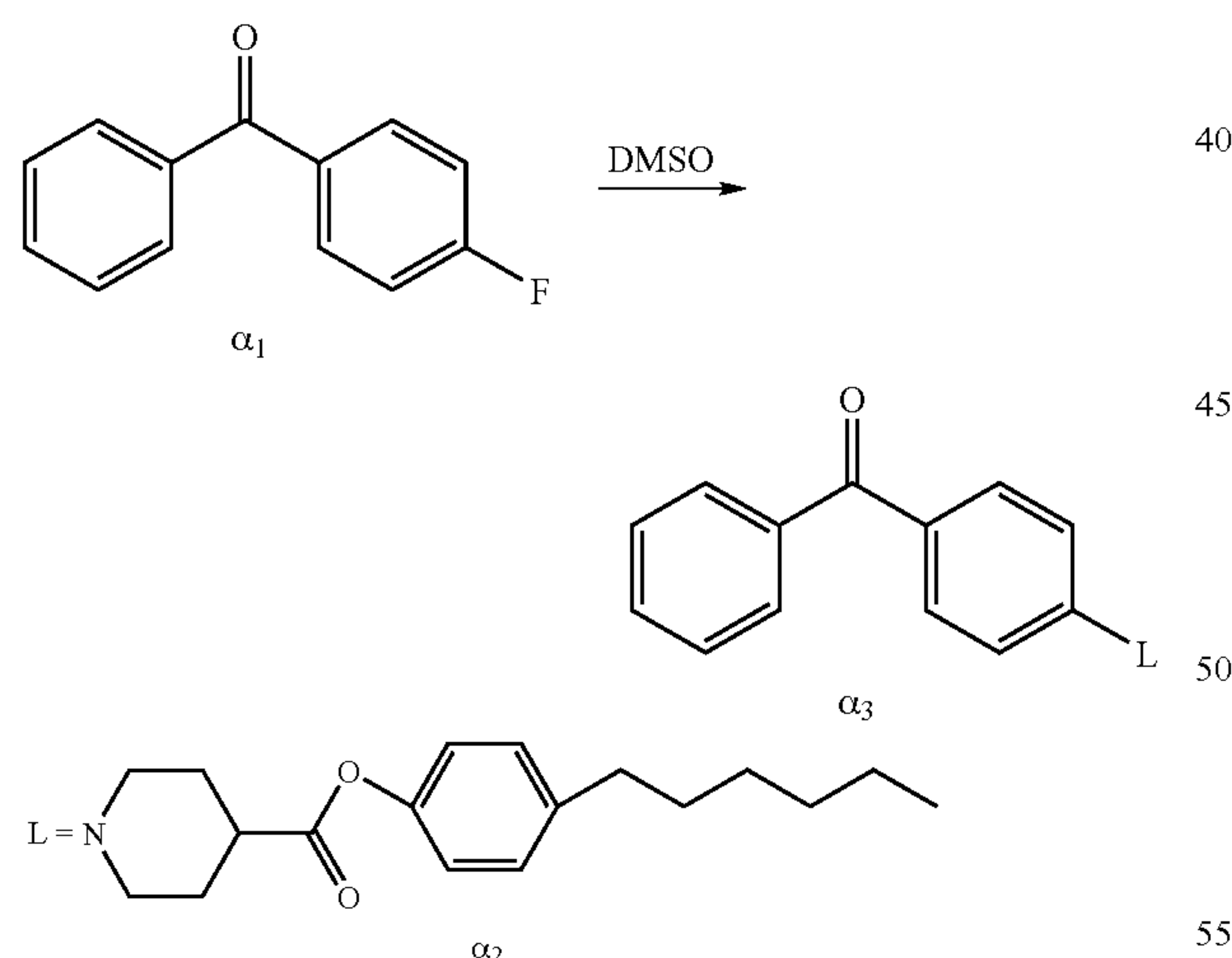
Reaction Sequence A
