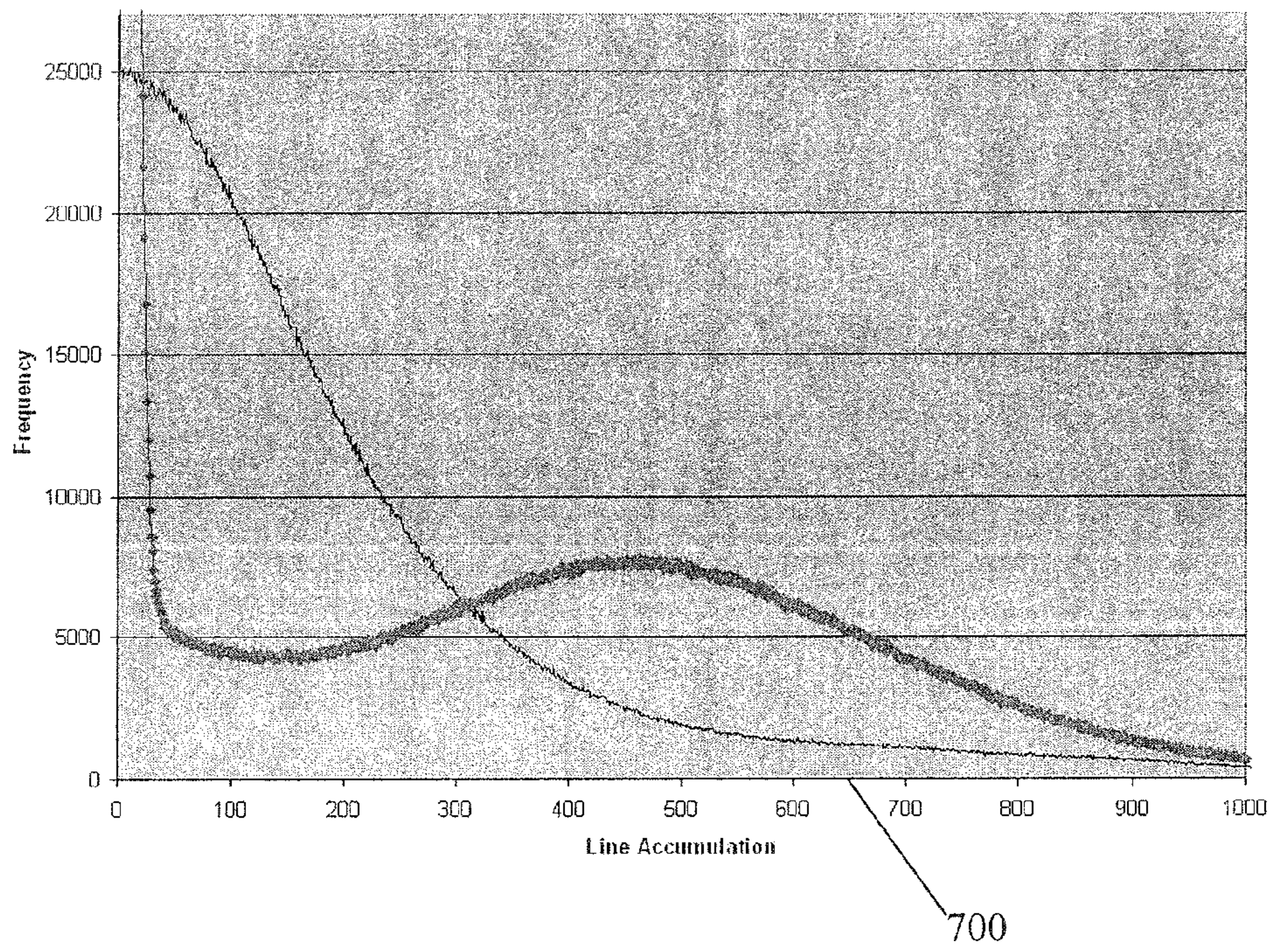
Histogram of Line Accumulation Values Over Five Minutes of Video
