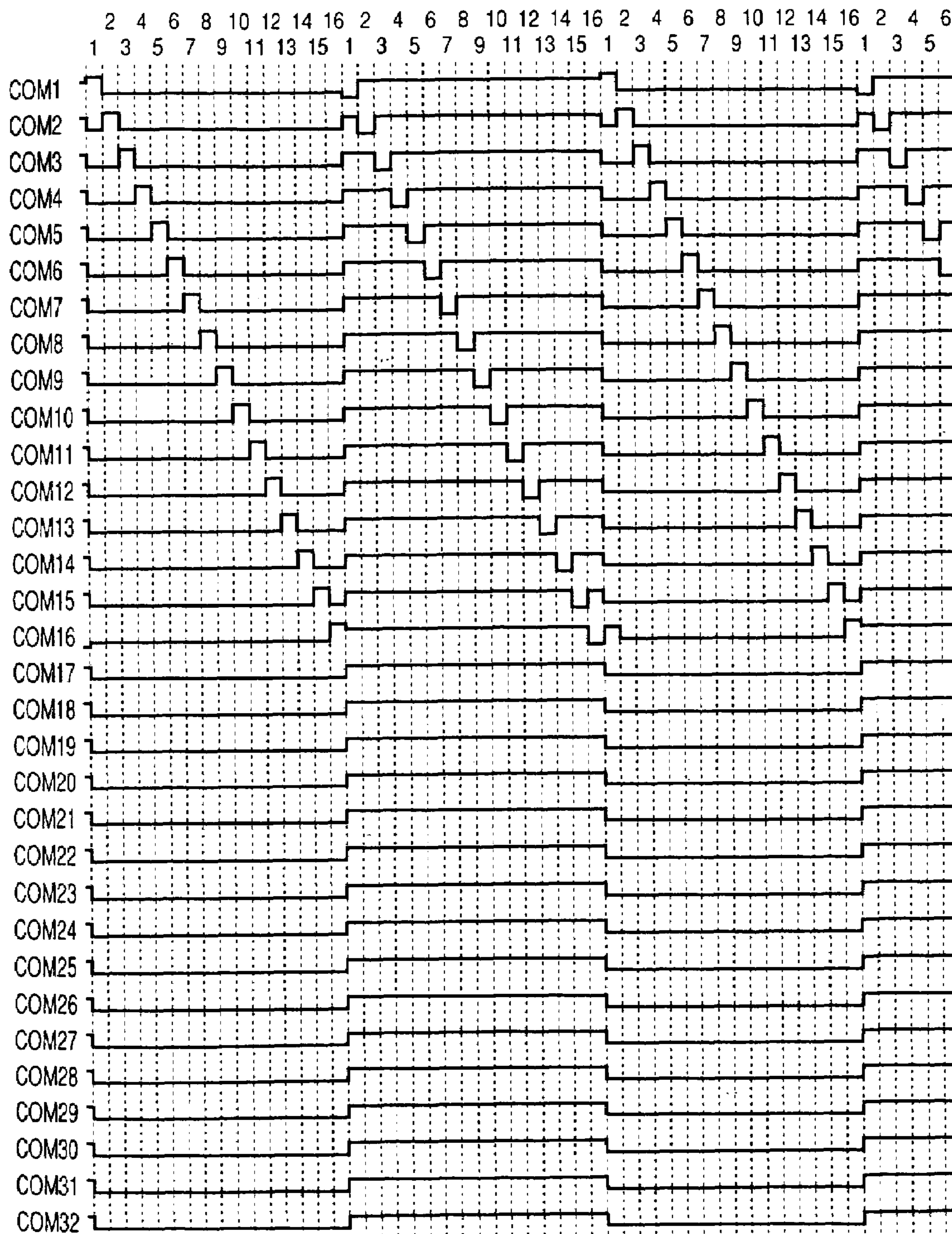
1/16 DUTY DRIVE (COM1~COM16)
