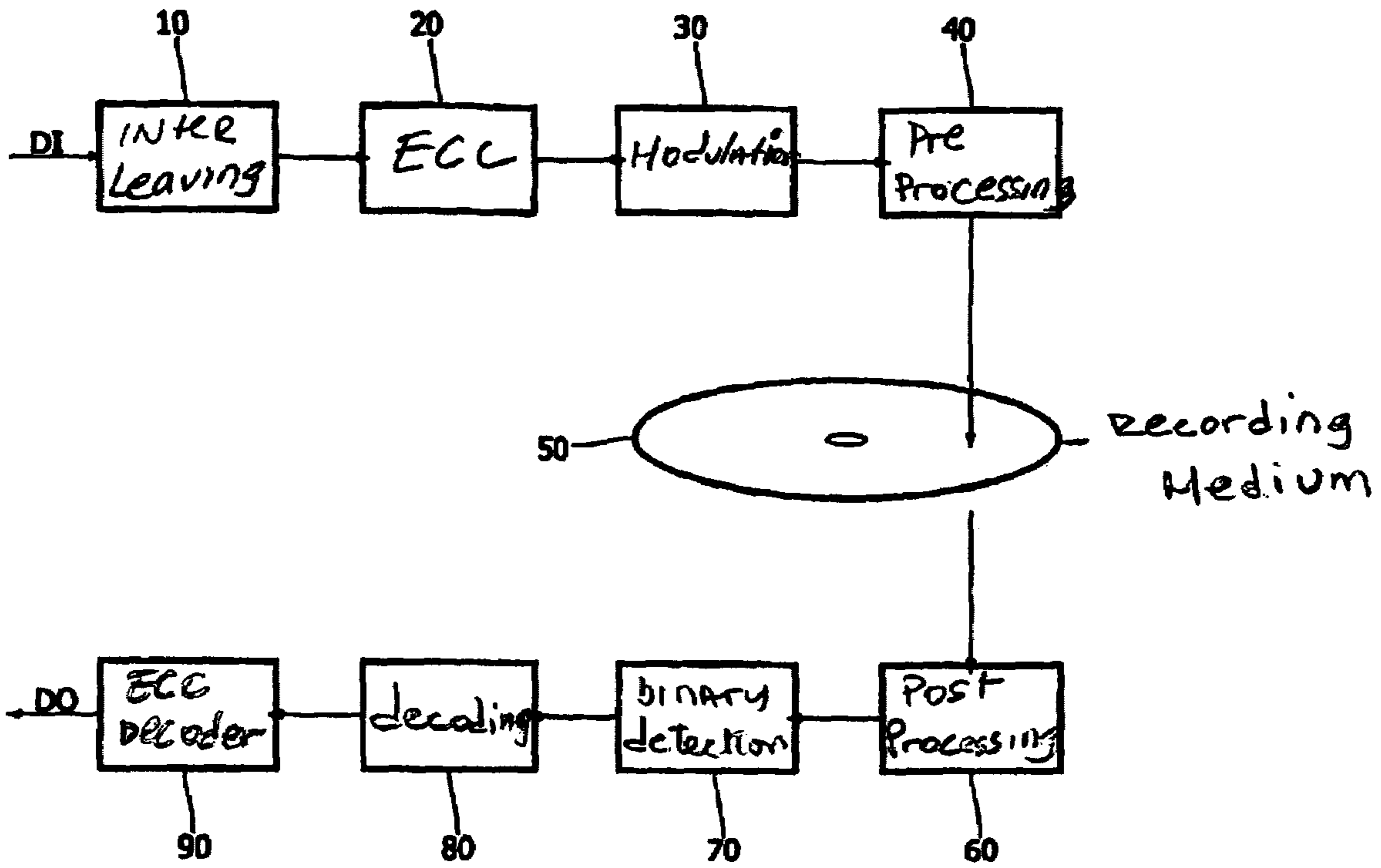
FIG.1 Prior Art
