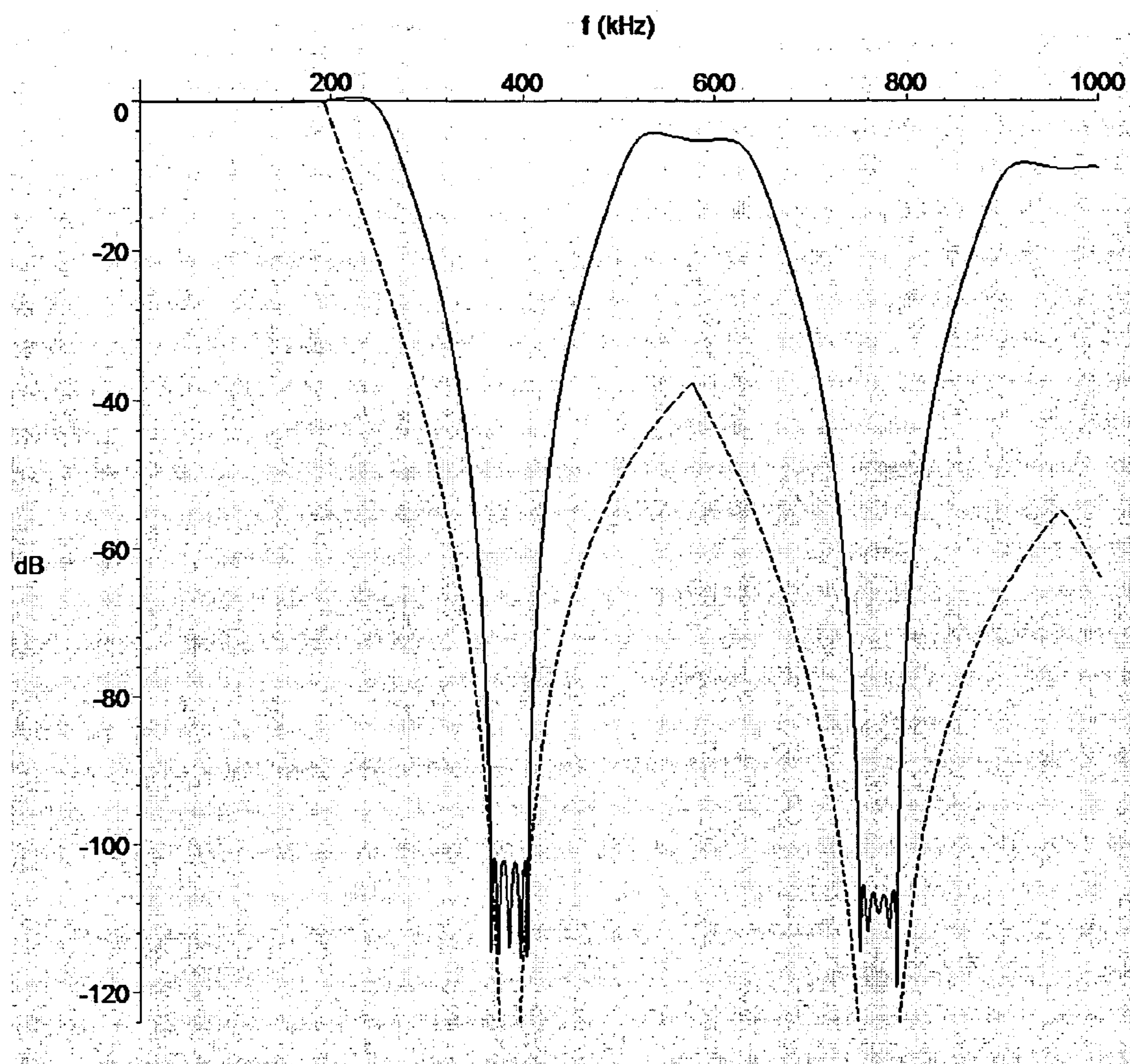
Figure 8: Alias attenuation of 80-tap FIR decimation filter and (dashed) of cascade of four combs.
