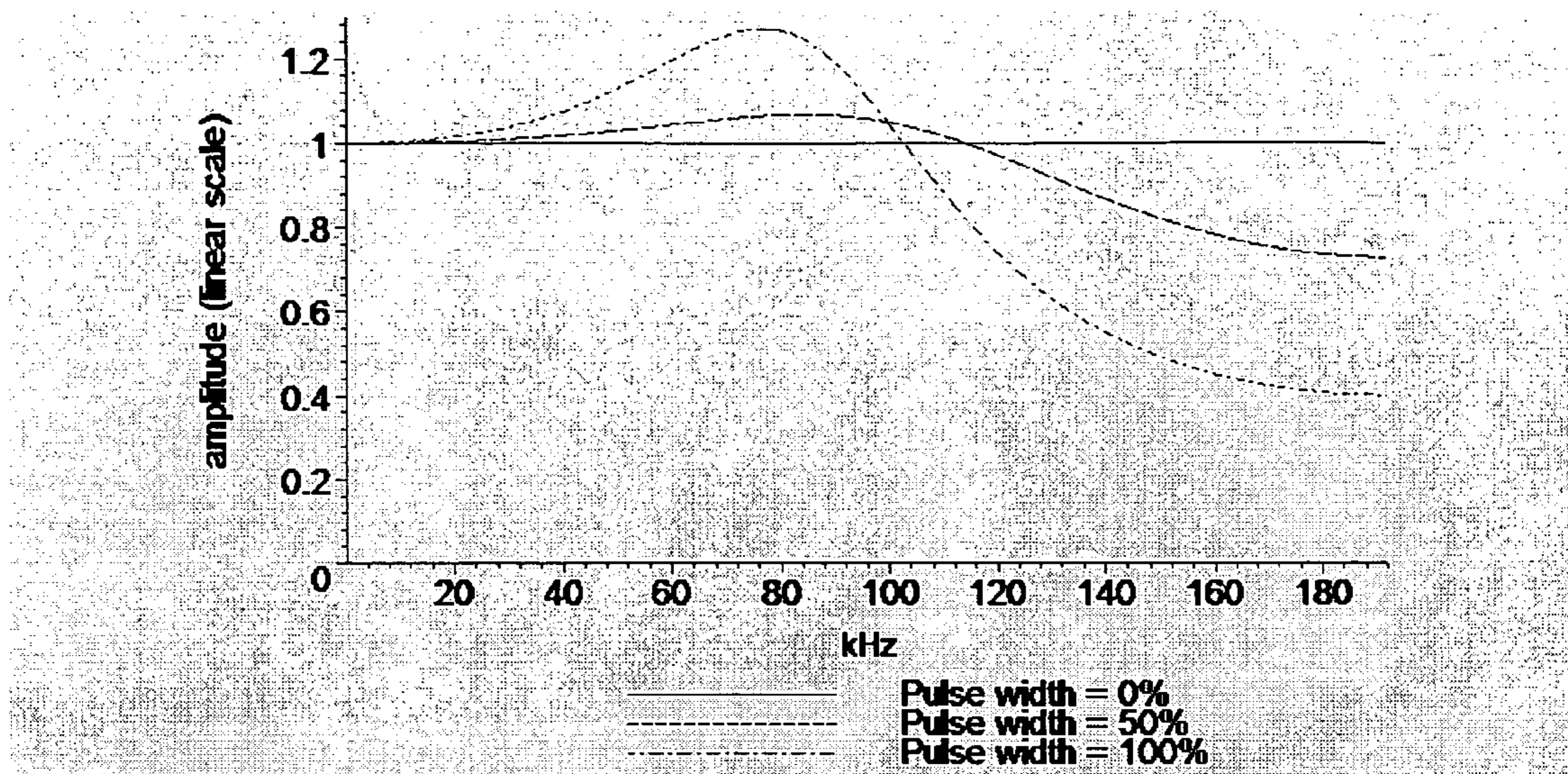
Figure 26: Small-signal amplitude response of low delay corrector unit of Figure 25, with pulse width as parameter.
