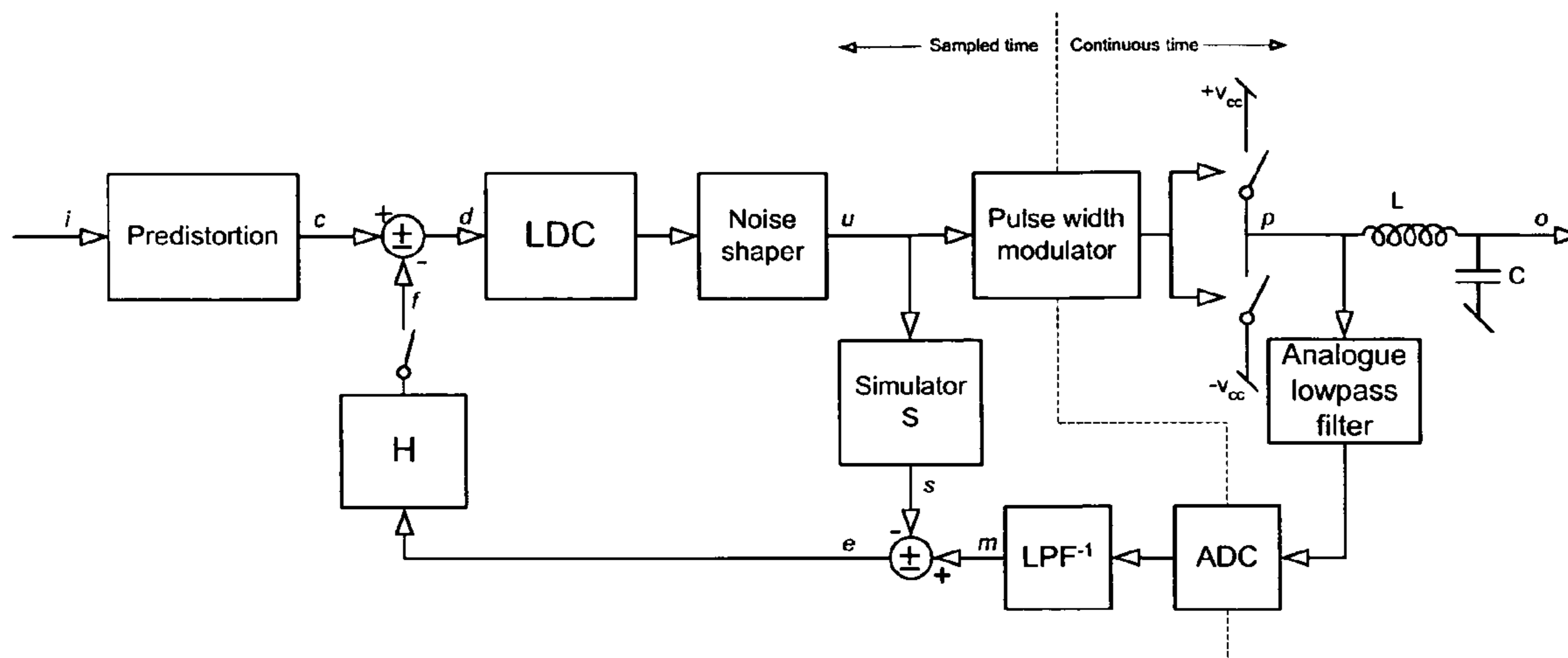
Digital pulse width modulated amplifier including feedback according to the invention.
