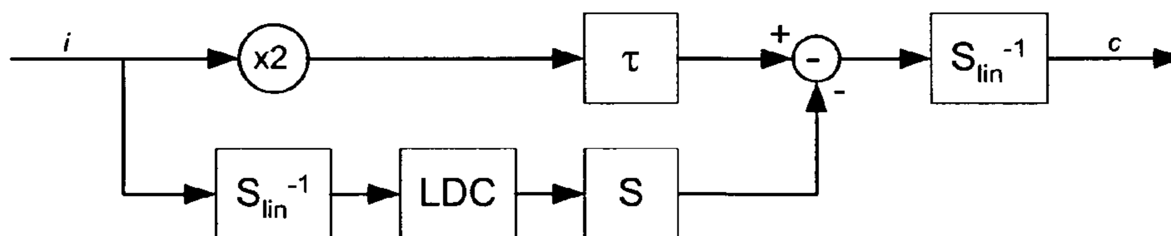
Figure 29: Gerzon predistortion unit incorporating correction for small-signal transfer function.
