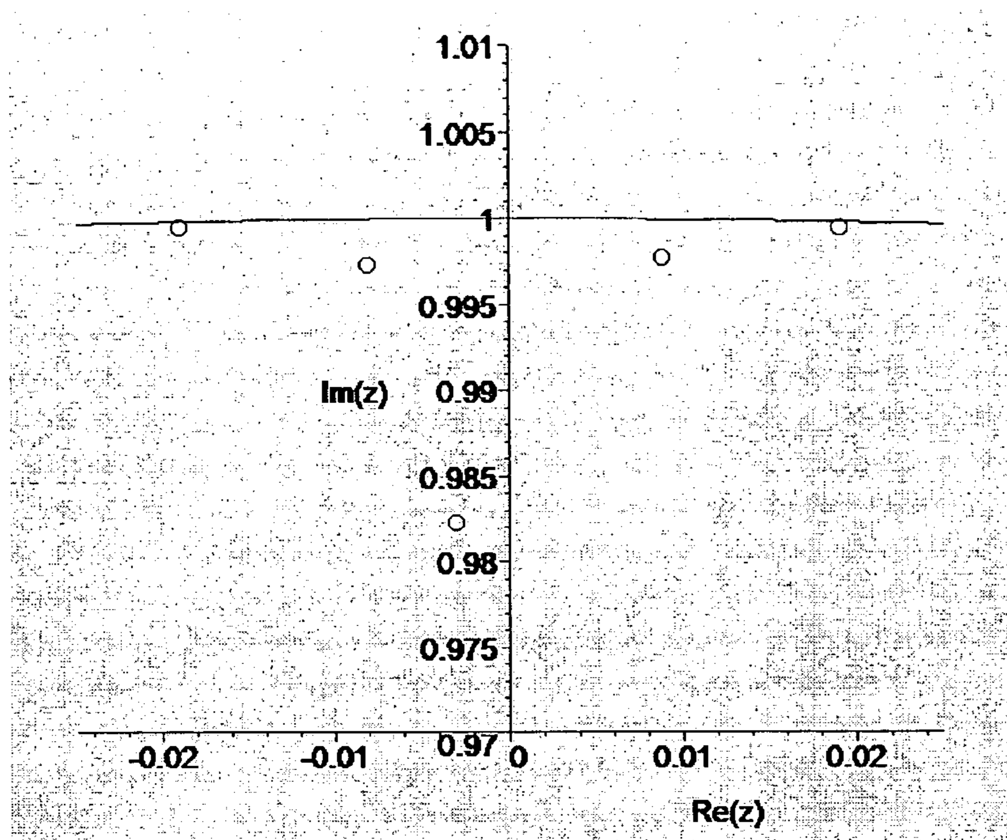
Figure 11: Close-up picture of five z -plane zeroes of 80-tap FIR decimation filter near to z = 0 + 1j
