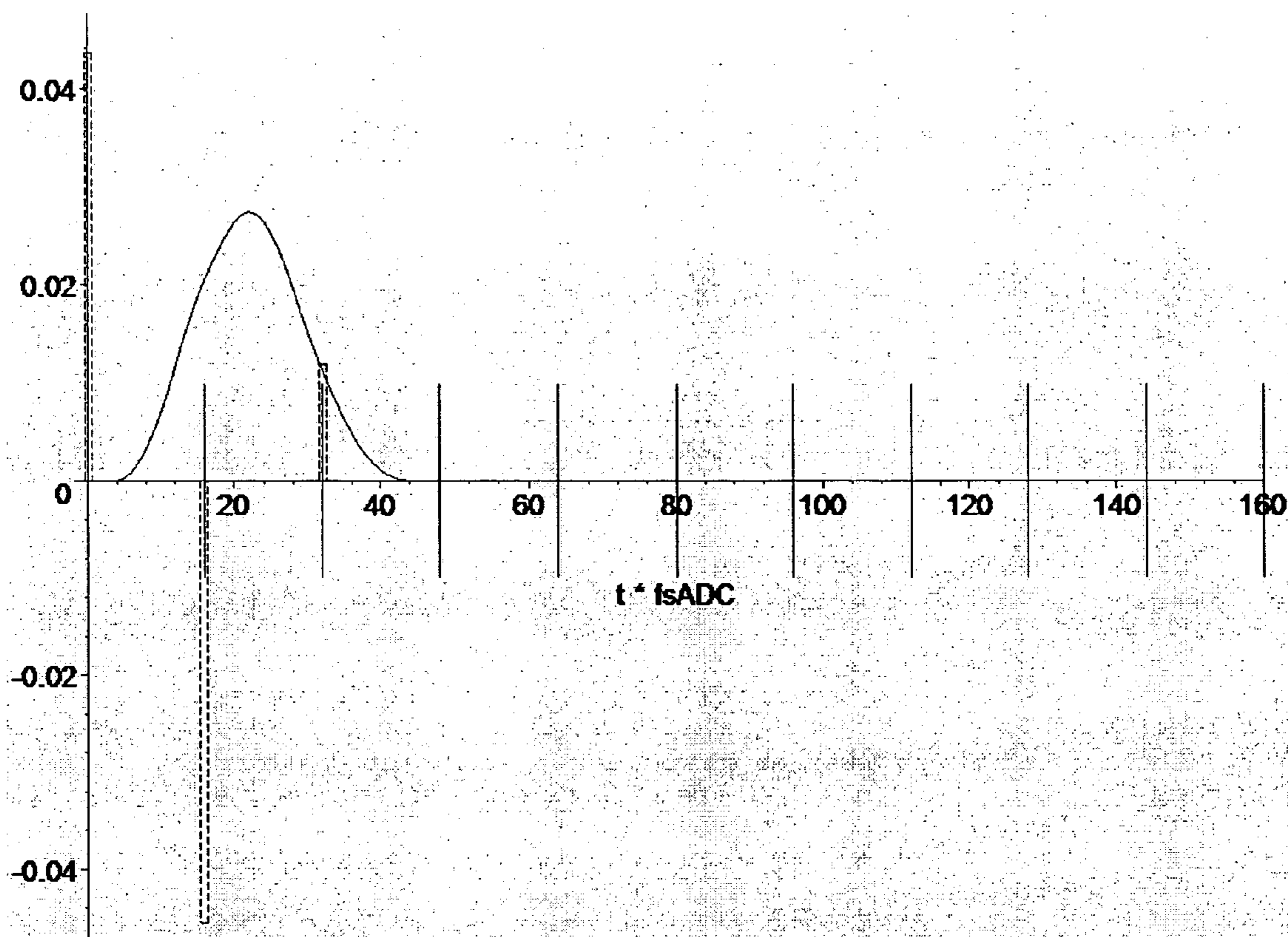
Figure 15: Sharpening of analog filter response using 3-point deconvolution filter.
