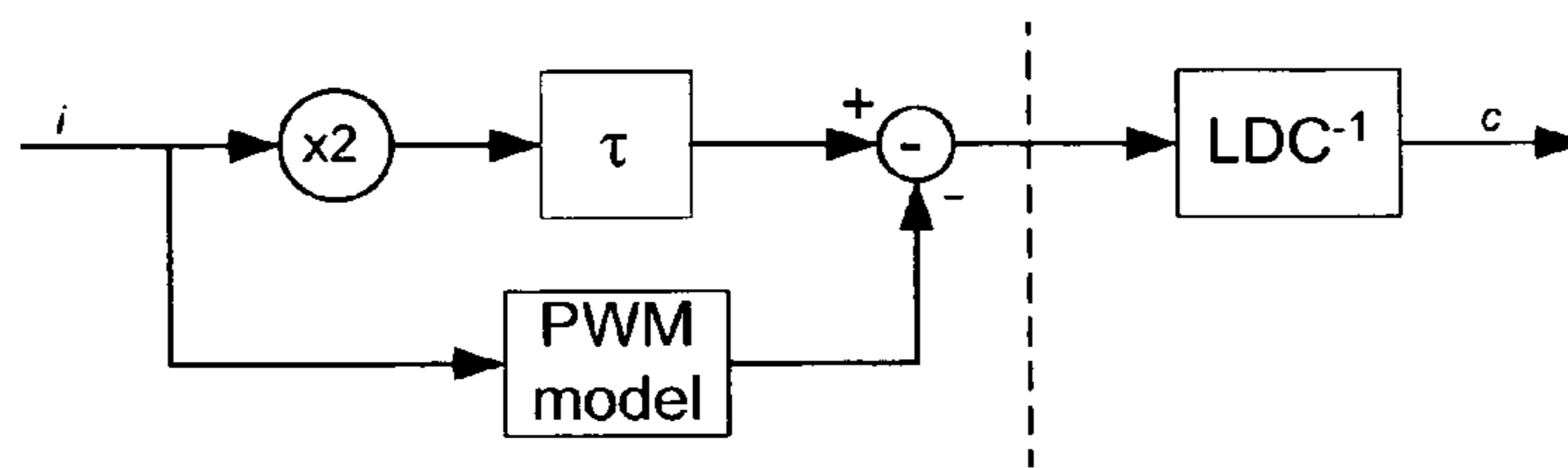
Figure 31: Gerzon predistortion unit adapted to compensate pulse width modulator, followed by compensator for LDC.
