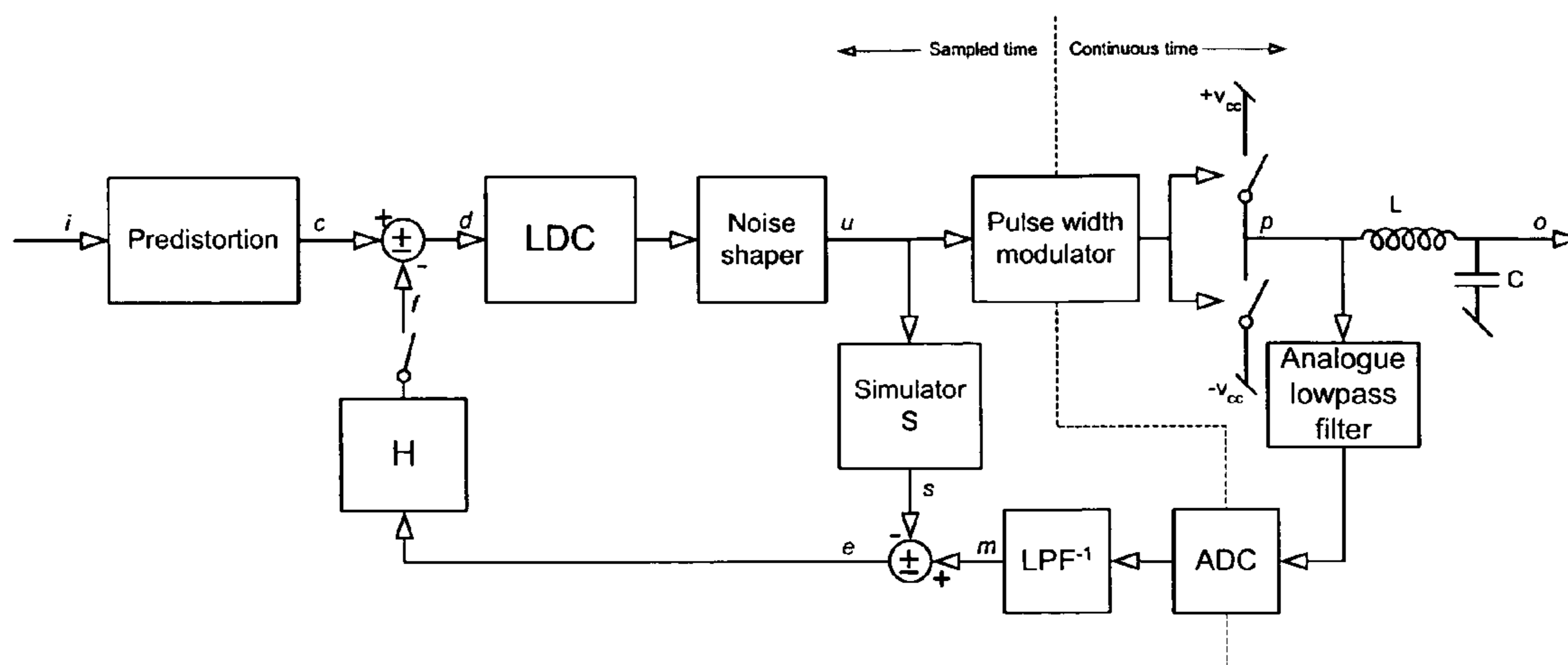
Figure 3: Digital pulse width modulated amplifier including feedback according to the invention.
