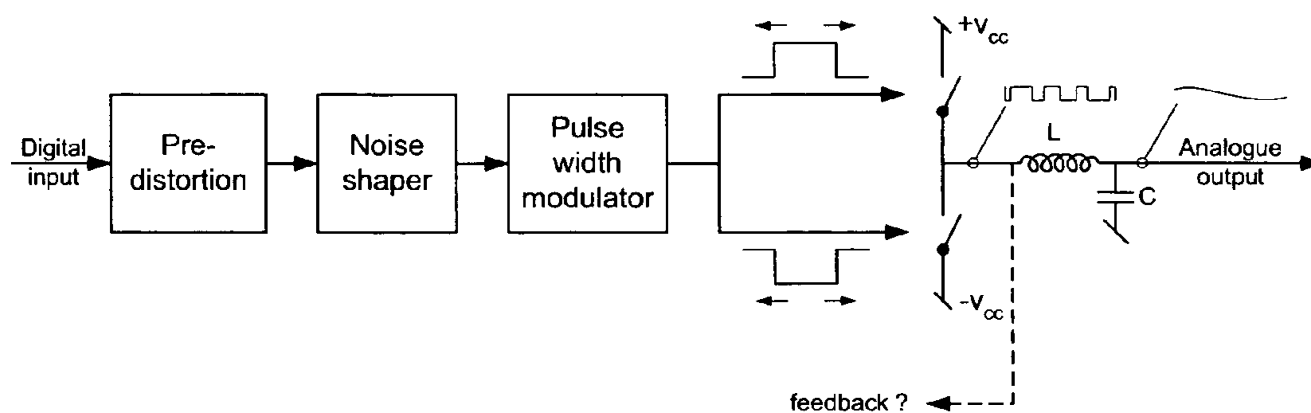
Figure 1: Digital pulse width modulated amplifier (prior art).
