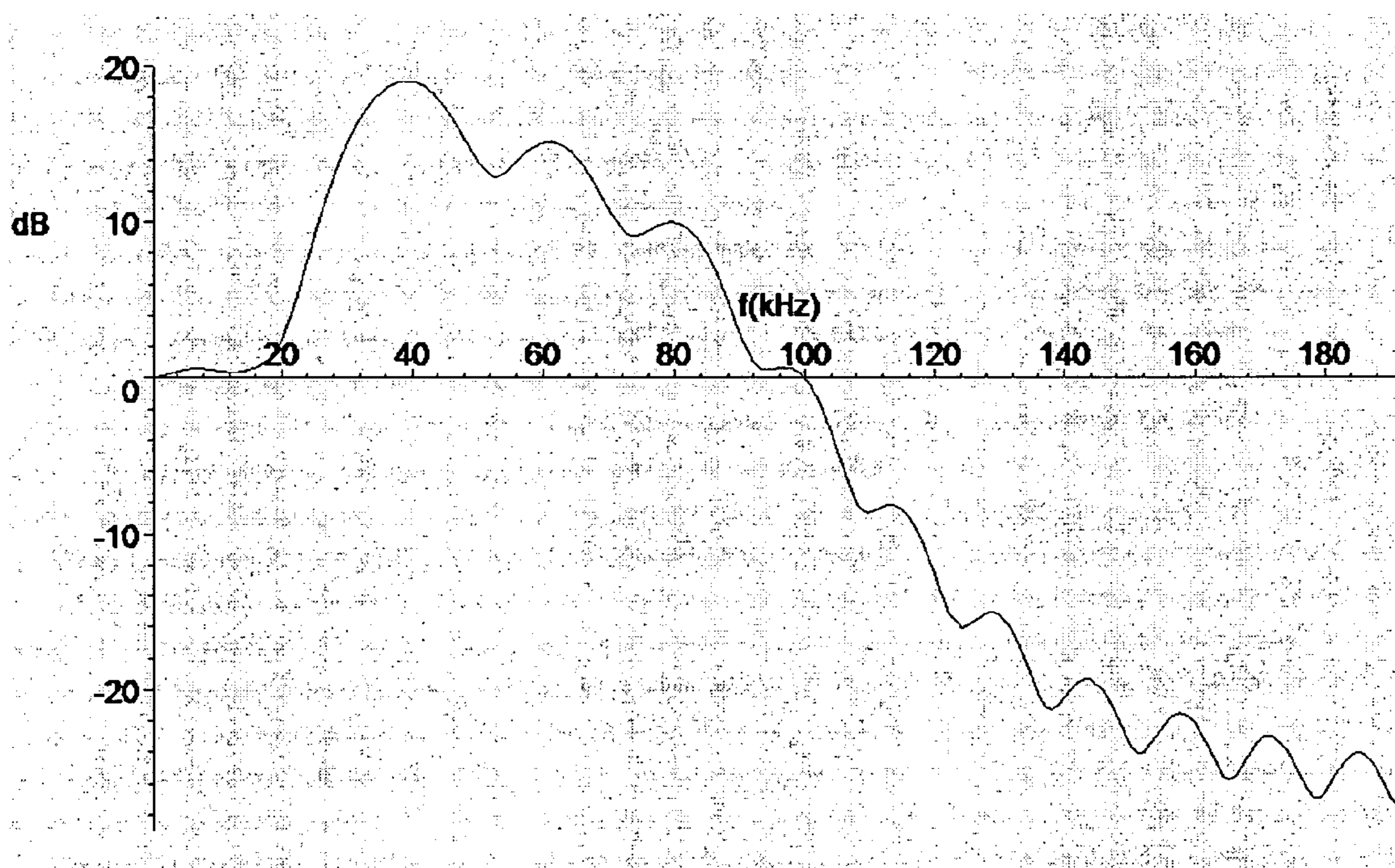
Figure 23: Magnitude of gain of feedback loop with simulator disabled.
