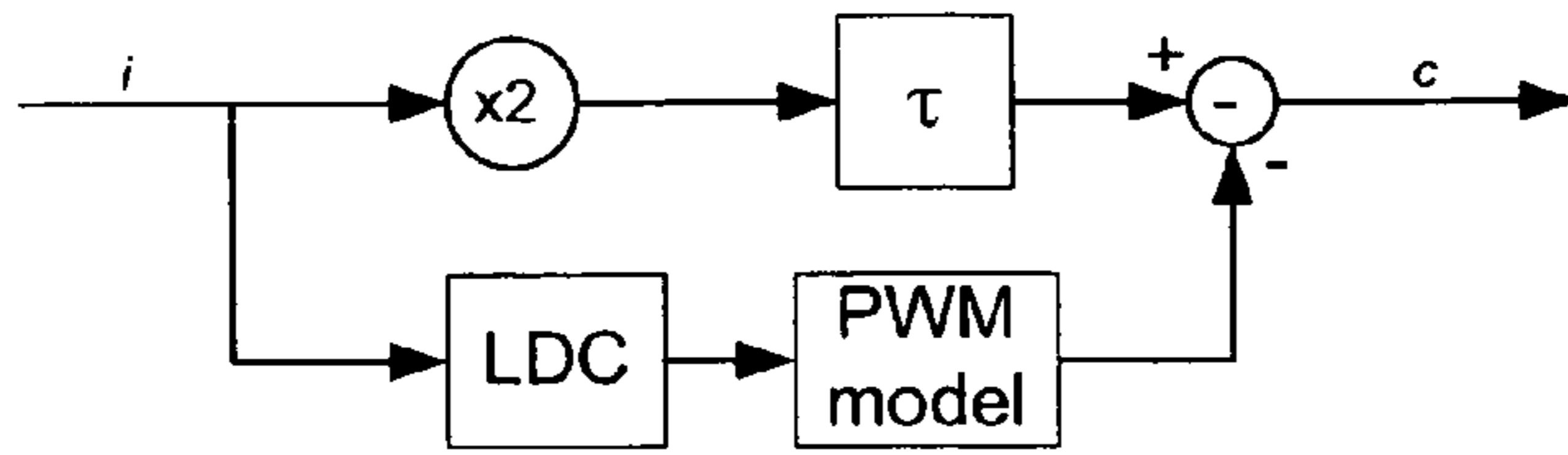
Figure 30: Gerzon predistortion unit adapted to compensate LDC and pulse width modulator.
