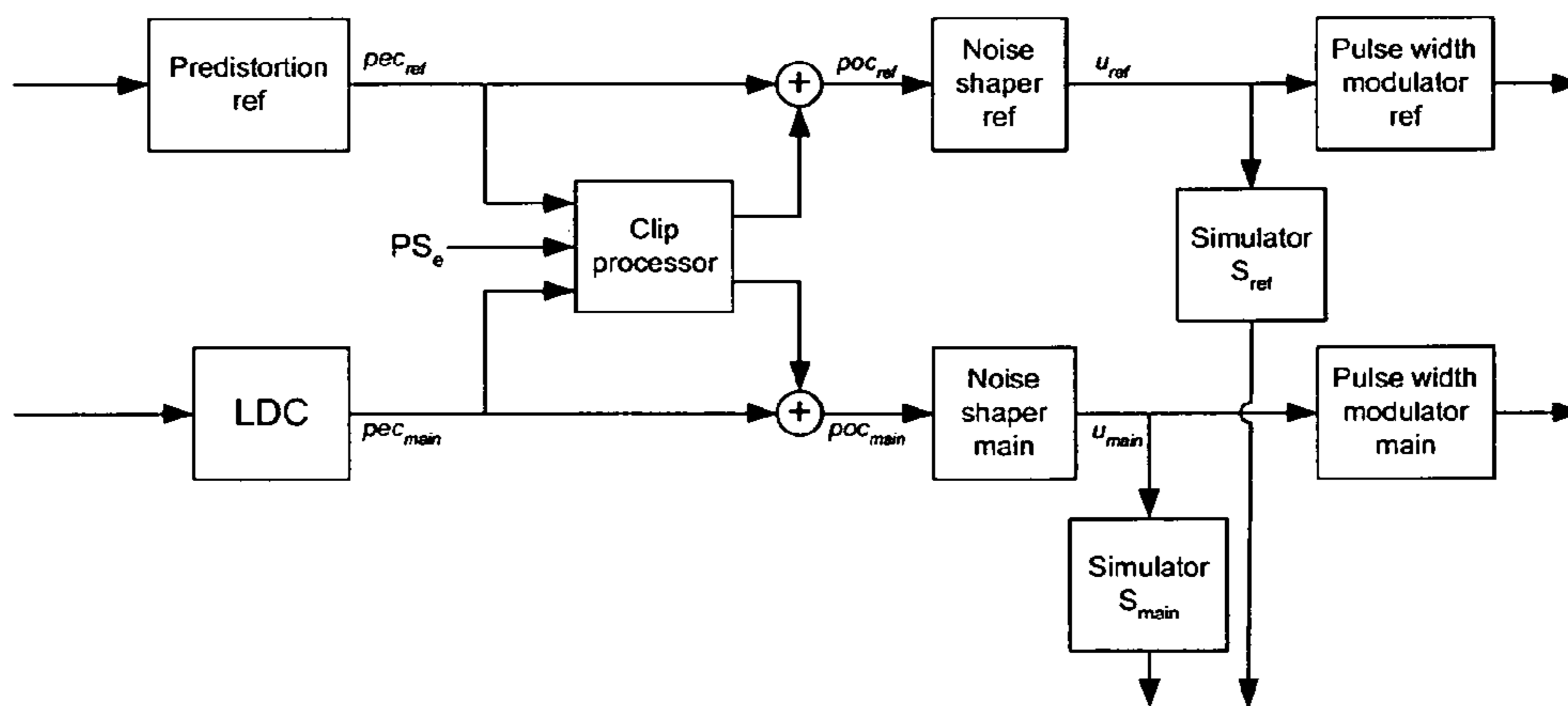
Figure 36: Joint clipping of the main and reference paths.
