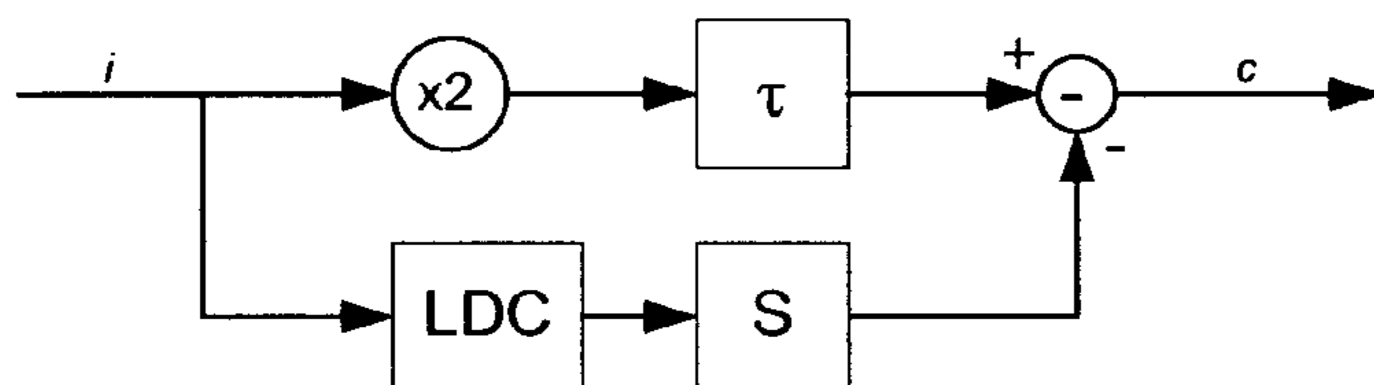
Figure 28: Gerzon predistortion unit adapted to compensate LDC and S.
