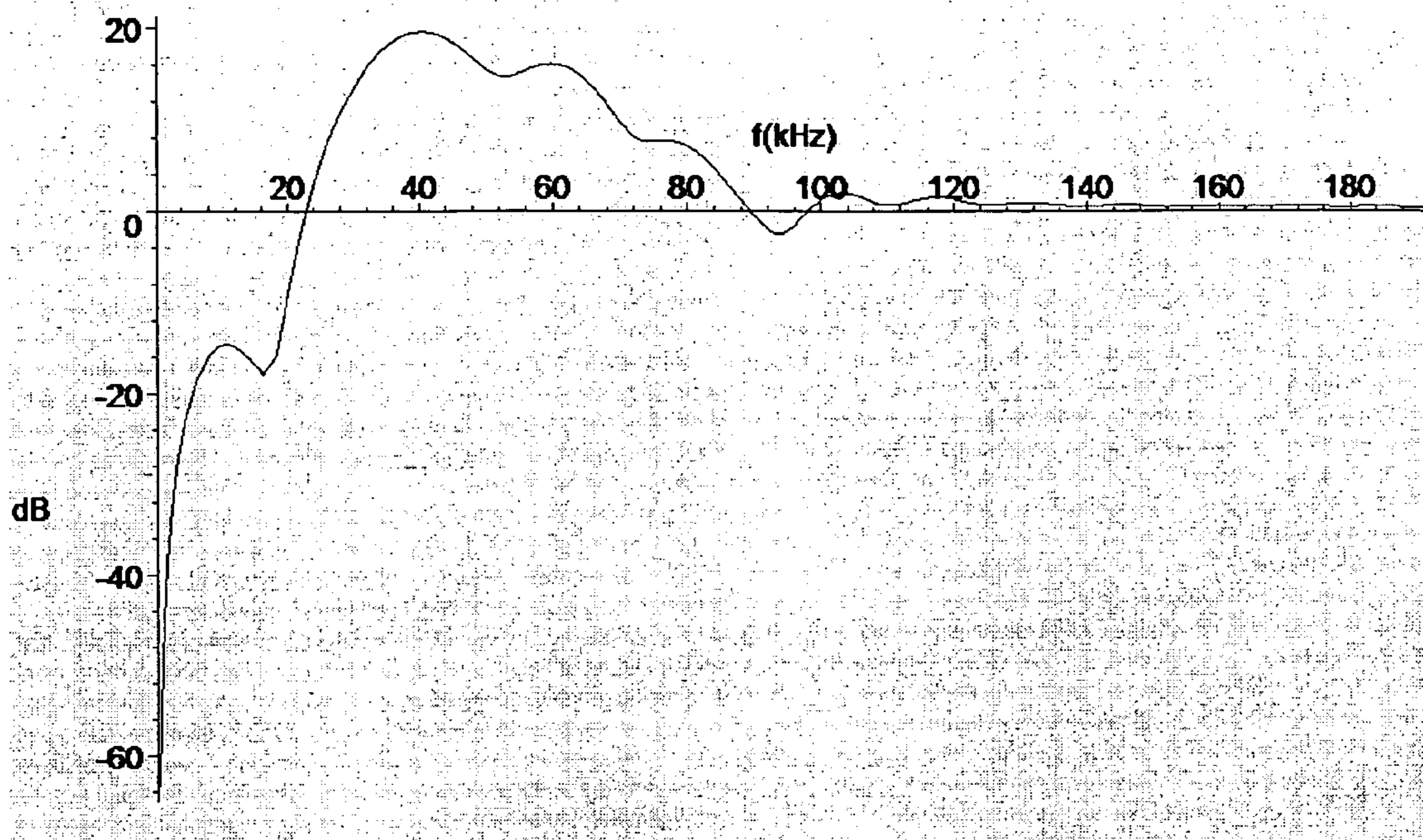
Figure 24: Magnitude of noise transfer function (NTF) of feedback loop.
