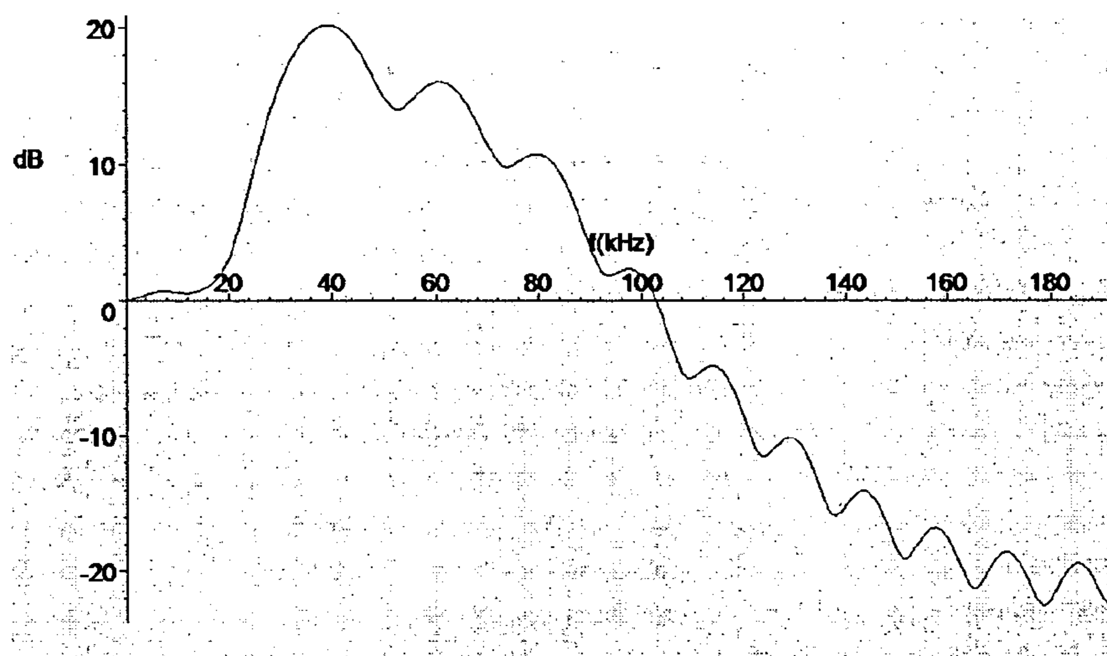
Figure 22: Amplitude response of the feedback filter H of Figure 21.
