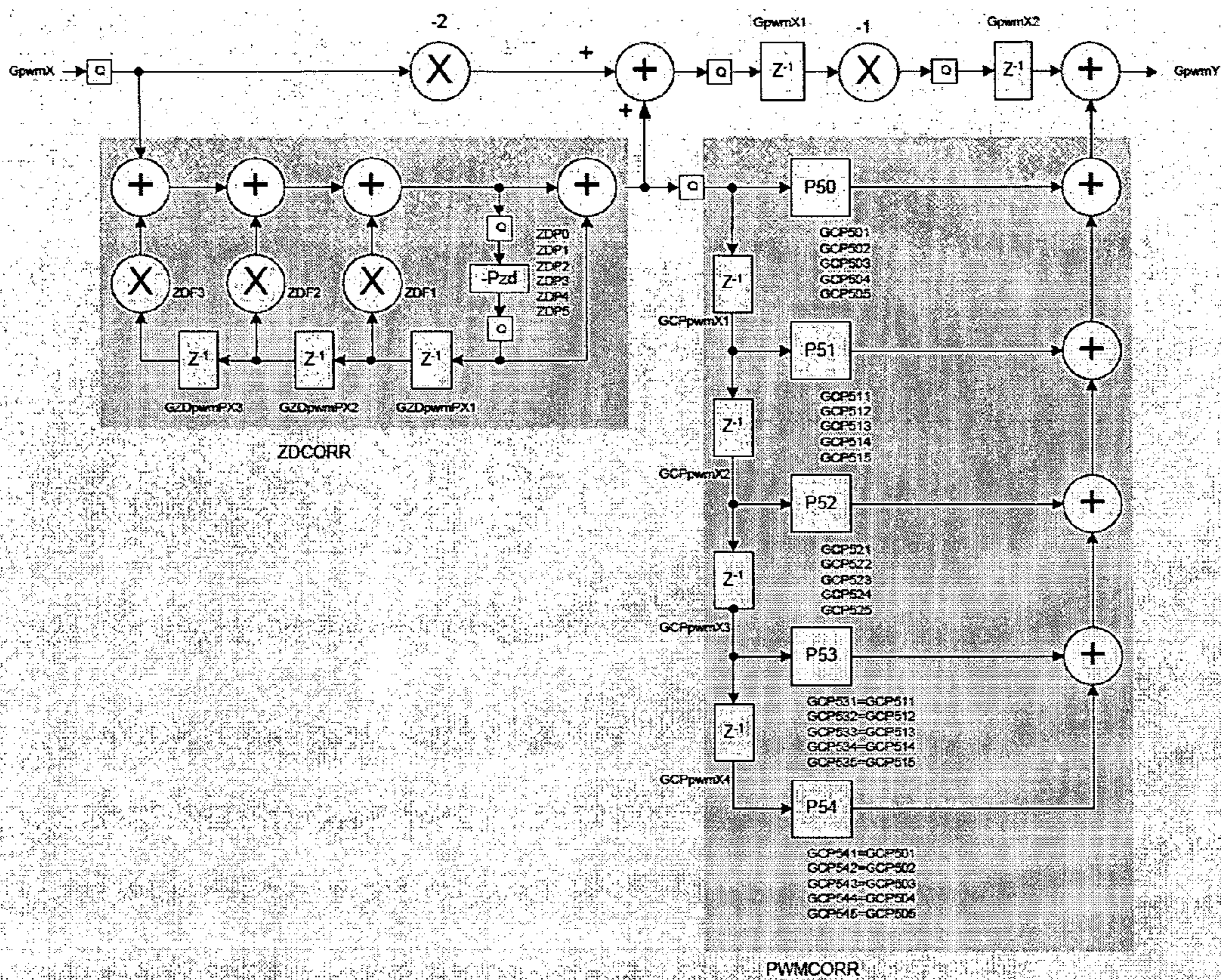
Figure 33: Detail of a predistortion unit using the principle of Figure 30.
