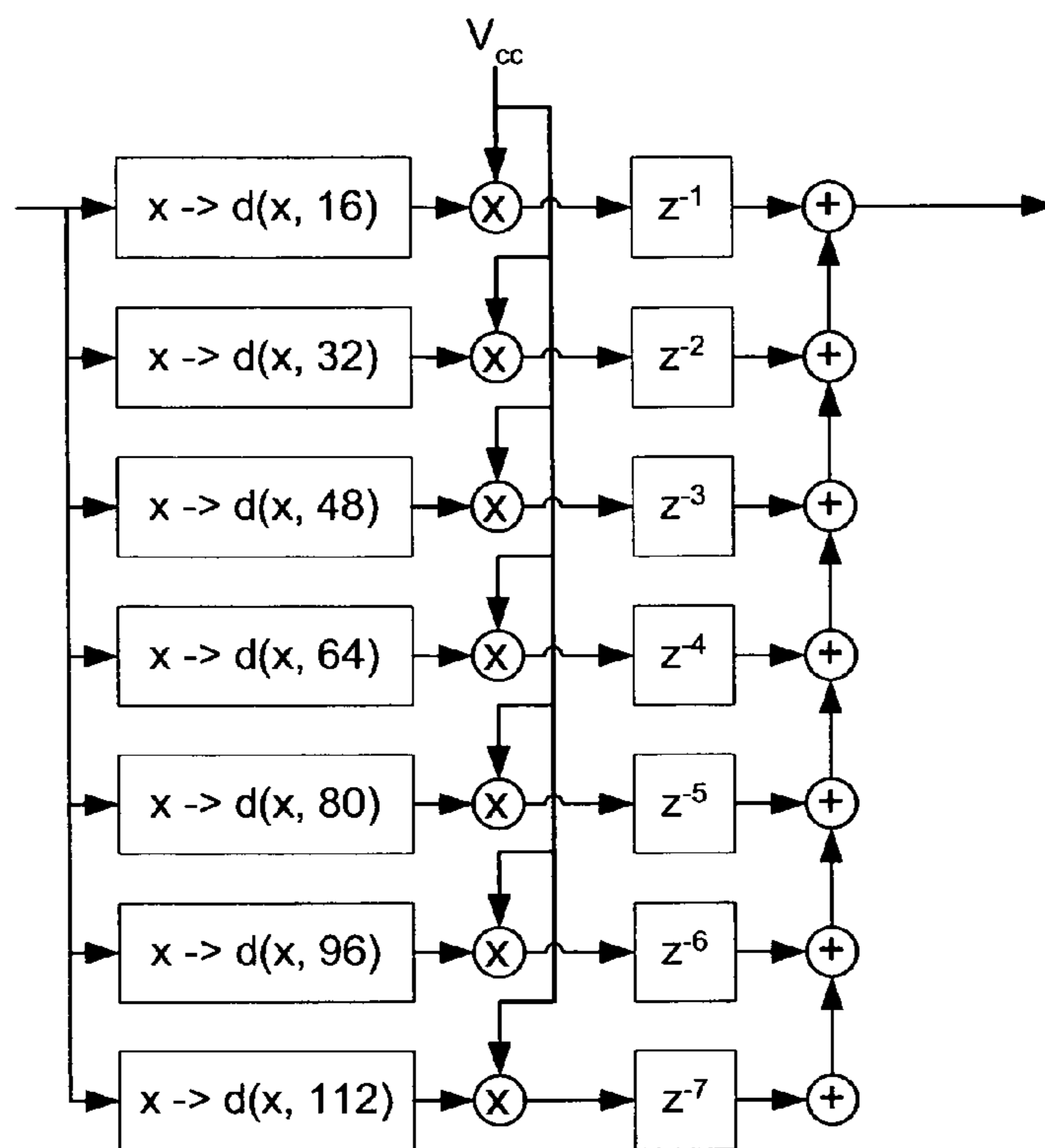
Figure 17: Conceptual model of measurement path.
