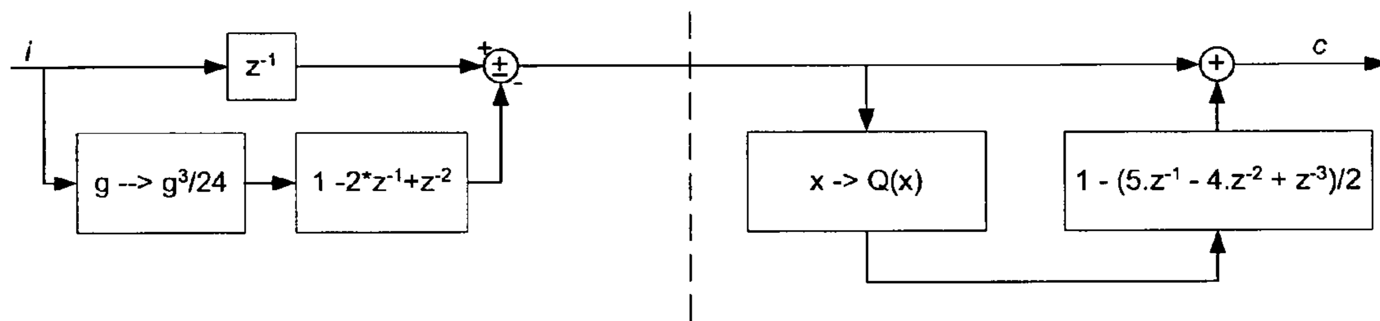
Figure 32: Detail of a predistortion unit using the principle of Figure 31.
