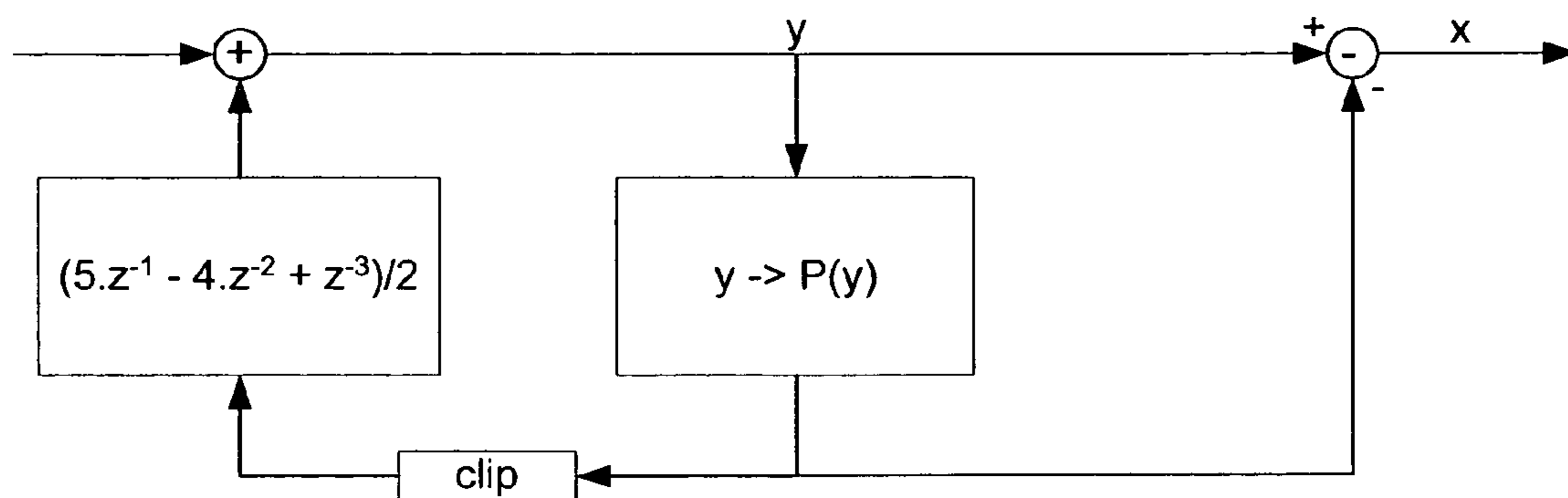
Figure 25: Low delay corrector unit LDC.
