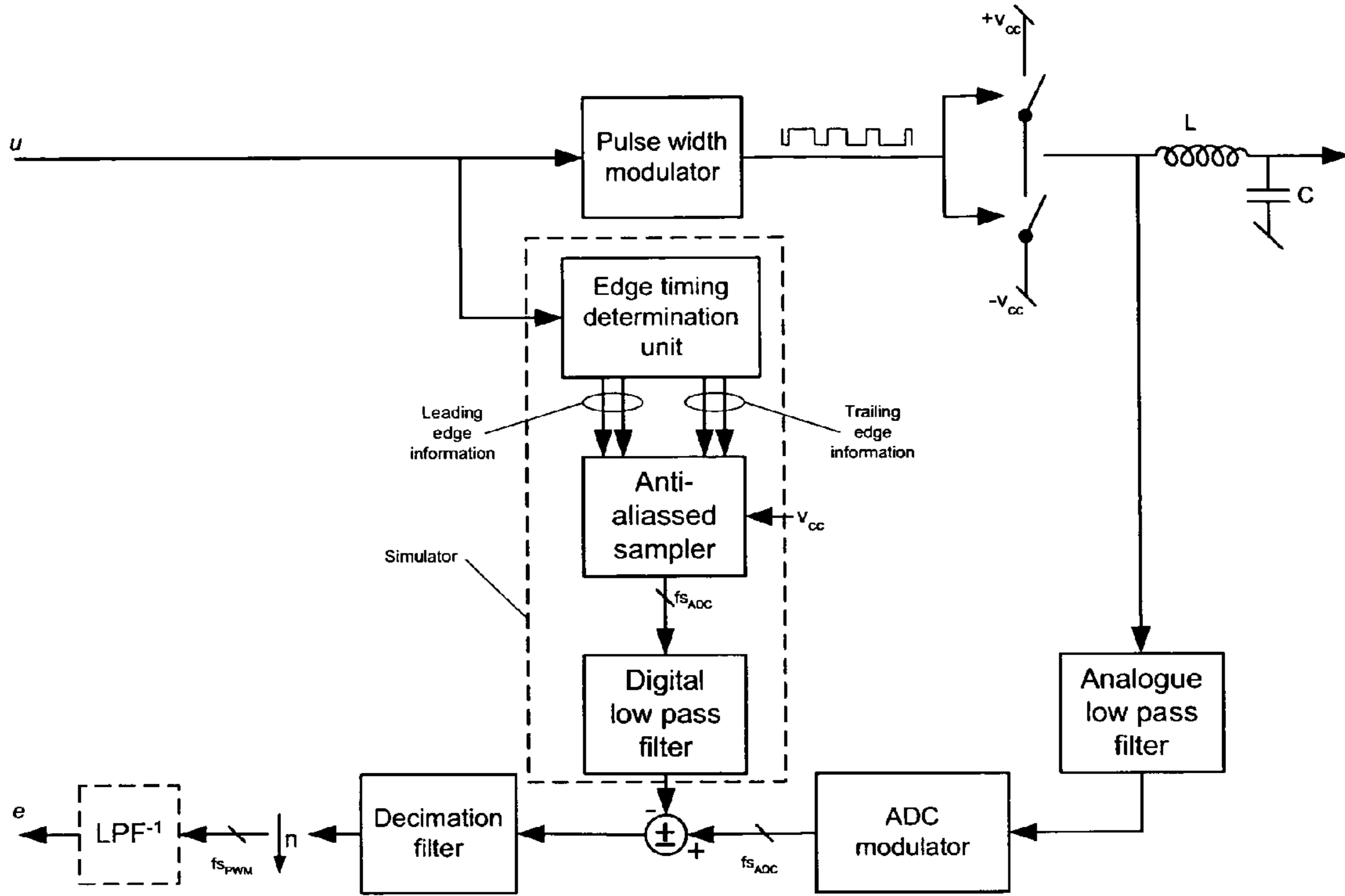
Figure 19: Amplifier detail incorporating alternative simulator.
