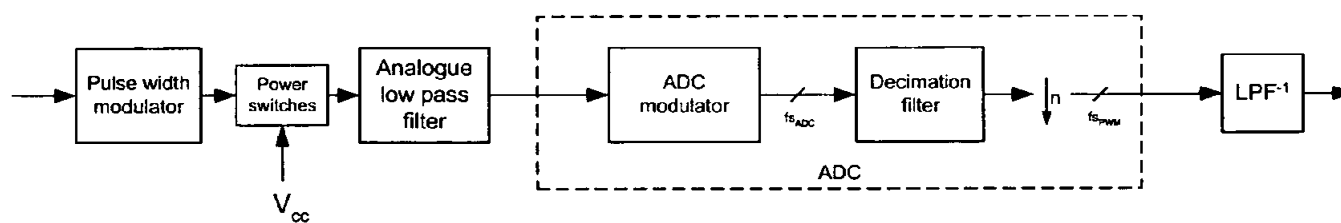
Figure 12: Measurement path.
