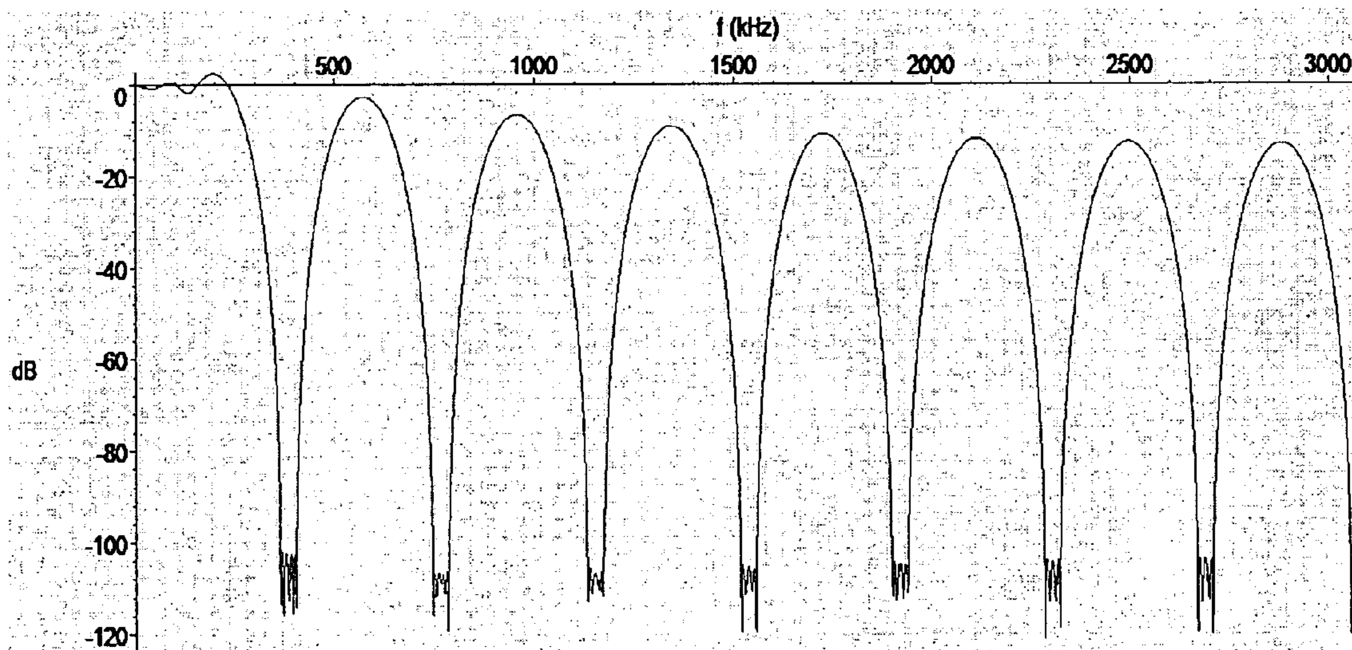
Figure 6: Amplitude response of 80-tap FIR decimation filter.
