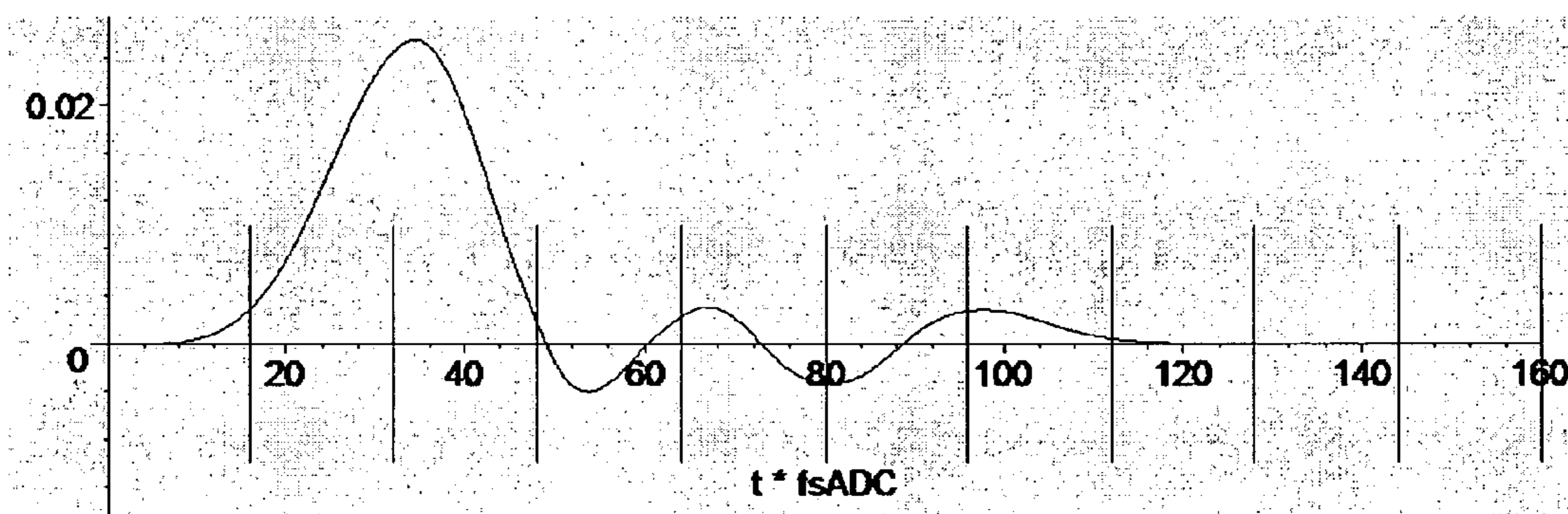
Figure 16: Response of 80-tap FIR decimation filter to sharpened analog filter response
