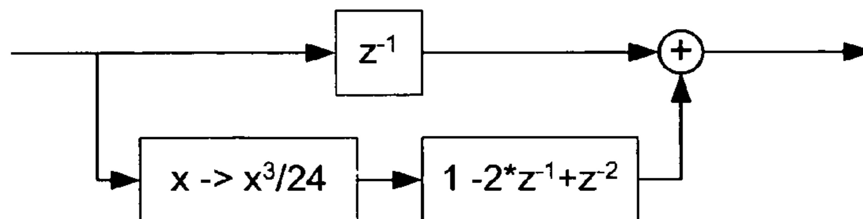
Figure 13: Low-frequency model of PWM nonlinearity
