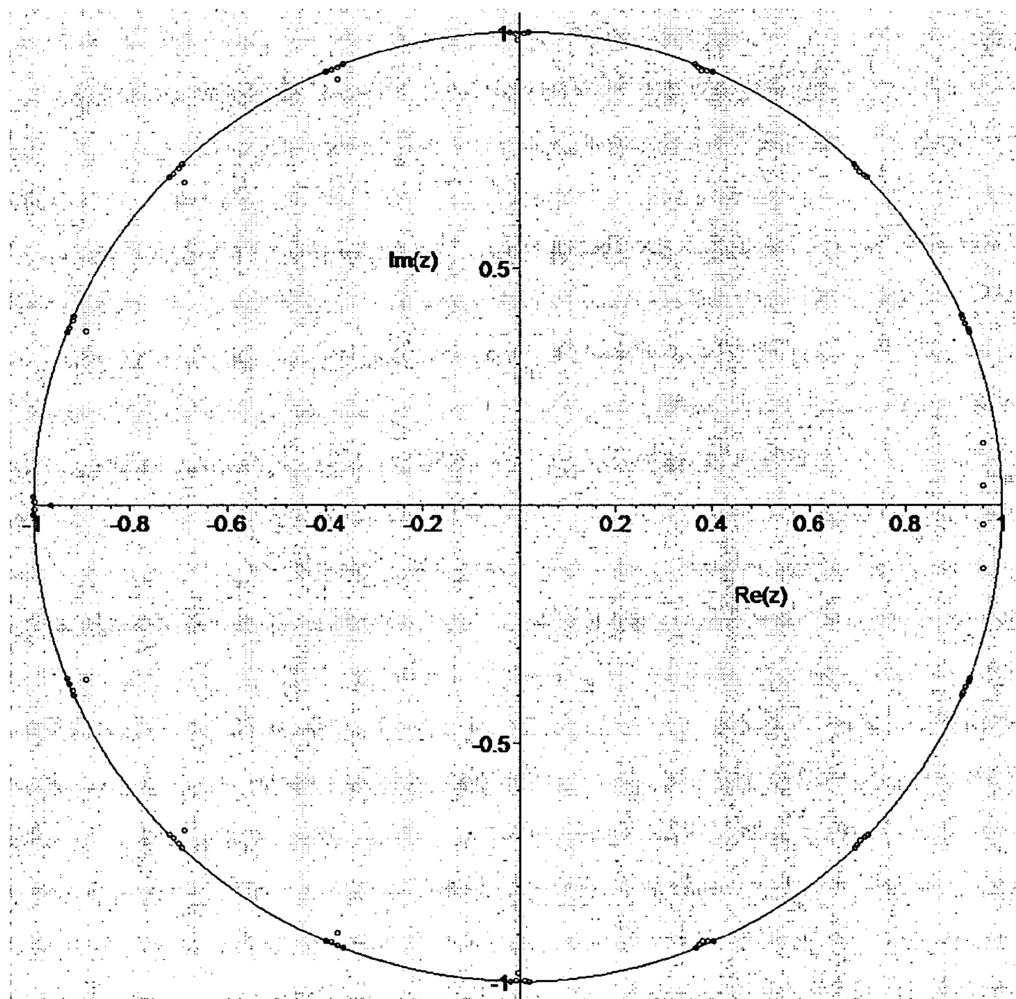
Figure 10: z -plane zeroes of 80-tap FIR decimation filter.
