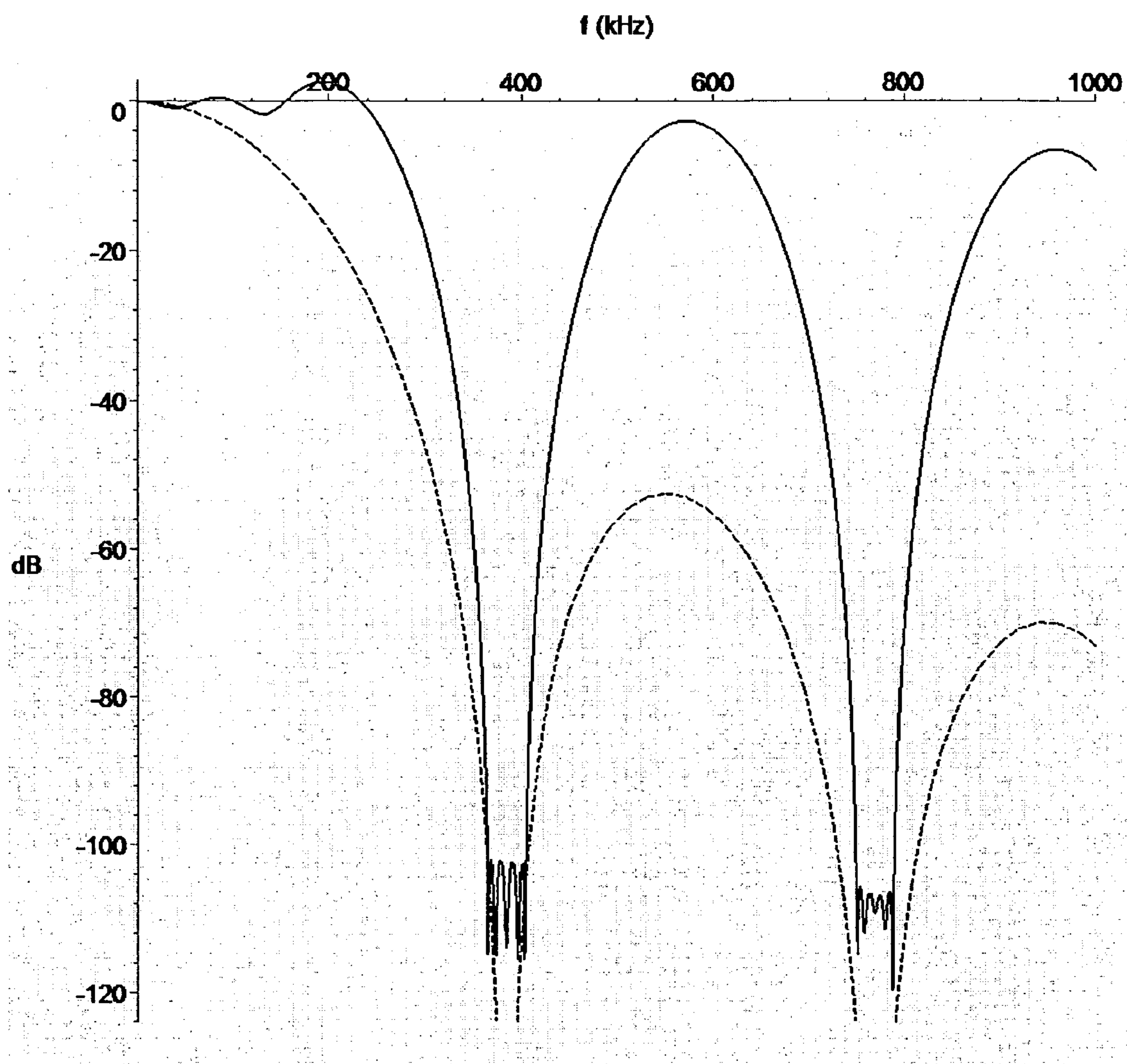
Figure 7: Amplitude response of 80-tap FIR decimation filter and (dashed) of cascade of four combs.
