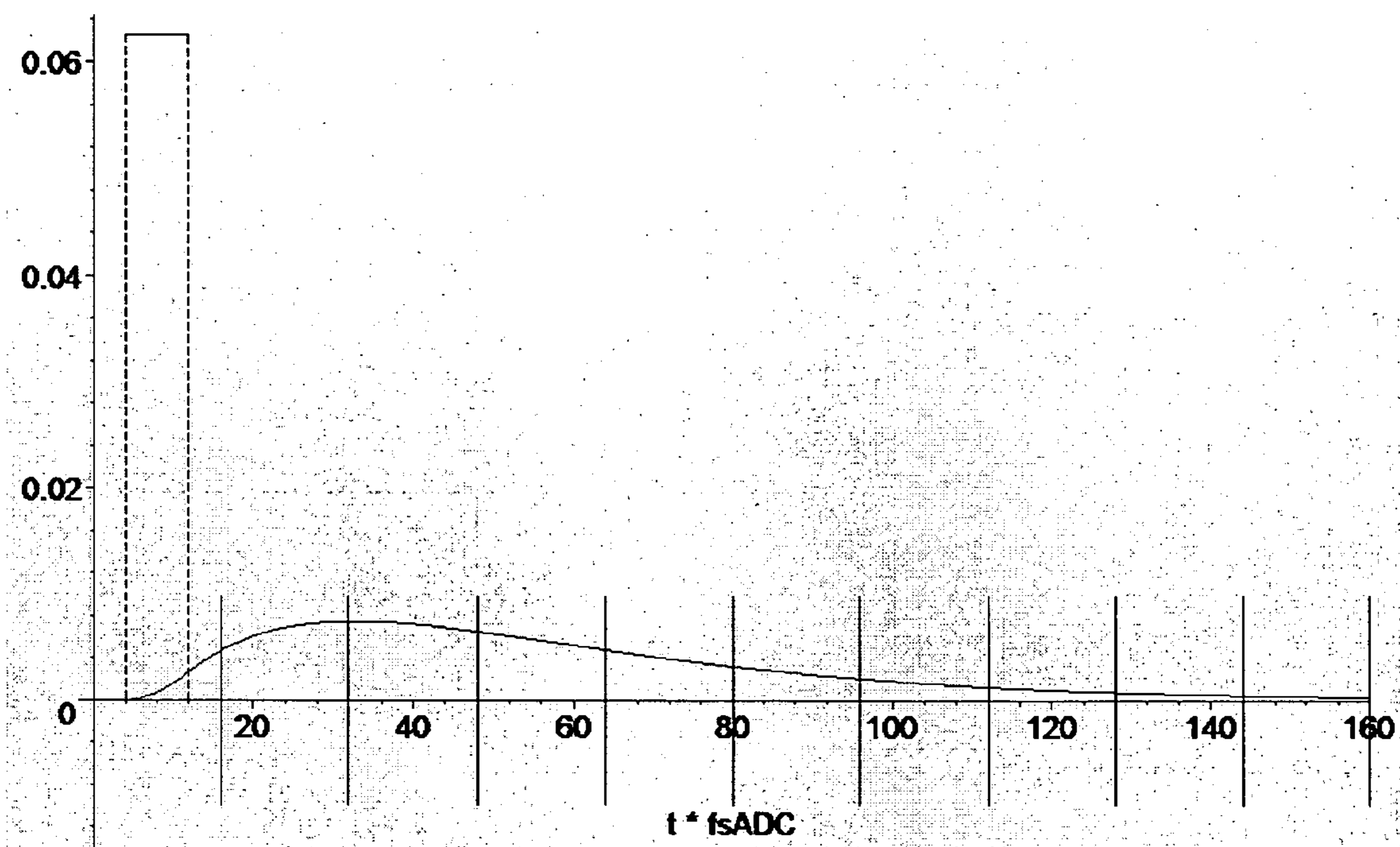
Figure 14: Response of analog lowpass filter to PWM pulse.
