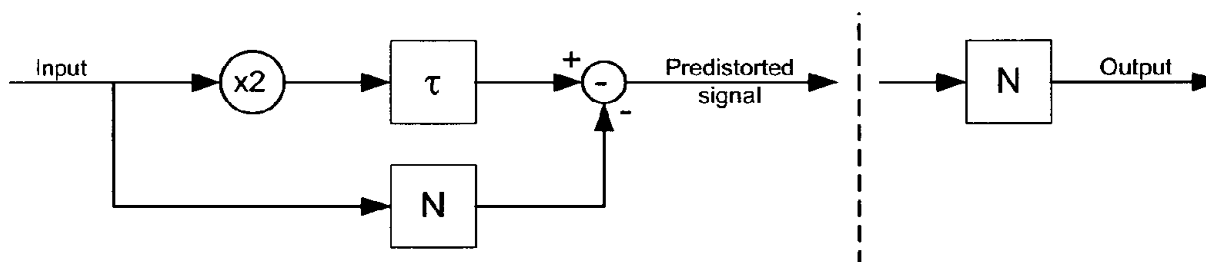
Figure 27: Gerzon first-order predistortion applied to nonlinear element N that approximates delay \tau .
