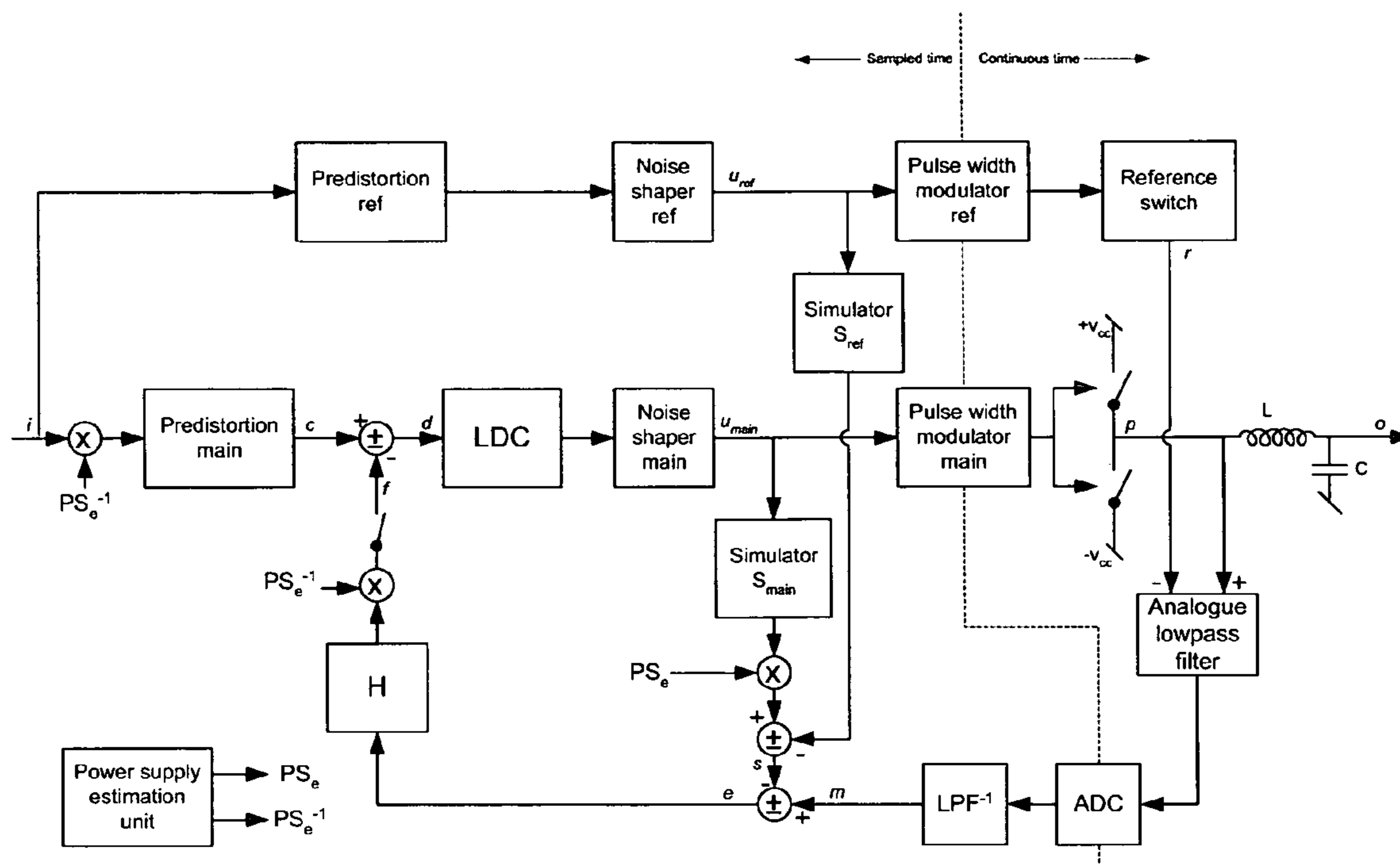
Figure 35: Amplifier with reference path.
