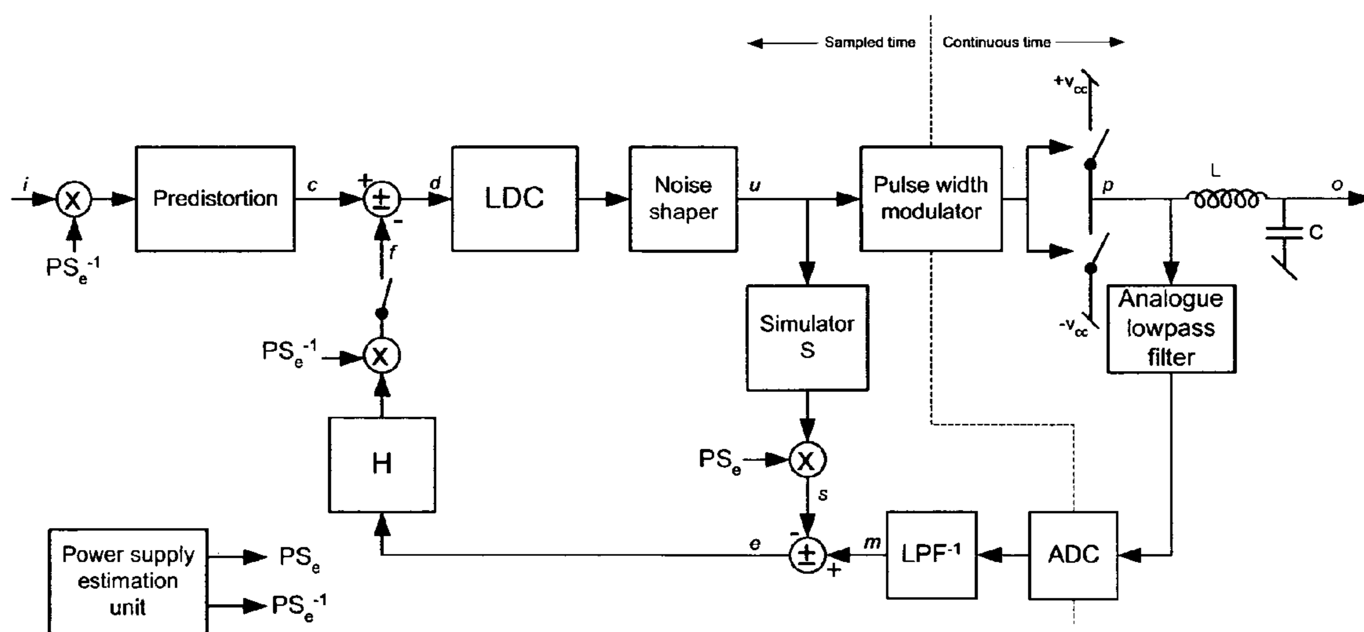
Figure 34: Amplifier with compensation for the effect of power supply variations.
