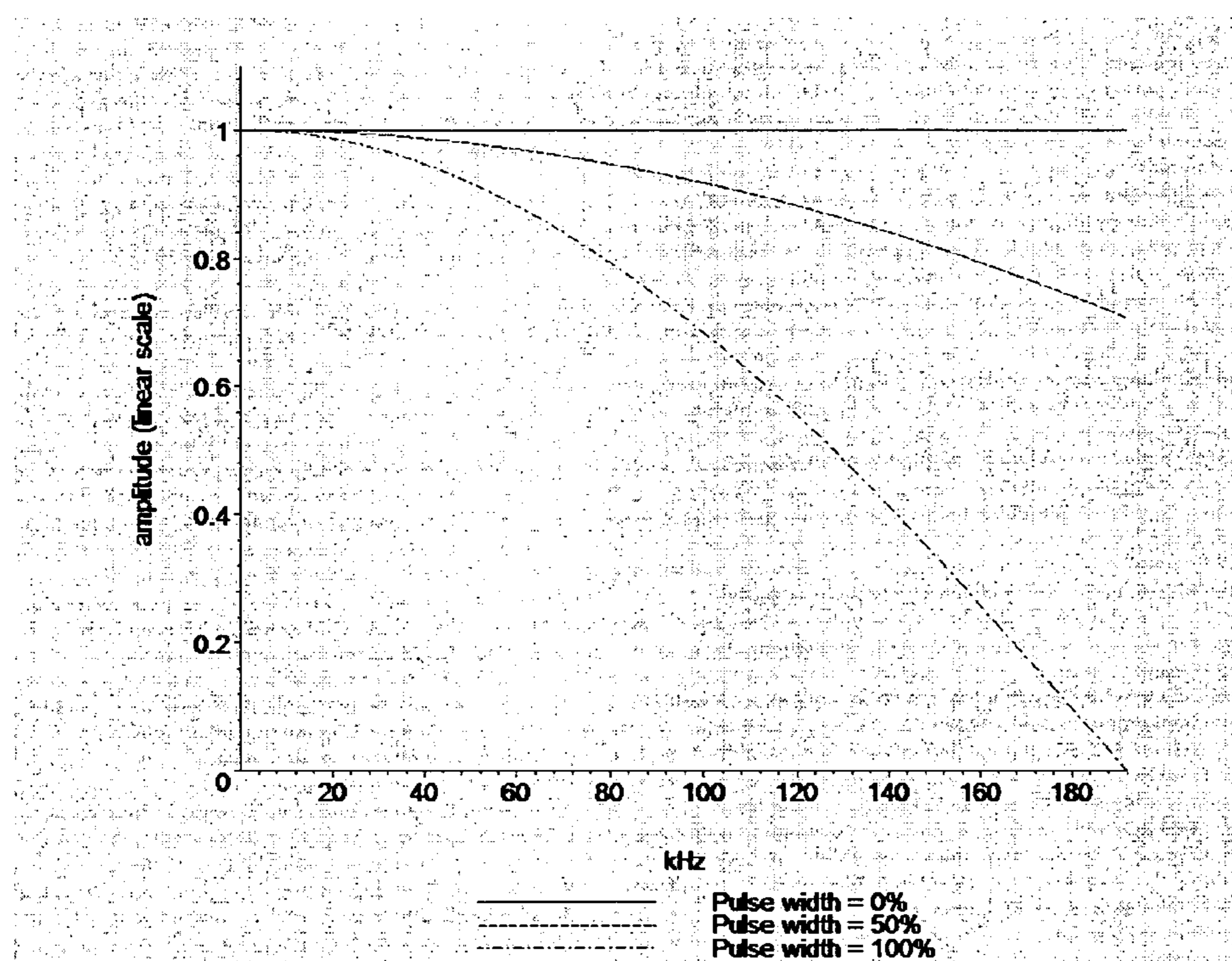
Figure 2: Small signal amplitude response of double edge (class AD or class BD) PWM modulator operating at 384kHz, with pulse width, as a percentage of the pulse repetition period, as parameter.
