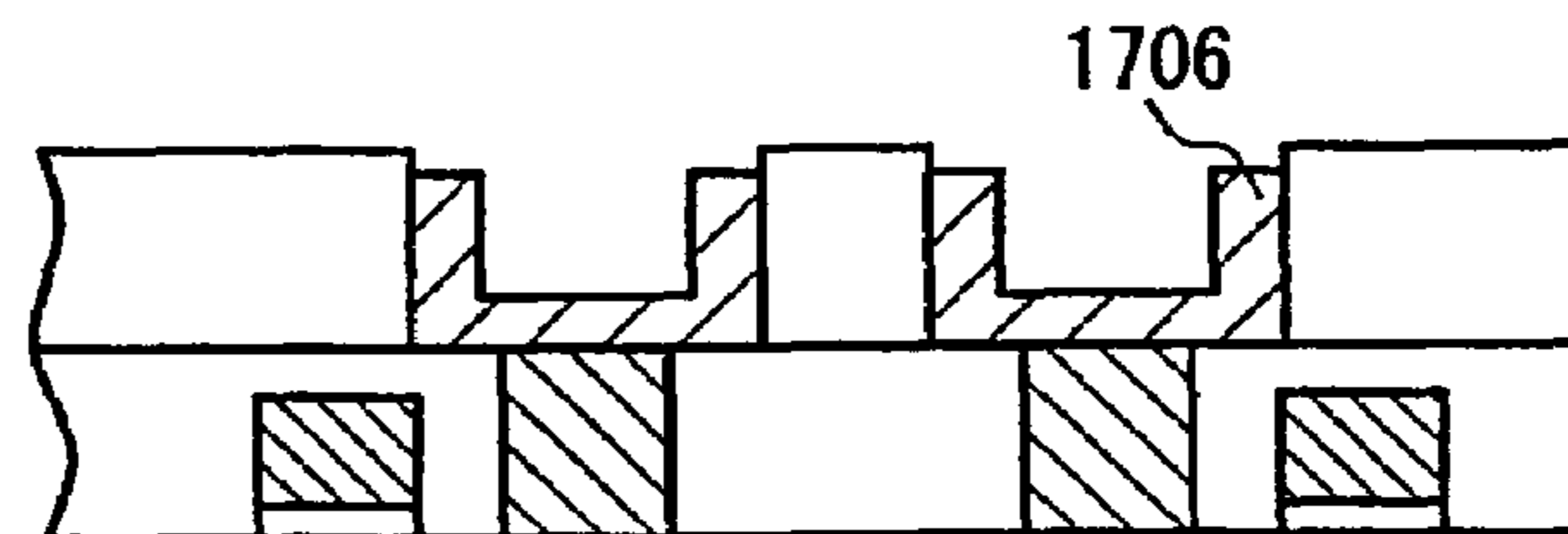
FIG. 17D PRIOR ART
