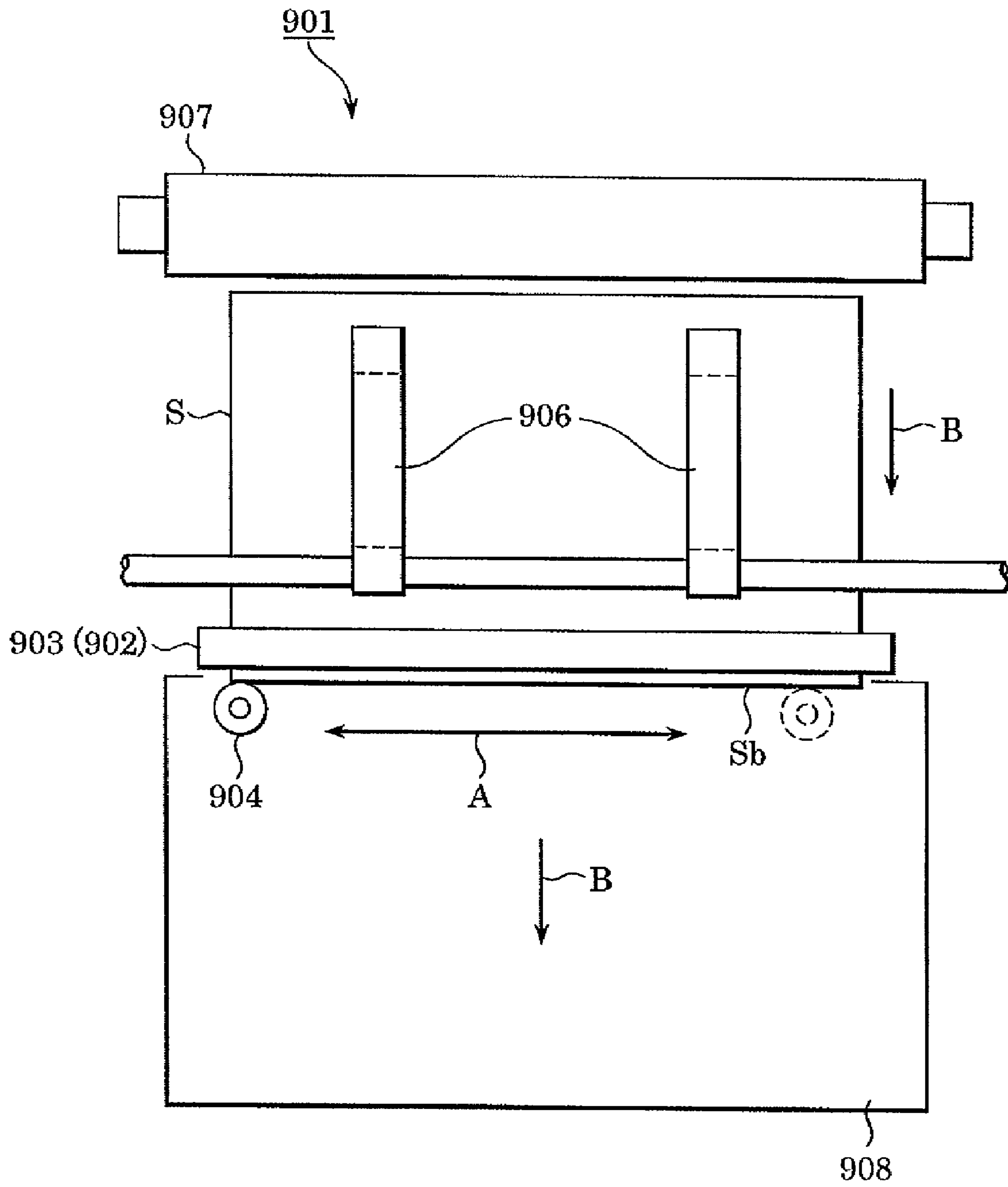
FIG. 15 PRIOR ART
