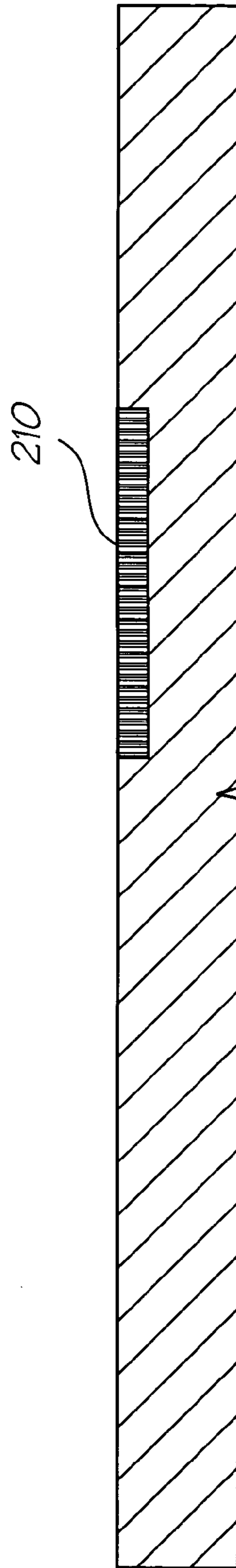
Implant N-Well
