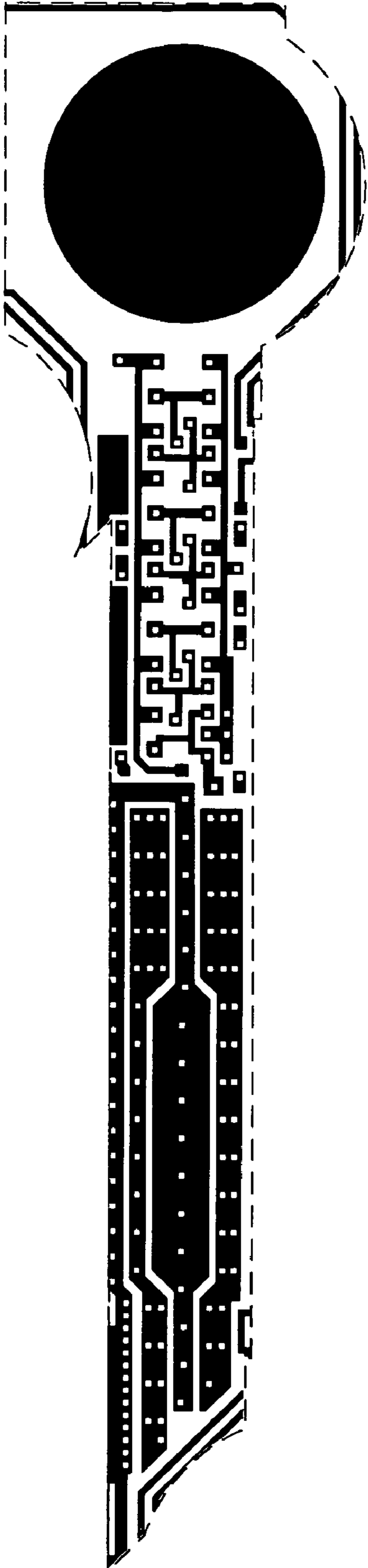
Metal 1 mask
