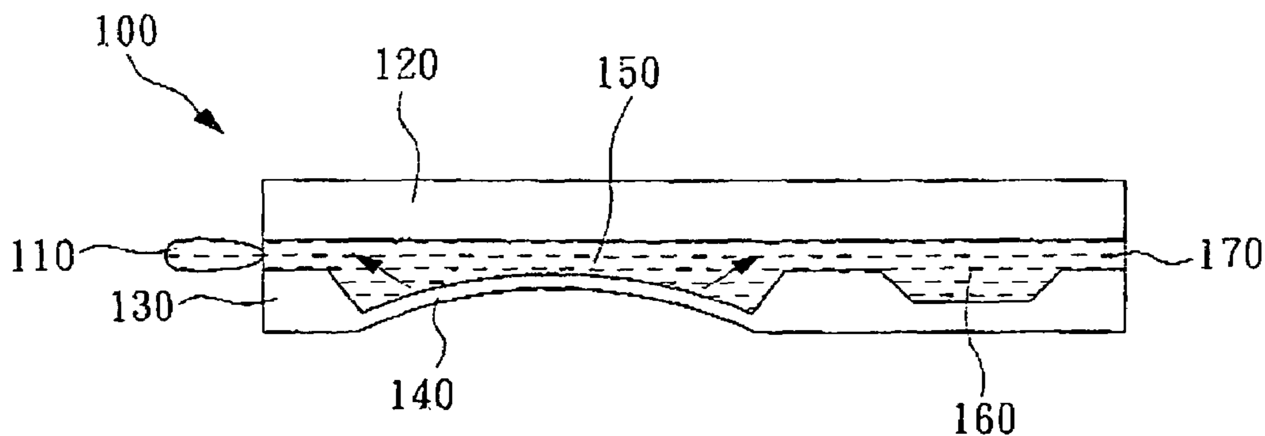
FIG. 1C (PRIOR ART)
