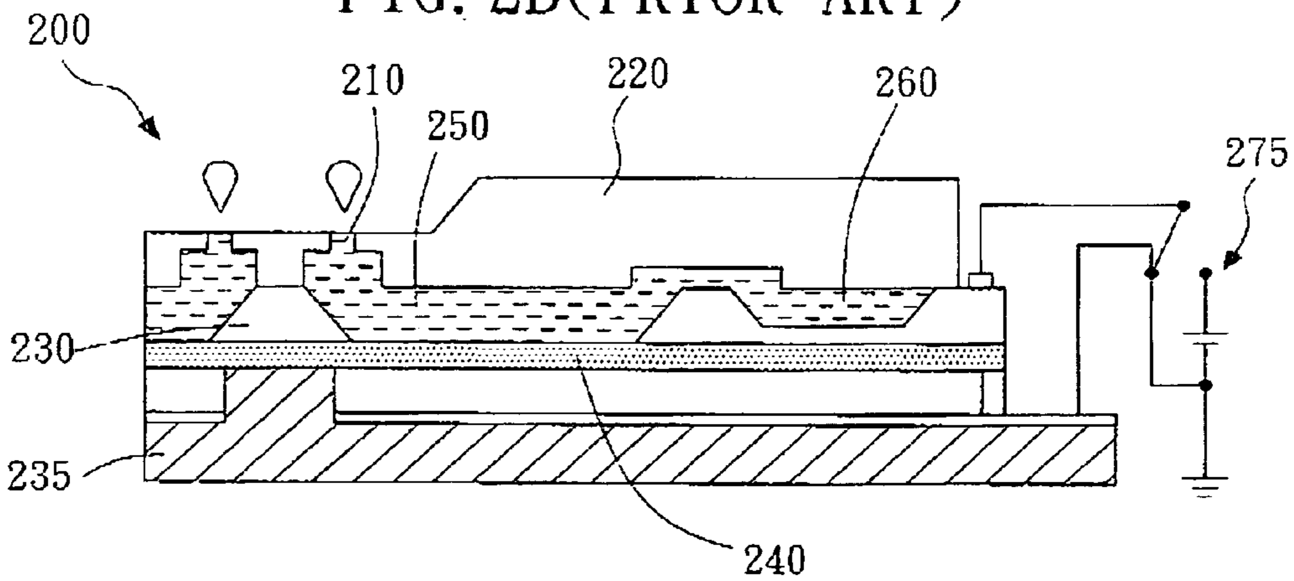
FIG. 2C(PRIOR ART)
