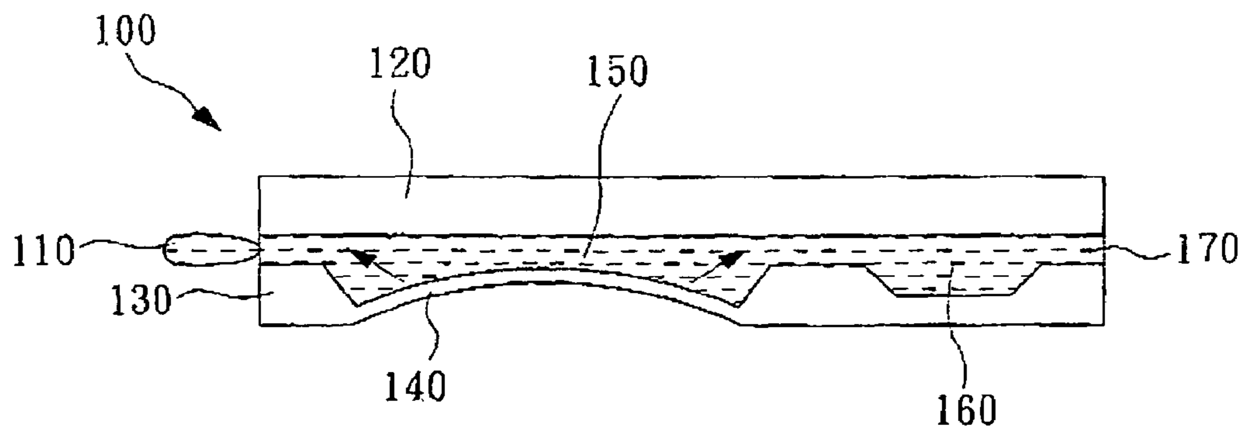
FIG. 1C (PRIOR ART)
