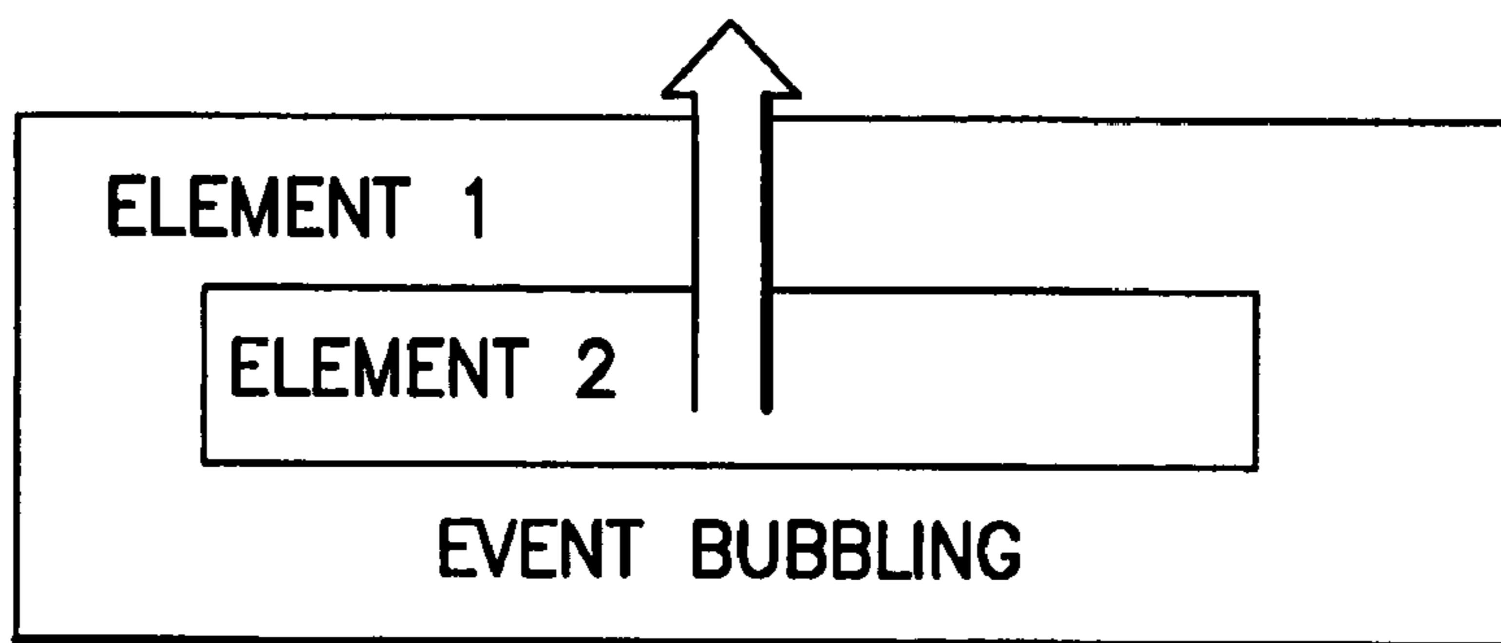
FIG.3A EVENT BUBBLING
