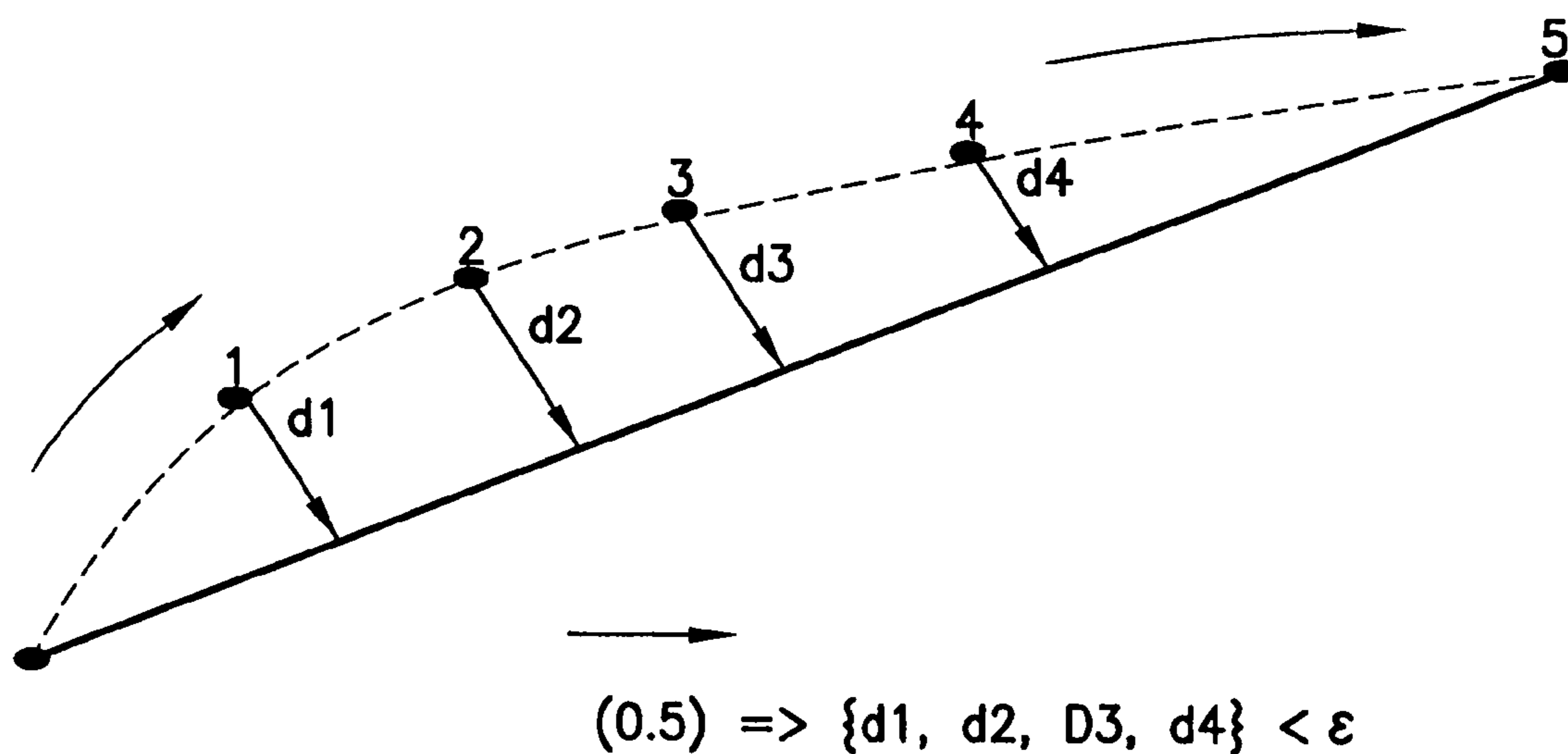
FIG.5 DIGITAL INK COMPRESSION
