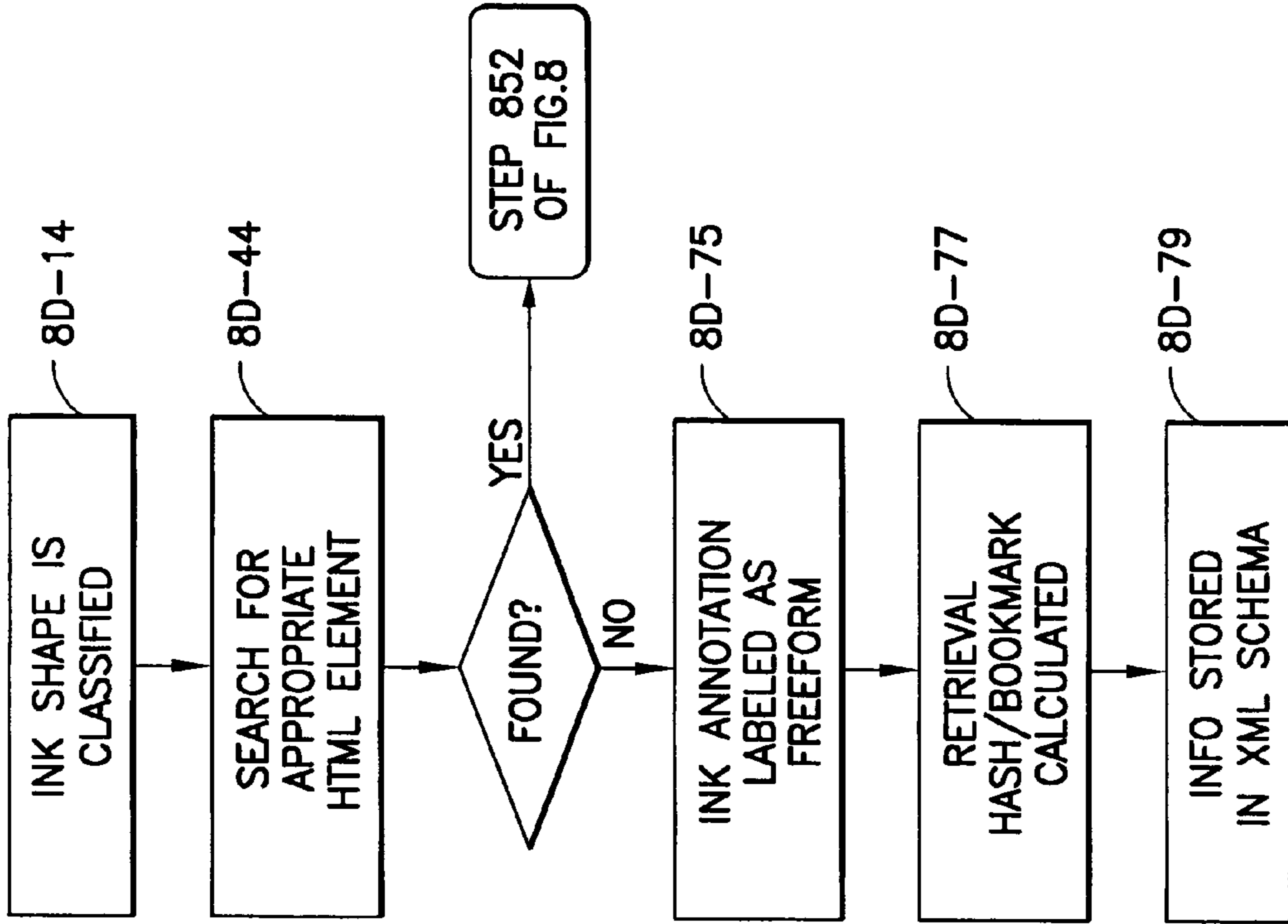
FIG. 8D NO NEARBY ELEMENT
