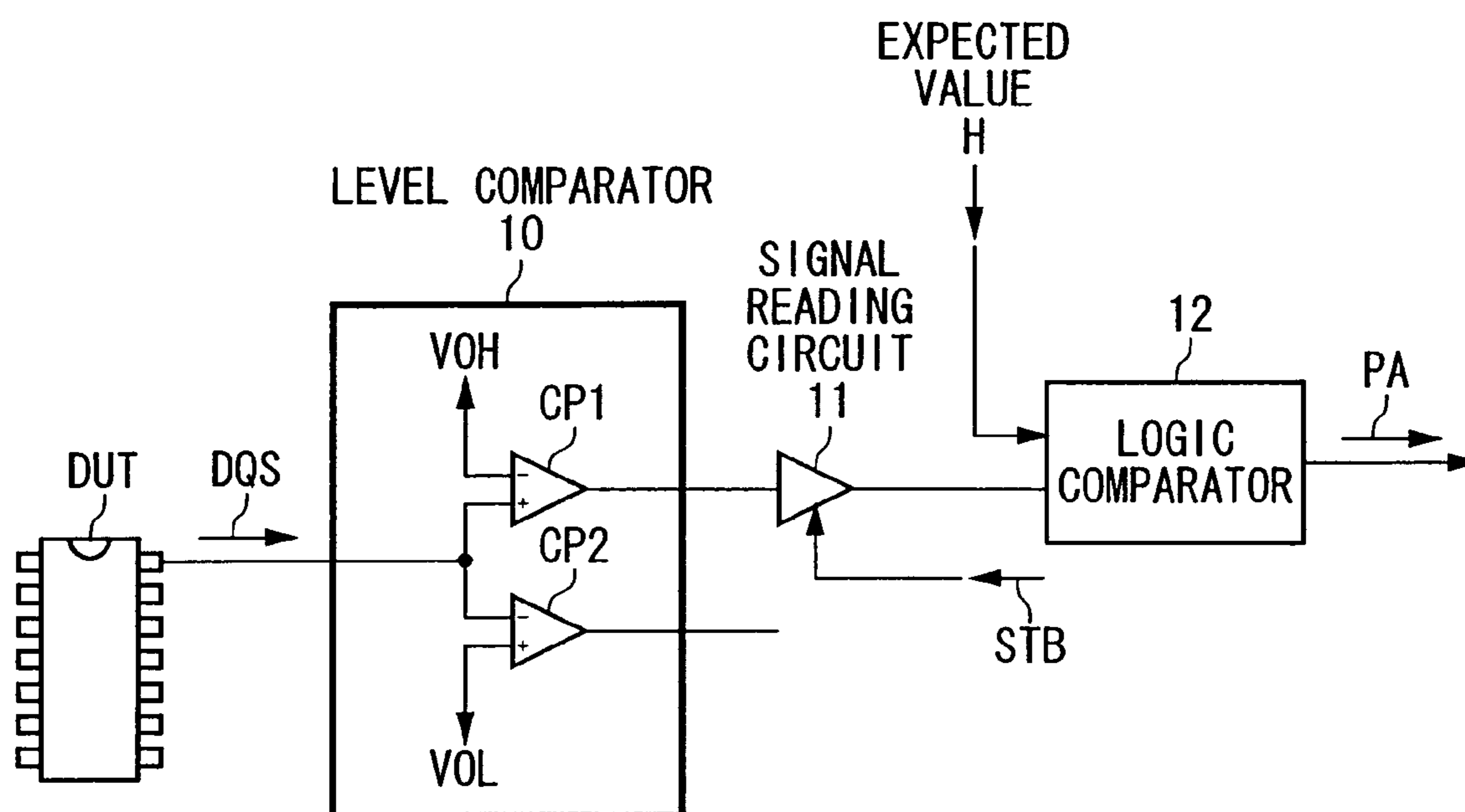
FIG. 28 (Prior Art)
