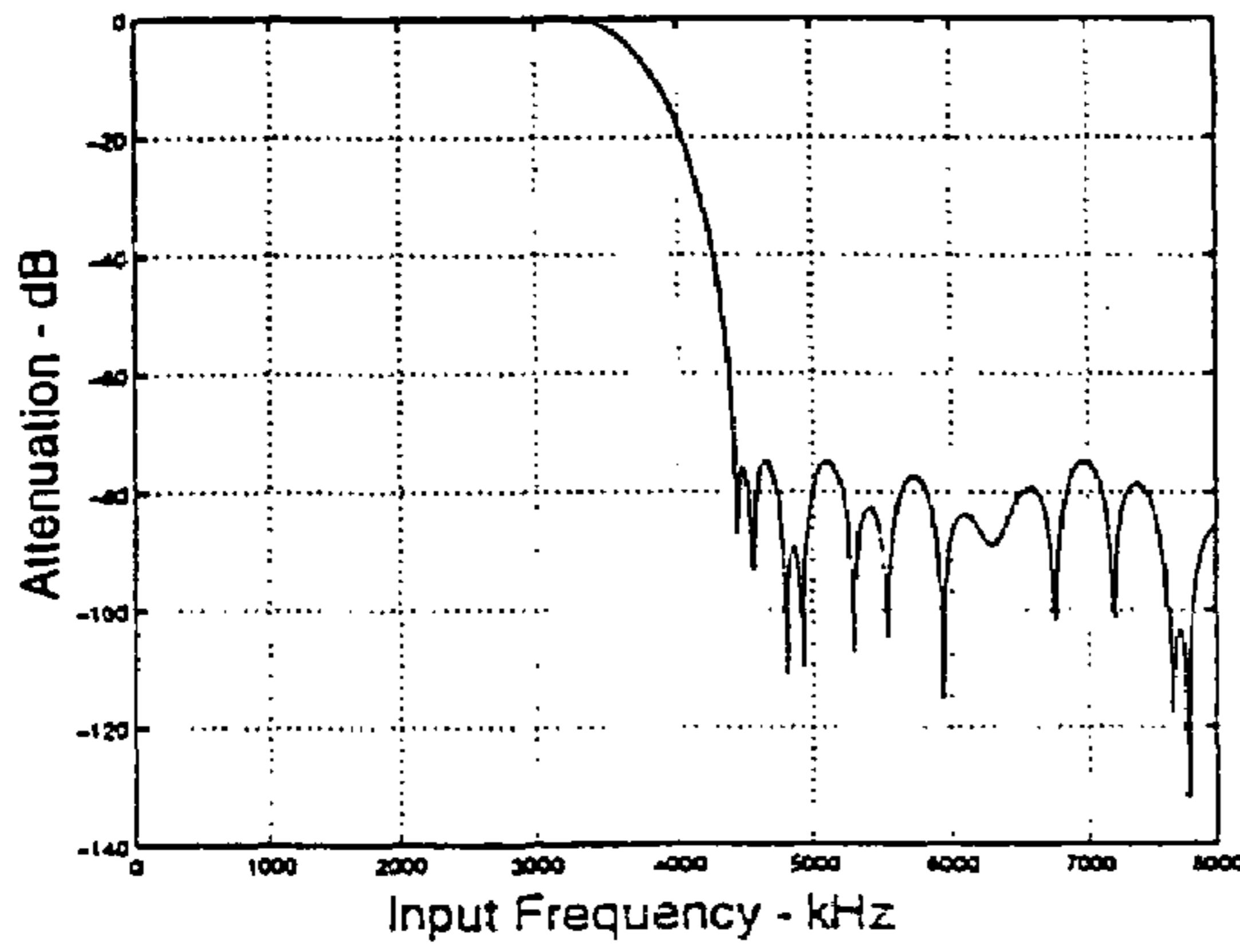
Figure 4. Decimation Filter Response
