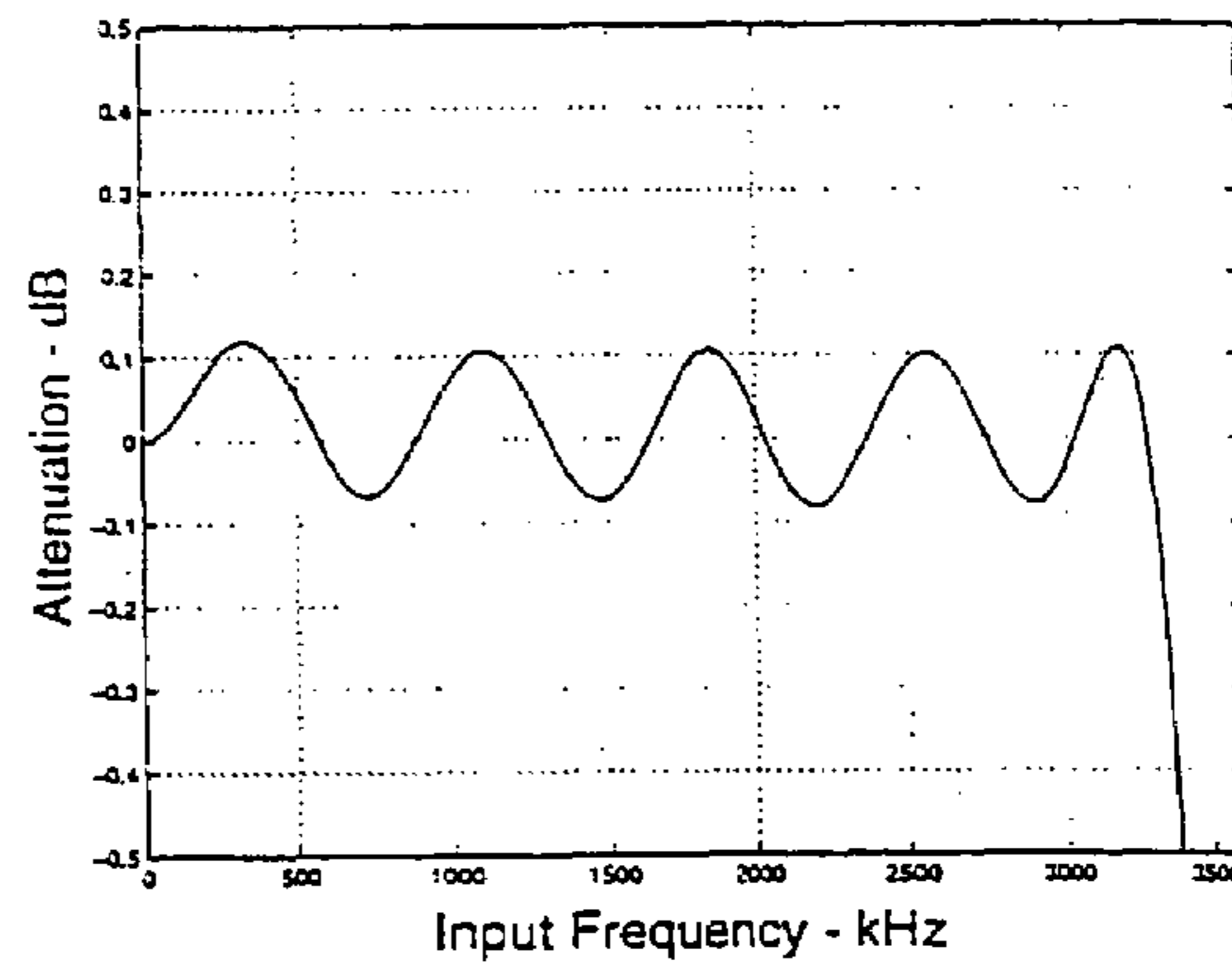
Figure 7. Interpolation Filter Passband Ripple
