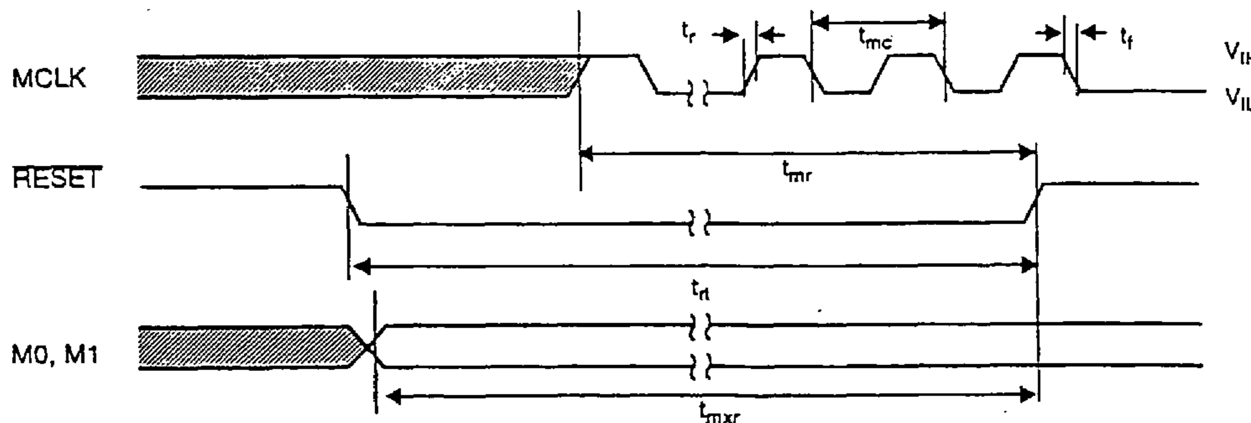
Figure 1. General Inputs Timing Diagram
