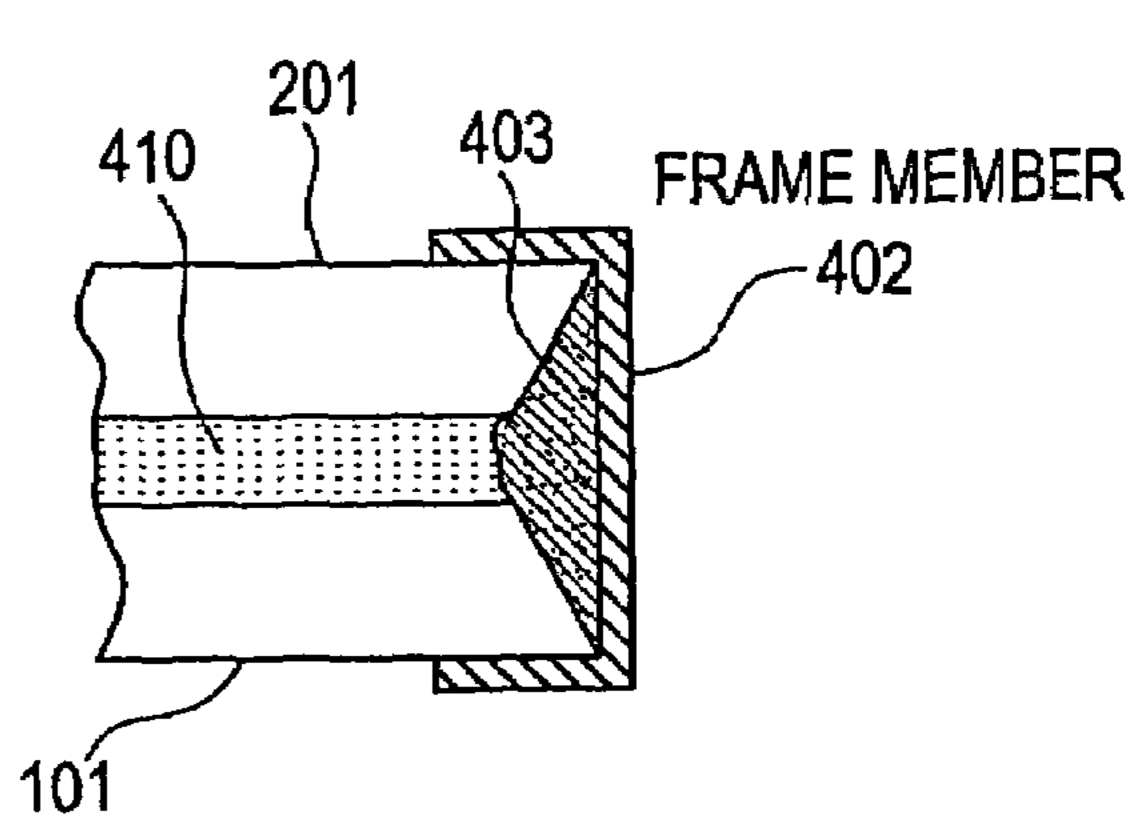
SECTIONAL VIEW OF PORTION a
