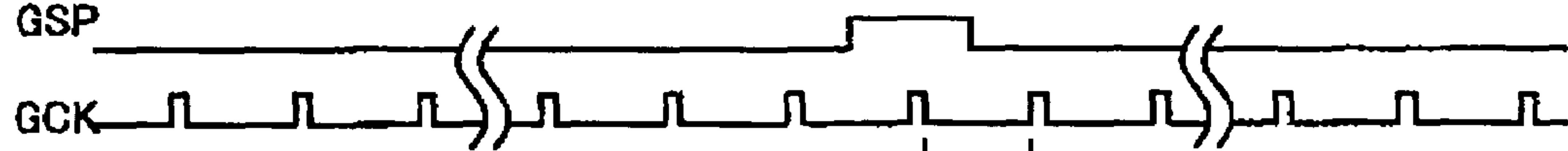
FIG. 26 (f) (PRIOR ART)
