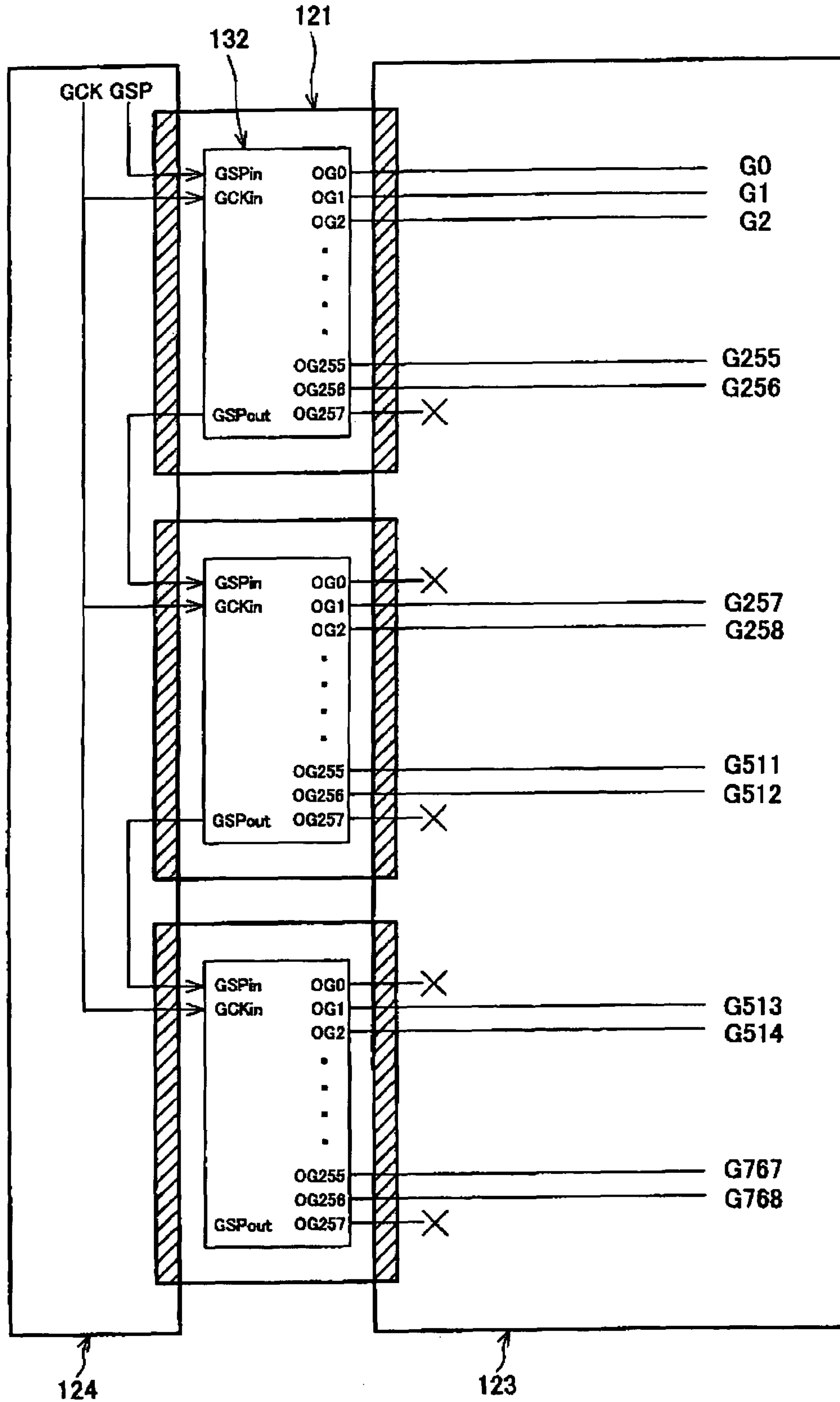
FIG. 29 (PRIOR ART)
