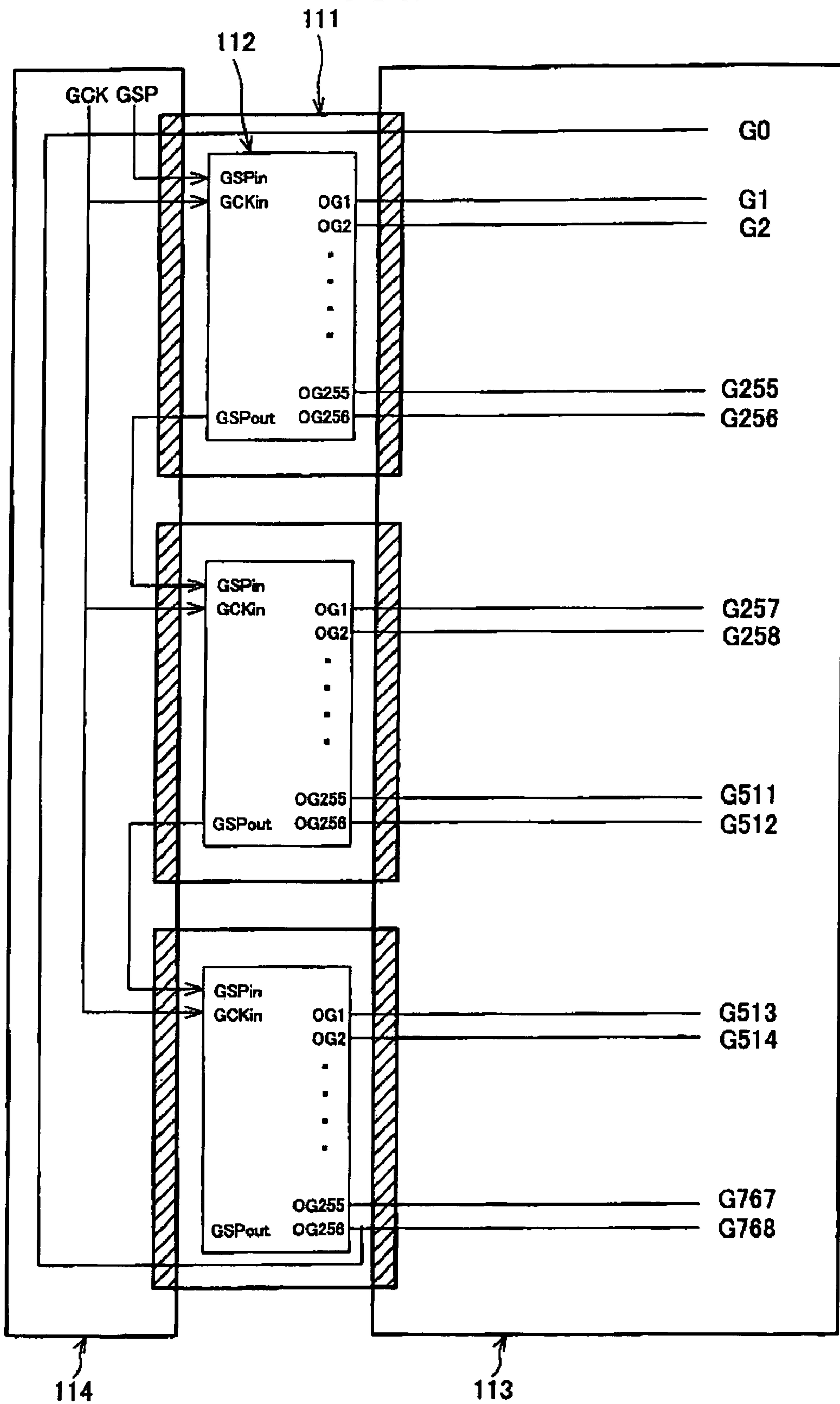
FIG. 21 (PRIOR ART)
