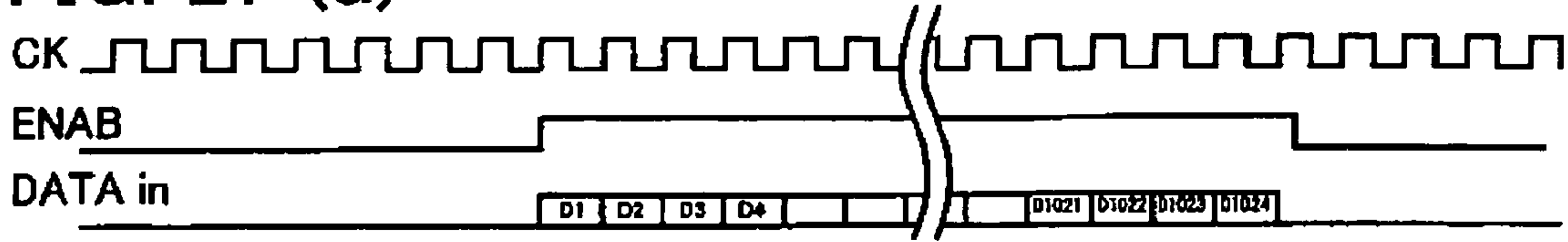
FIG. 27 (b) (PRIOR ART)
