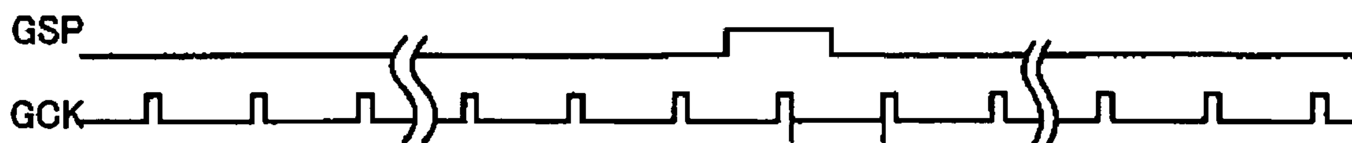
FIG. 27 (e) (PRIOR ART)
