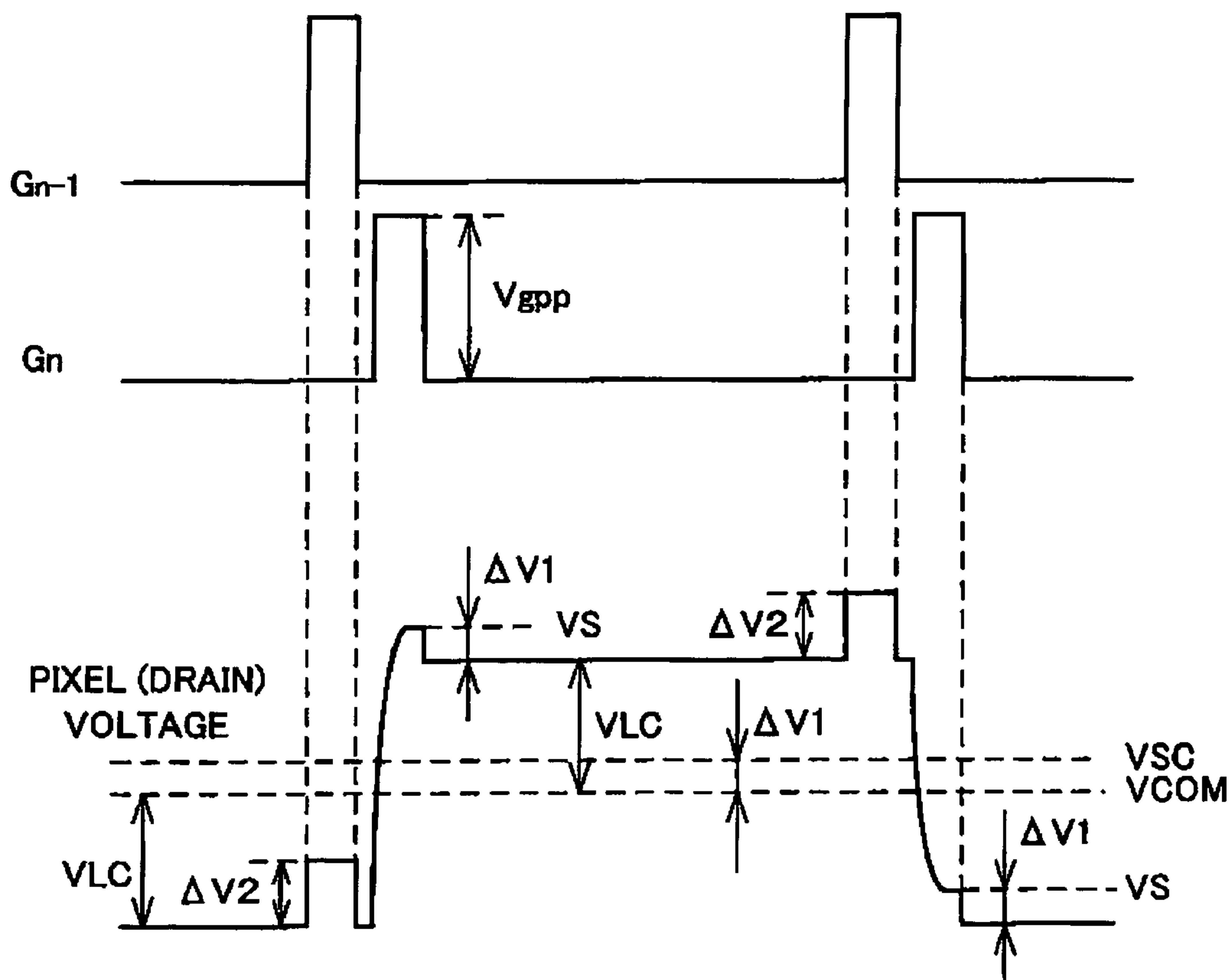
FIG. 20 (PRIOR ART)
