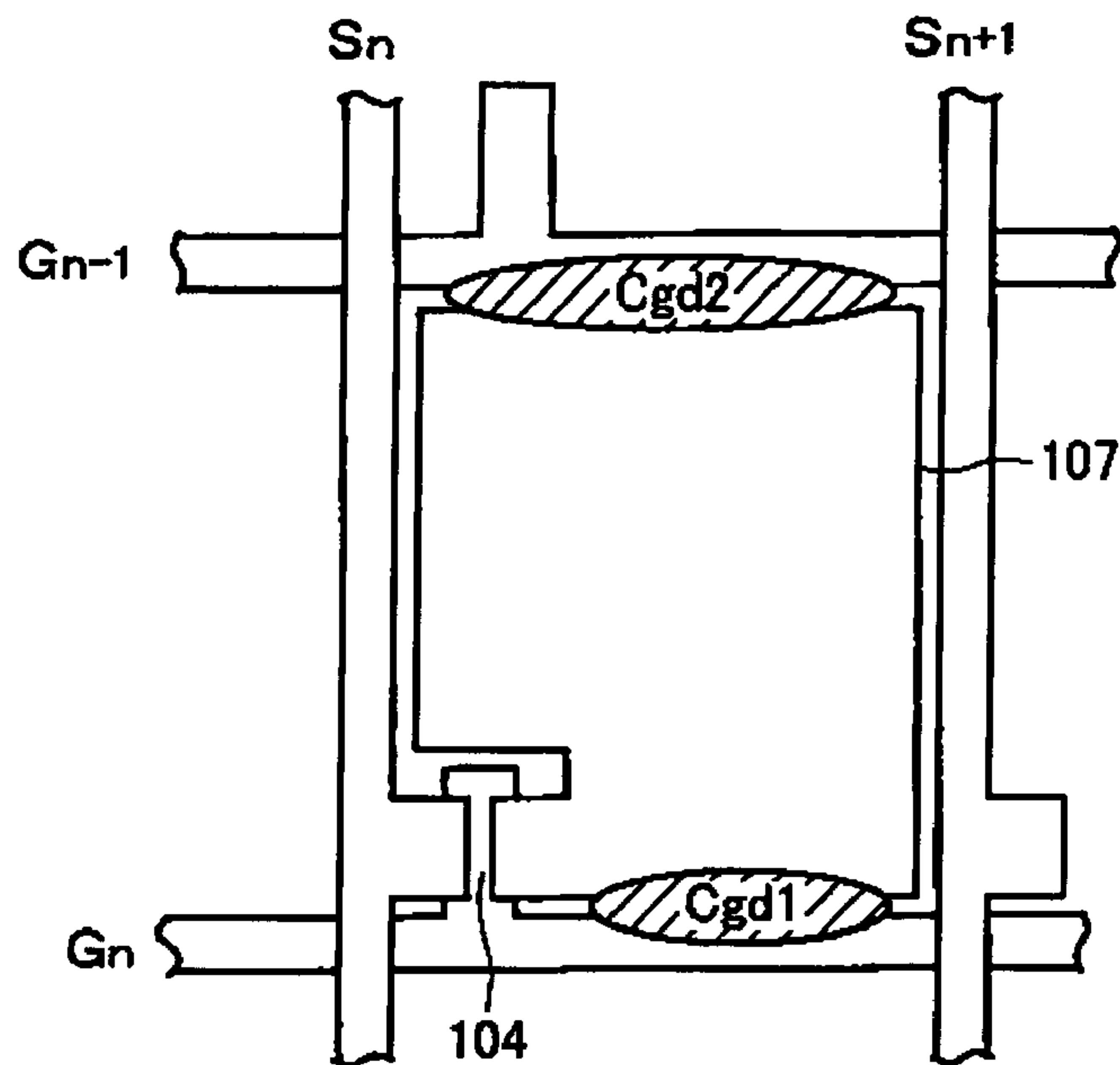
FIG. 20 (PRIOR ART)
