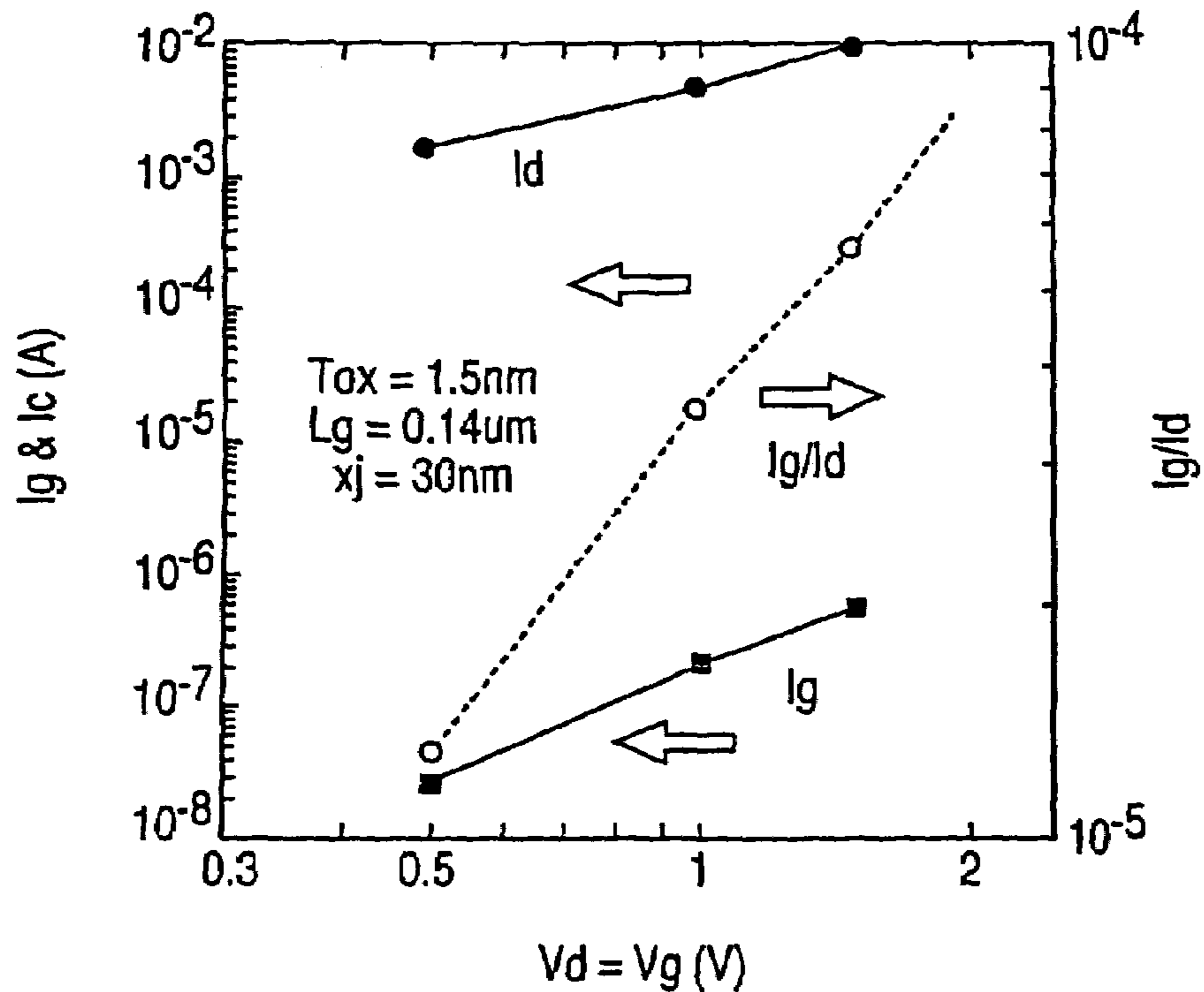
DEPENDANCE OF CURRENT I_g AND I_d UPON SUPPLY VOLTAGE V_d = V_g
