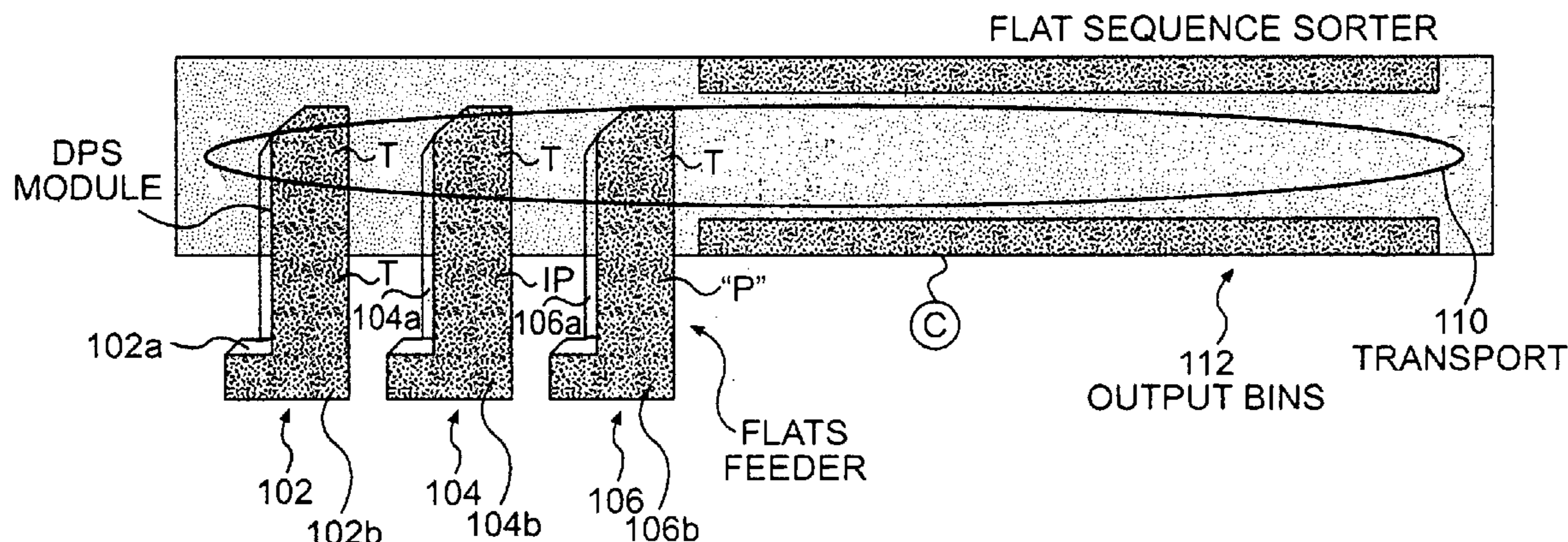
FLATS SEQUENCE SORTER WITH THREE ADDED DPS MODULES
