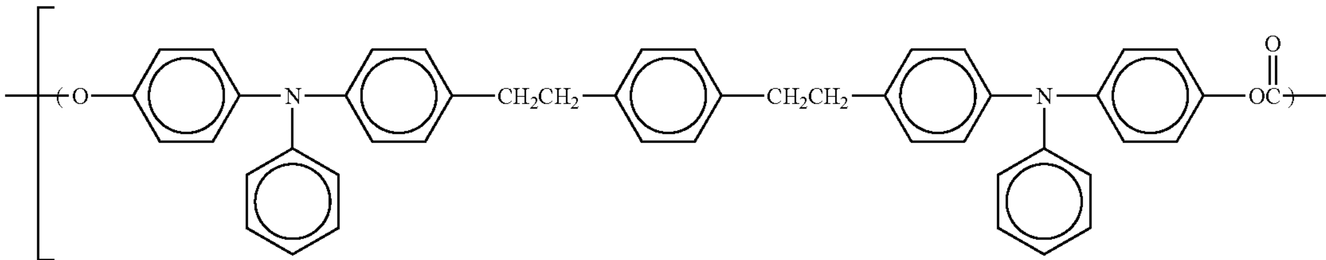
Specific compound 24
