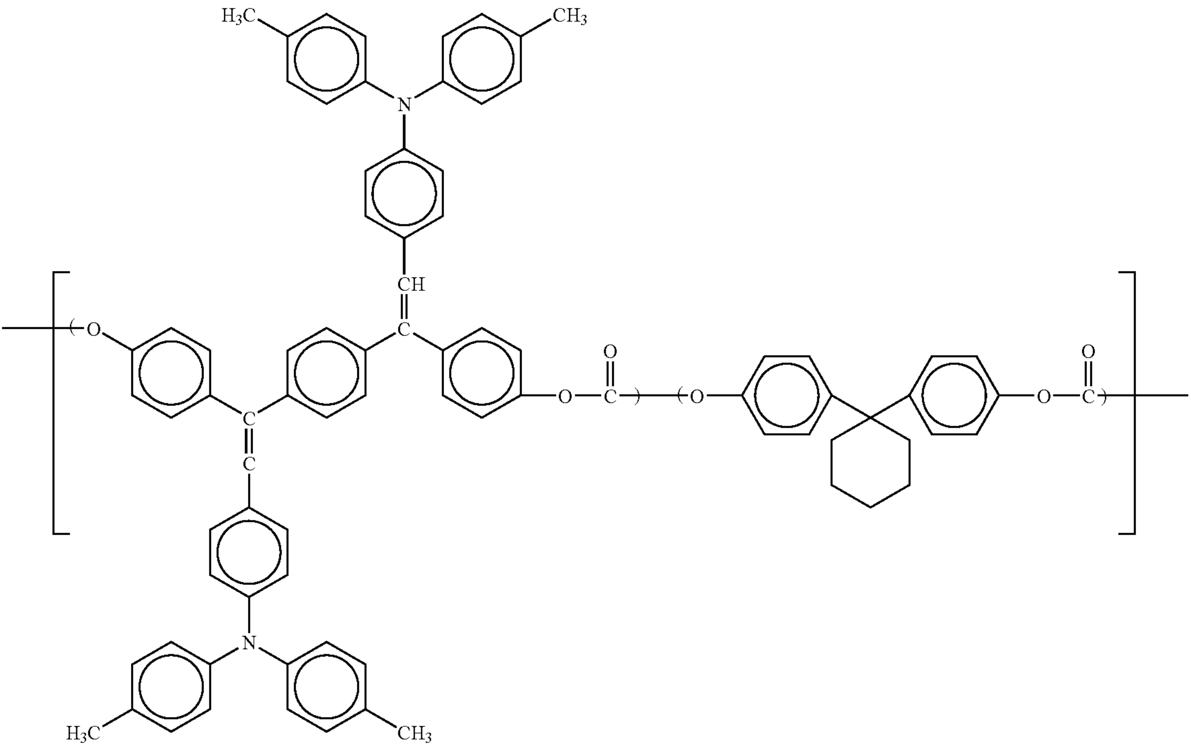
Specific compound 27
