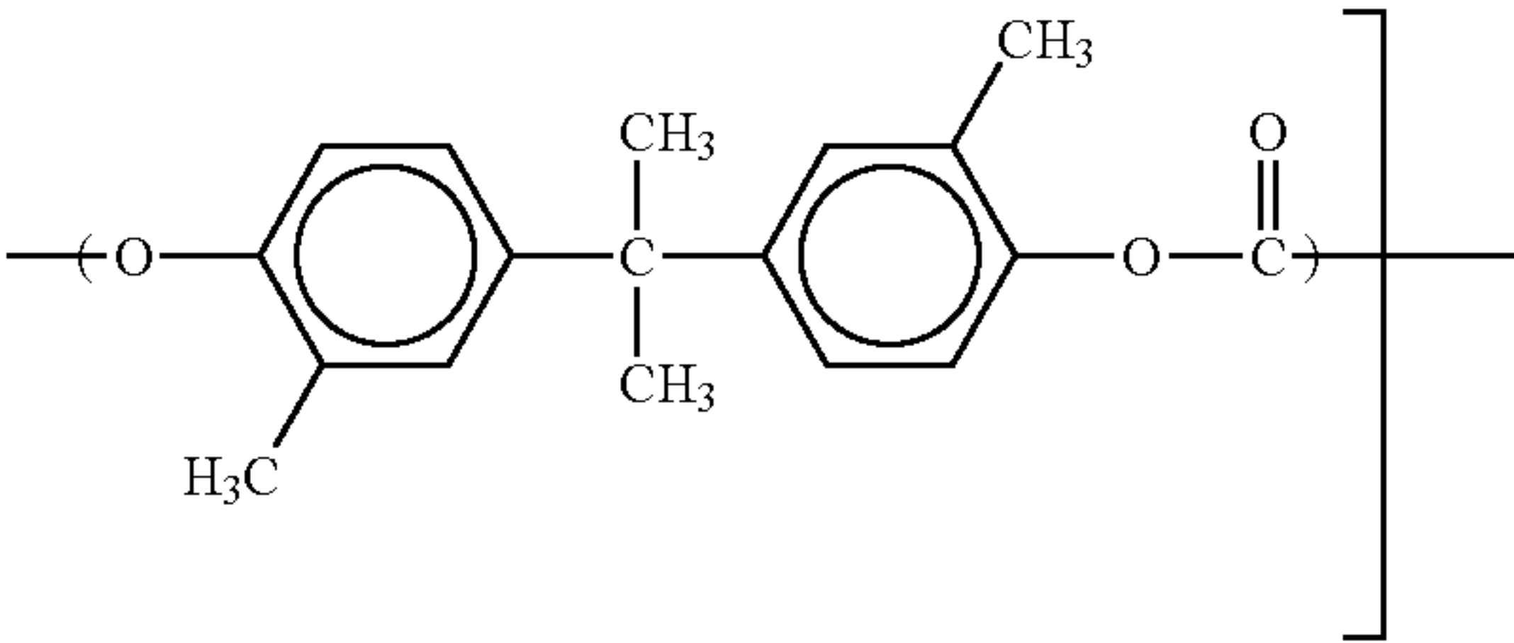
Specific compound 27
