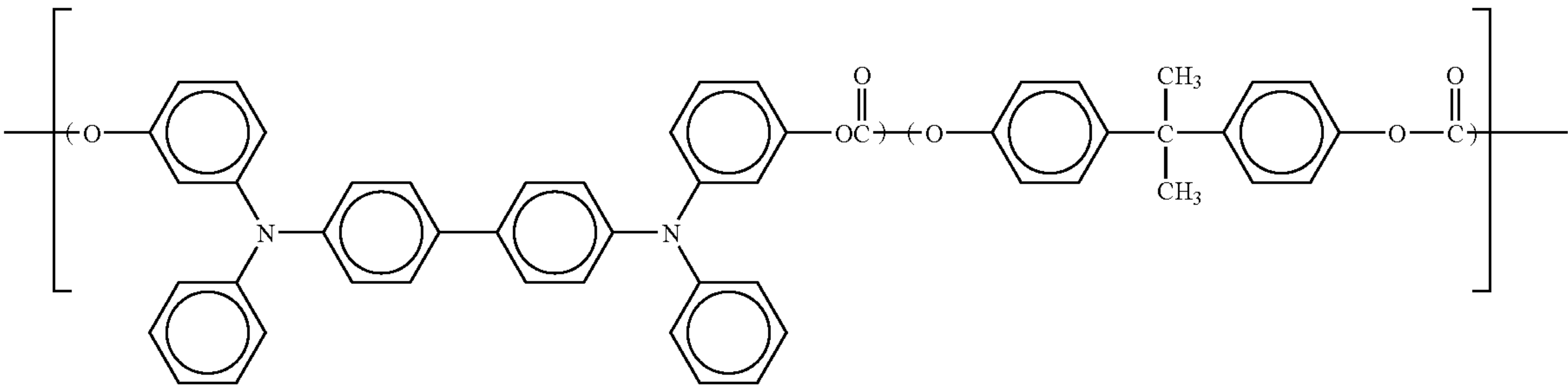
Specific compound 23
