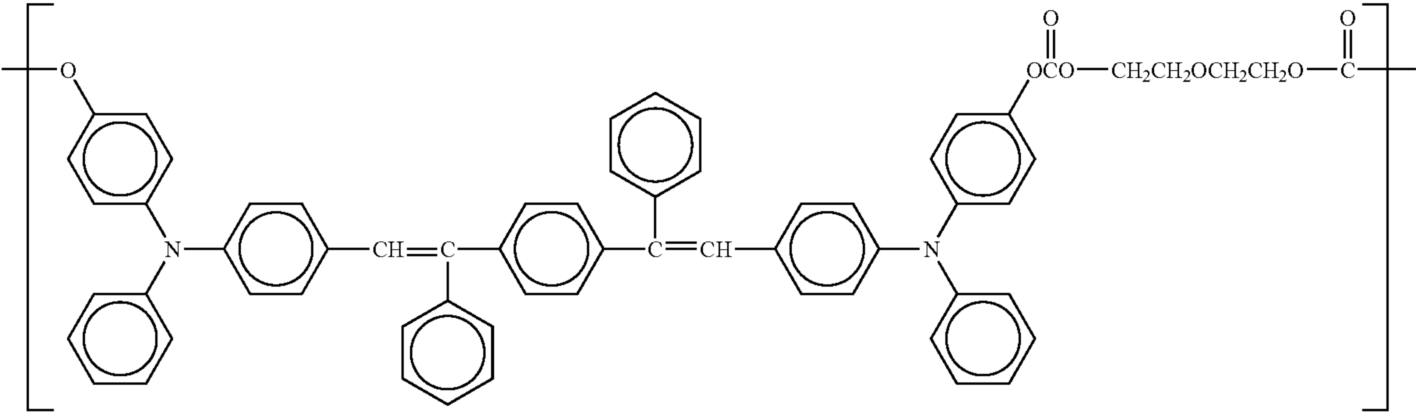
Specific compound 26
