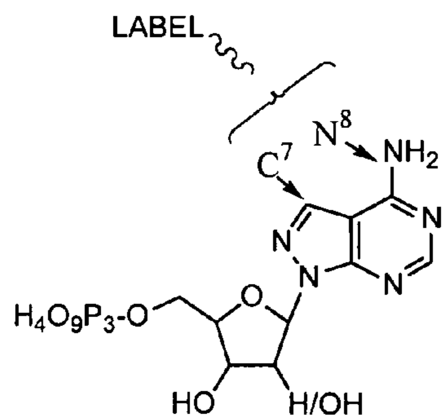
A/dA analogs
