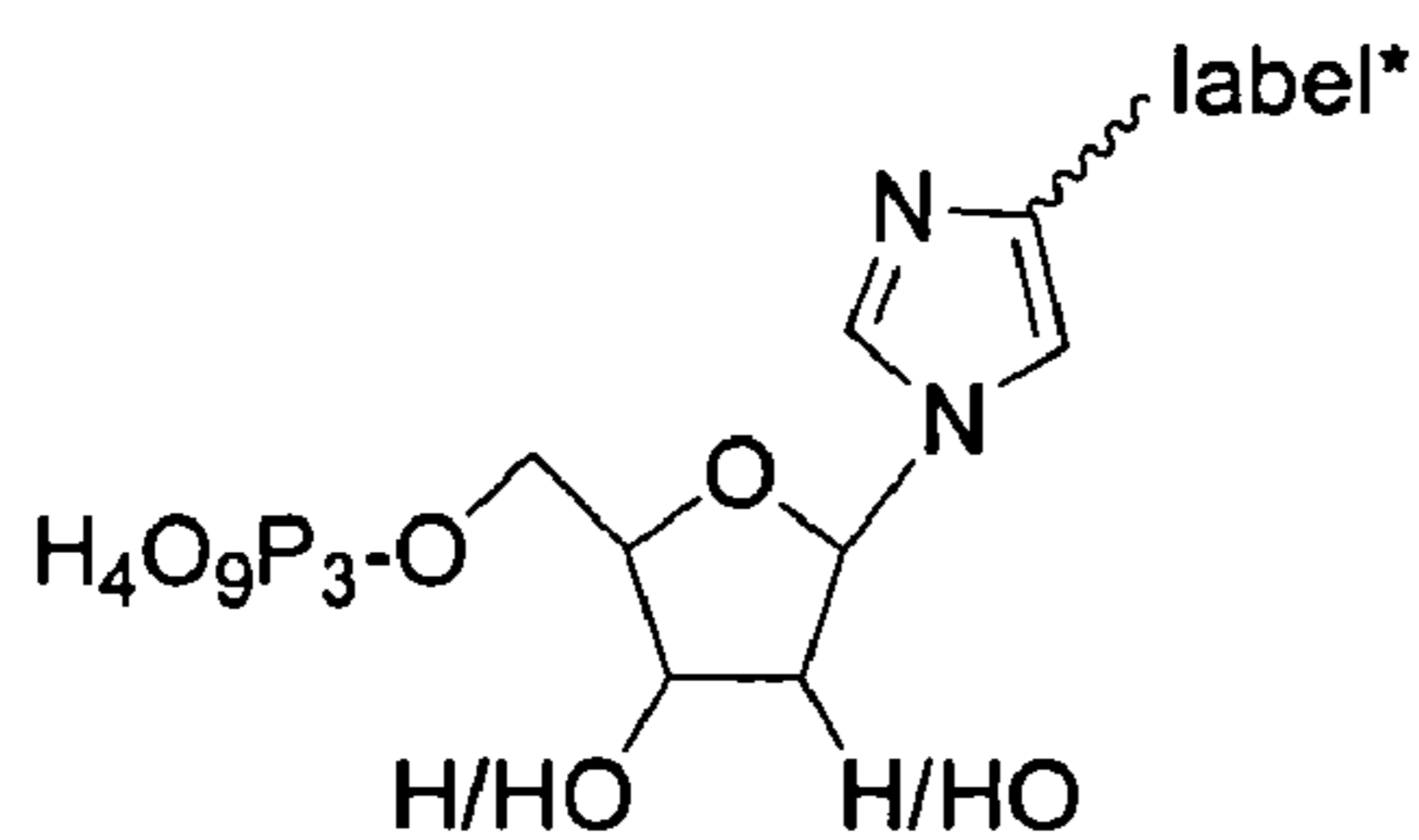
Imidazole
