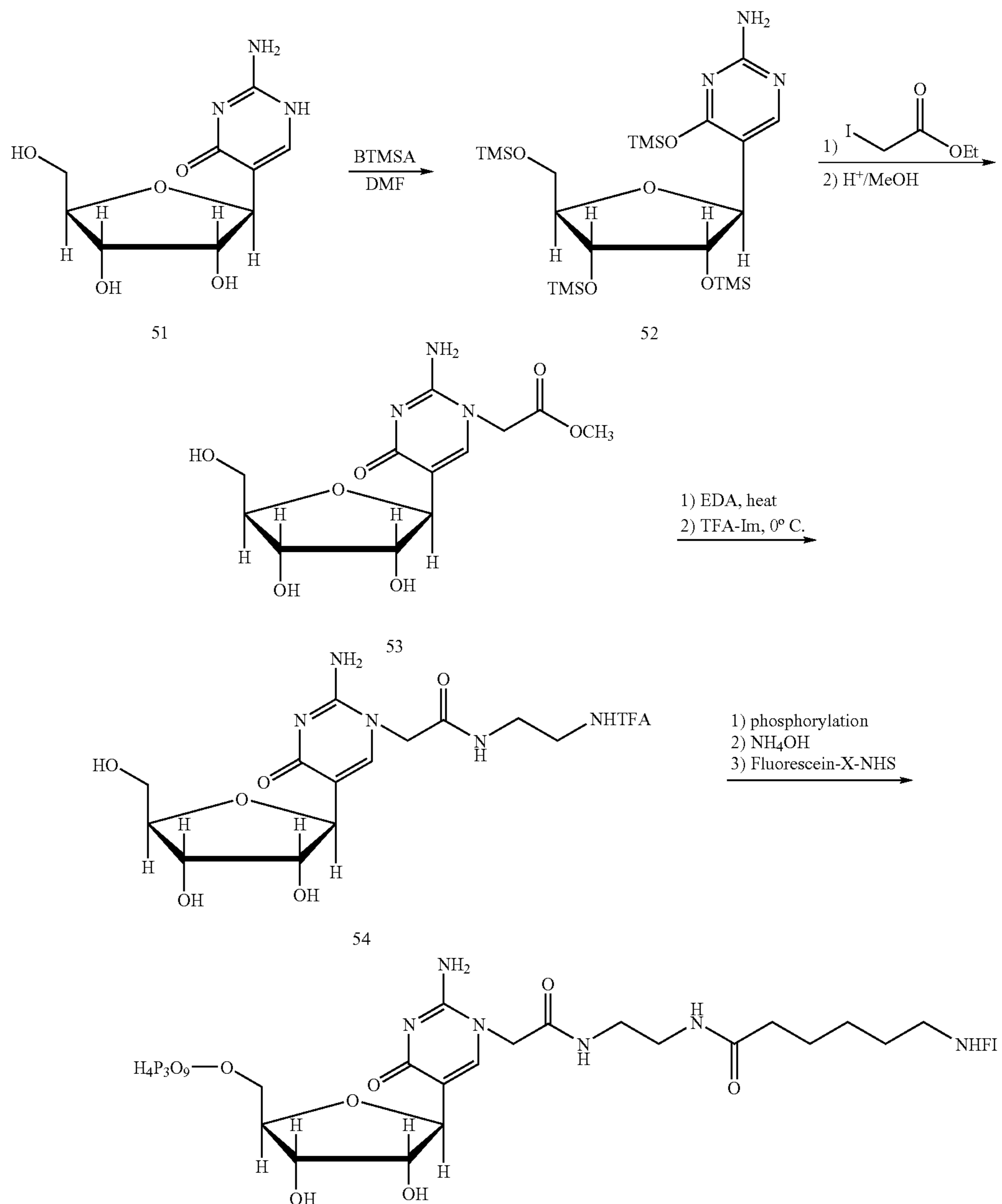
Scheme 2
