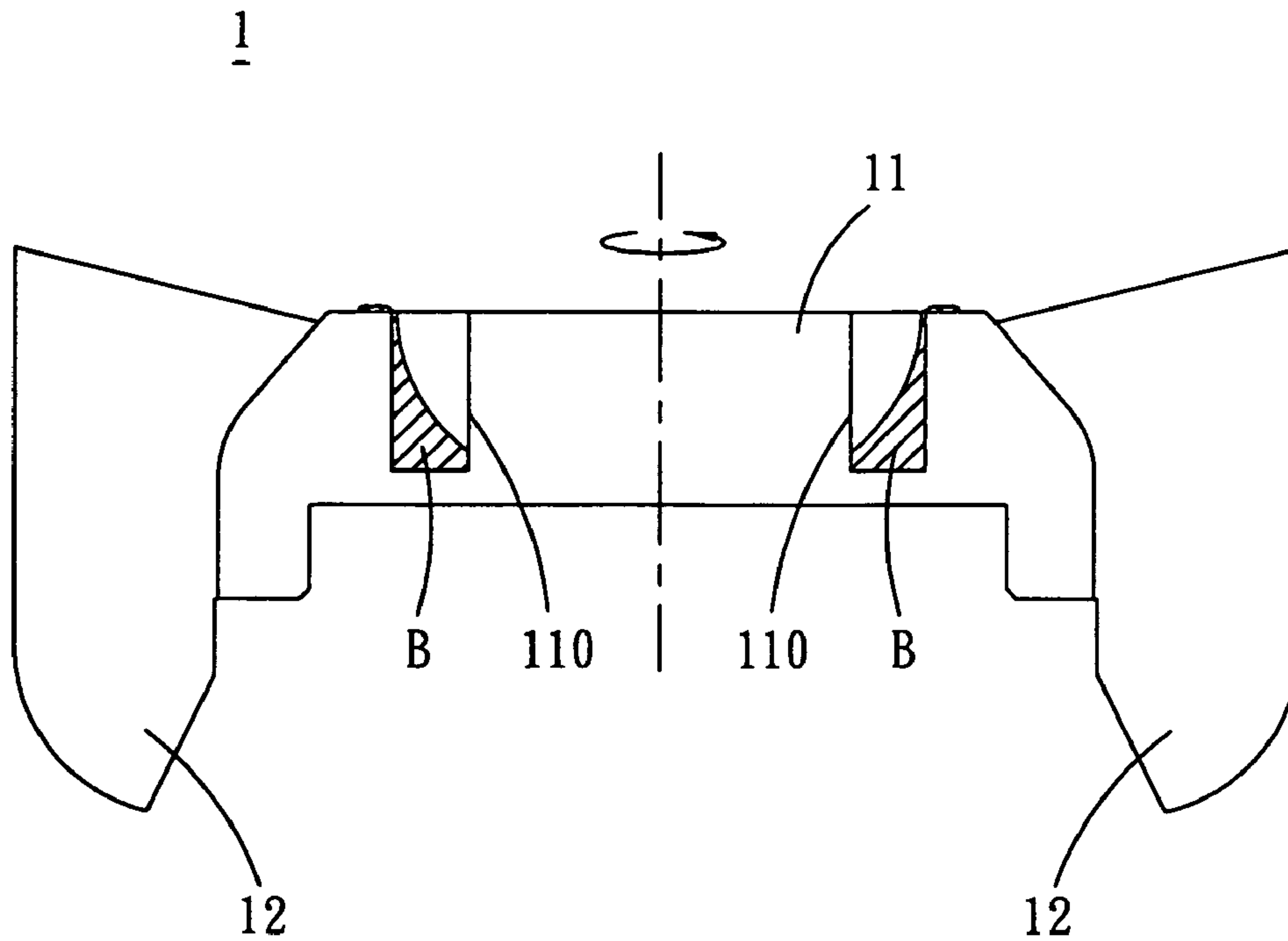
FIG. 2 (PRIOR ART)
